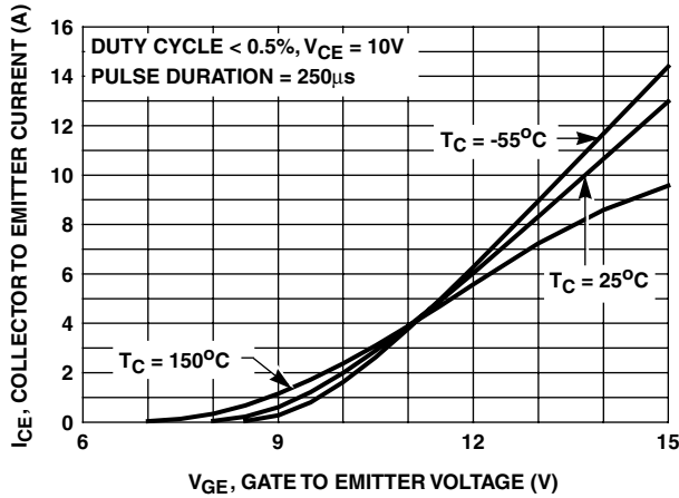
FIGURE 13. TRANSFER CHARACTERISTIC
