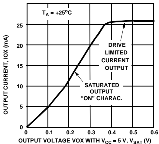
FIGURE 2. TYPICAL OUTPUT DRIVER SATURATED “ON” CHARACTERISTIC
