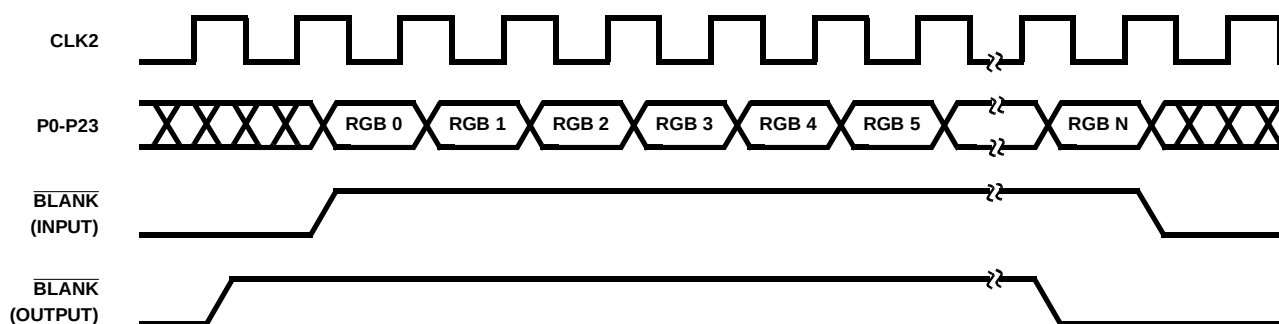
FIGURE 11. PIXEL AND OVERLAY INPUT TIMING - 24-BIT RGB WITH FLICKER FILTERING
