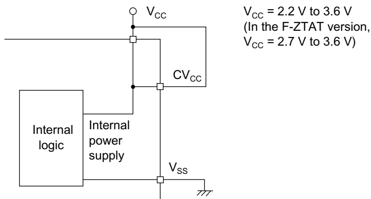
Figure 24.2 Power Supply Connection for H8S/2239, H8S/2238R, H8S/2237, and H8S/2227 (No Internal Power Supply Step-Down Circuit)
