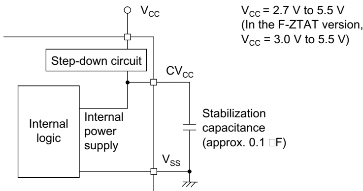
Figure 24.1 Power Supply Connection for H8S/2238B (On-Chip Internal Power Supply Step-Down Circuit)
