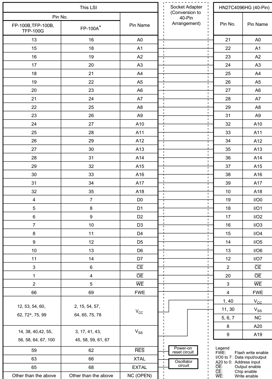
Figure 19.13 Socket Adapter Pin Correspondence Diagram
