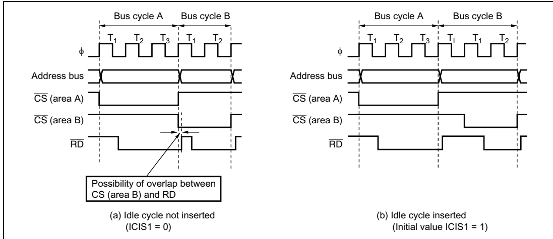
Figure 7.23 Relationship between Chip Select ( \overline{\text{CS}} ) and Read ( \overline{\text{RD}} )
