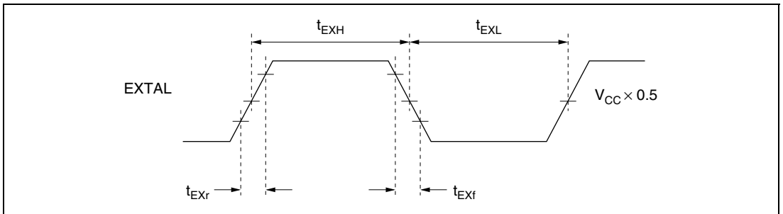
Figure 21.5 External Clock Input Timing
