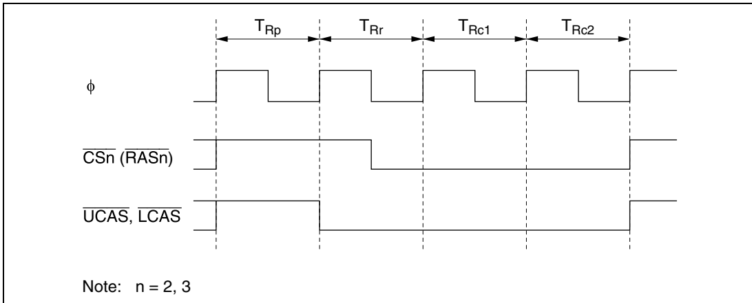
Figure 6.35 CBR Refresh Timing
