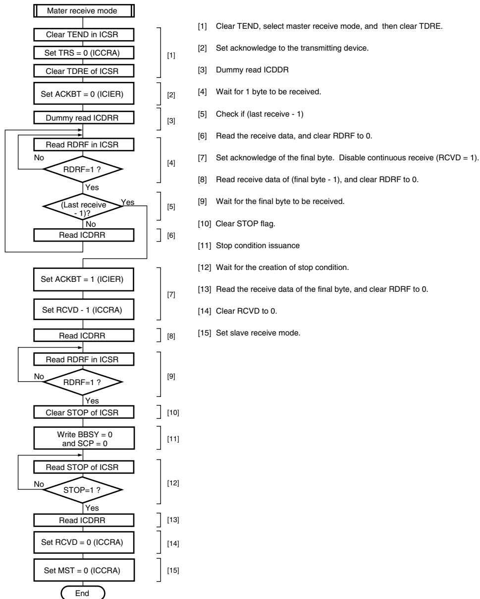
Figure 15.15 Sample Flowchart for Master Receive Mode
