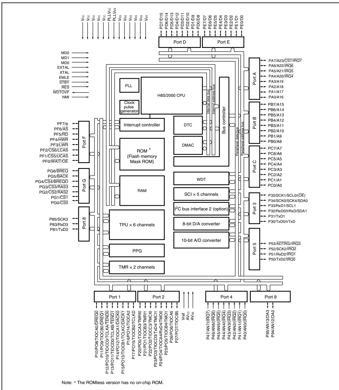
Figure 1.1 Internal Block Diagram of H8S/2367, H8S/2365, and H8S/2363
