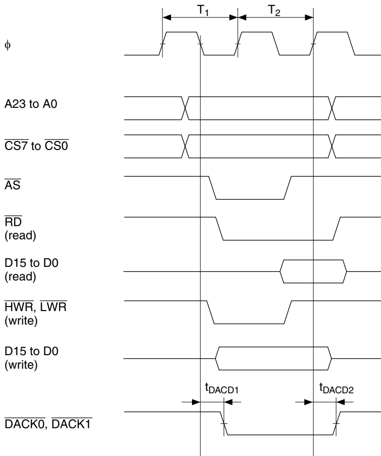
Figure 24.24 DMAC Single Address Transfer Timing: Two-State Access
