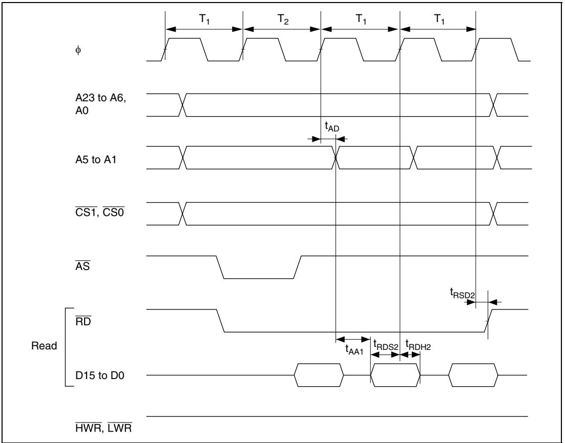
Figure 24.11 Burst ROM Access Timing: One-State Burst Access
