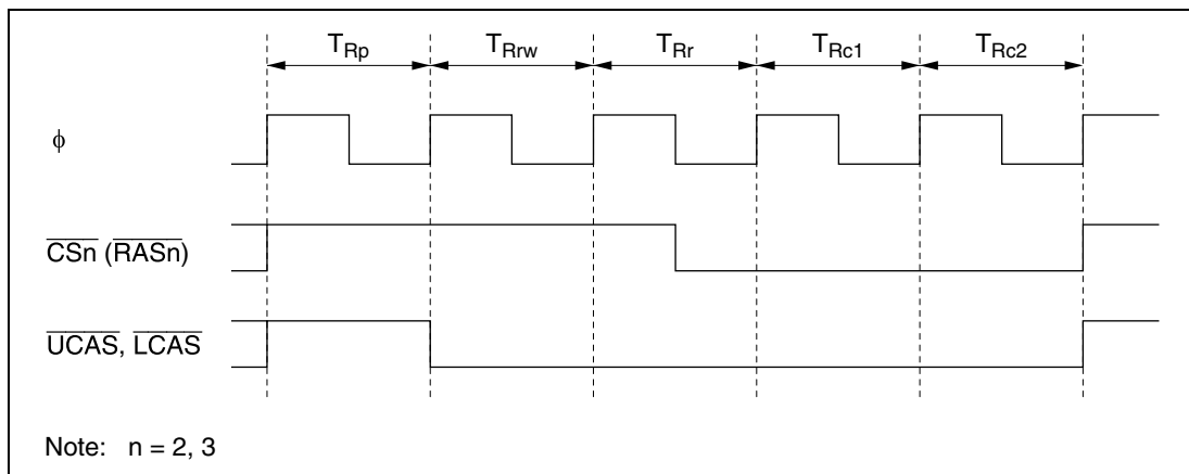
Figure 6.36 CBR Refresh Timing (RCW1 = 0, RCW0 = 1, RLW1 = 0, RLW0 = 0)
