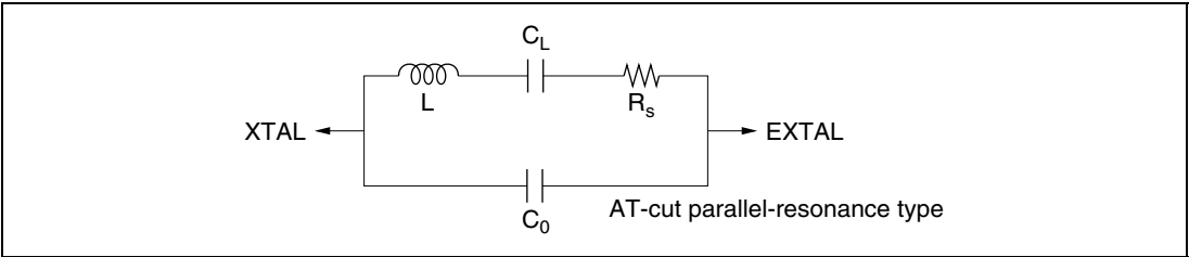
Figure 21.3 Crystal Oscillator Equivalent Circuit
