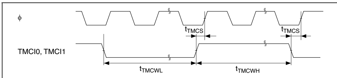
Figure 24.33 8-Bit Timer Clock Input Timing
