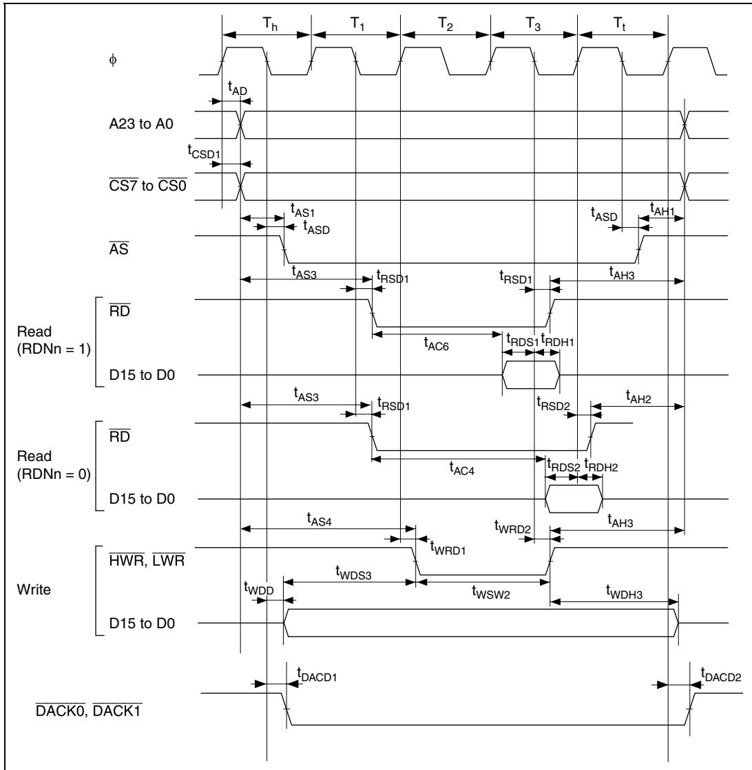
Figure 24.10 Basic Bus Timing: Three-State Access ( \overline{CS} Assertion Period Extended)
