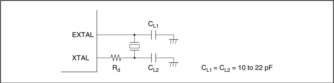
Figure 21.2 Connection of Crystal Oscillator (Example)
