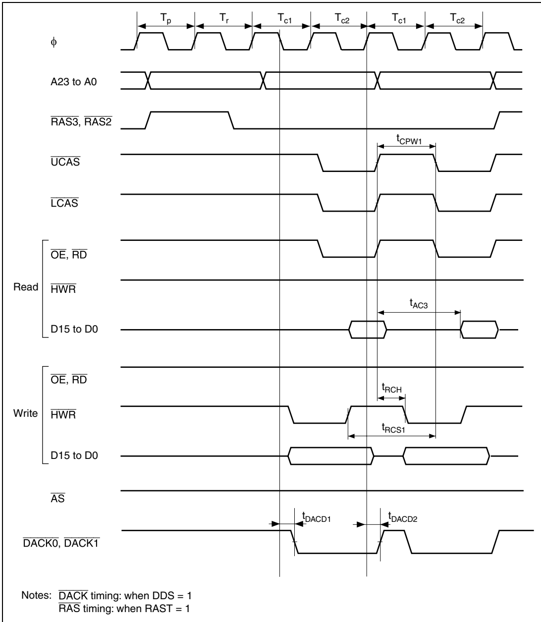
Figure 24.15 DRAM Access Timing: Two-State Burst Access
