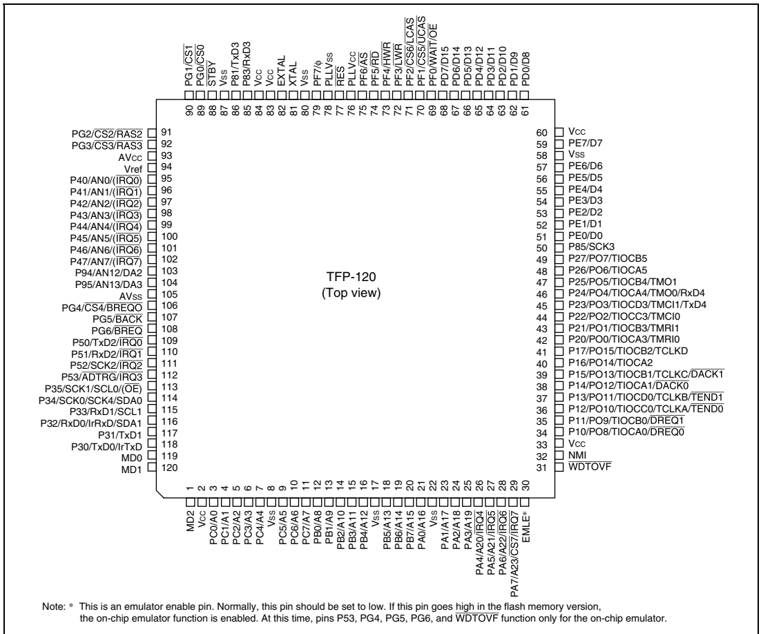
Figure 1.3 Pin Arrangement of H8S/2367, H8S/2365, and H8S/2363
