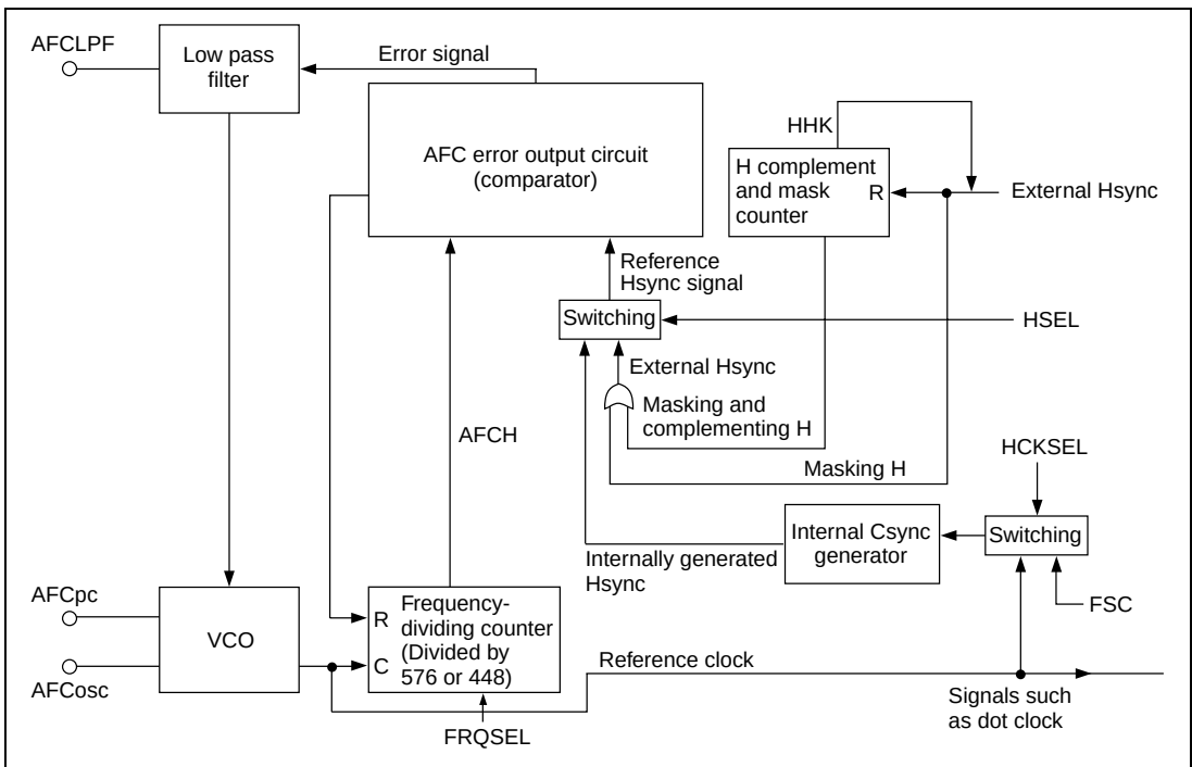
Figure 27.22 AFC Configuration
