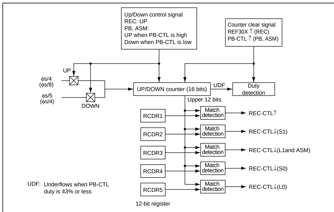
Figure 26.49 CTL Discrimination/Record Circuit
