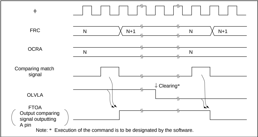
Figure 16.5 Output Comparing Signal Outputting A Timing
