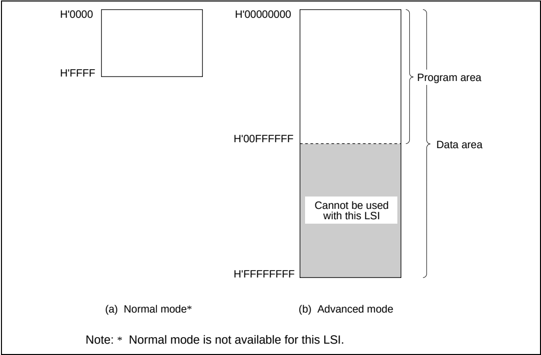
Figure 2.6 Memory Map
