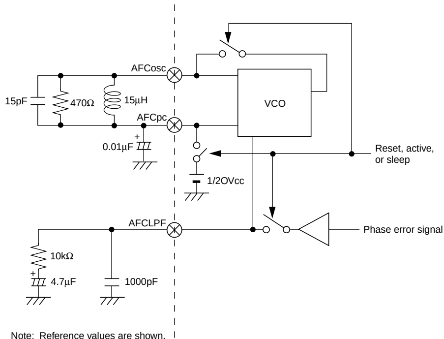
Figure 27.24 Circuit Example for a 448 × fh Reference Clock
