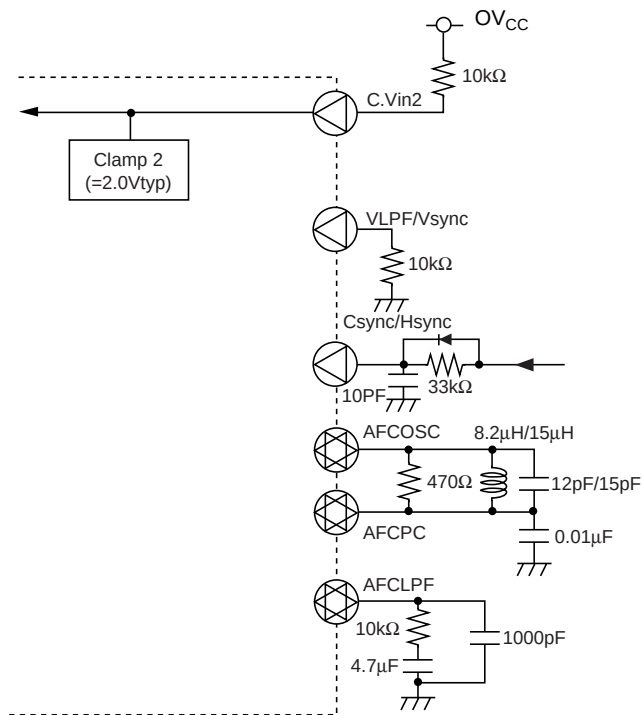
Figure E.9 Example of External Circuit for Sync Separator and Data Slicer ((2) Separation from Csync)
