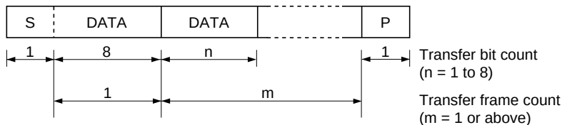
Figure 23.4 I²C Bus Data Format (Serial Format)
