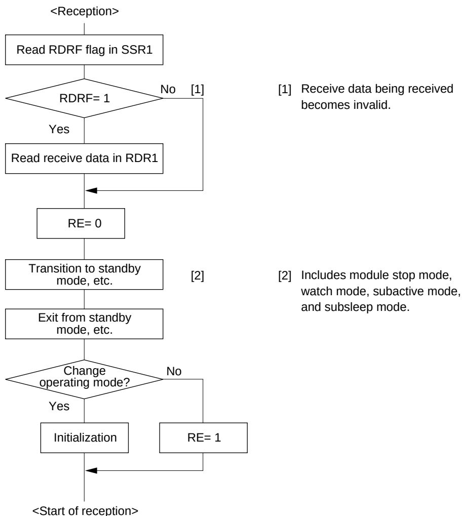
Figure 22.27 Sample Flowchart for Mode Transition during Reception
