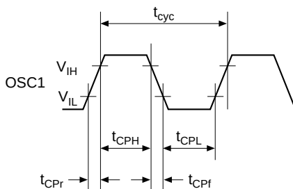
Figure 31.9 System Clock Timing
