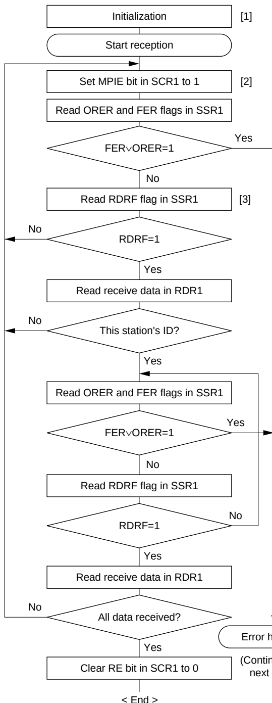
Figure 22.13 Sample Multiprocessor Serial Reception Flowchart (1)
