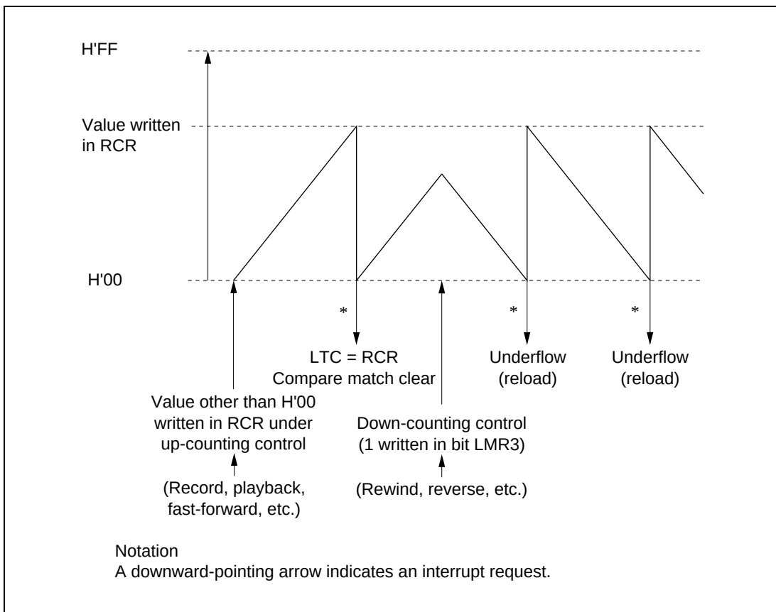
Figure 14-6 Typical Usage of Linear Time Counter
