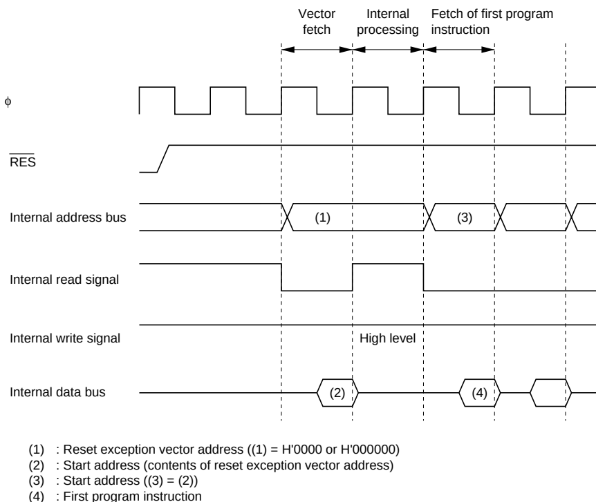
Figure 5.2 Reset Sequence (Mode 1)
