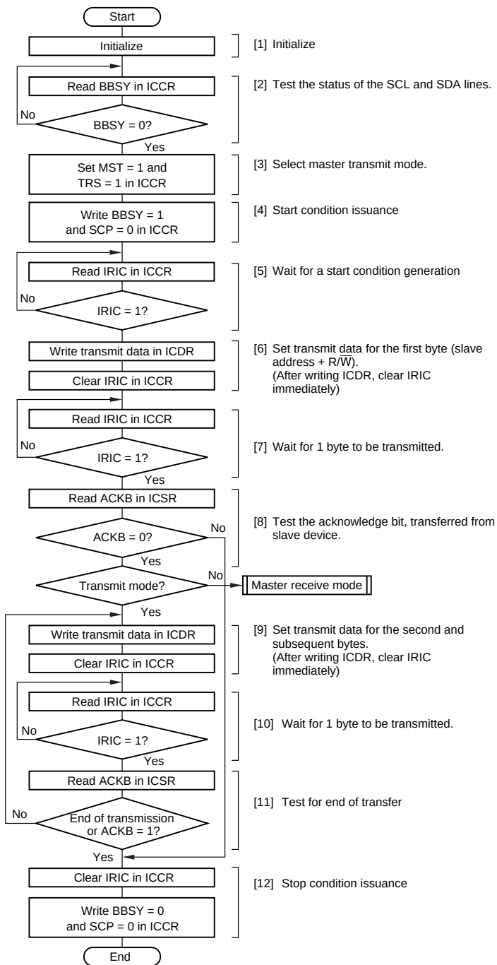
Figure 23.14 Flowchart for Master Transmit Mode (Example)
