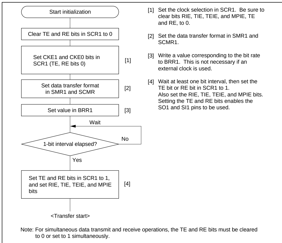
Figure 22.17 Sample SCI Initialization Flowchart
