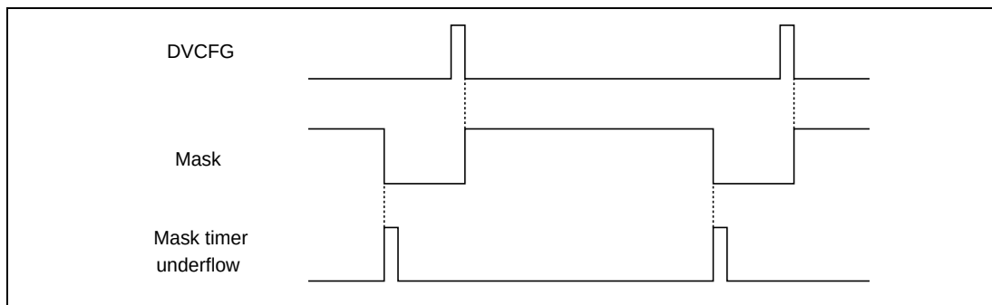
Figure 26.67 Mask Signal
