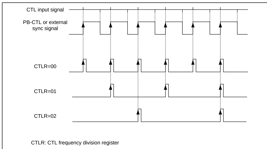
Figure 26.64 CTL Frequency Division Waveforms
