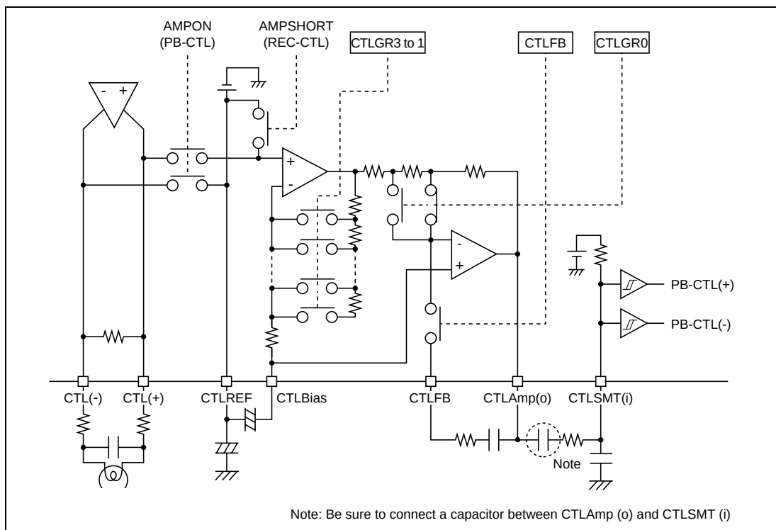
Figure 26.4 CTL Input Circuit
