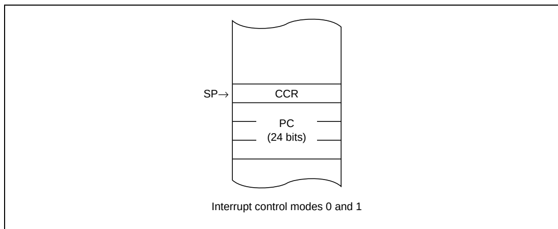
Figure 5.5 Stack Status after Exception Handling (Advanced Mode)
