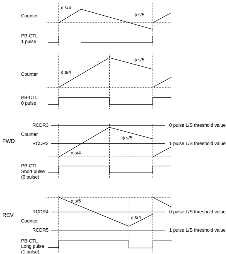
Figure 26.56 Duty Discriminator
