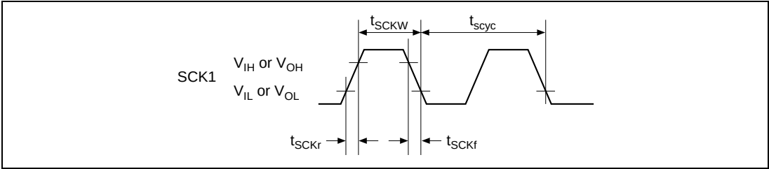
Figure 31.21 SCK1 Clock Timing
