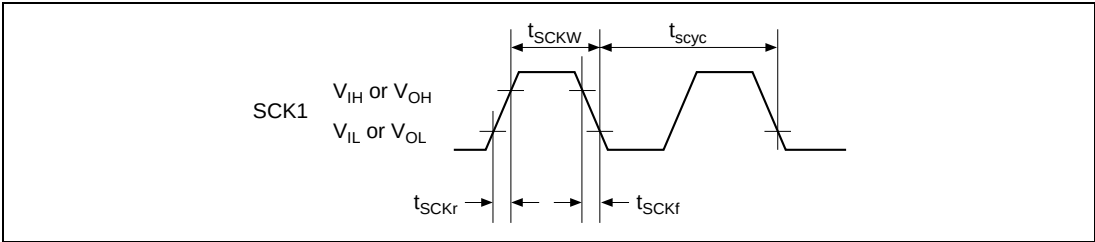
Figure 31.5 SCK1 Clock Timing
