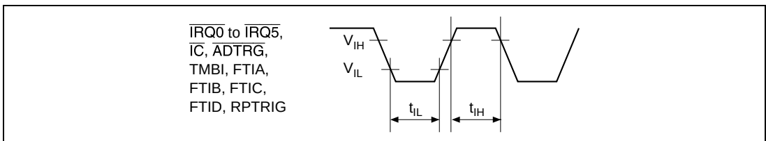
Figure 31.4 Input Timing
