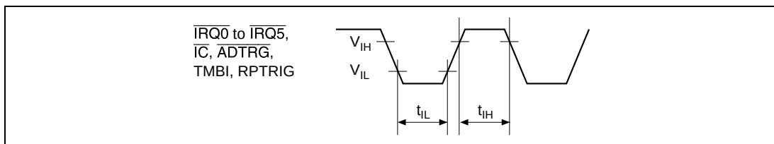
Figure 31.12 Input Timing
