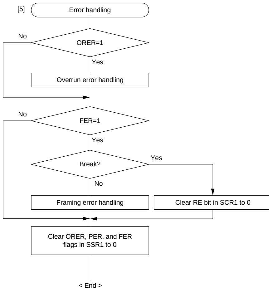
Figure 22.14 Sample Multiprocessor Serial Reception Flowchart (2)
