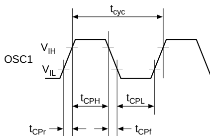
Figure 31.1 System Clock Timing
