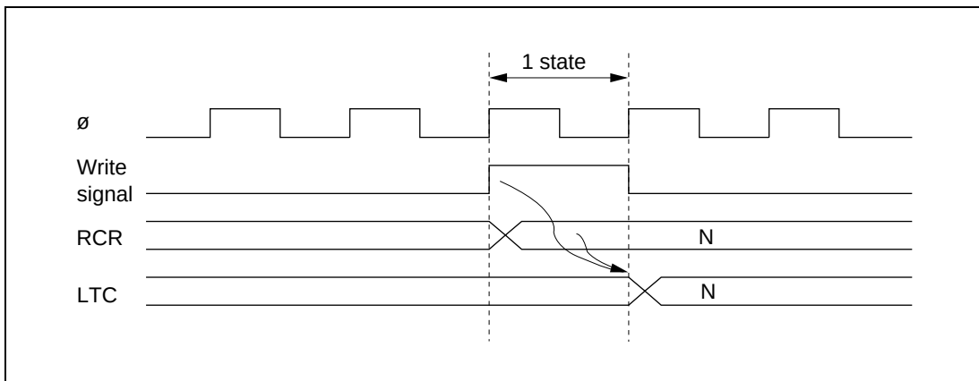
Figure 14-4 Timing of Writing and Reloading of RCR
