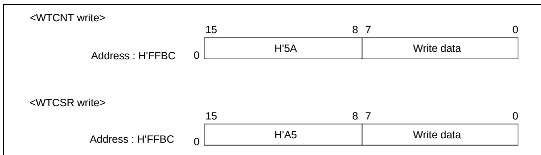
Figure 17.2 Format of Data Written to WTCNT and WTCR
