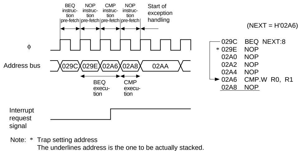
Figure 25.6 When the Condition Satisfied by Bcc Instruction (8-bit Displacement)
