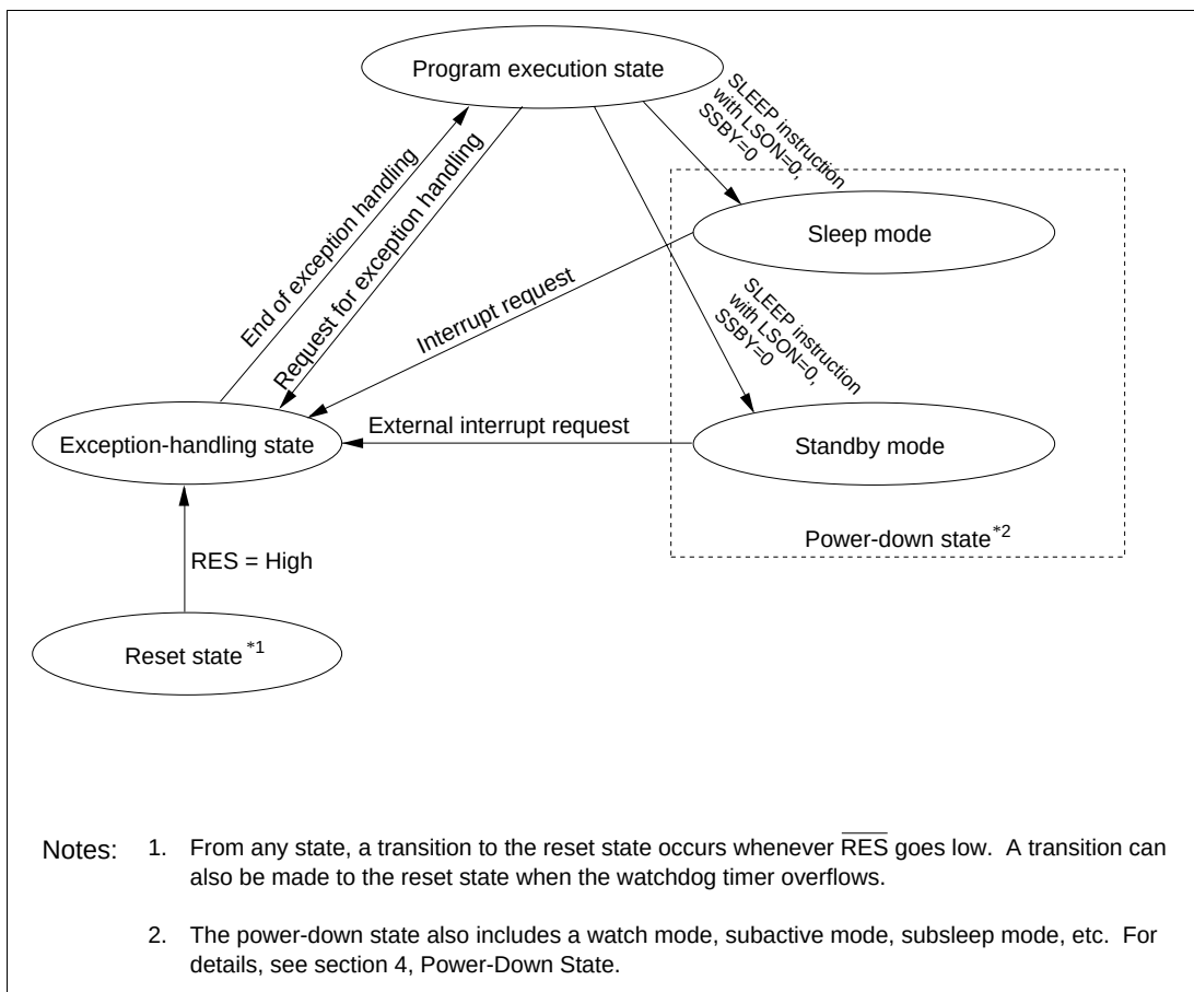
Figure 2.15 State Transitions
