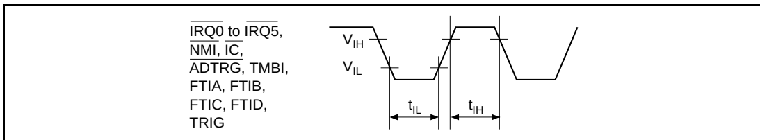
Figure 29.15 Input Timing
