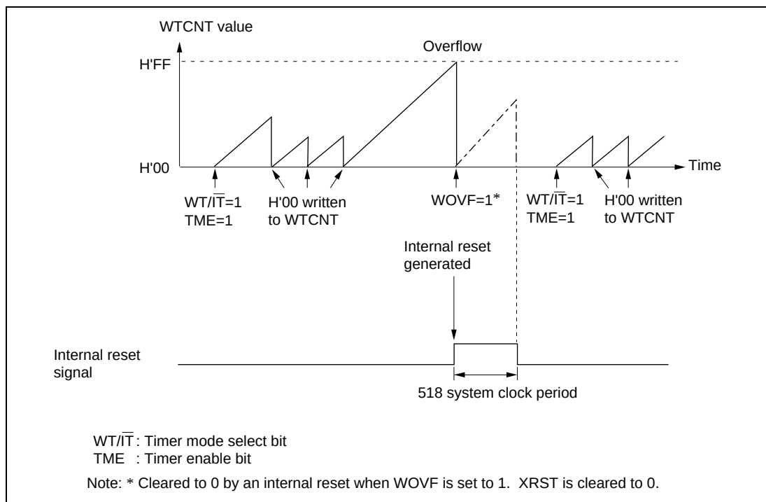
Figure 18.3 Operation in Watchdog Timer Mode
