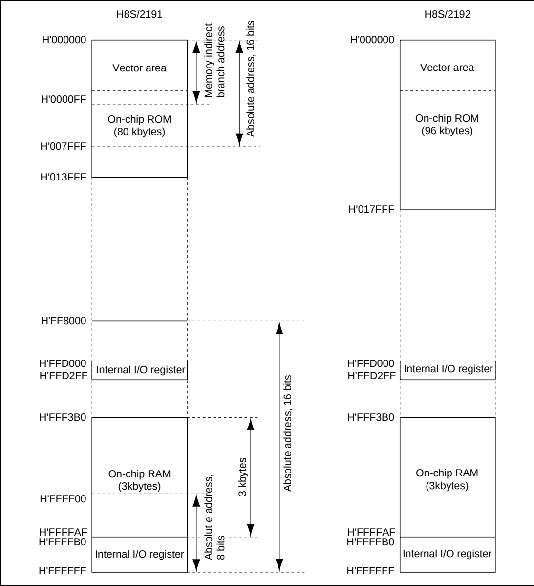
Figure 3.1 Address Map (1)
