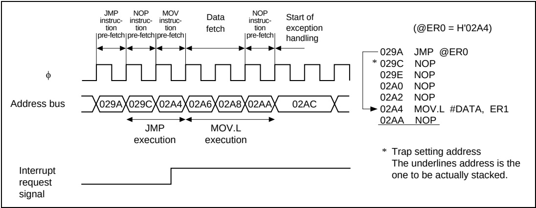
Figure 27.13 JMP Instruction (Register Indirect)
