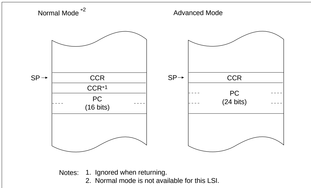
Figure 2.16 Stack Structure after Exception Handling (Examples)
