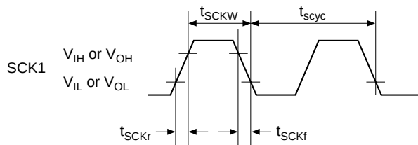
Figure 29.6 SCK1 Clock Timing
