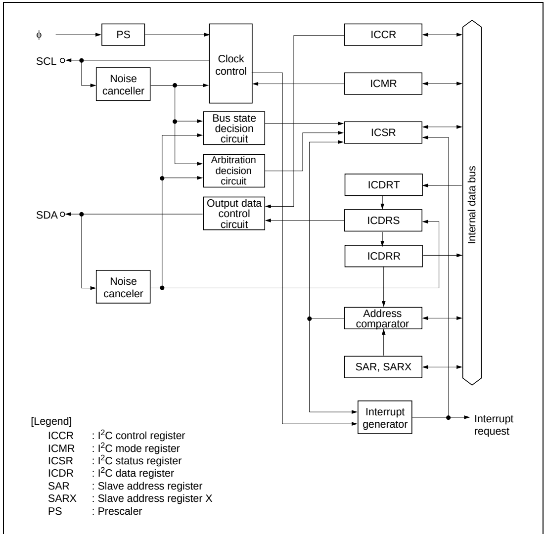
Figure 25.1 Block Diagram of I 2 C Bus Interface
