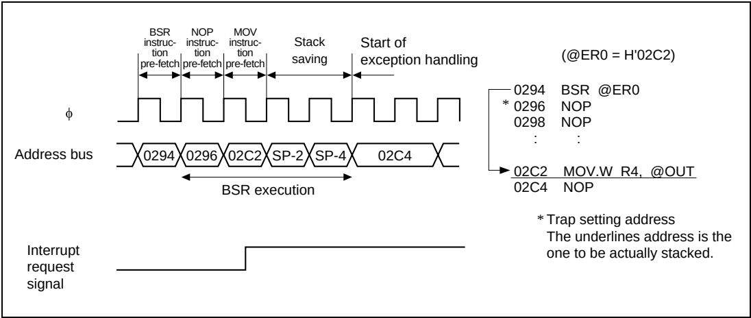
Figure 27.10 BSR Instruction (8-bit Displacement)
