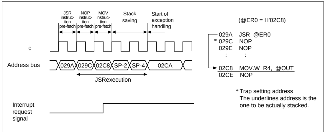
Figure 27.11 JSR Instruction (Register indirect)
