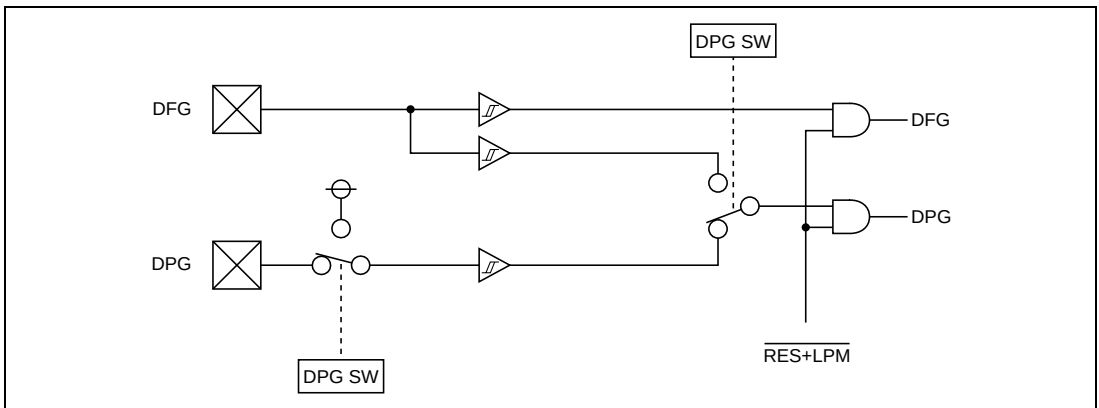
Figure 28.2 Input Circuits of DFG and DPG
