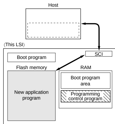
Figure 7.4 Boot Mode
