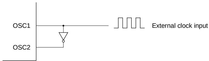
(b) Completely clock input at OSC2 pin
