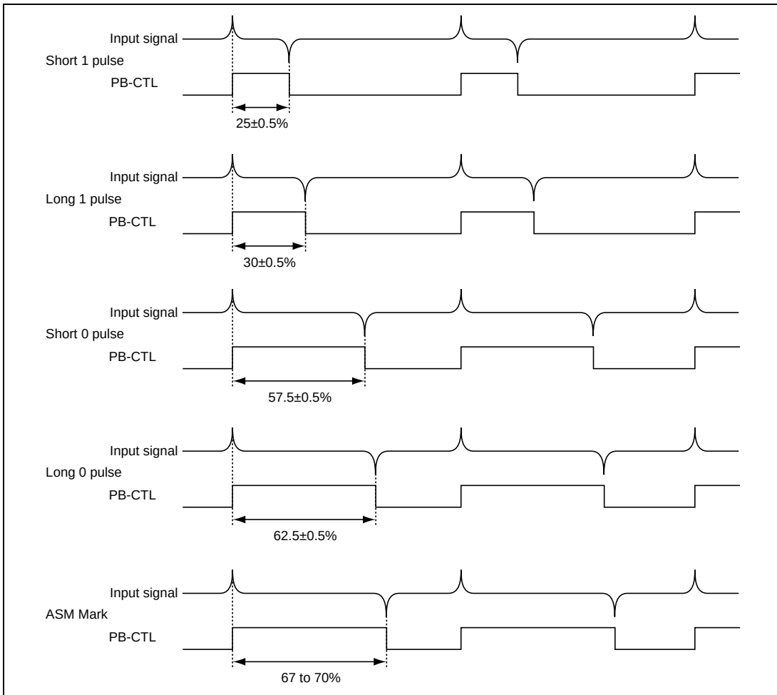
Figure 28.55 PB-CTL Signal Duty Cycle
