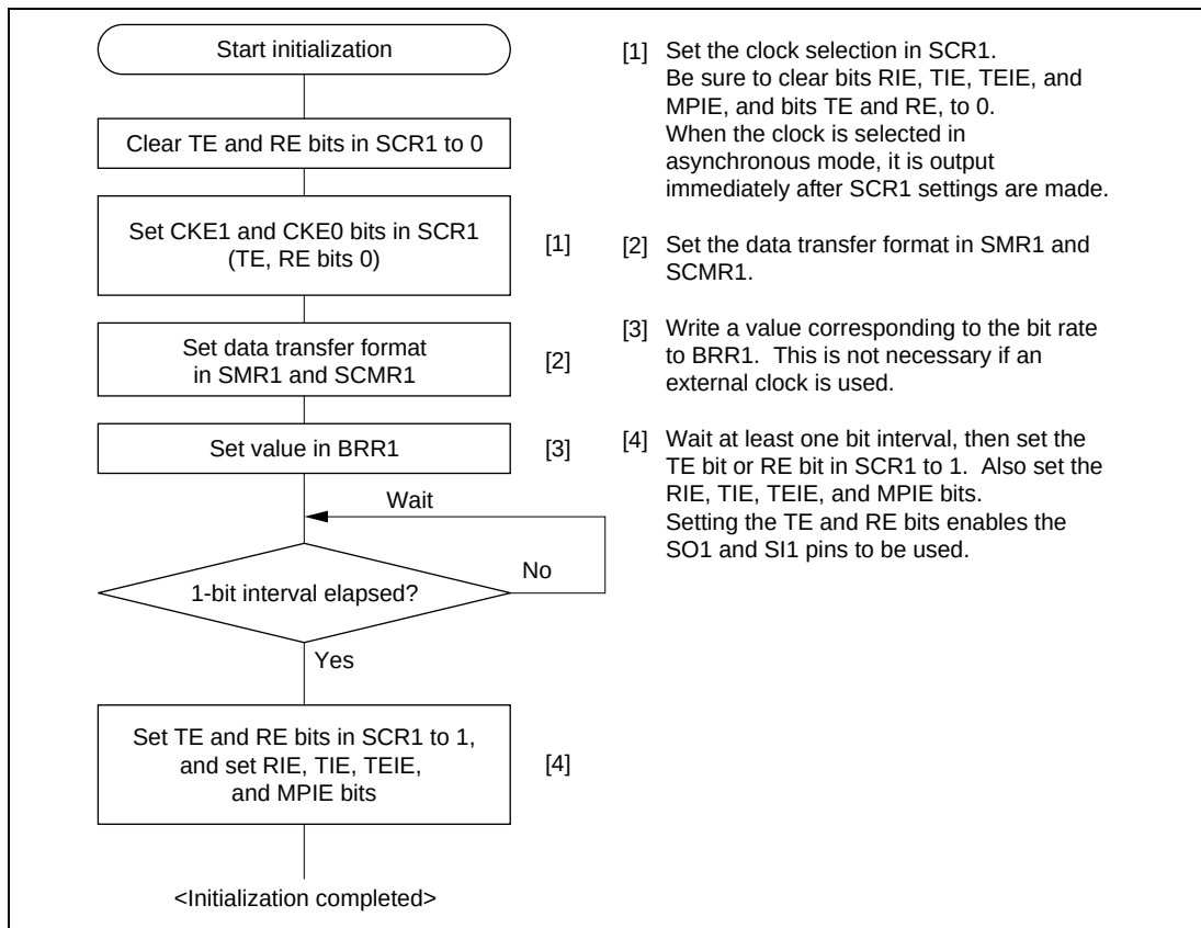
Figure 23.4 Sample SCI1 Initialization Flowchart
