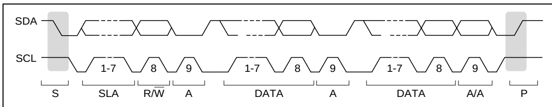
Figure 25.5 I²C Bus Timing
