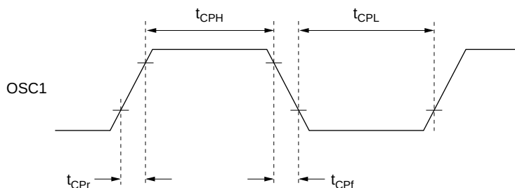
Figure 10.6 External Clock Input Timing
