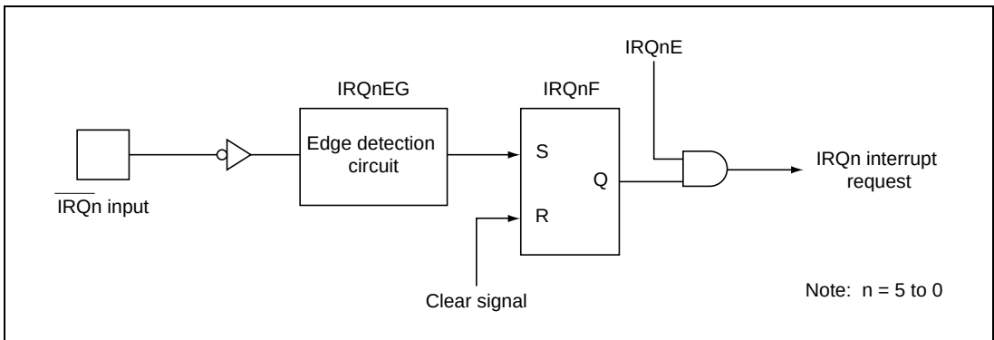
Figure 6.2 Block Diagram of Interrupts IRQ5 to IRQ0
