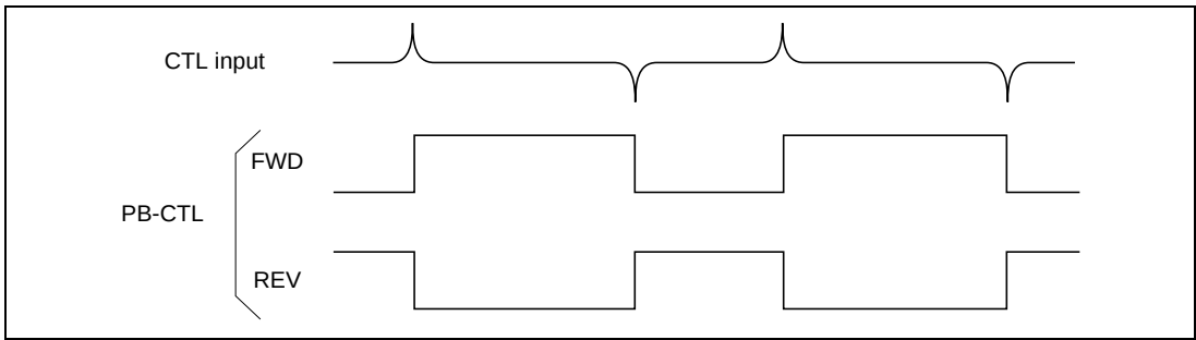
Figure 28.48 Internal PB-CTL Signal in Forward and Reverse
