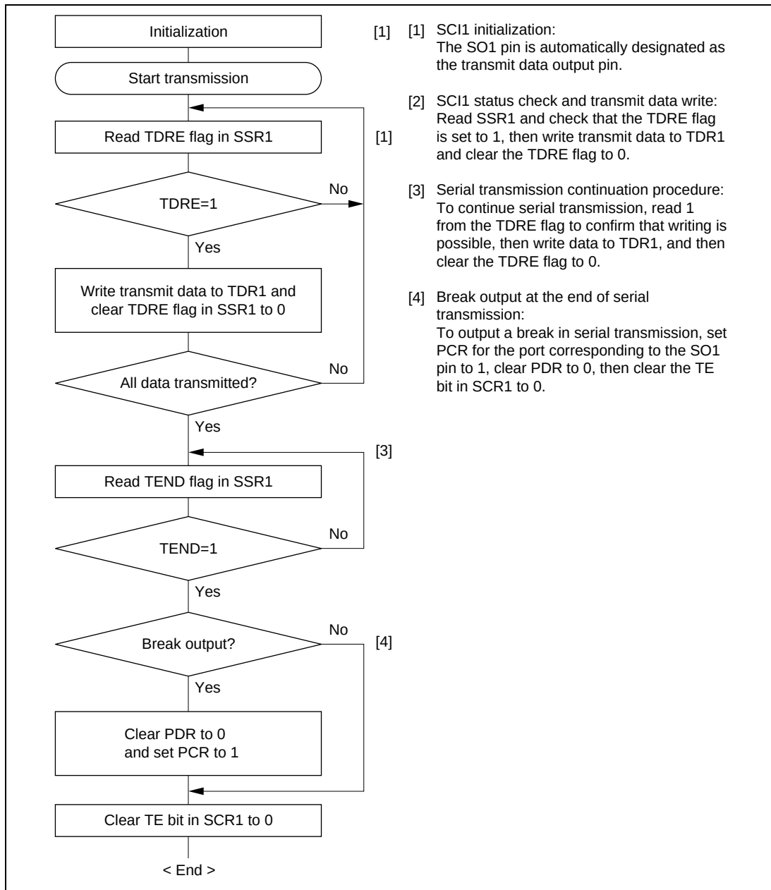
Figure 23.5 Sample Serial Transmission Flowchart
