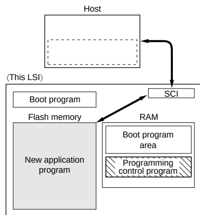
Figure 8.4 Boot Mode
