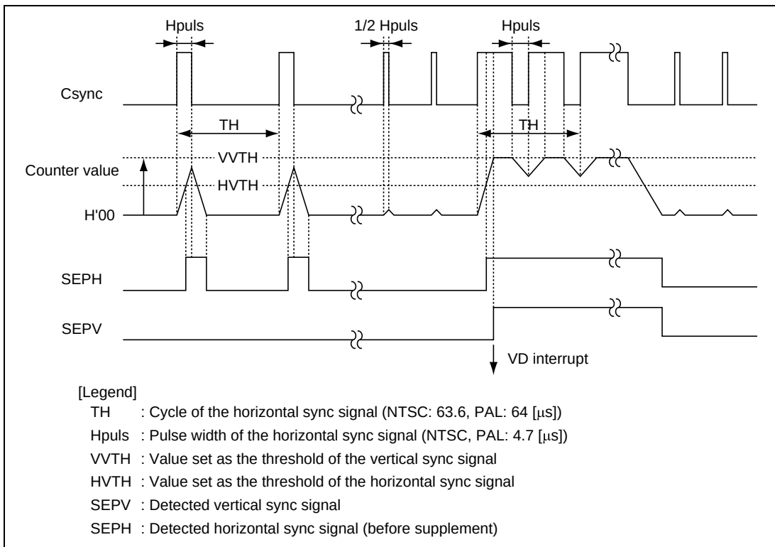
Figure 28.73 Threshold and Separated Sync Signals
