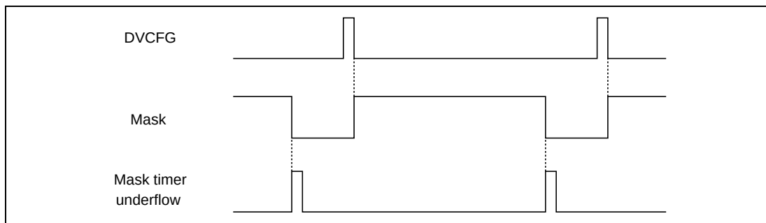
Figure 28.67 Mask Signal
