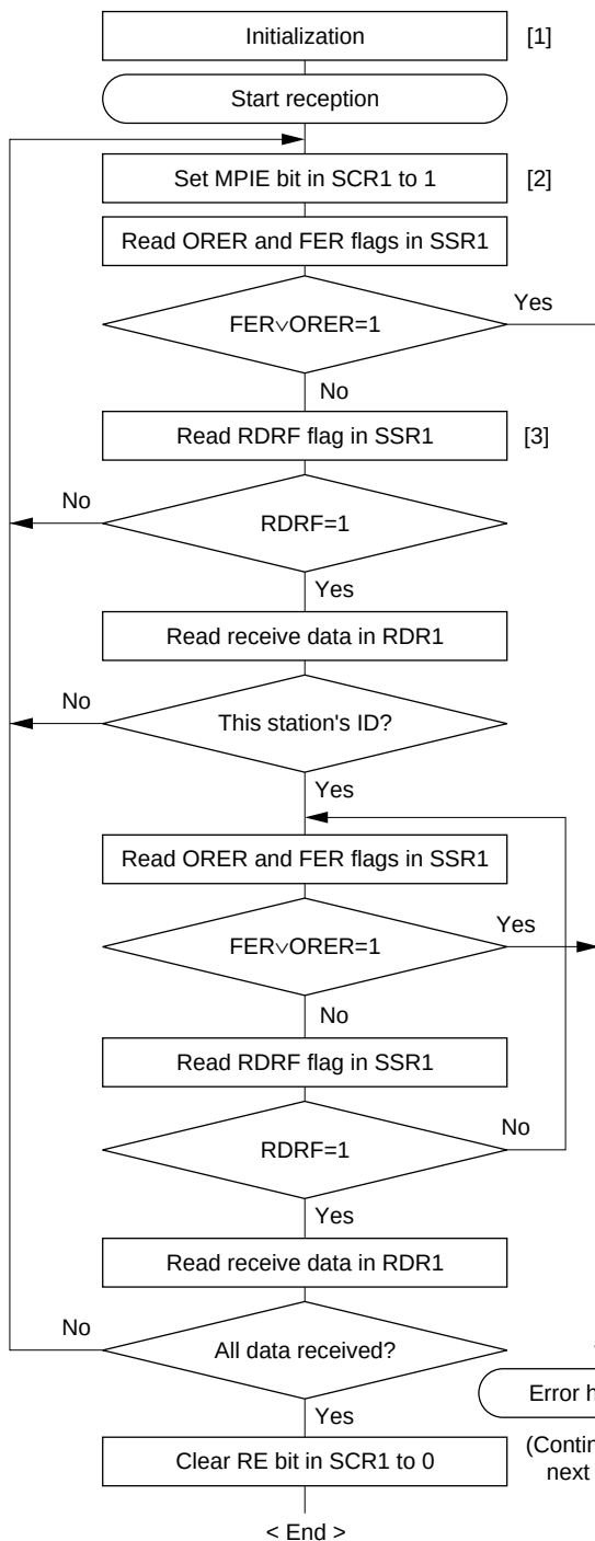
Figure 23.12 Sample Multiprocessor Serial Reception Flowchart (1)
