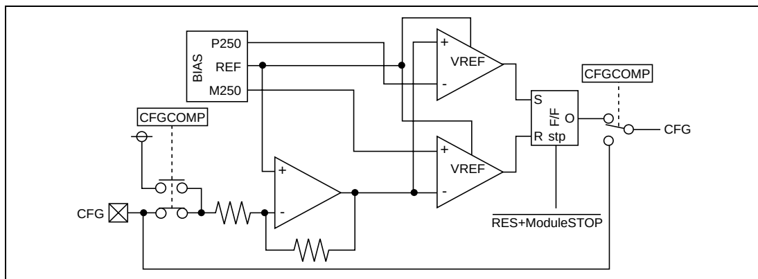
Figure 28.3 CFG Input Circuit
