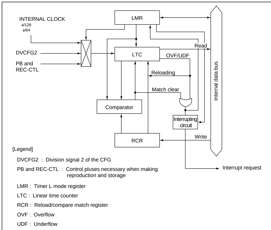
Figure 15.1 Block Diagram of the Timer L
