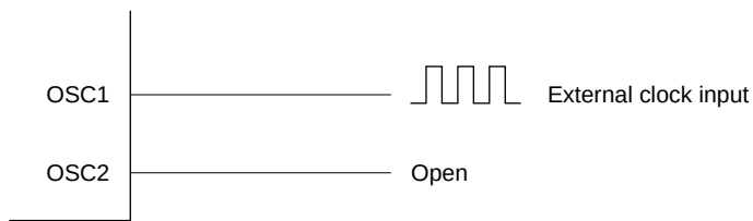
(a) OSC2 pin left open
