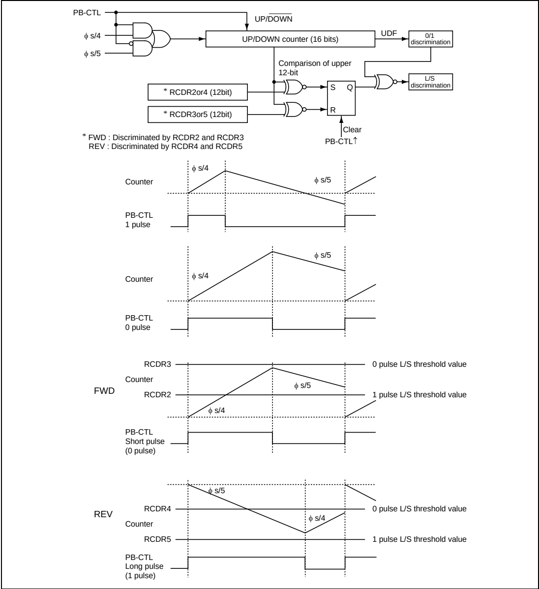
Figure 28.56 Duty Discriminator
