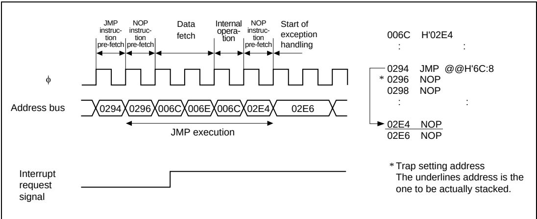
Figure 27.14 JMP Instruction (Memory Indirect)
