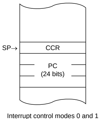
Figure 5.4 (2) Stack Status after Exception Handling (Advanced Mode)
