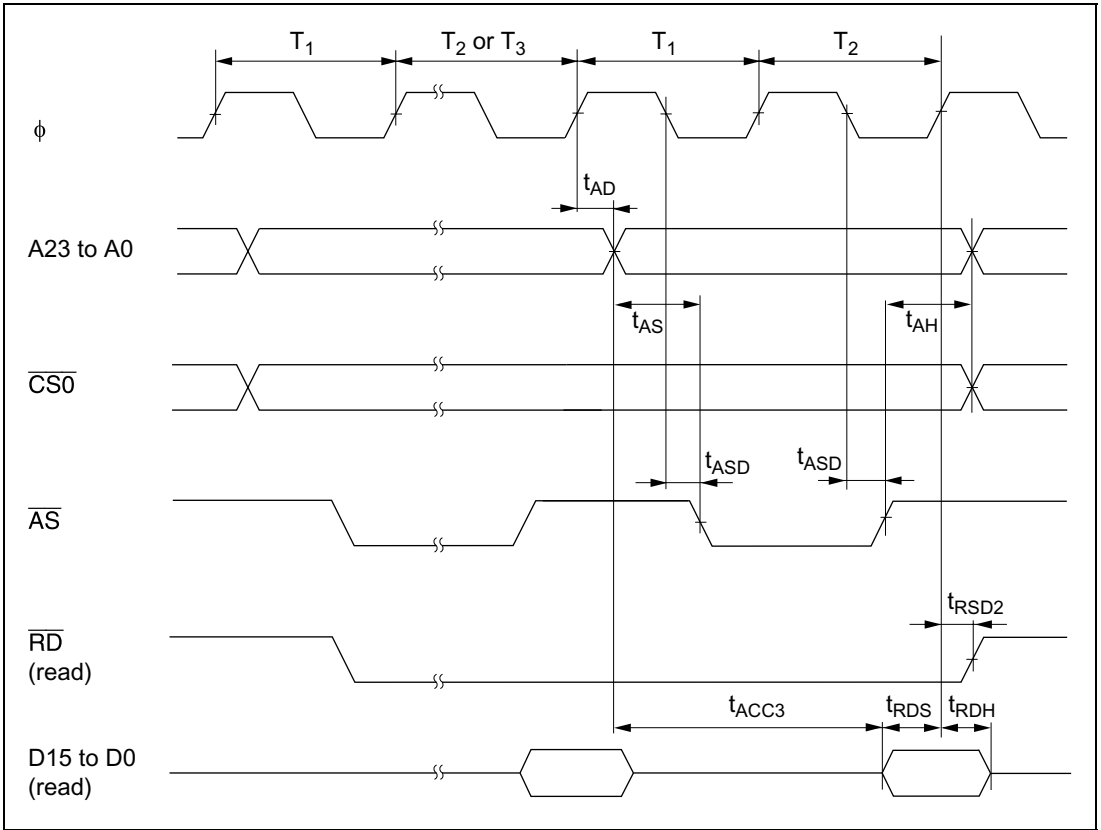
Figure 20-9 Burst ROM Access Timing (2-State Access)
