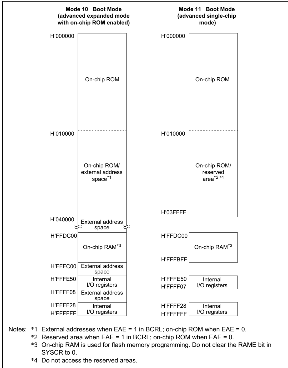
Figure 3-3 (b) H8S/2318 Memory Map in Each Operating Mode (F-ZTAT Version Only)
