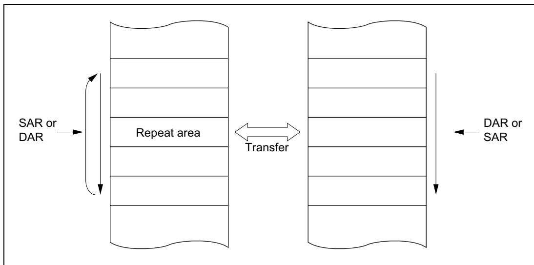
Figure 7-7 Memory Map in Repeat Mode
