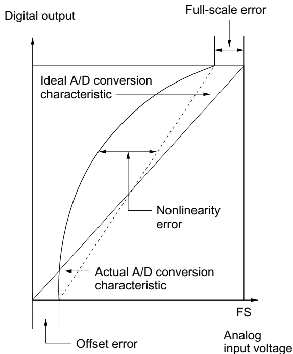
Figure 14-9 A/D Conversion Precision Definitions (2)
