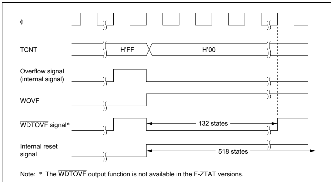
Figure 11-7 Timing of WOVF Setting
