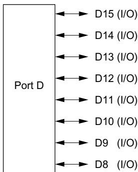
Figure 8-18 Port D Pin Functions (Modes 4 to 6)
