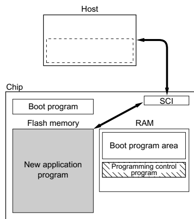
Figure 17-4 Boot Mode
