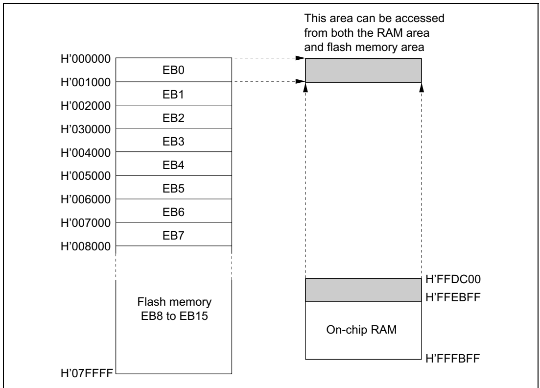
Figure 17-49 Example of RAM Overlap Operation
