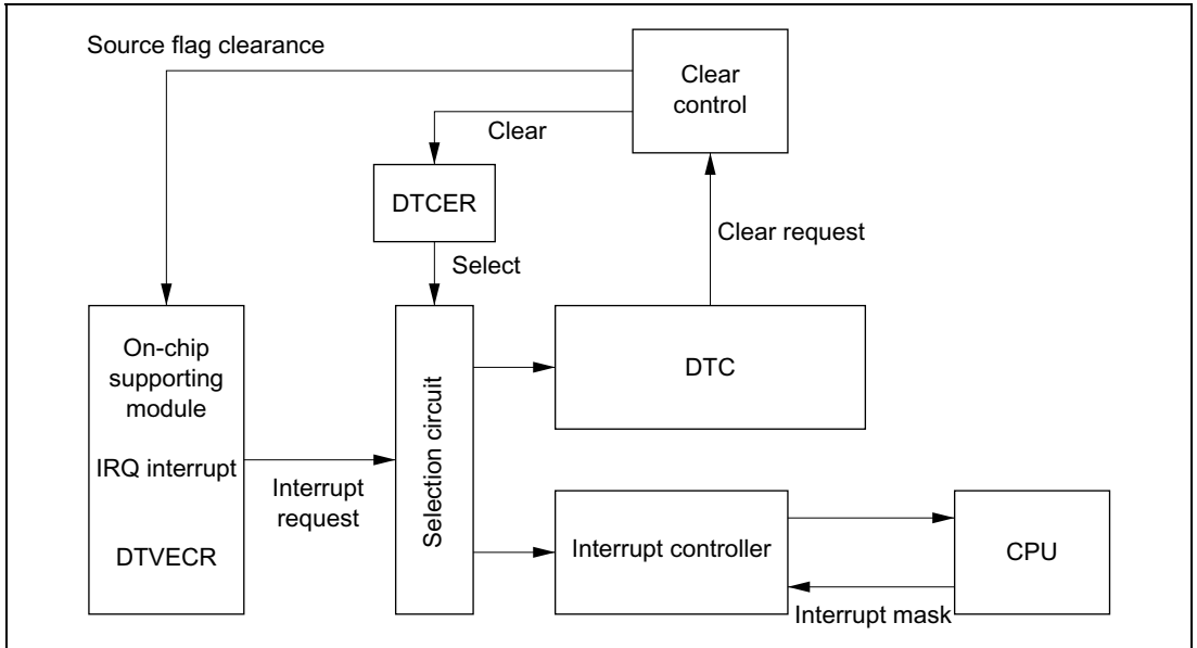
Figure 7-3 Block Diagram of DTC Activation Source Control
