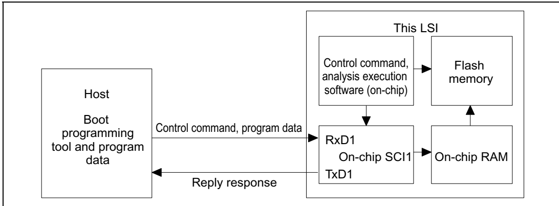
Figure 17-65 System Configuration in Boot Mode
