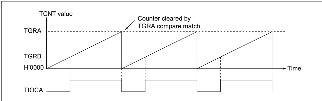
Figure 9-25 Example of PWM Mode Operation (1)
