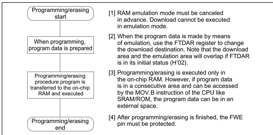
Figure 17-68 Programming/Erasing Overview Flow
