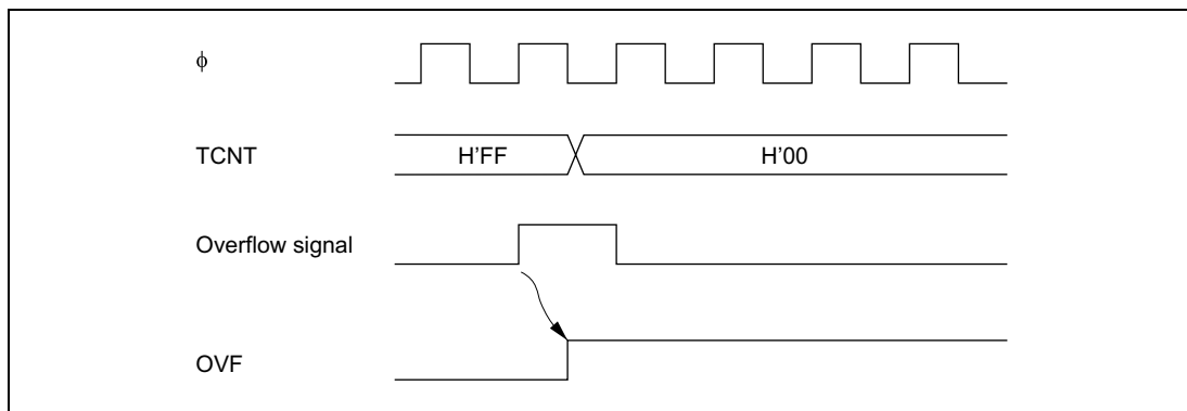
Figure 10-8 Timing of OVF Setting
