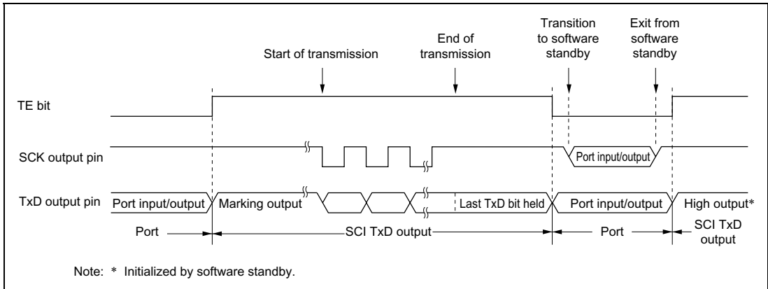
Figure 12-25 Synchronous Transmission Using Internal Clock
