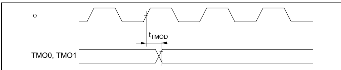
Figure 20-16 8-Bit Timer Output Timing
