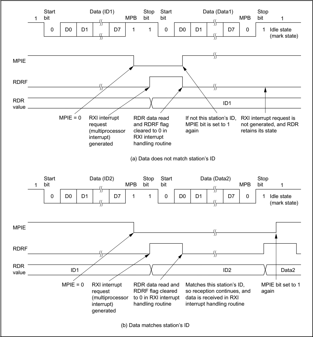
Figure 12-13 Example of SCI Receive Operation (Example with 8-Bit Data, Multiprocessor Bit, One Stop Bit)
