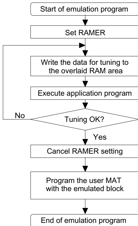
Figure 17-76 Emulation of Flash Memory in RAM
