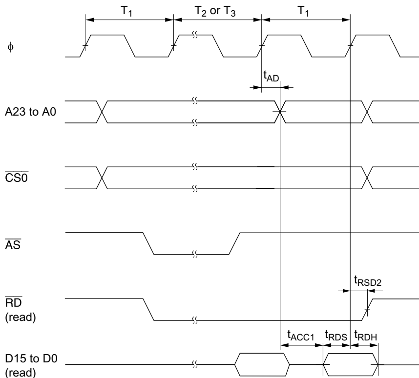
Figure 20-10 Burst ROM Access Timing (1-State Access)
