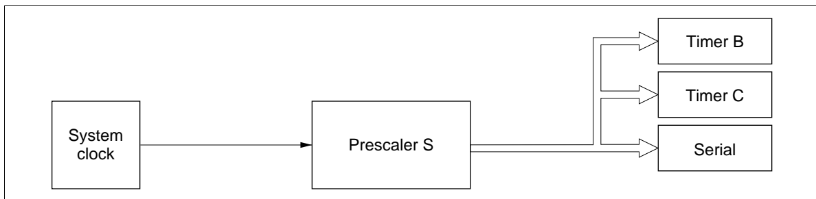
Figure 25 Prescaler Output Supply
