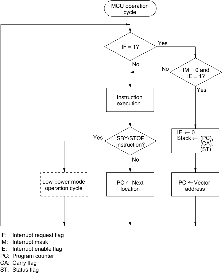
Figure 15 MCU Operation Sequence (MCU Operation Cycle)
