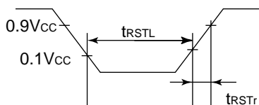
Figure 81 Reset Timing
