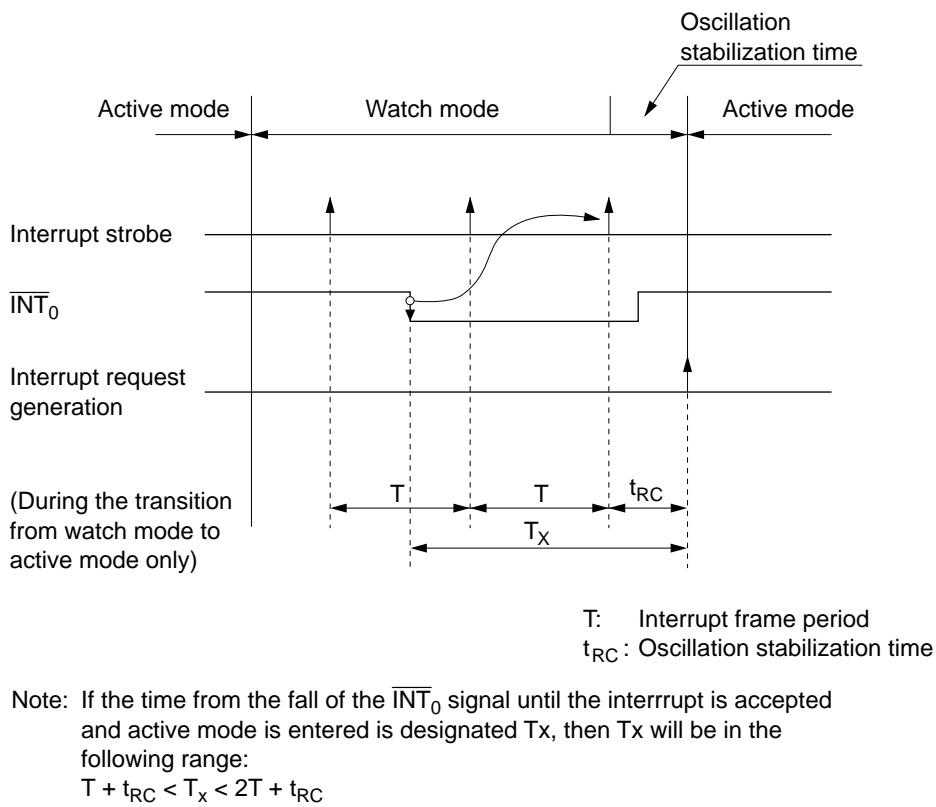
Figure 17 Interrupt Frame
