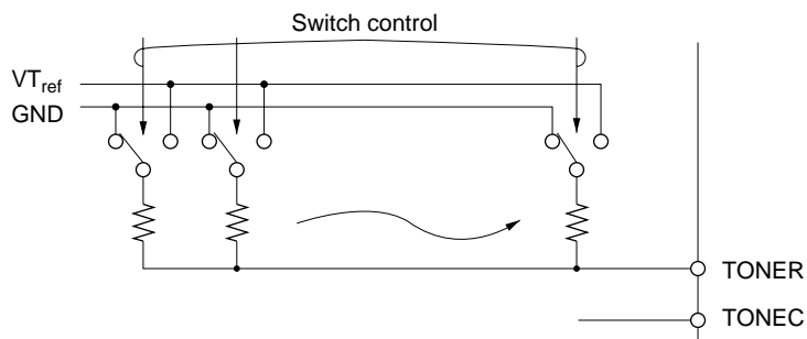
Figure 74 Tone Output Equivalent Circuit
