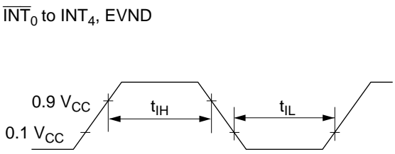
Figure 92 Interrupt Timing
