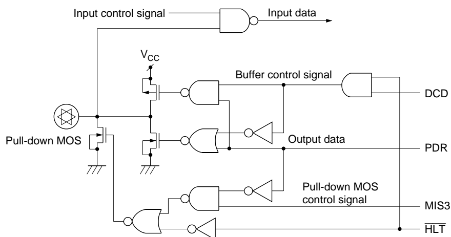
Figure 28 I/O Buffer Configuration (with Pull-Down MOS)
