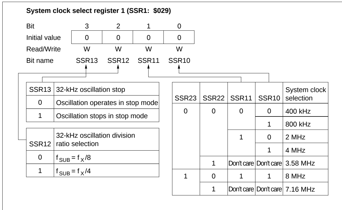
Figure 85 System Clock Select Register 1(SSR1)
