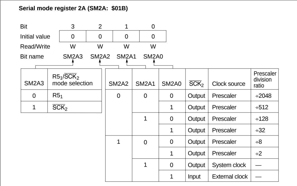
Figure 35 Serial Mode Register 2A (SM2A)
