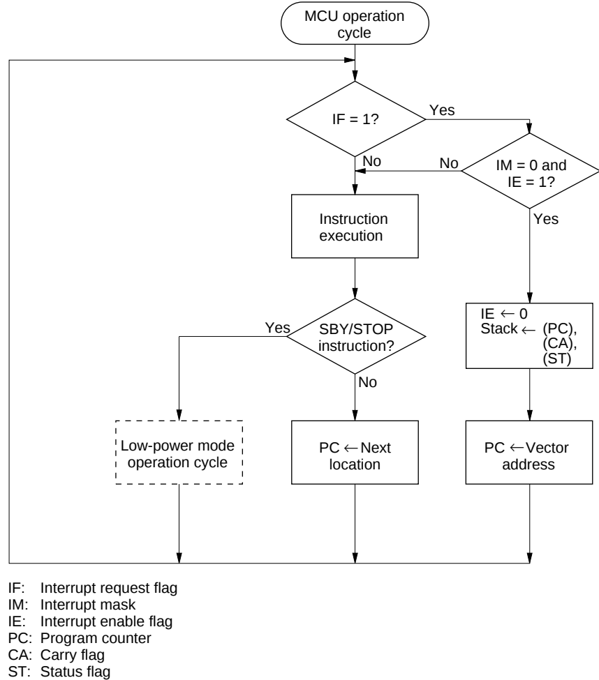
Figure 21 MCU Operating Sequence (MCU Operation Cycle)
