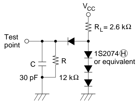
Figure 54 Timing Load Circuit
