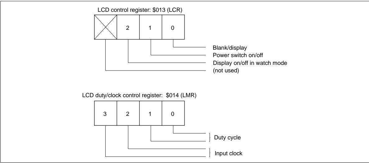
Figure 37 LCD Control and LCD Mode Registers
