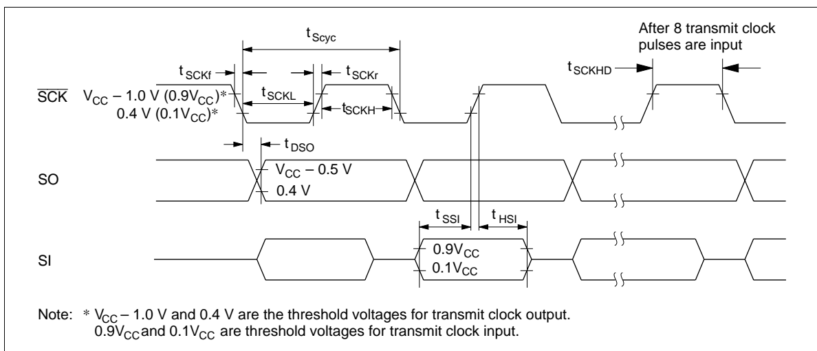
Figure 53 Serial Interface Timing
