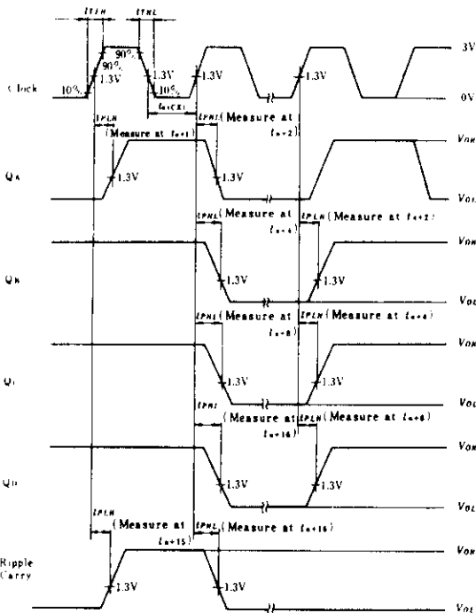
Waveform—1 f_{max} , t_{PLH} , t_{PHL} (Clock→Q, Ripple Carry)
