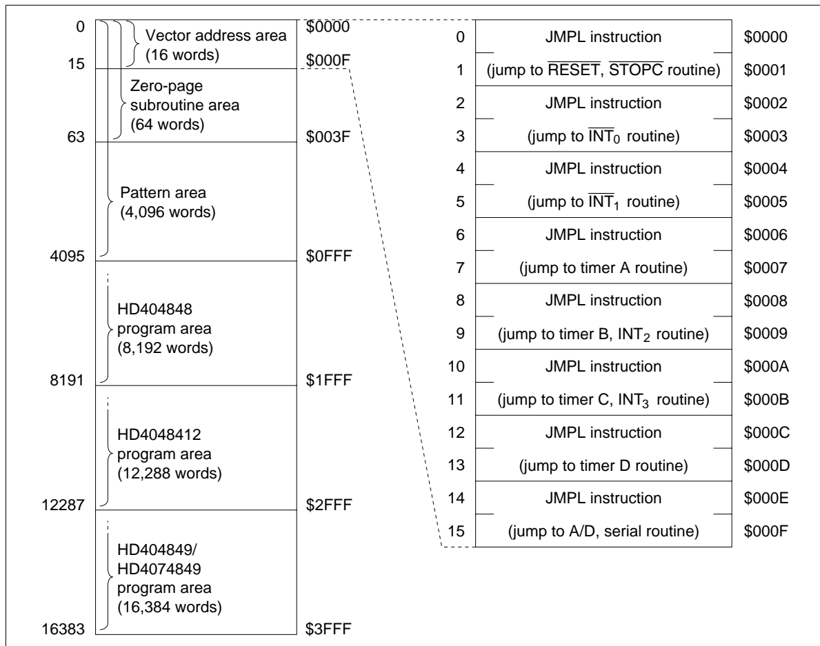
Figure 1 ROM Memory Map
