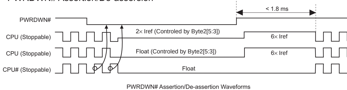
PWRDWN# Functionality
