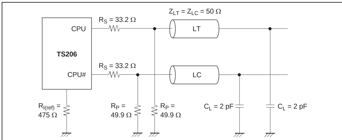
Fig.3 Load Circuit for CPU/CPU#
