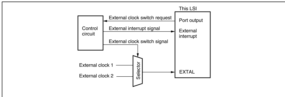
Figure 21.6 External Clock Switching Circuit (Examples)
