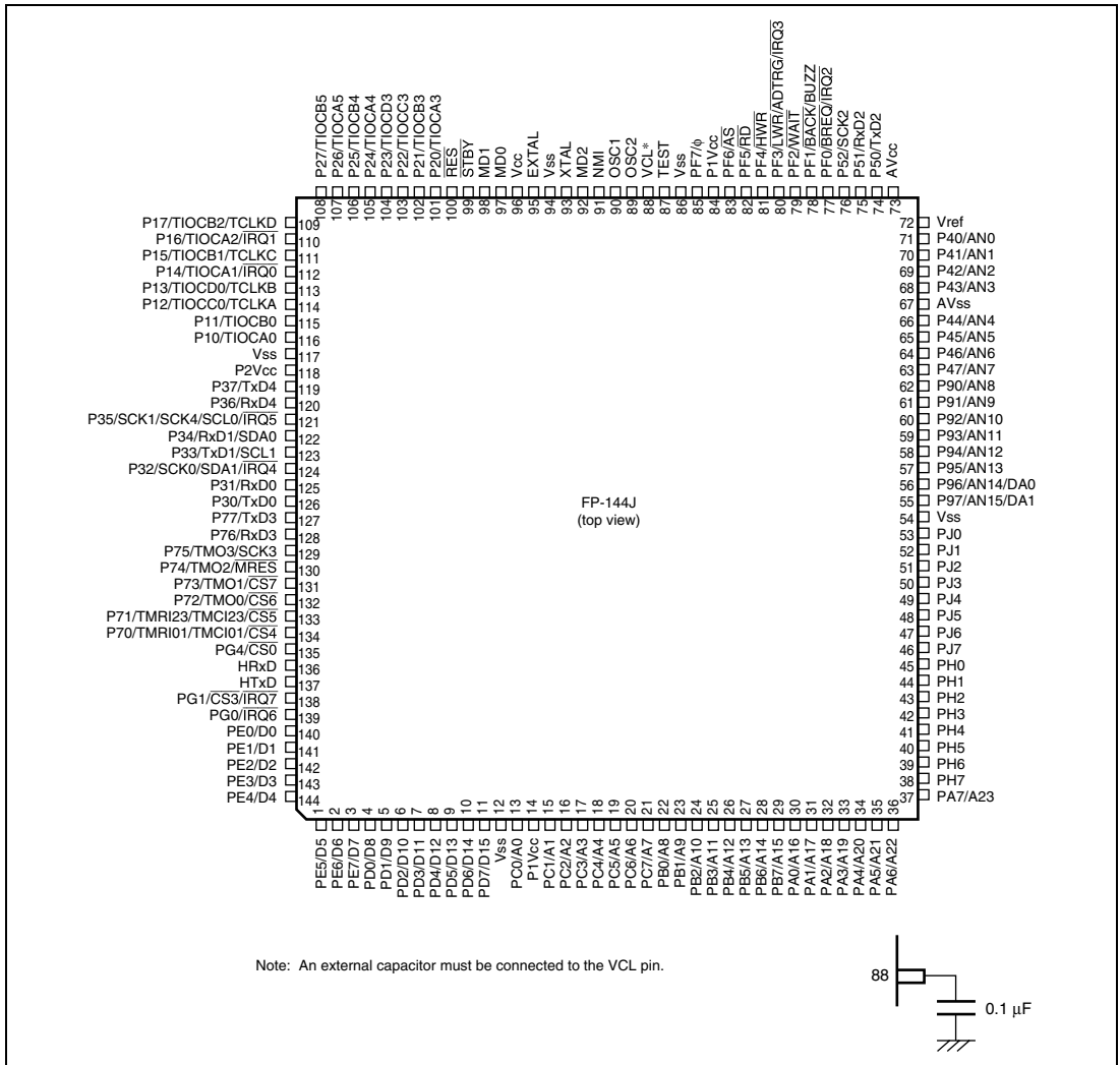
Figure 1.4 Pin Arrangement of H8S/2556 Series (FP-144J)
