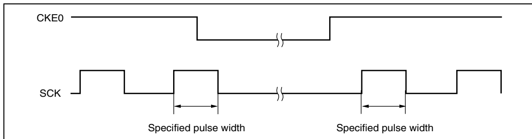
Figure 13.31 Timing for Fixing Clock Output Level
