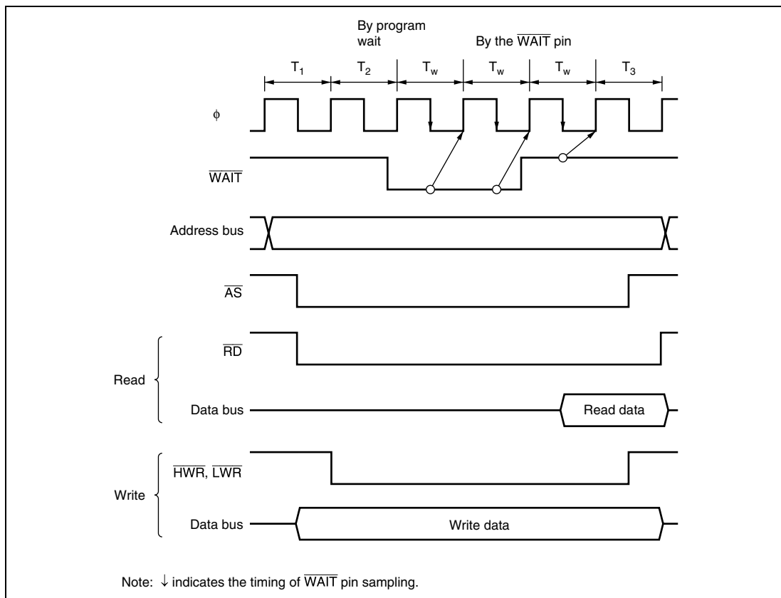
Figure 7.24 Example of Wait State Insertion Timing
