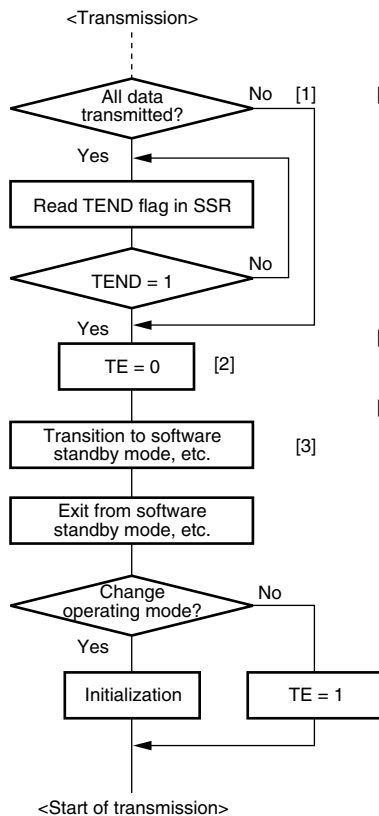
Figure 13.34 Sample Flowchart for Mode Transition during Transmission
