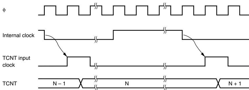
Figure 11.3 Count Timing for Internal Clock Input
