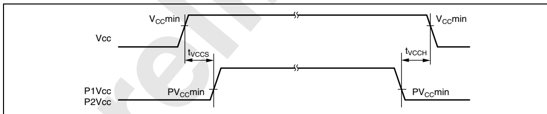
Figure 24.3 Power-On/Off Timing
