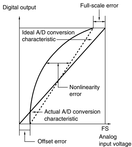
Figure 15.5 A/D Conversion Accuracy Definitions
