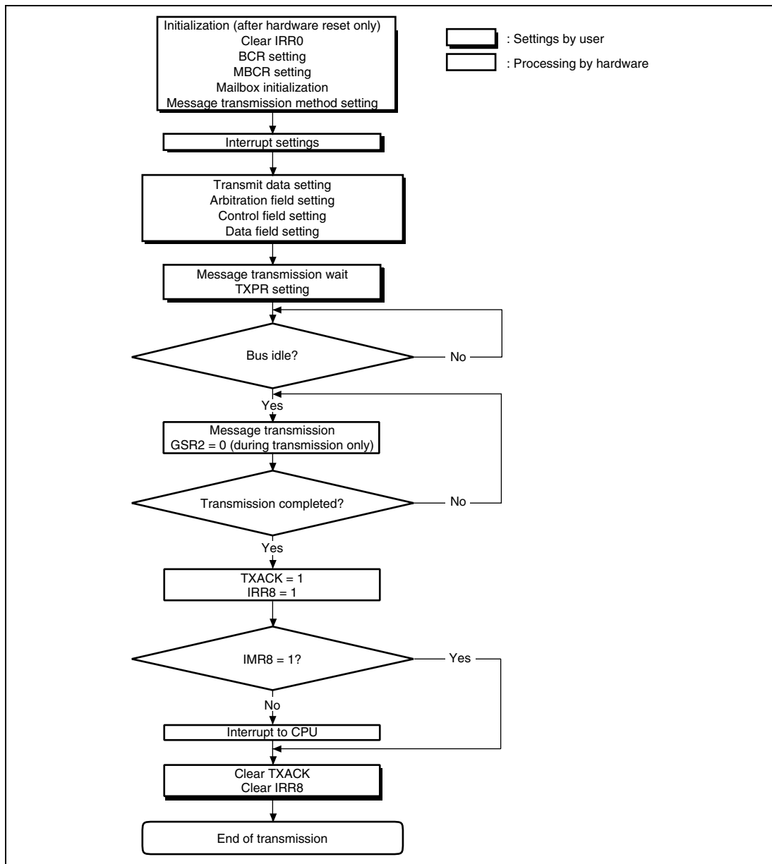
Figure 18.9 Transmission Flowchart
