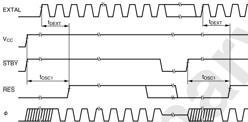
Figure 24.5 Oscillator Settling Timing
