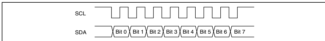
Figure 14.13 Clocked Synchronous Serial Transfer Format
