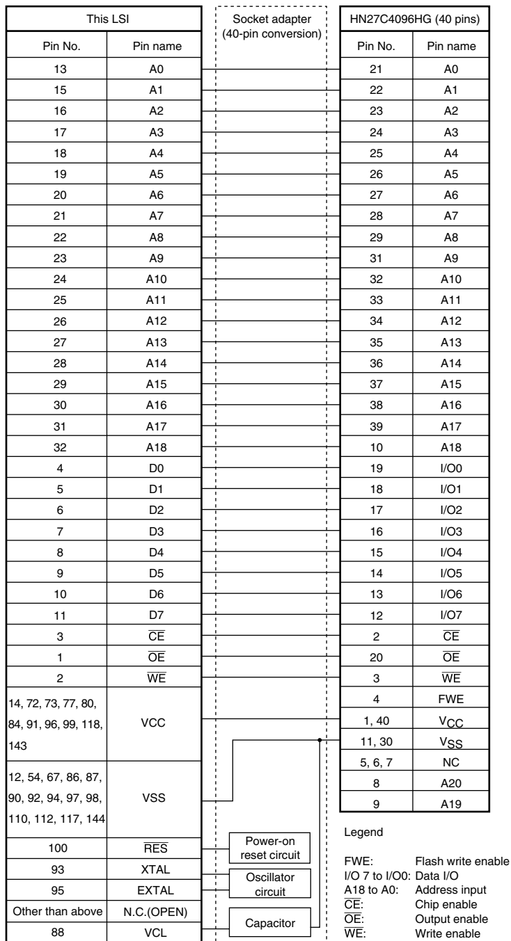
Figure 20.22 Pin arrangement of Socket Adapter
