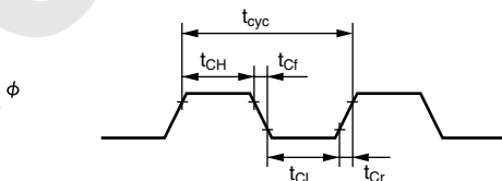
Figure 24.4 System Clock Timing
