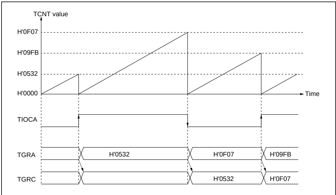
Figure 9.16 Example of Buffer Operation (2)
