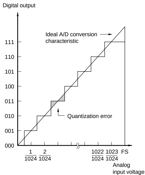
Figure 14.4 A/D Conversion Accuracy Definitions
