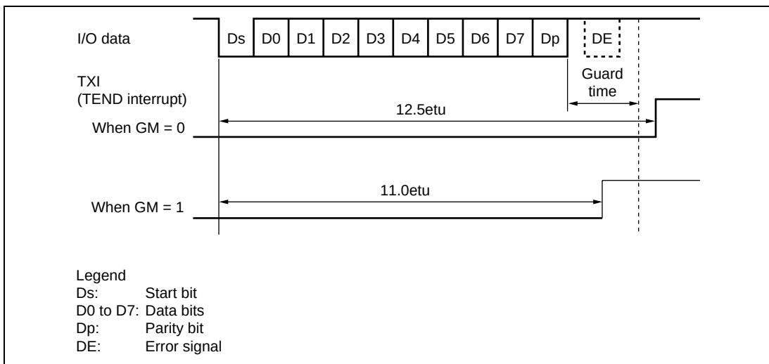
Figure 13.27 TEND Flag Generation Timing in Transmission Operation
