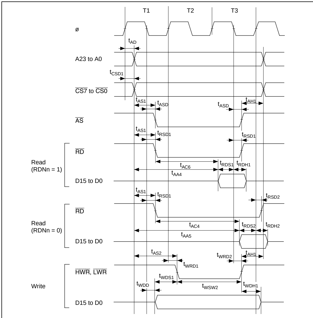
Figure 21.7 Basic Bus Timing: Three-State Access
