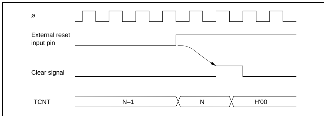
Figure 11.8 Timing of Clearance by External Reset
