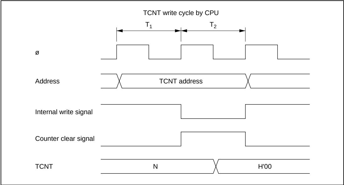
Figure 11.10 Contention between TCNT Write and Clear
