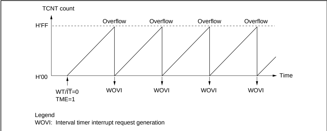
Figure 12.3 Operation in Interval Timer Mode
