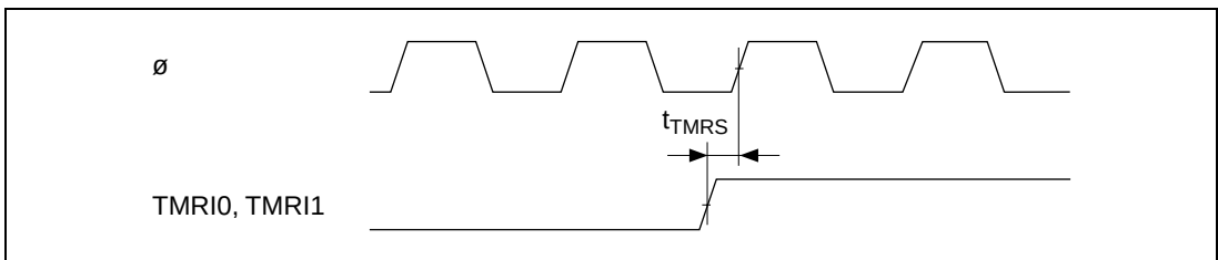
Figure 21.19 8-Bit Timer Reset Input Timing
