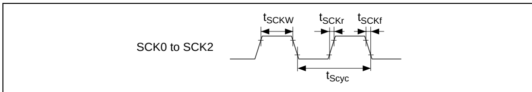
Figure 21.21 SCK Clock Input Timing
