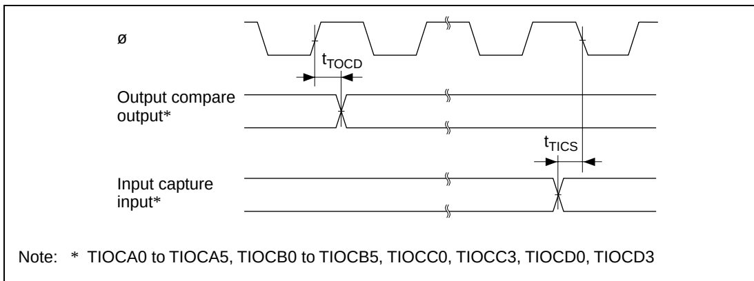
Figure 21.15 TPU Input/Output Timing
