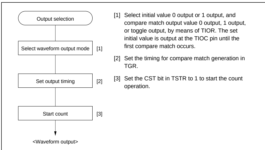
Figure 9.5 Example of Setting Procedure for Waveform Output by Compare Match
