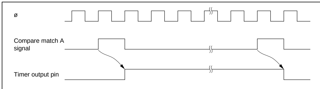
Figure 11.6 Timing of Timer Output
