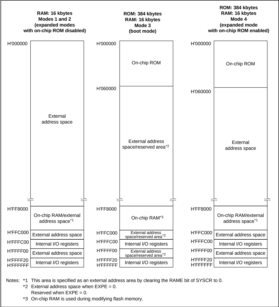
Figure 3.1 Memory Map (1)
