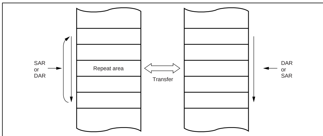
Figure 7.6 Memory Mapping in Repeat Mode
