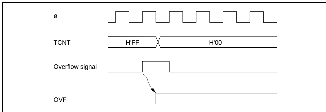
Figure 11.9 Timing of OVF Setting
