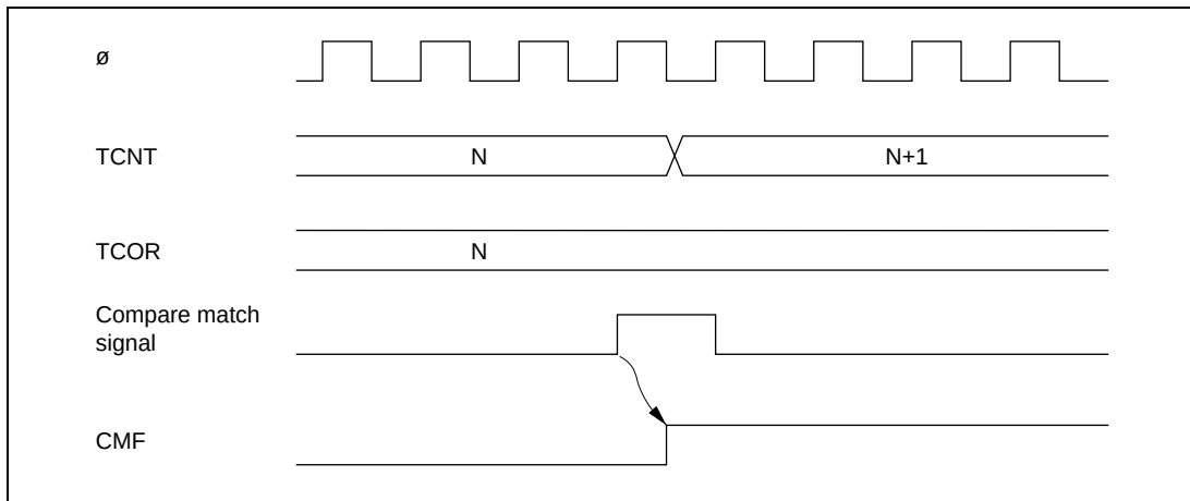
Figure 11.5 Timing of CMF Setting
