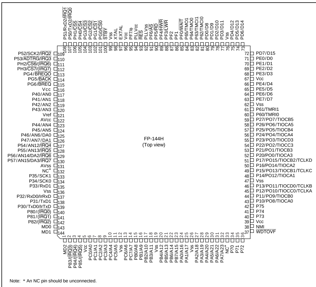
Figure 1.2 Pin Arrangement
