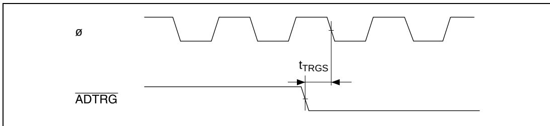
Figure 21.23 A/D Converter External Trigger Input Timing
