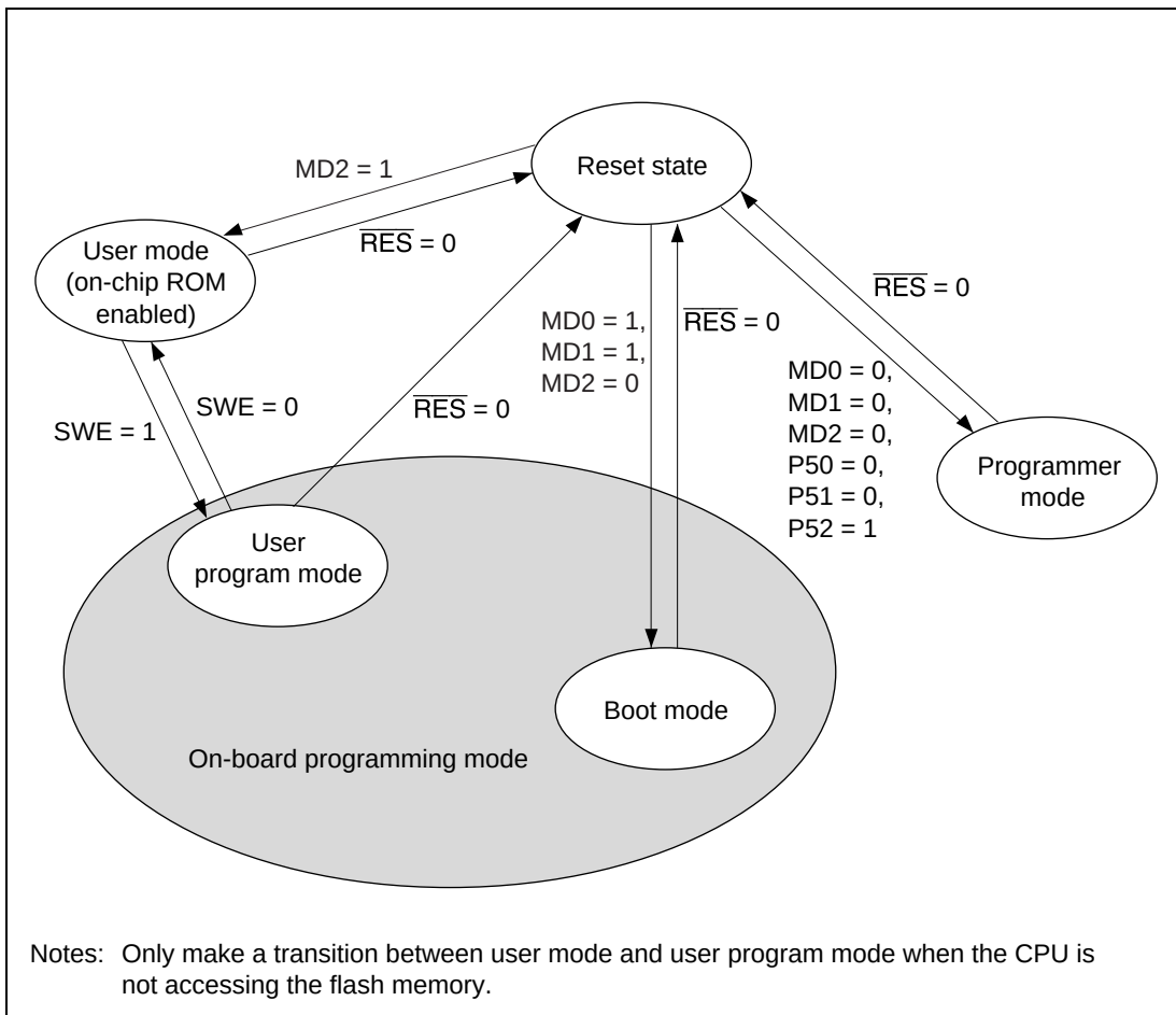
Figure 17.2 Flash Memory State Transitions
