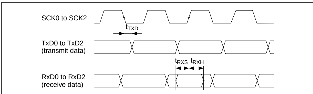
Figure 21.22 SCI Input/Output Timing: Synchronous Mode
