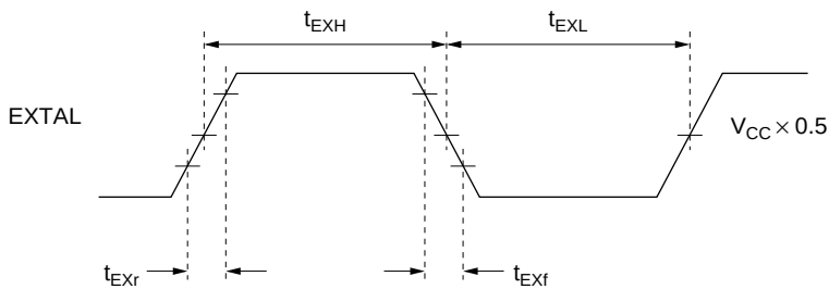
Figure 18.5 External Clock Input Timing
