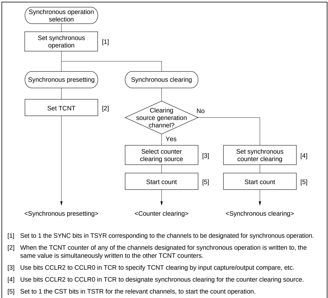
Figure 9.10 Example of Synchronous Operation Setting Procedure
