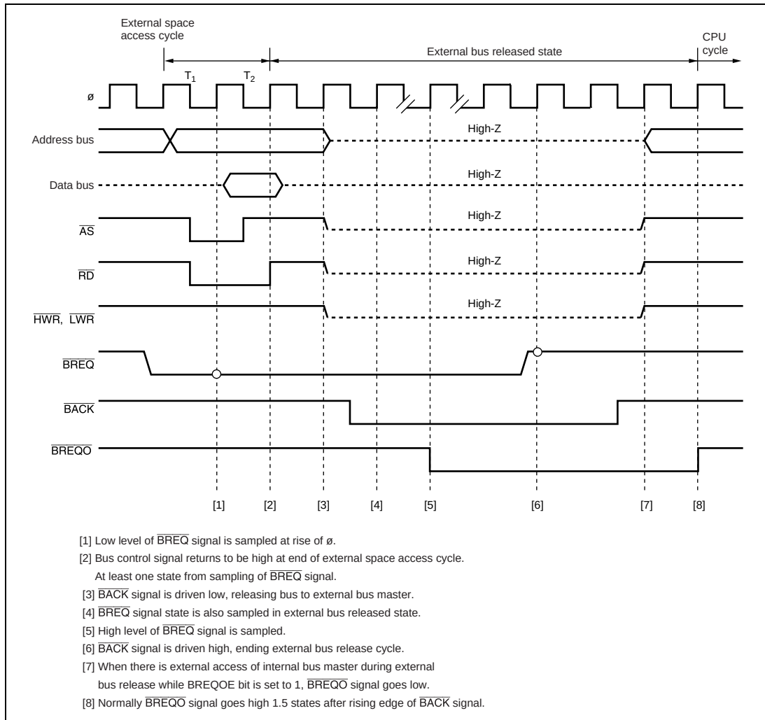
Figure 6.24 Bus Released State Transition Timing
