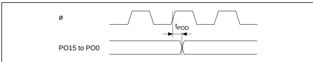
Figure 21.14 PPG Output Timing
