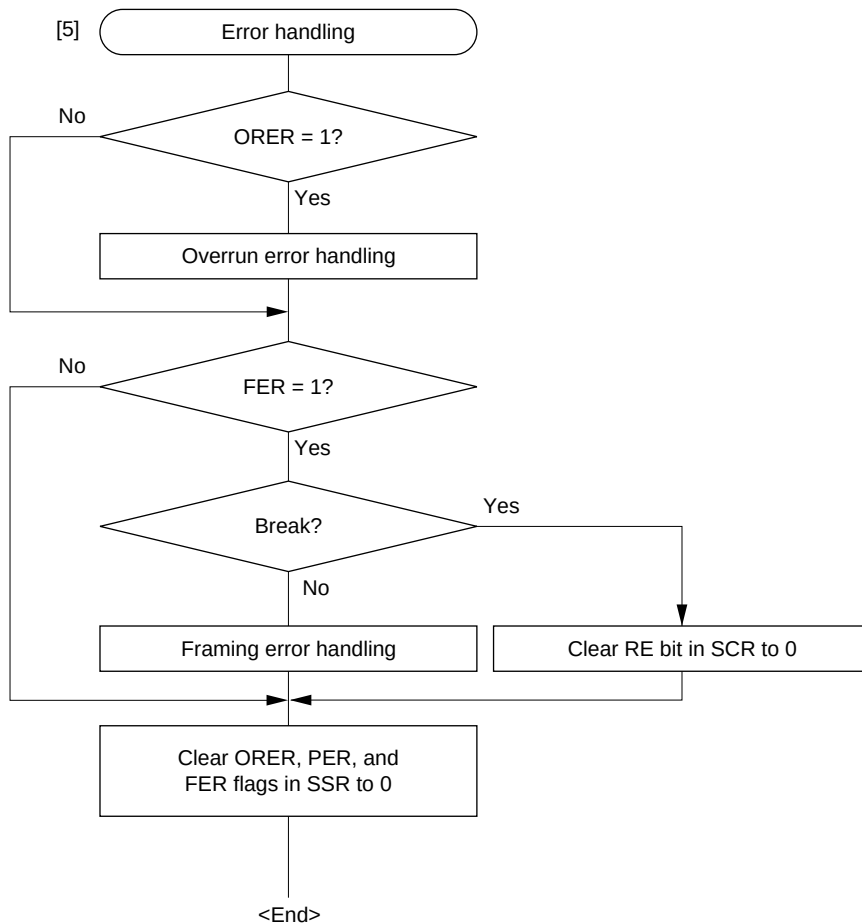
Figure 13.13 Sample Multiprocessor Serial Reception Flowchart (2)
