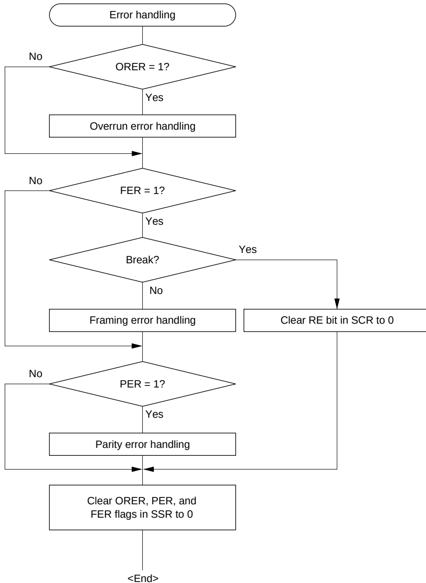
Figure 13.9 Sample Serial Reception Data Flowchart (2)
