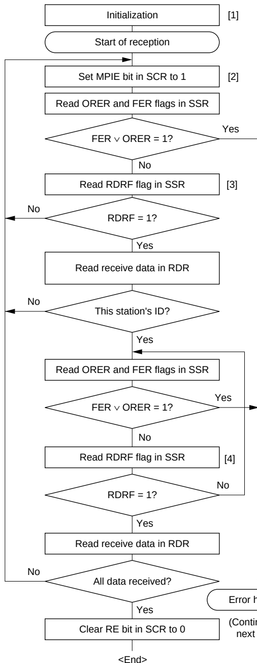
Figure 13.13 Sample Multiprocessor Serial Reception Flowchart (1)
