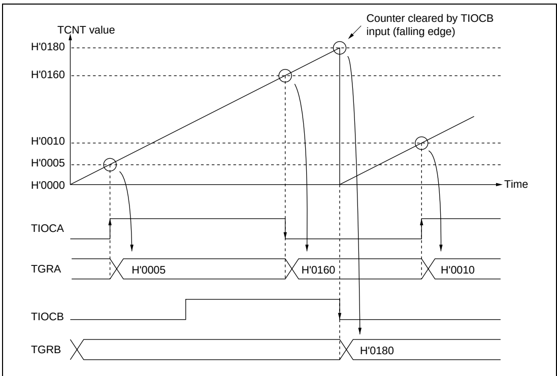
Figure 9.9 Example of Input Capture Operation
