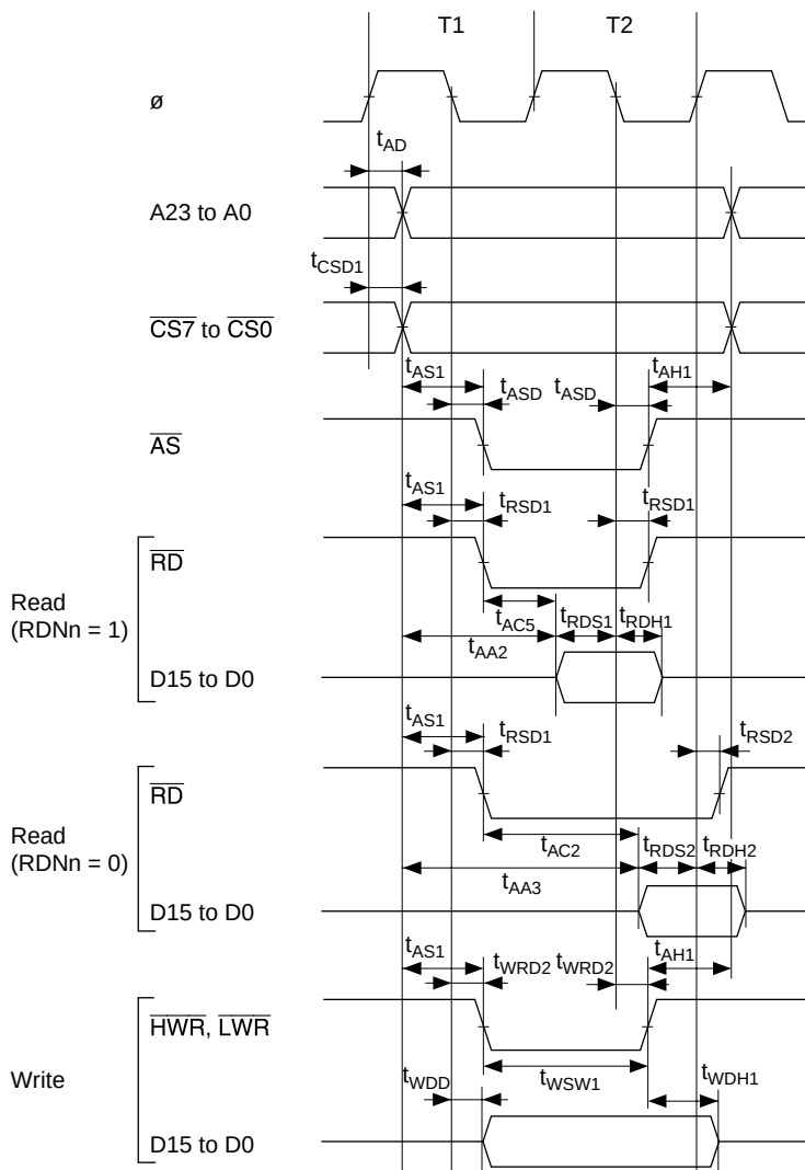
Figure 21.6 Basic Bus Timing: Two-State Access
