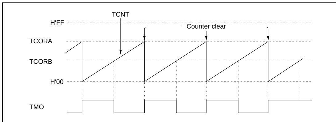
Figure 11.2 Example of Pulse Output
