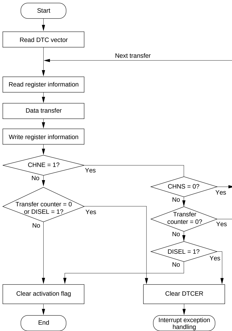
Figure 7.4 Flowchart of DTC Operation
