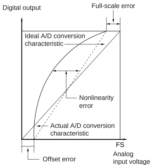
Figure 14.5 A/D Conversion Accuracy Definitions
