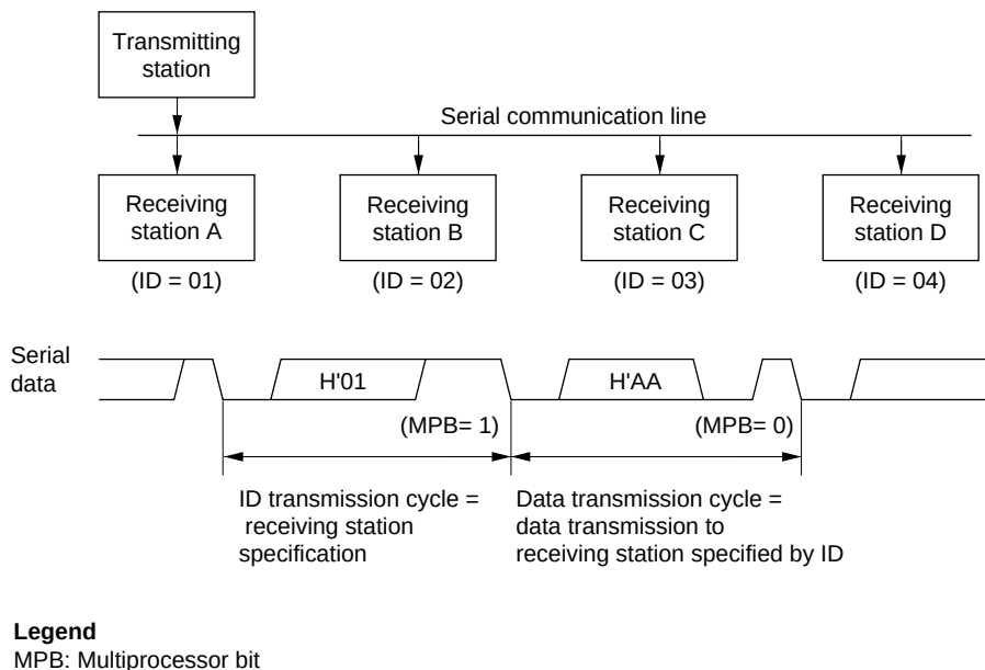
Figure 13.10 Example of Communication Using Multiprocessor Format (Transmission of Data H'AA to Receiving Station A)
