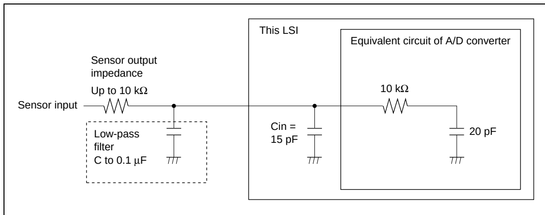
Figure 14.6 Example of Analog Input Circuit
