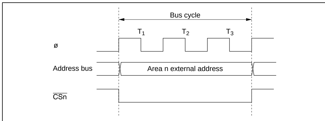
Figure 6.5 \overline{CSn} Signal Output Timing (n = 0 to 7)
