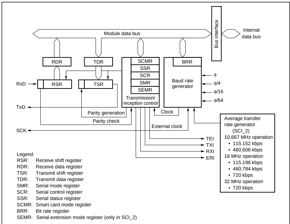
Figure 13.1 Block Diagram of SCI
