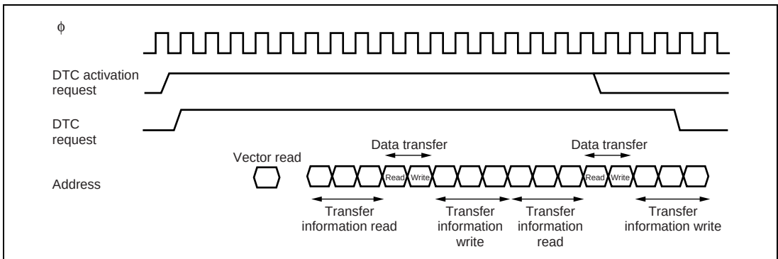
Figure 7.11 DTC Operation Timing (Example of Chain Transfer)
