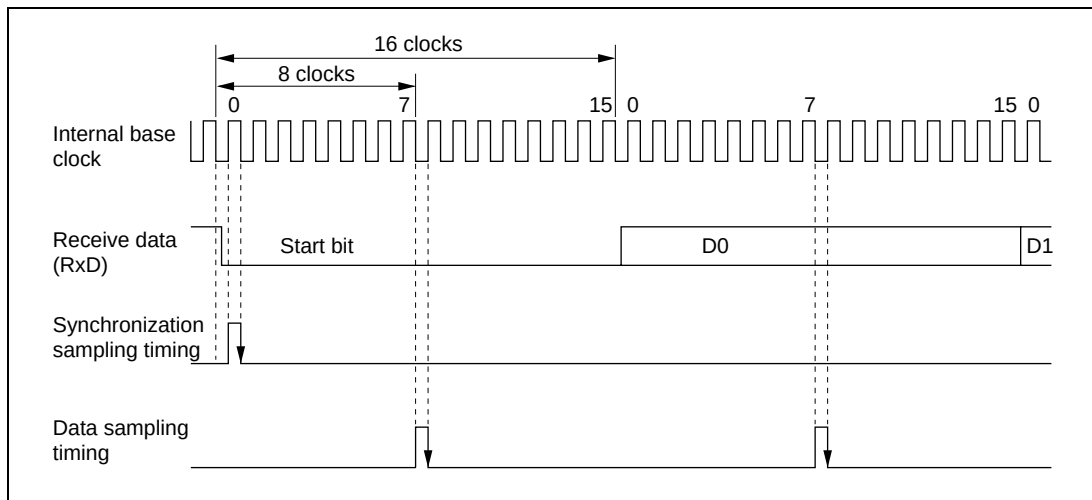
Figure 13.3 Receive Data Sampling Timing in Asynchronous Mode
