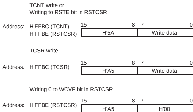
Figure 12.4 Writing to TCNT, TCSR, and RSTCSR
