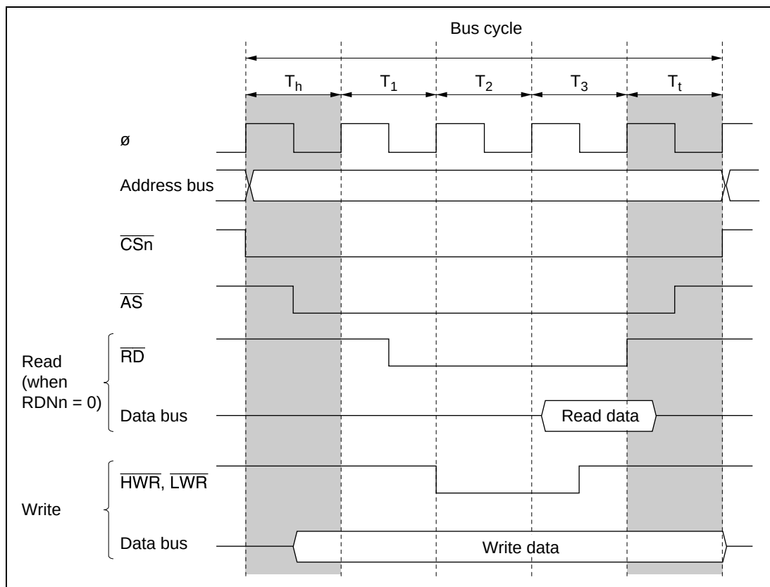
Figure 6.18 Example of Timing when Chip Select Assertion Period is Extended
