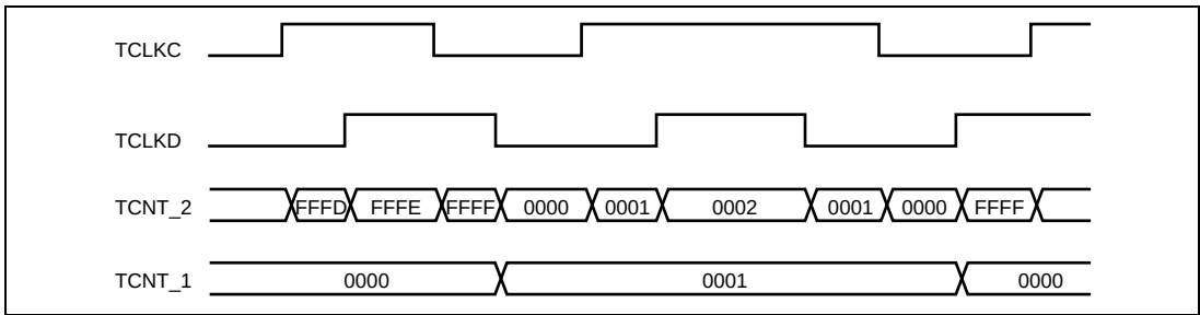
Figure 9.19 Example of Cascaded Operation (2)
