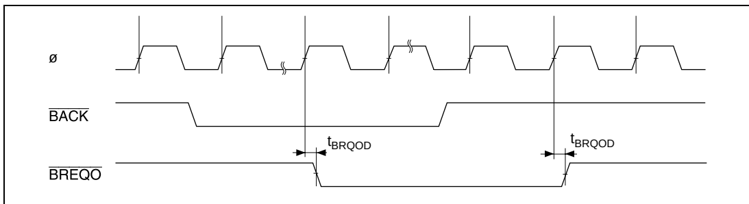
Figure 21.12 External Bus Request Output Timing
