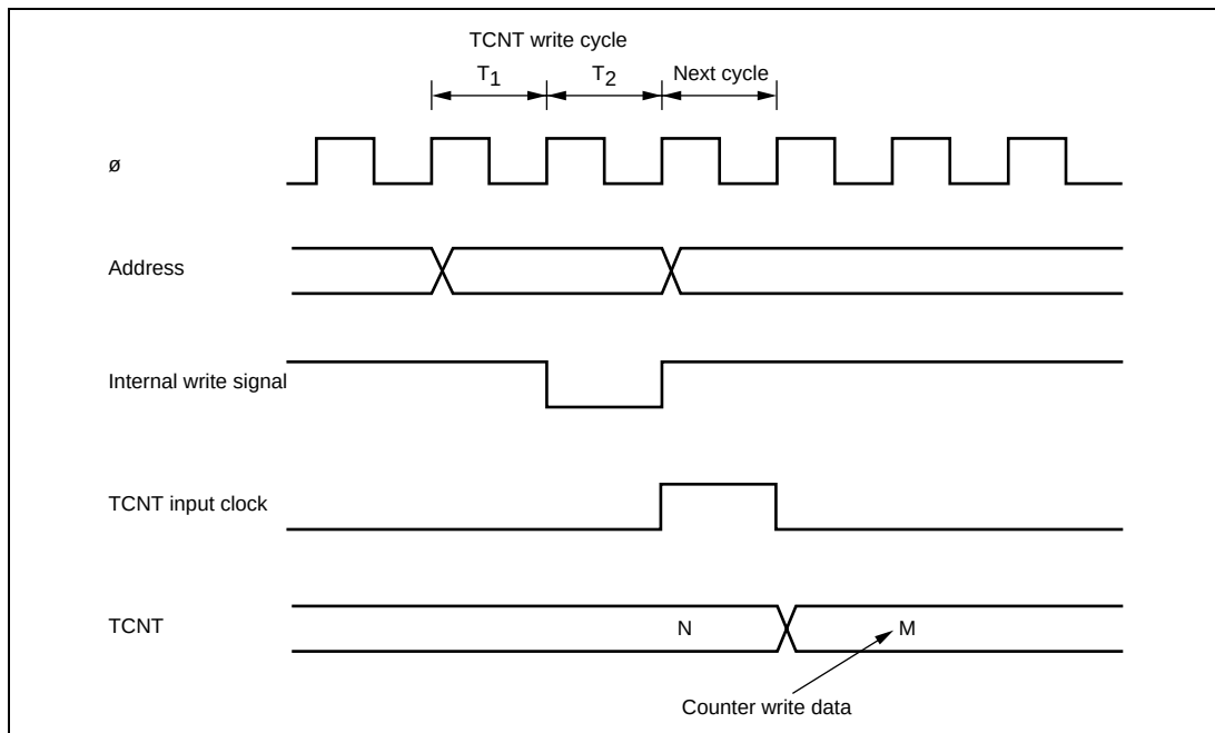
Figure 12.5 Contention between TCNT Write and Increment
