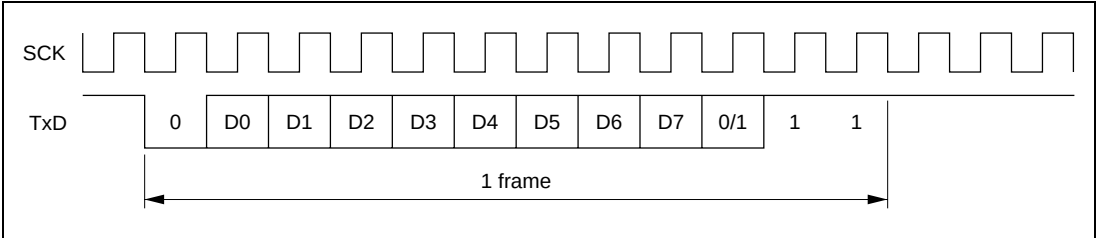
Figure 13.4 Relation between Output Clock and Transfer Data Phase (Asynchronous Mode)
