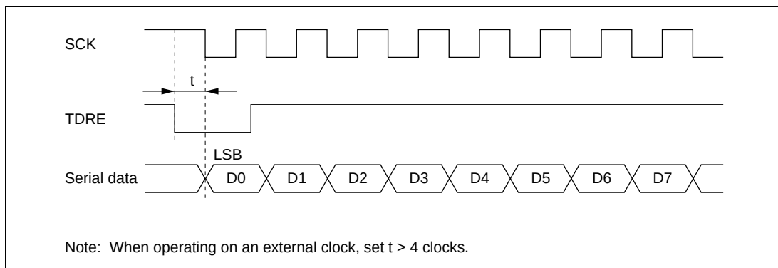
Figure 13.35 Example of Synchronous Transmission Using DTC
