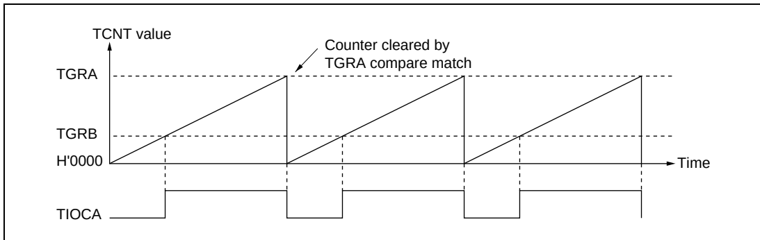
Figure 9.21 Example of PWM Mode Operation (1)
