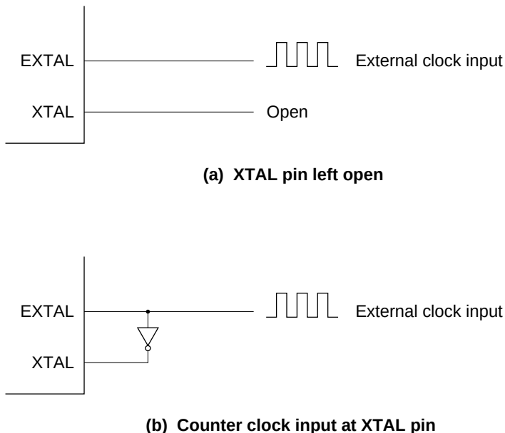
Figure 18.4 External Clock Input (Examples)
