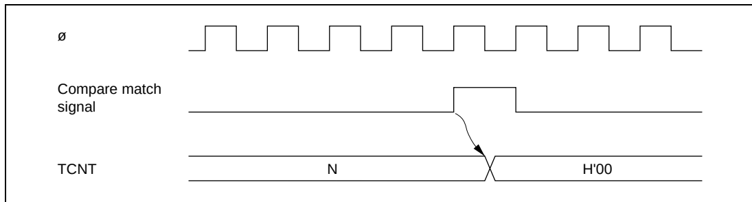
Figure 11.7 Timing of Compare Match Clear
