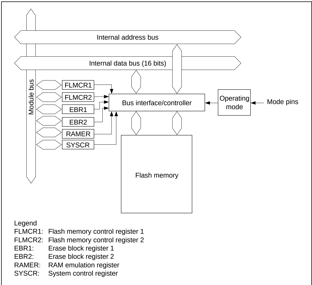
Figure 17.1 Block Diagram of Flash Memory
