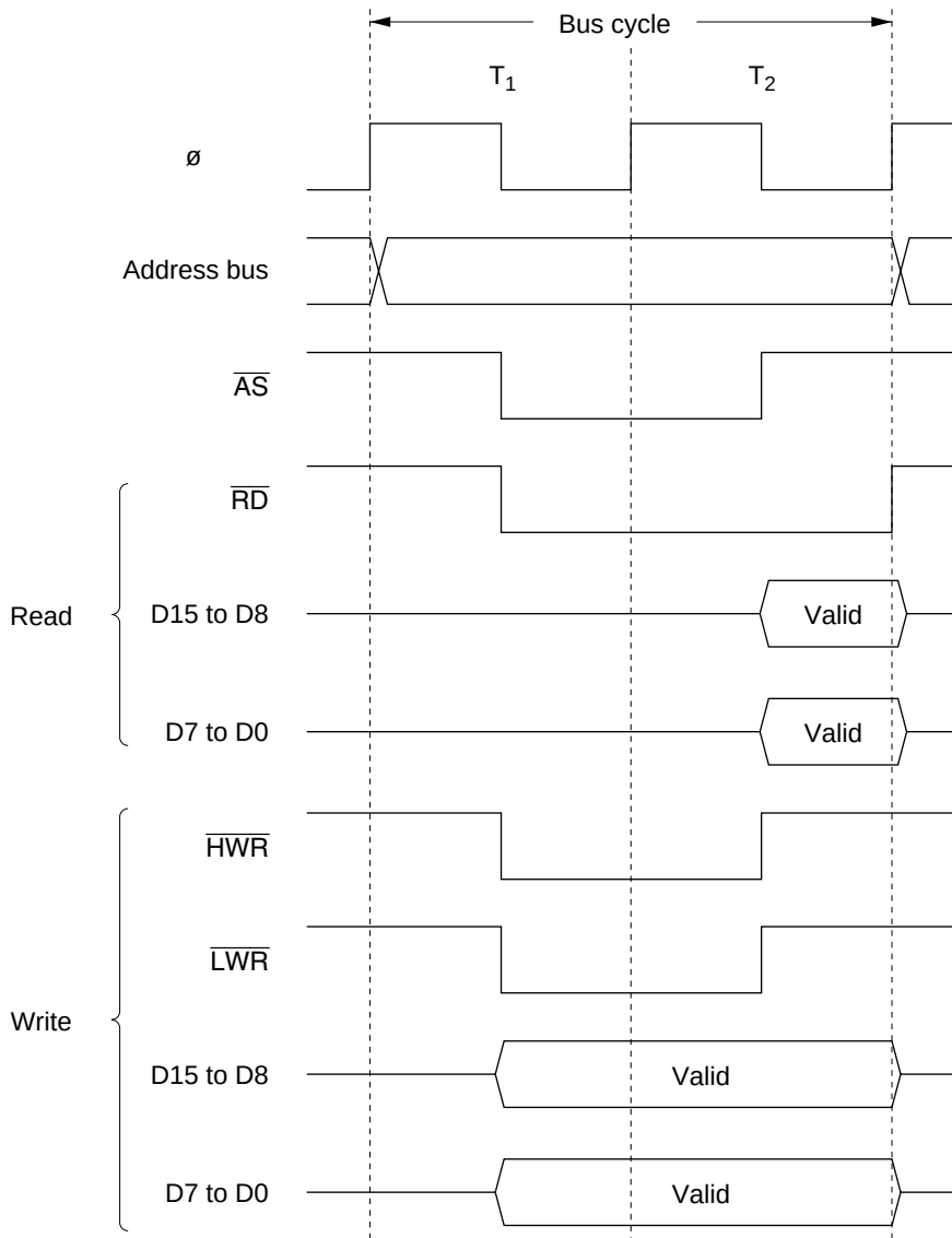
Figure 7-9 Bus Timing for 16-Bit 2-State Access Space (3) (Word Access)
