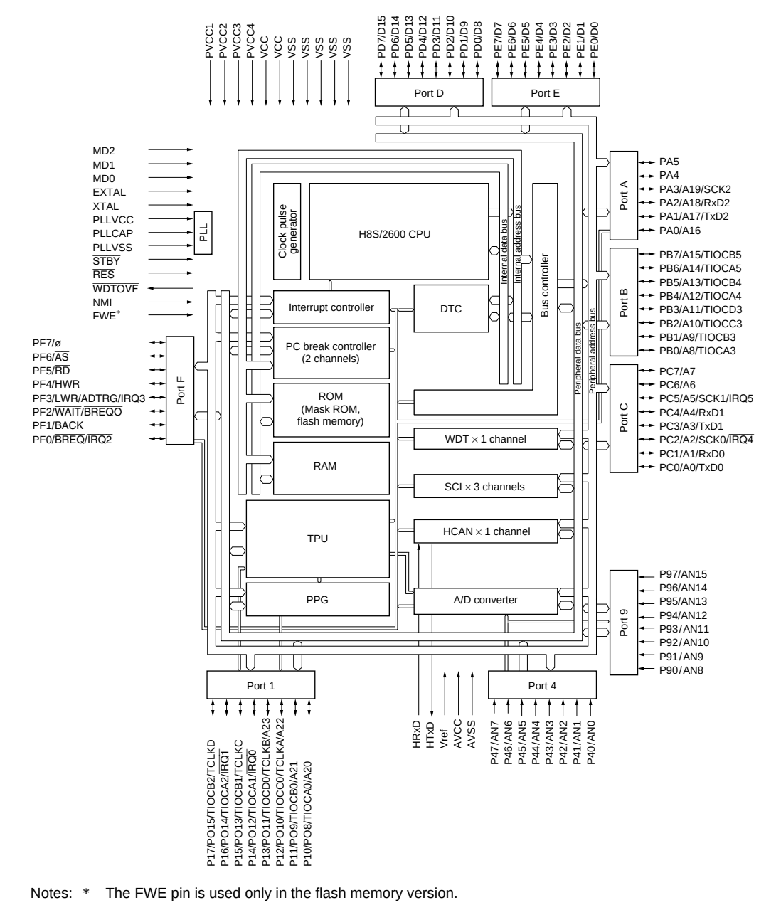
Figure 1-1 Internal Block Diagram (H8S/2623 Series)
