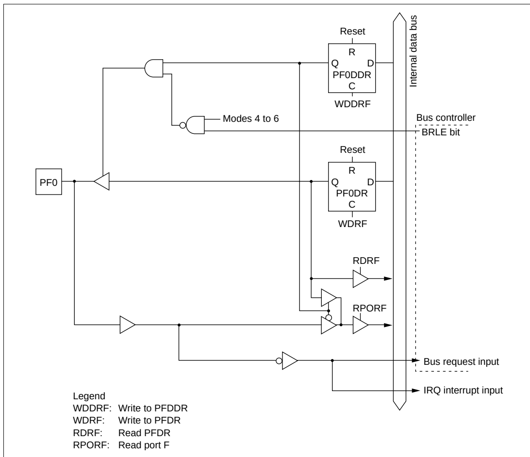
Figure C-9 (a) Port F Block Diagram (Pin PF0)
