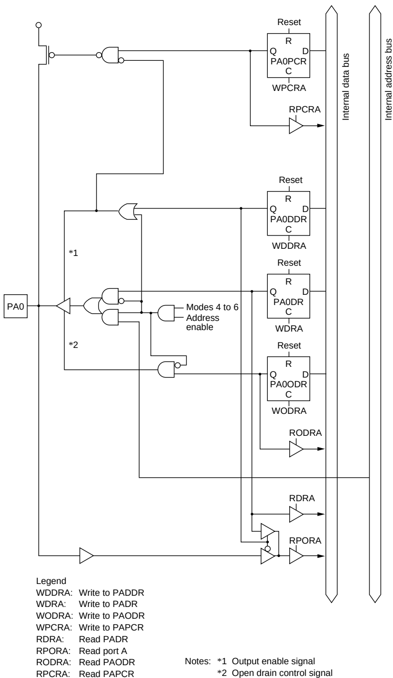
Figure C-4 (a) Port A Block Diagram (Pin PA0)
