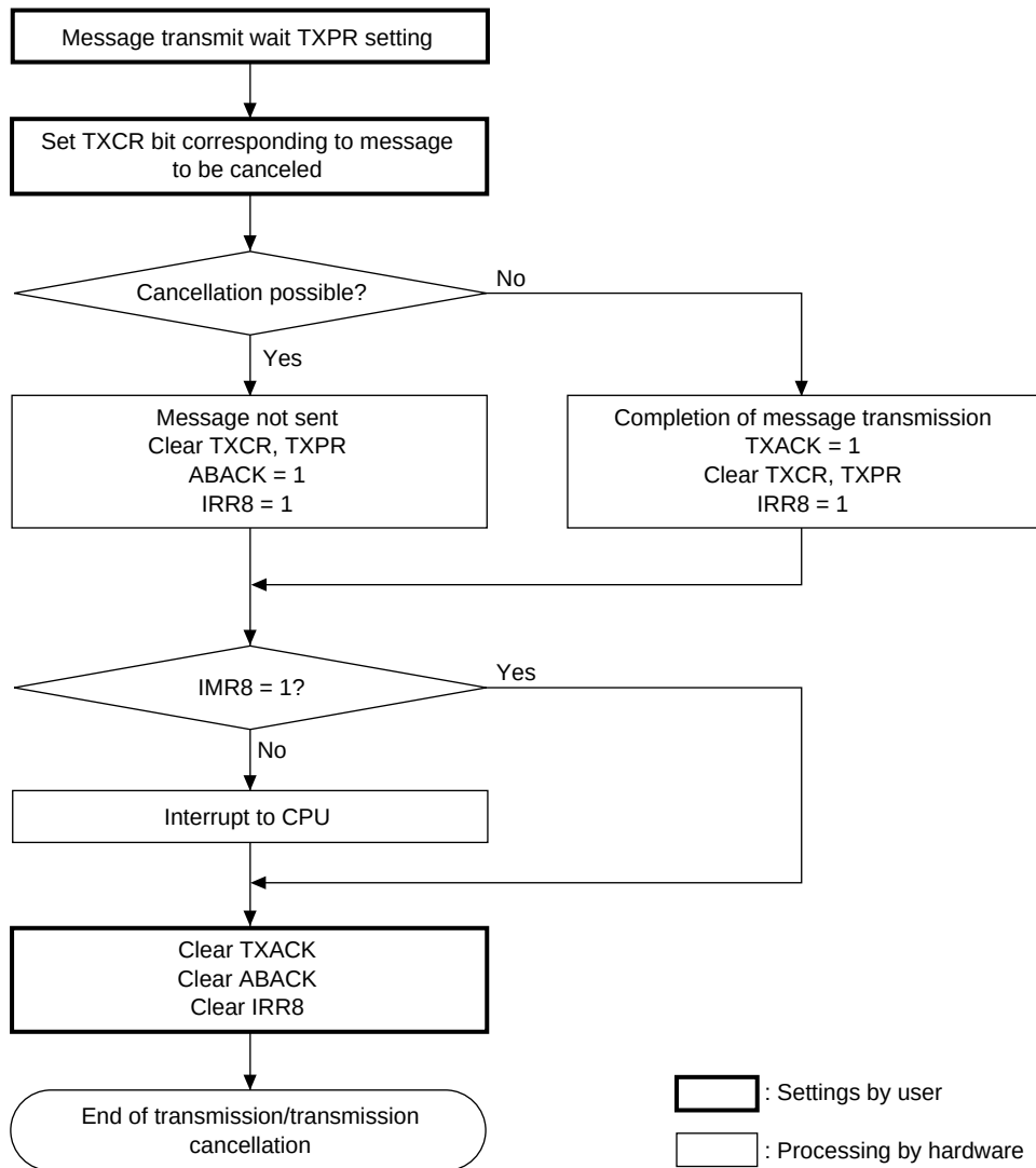
Figure 15-8 Transmit Message Cancellation Flowchart
