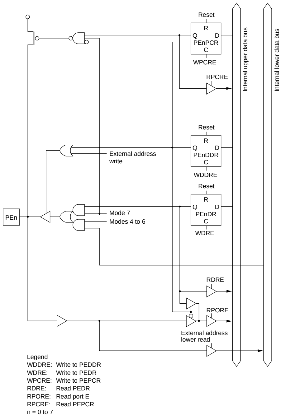
Figure C-8 Port E Block Diagram (Pins PE0 to PE7)
