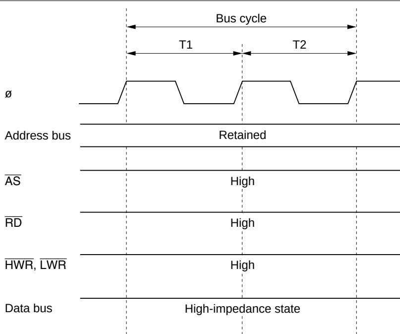
Figure 2-20 Pin States during On-Chip Supporting Module Access Cycle
