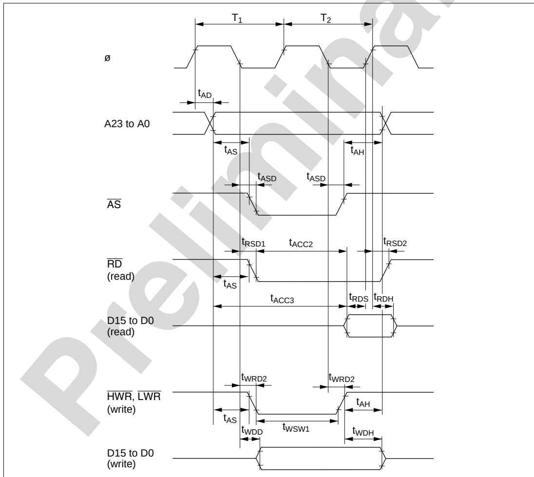
Figure 22-6 Basic Bus Timing (Two-State Access)
