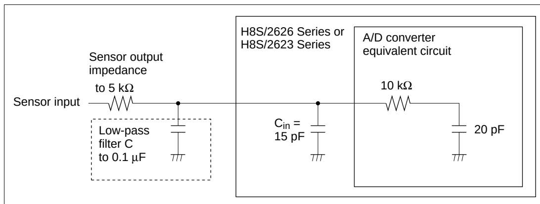
Figure 16-11 Example of Analog Input Circuit
