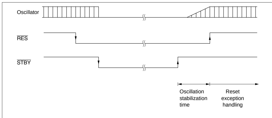
Figure 21A-4 Hardware Standby Mode Timing
