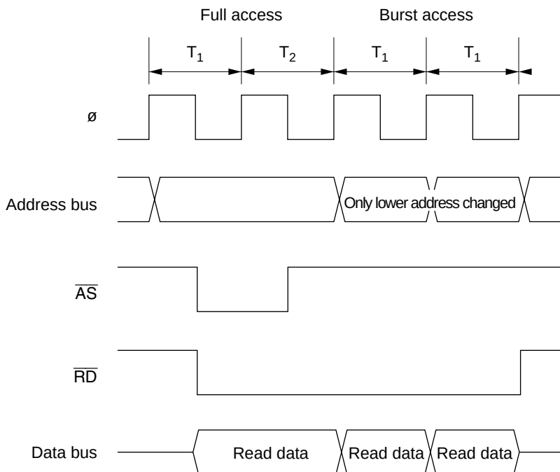
Figure 7-14 (b) Example of Burst ROM Access Timing (When AST0 = BRSTS1 = 0 )
