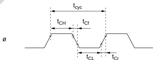
Figure 22-2 System Clock Timing
