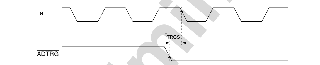
Figure 22-18 A/D Converter External Trigger Input Timing
