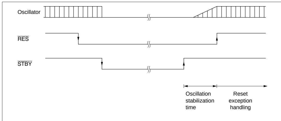
Figure 21B-4 Hardware Standby Mode Timing
