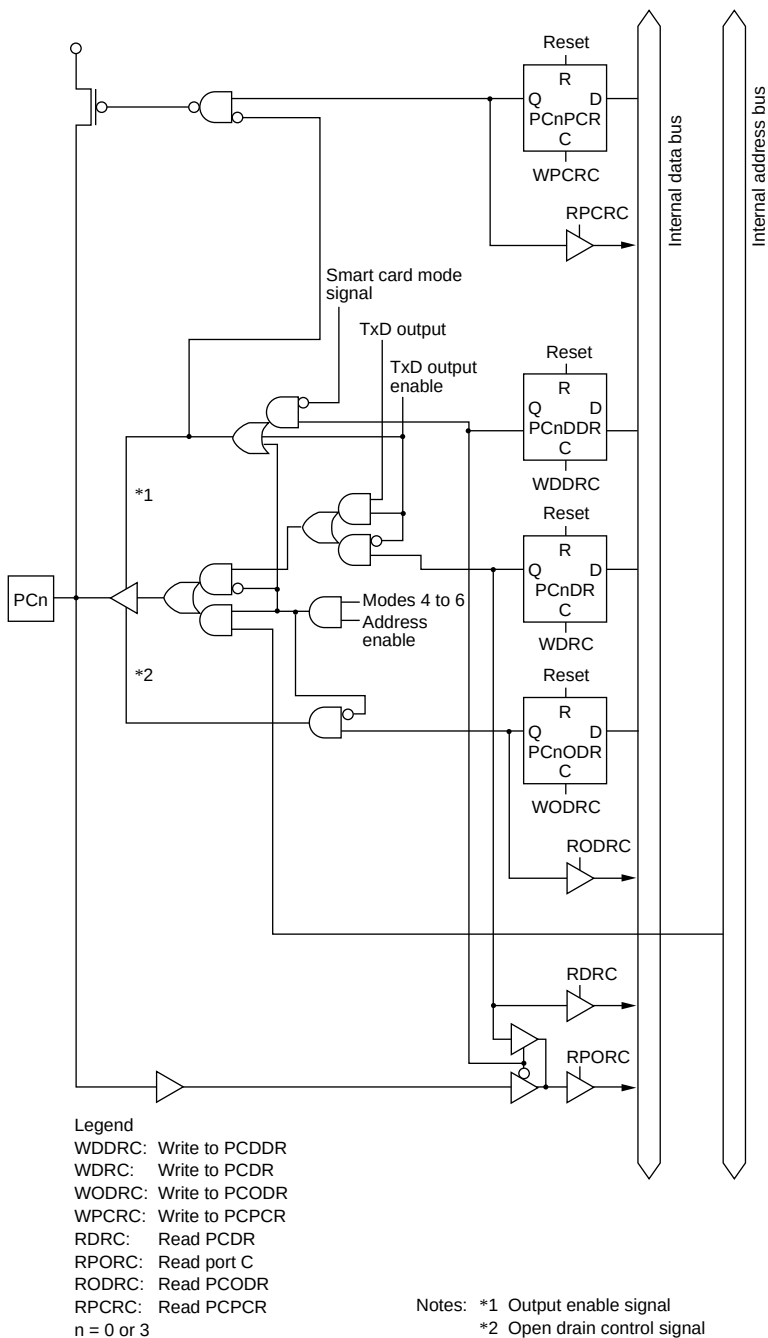
Figure C-6 (a) Port C Block Diagram (Pins PC0 and PC3)
