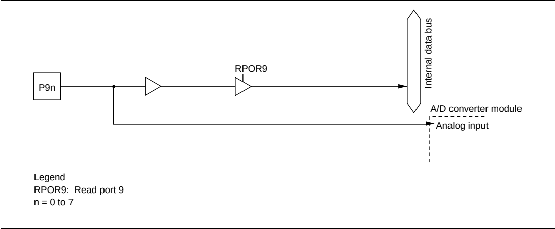
Figure C-3 Port 9 Block Diagram (Pins P90 to P97)
