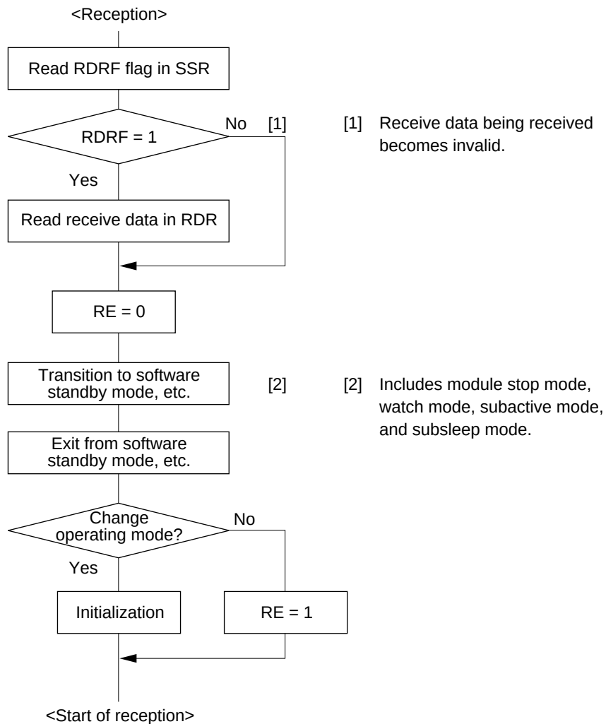
Figure 13-26 Sample Flowchart for Mode Transition during Reception
