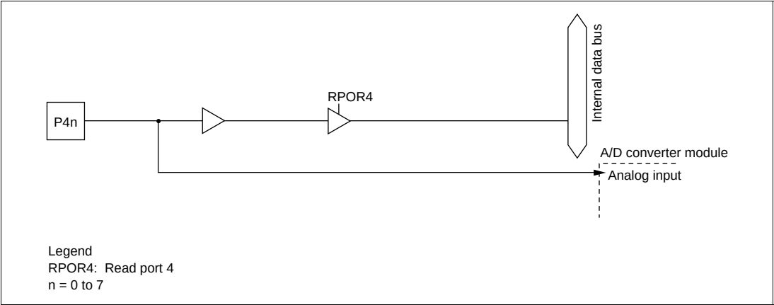
Figure C-2 Port 4 Block Diagram (Pins P40 to P47)
