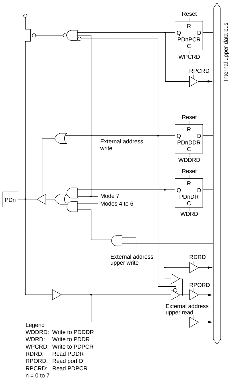
Figure C-7 Port D Block Diagram (Pins PD0 to PD7)
