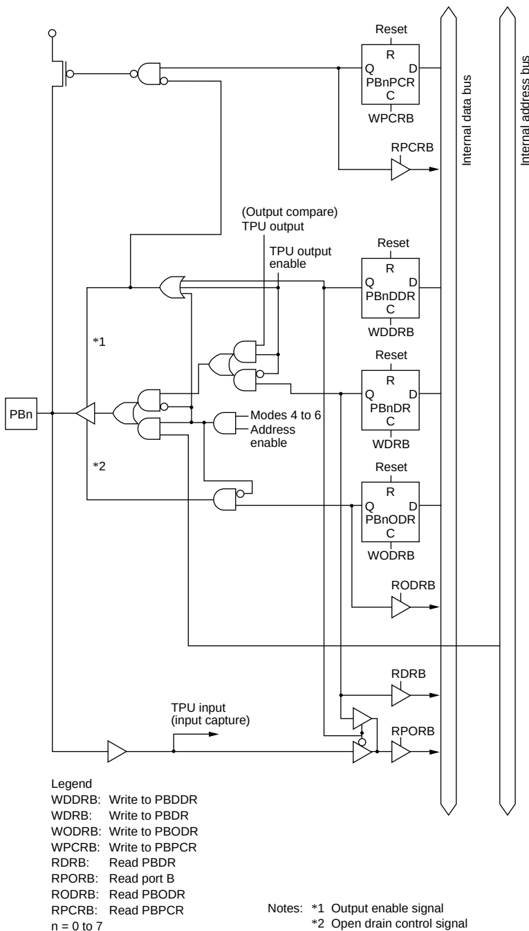
Figure C-5 Port B Block Diagram (Pins PB0 to PB7)
