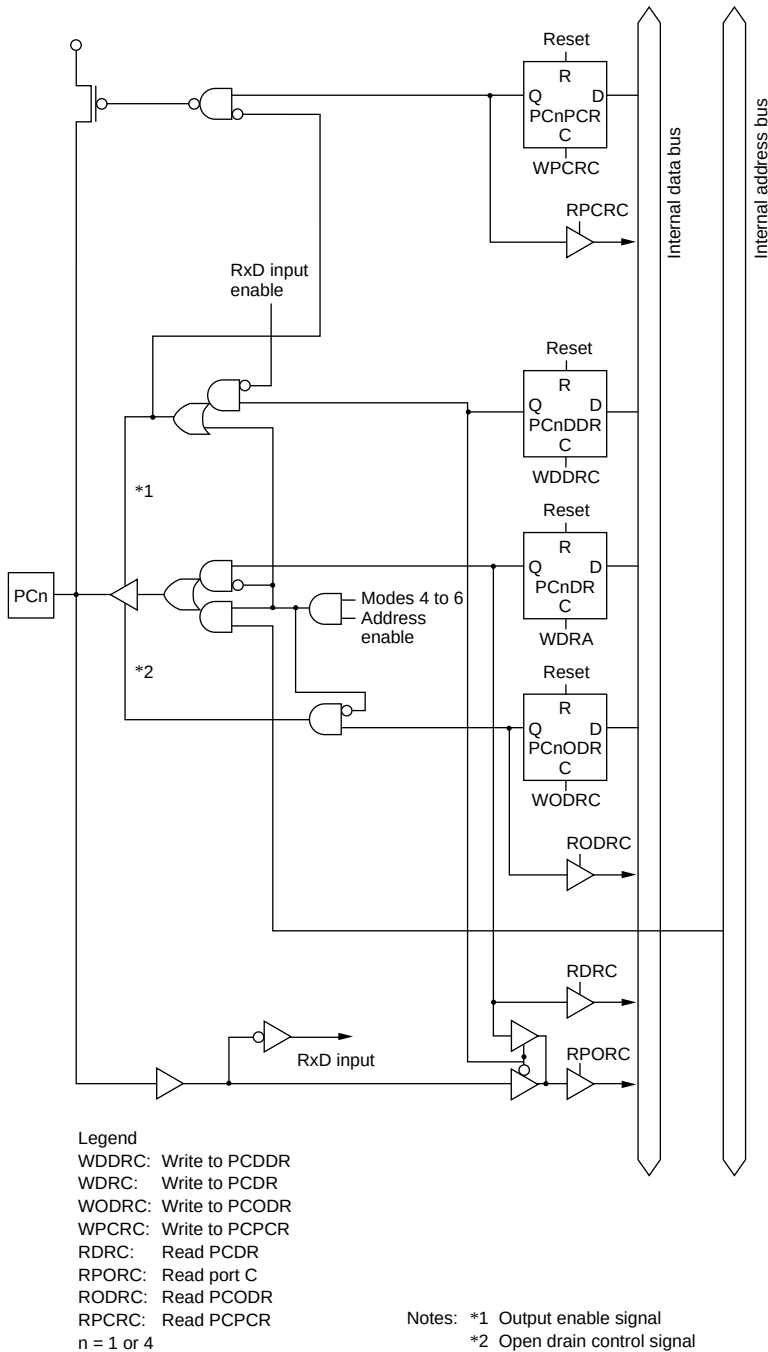
Figure C-6 (b) Port C Block Diagram (Pins PC1 and PC4)
