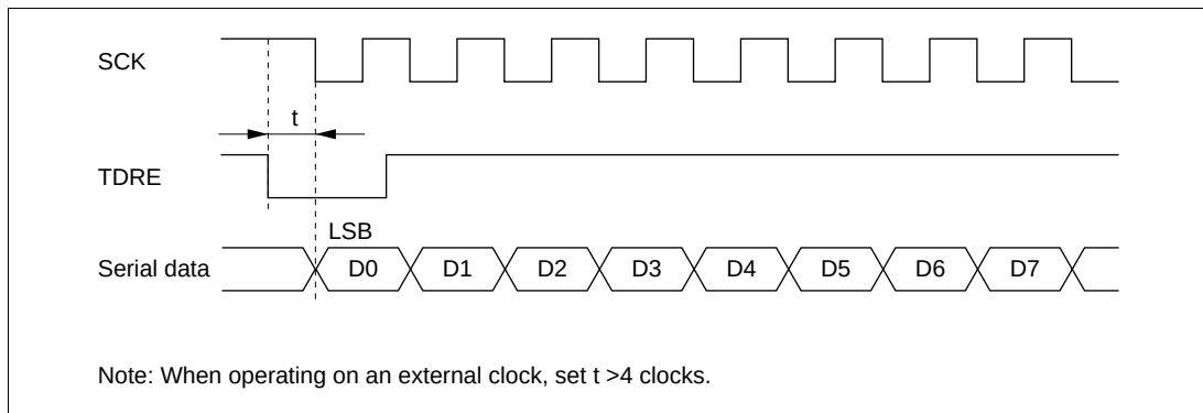
Figure 13-22 Example of Clocked Synchronous Transmission by DTC
