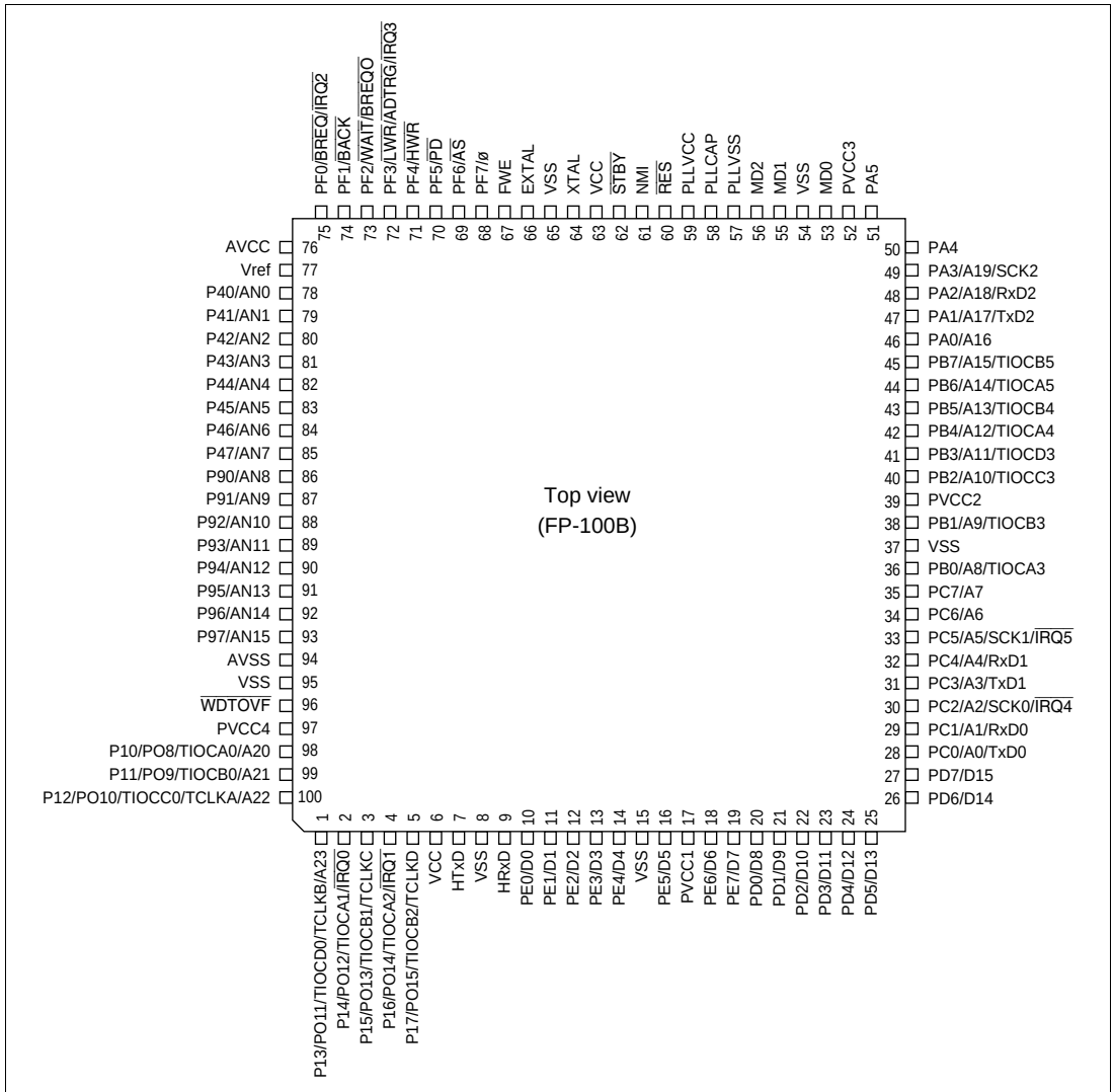
Figure 1-3 Pin Arrangement (FP-100B: Top View) (H8S/2623 Series)
