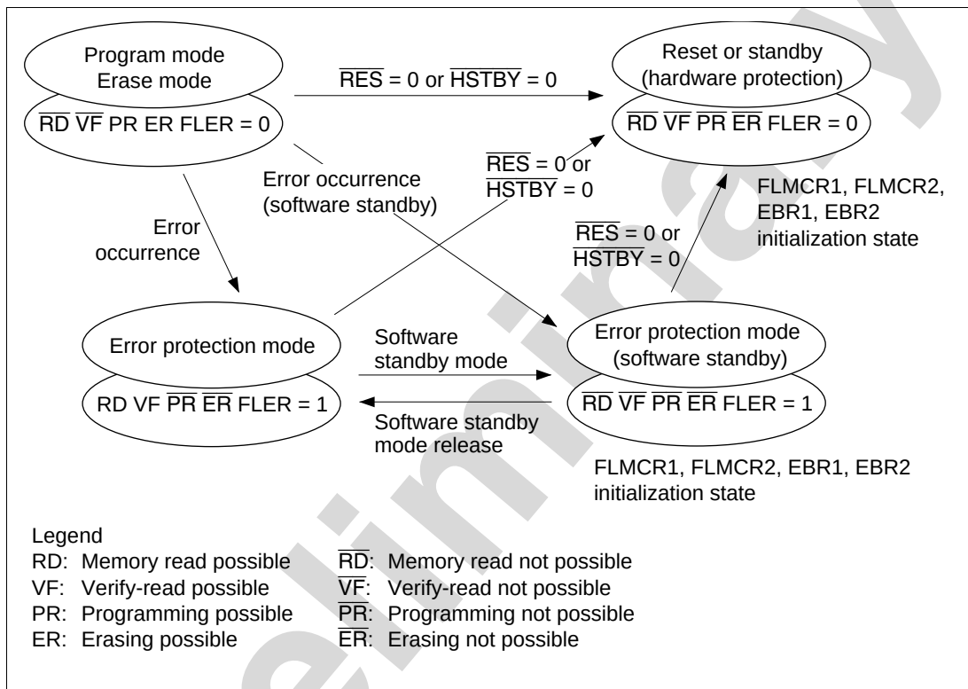
Figure 19-13 Flash Memory State Transitions
