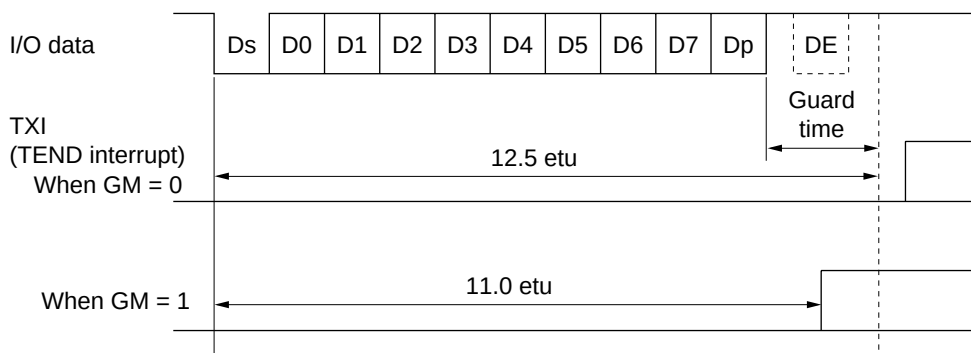
Figure 17-5 Relation Between Transmit Operation and Internal Registers
