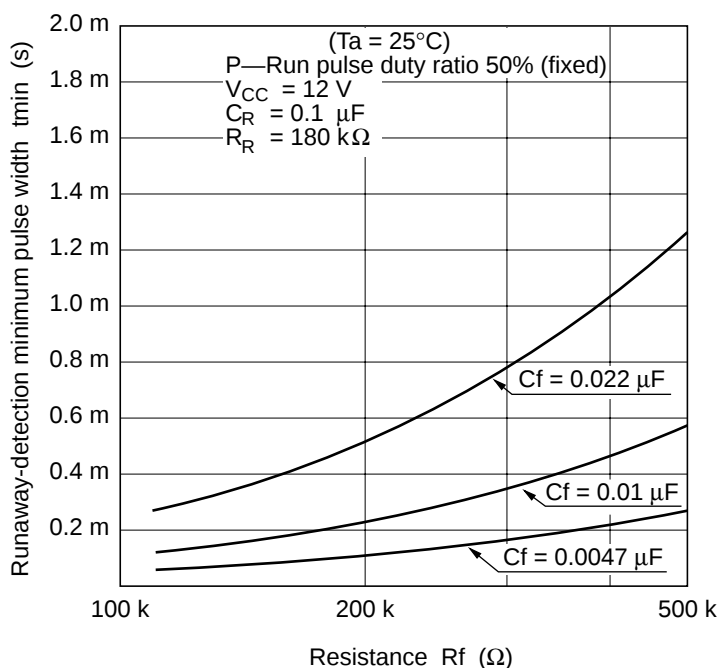
Figure 4 Characteristic of Power-On Reset Circuit
