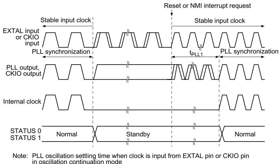
Figure 24.8 PLL Synchronization Settling Time during Standby Recovery (Reset or NMI)
