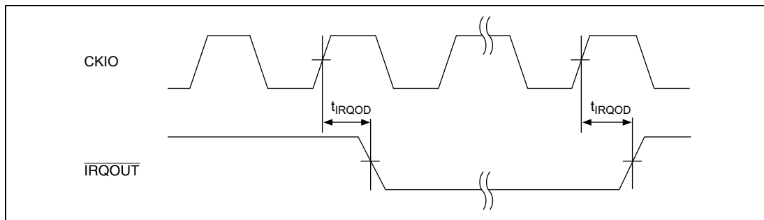
Figure 24.13 \overline{\text{IRQOUT}} Timing
