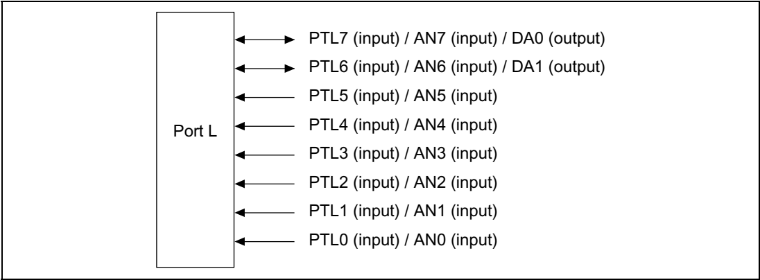
Figure 20.11 Port L
