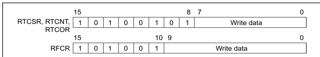
Figure 11.5 Writing to RFCR, RTCSR, RTCNT, and RTCOR
