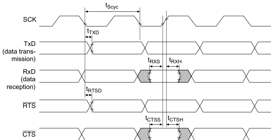
Figure 24.51 SCI I/O Timing in Synchronous Mode
