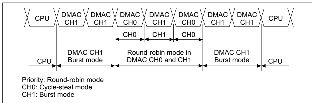
Figure 12.16 Bus State when Multiple Channels Are Operating
