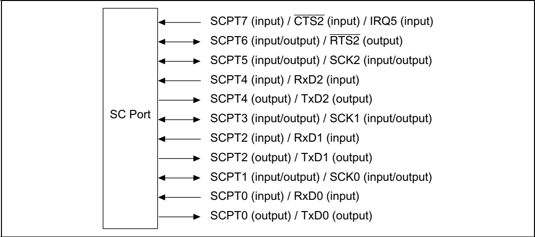
Figure 20.12 SC Port
