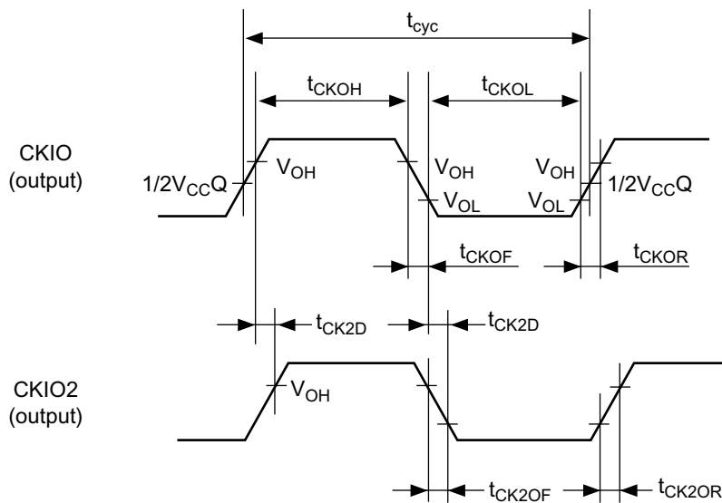
Figure 24.3 CKIO Clock Output Timing
