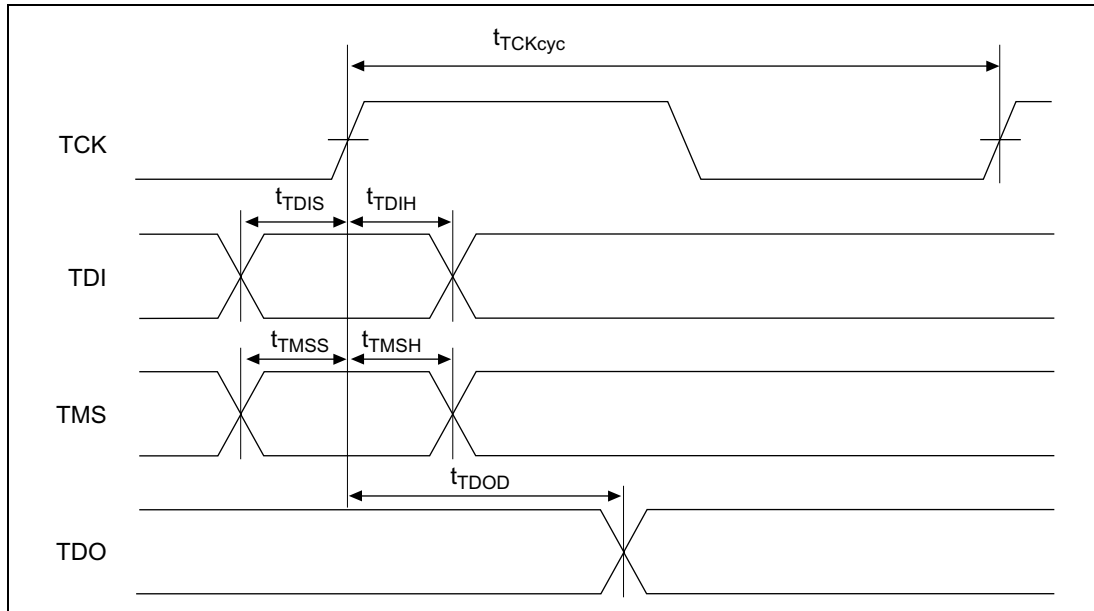
Figure 24.57 H-UDI Data Transfer Timing
