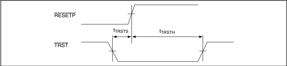
Figure 24.56 TRST Input Timing (Reset Hold)
