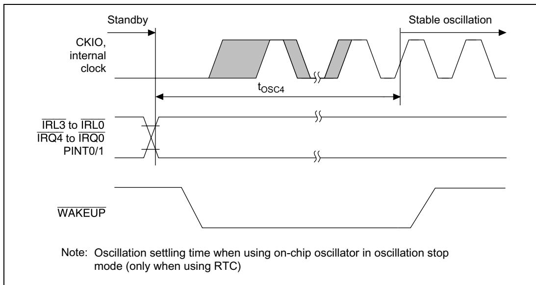
Figure 24.7 Oscillation Settling Time on Return from Standby (Return by \overline{IRQ4} to \overline{IRQ0} , \overline{PINT0/1} and \overline{IRL3} to \overline{IRL0} )
