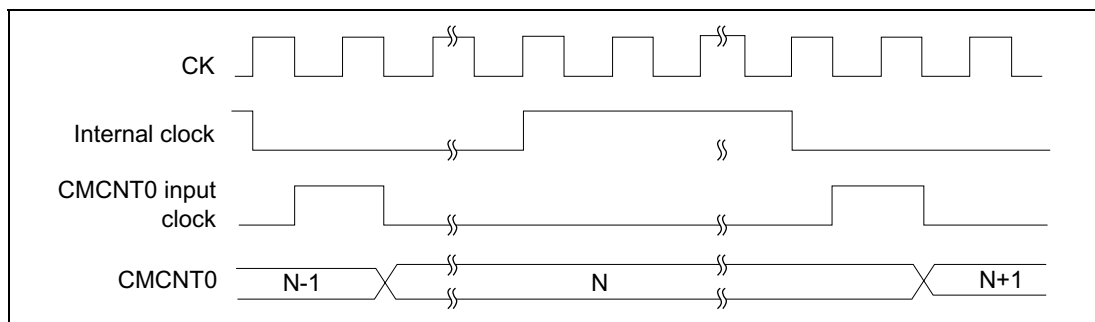
Figure 12.28 Count Timing
