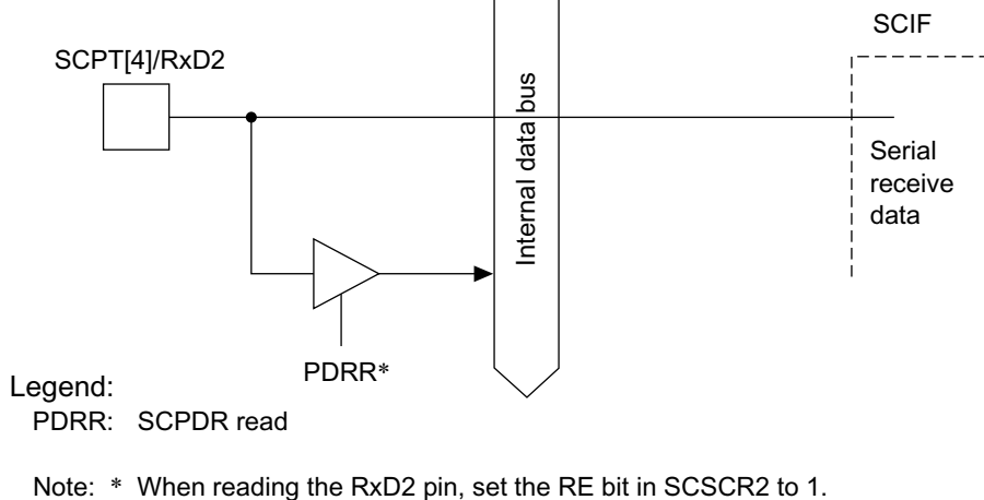
Figure 19.3 SCPT[4]/RxD2 Pin
