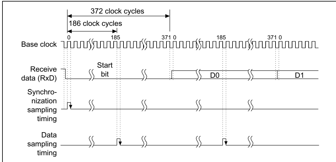
Figure 18.8 Receive Data Sampling Timing in Smart Card Mode
