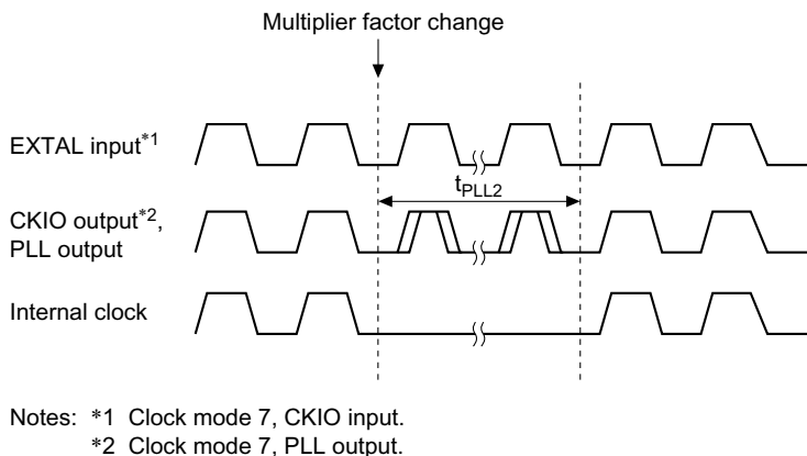
Figure 32.10 PLL Sync Stabilization Time at Frequency Multiplier Factor Change
