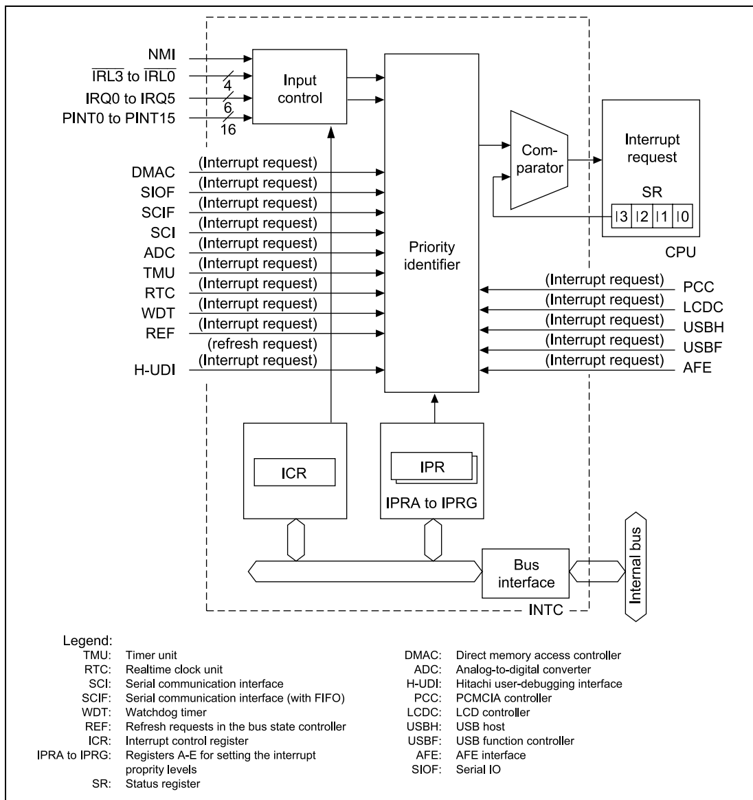
Figure 7.1 INTC Block Diagram
