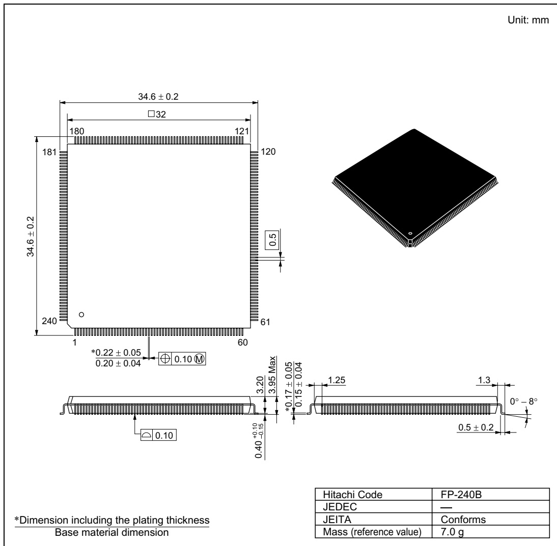
Figure D.1 Package Dimensions (FP-240B)
