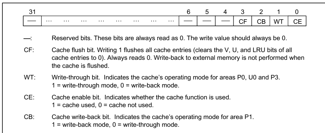
Figure 5.2 CCR Register Configuration
