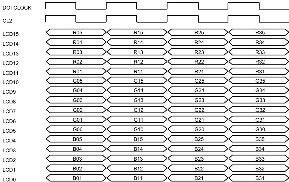
Figure 25.20 Clock and LCD Data Signal Example
