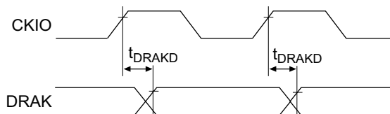
Figure 32.44 DRAK Output Timing
