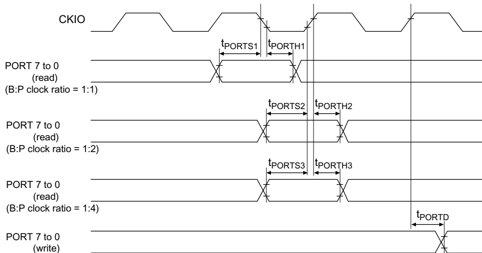
Figure 32.42 I/O Port Timing
