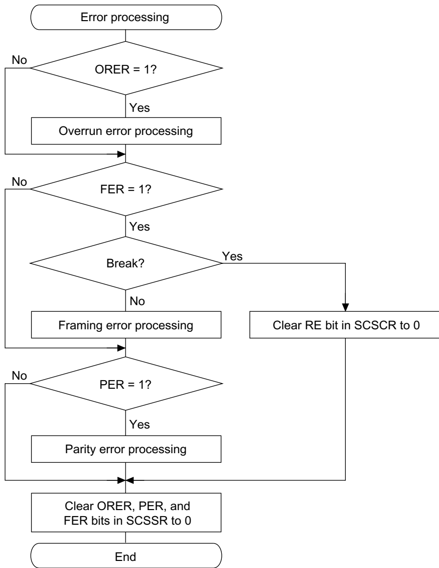
Figure 17.10 Sample Serial Reception Data Flowchart (2)
