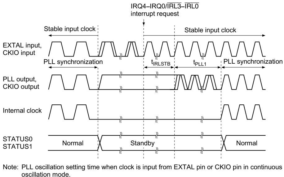
Figure 32.9 PLL Synchronization Settling Time by IRQ/IRL and PINT0/1 Interrupt
