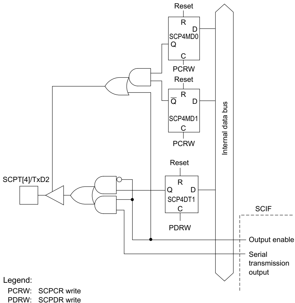
Figure 19.2 SCPT[4]/TxD2 Pin
