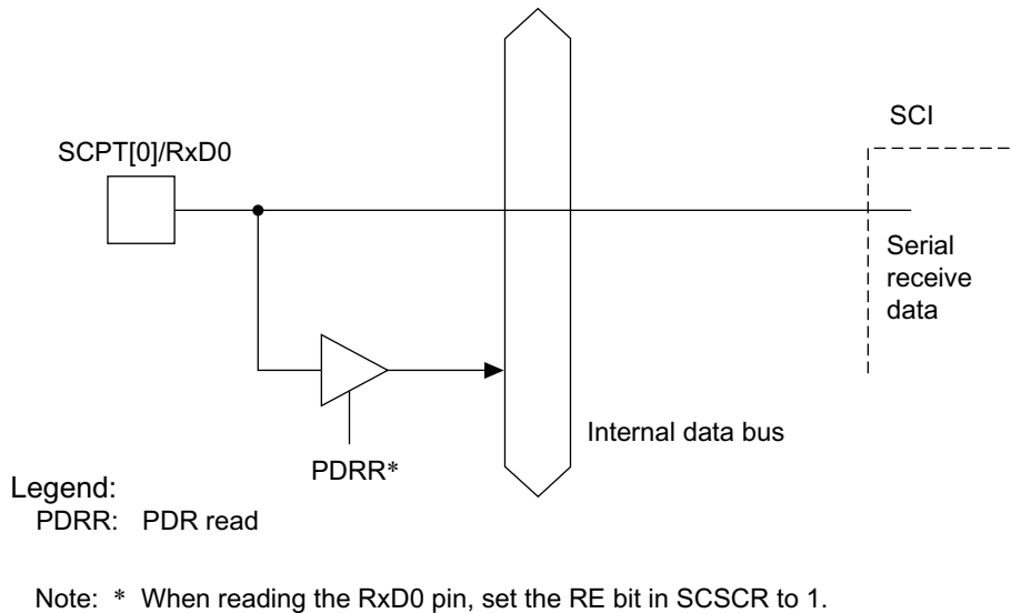
Figure 17.4 SCPT[0]/RxD0 Pin
