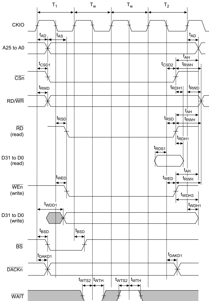
Figure 32.17 Basic Bus Cycle (External Wait, WAITSEL = 1)
