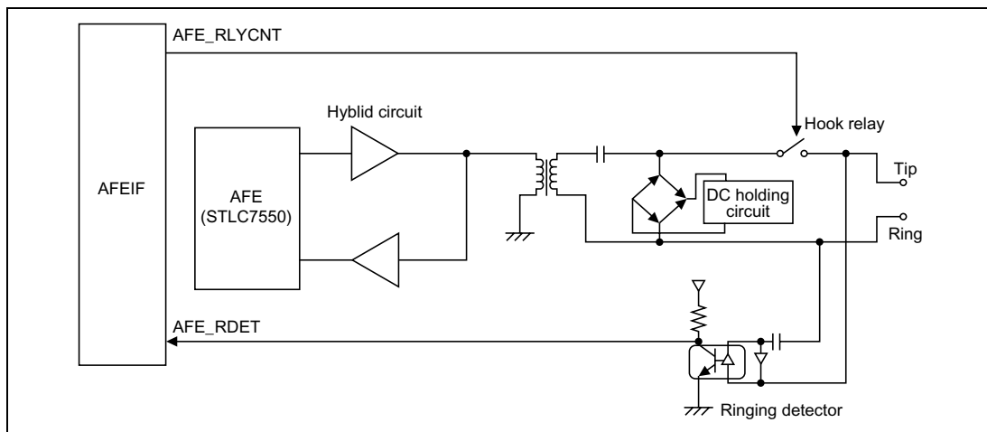
Figure 21.7 DAA Block Diagram
