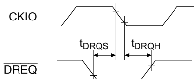
Figure 32.43 \overline{DREQ} Input Timing
