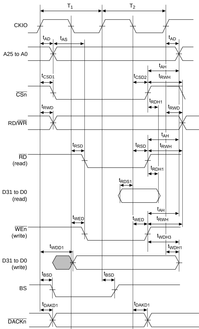
Figure 23.16 Basic Bus Cycle (No Wait)
