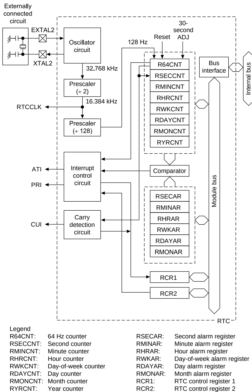
Figure 13.1 Block Diagram of RTC
