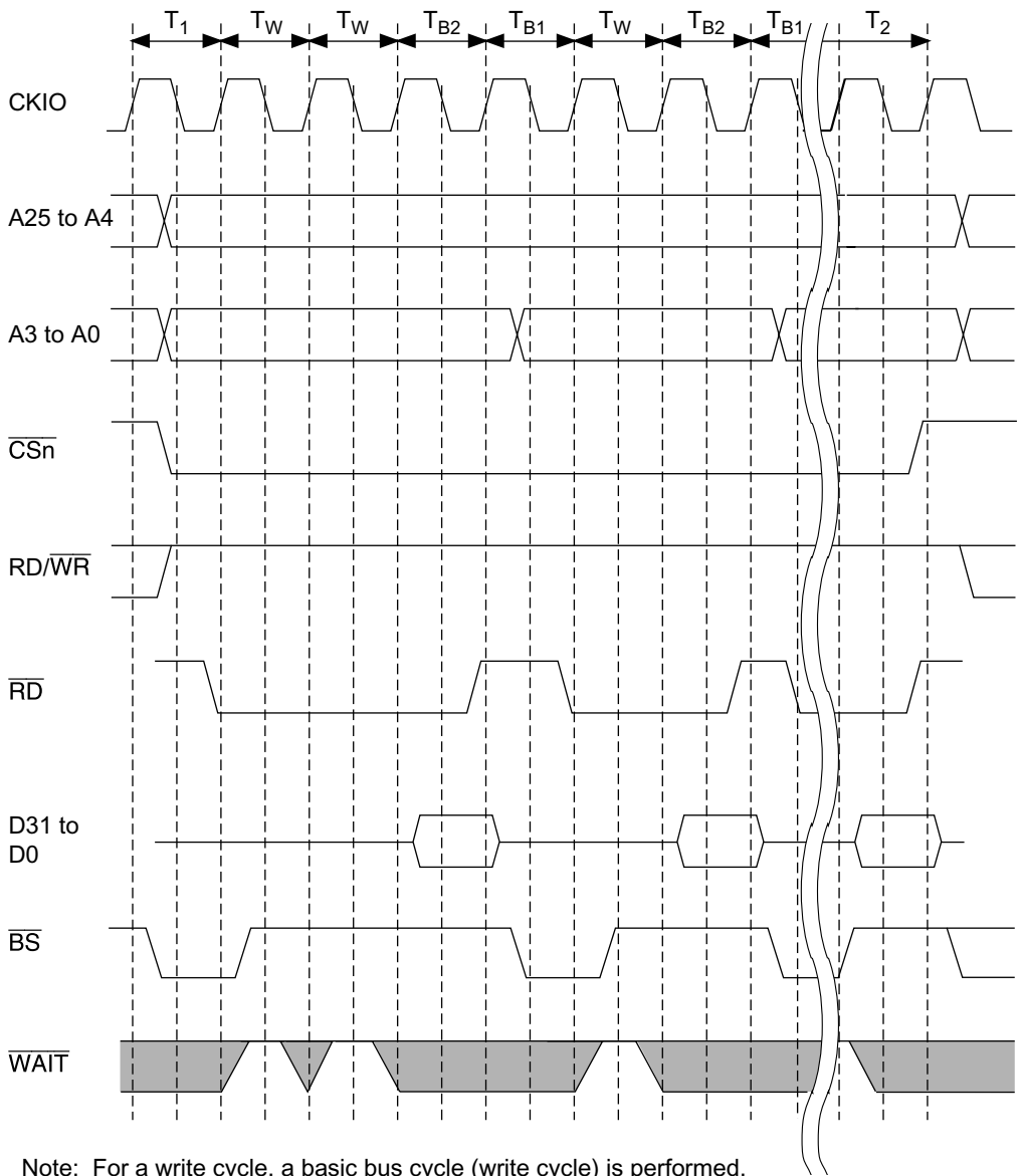
Figure 10.29 Burst ROM Wait Access Timing
