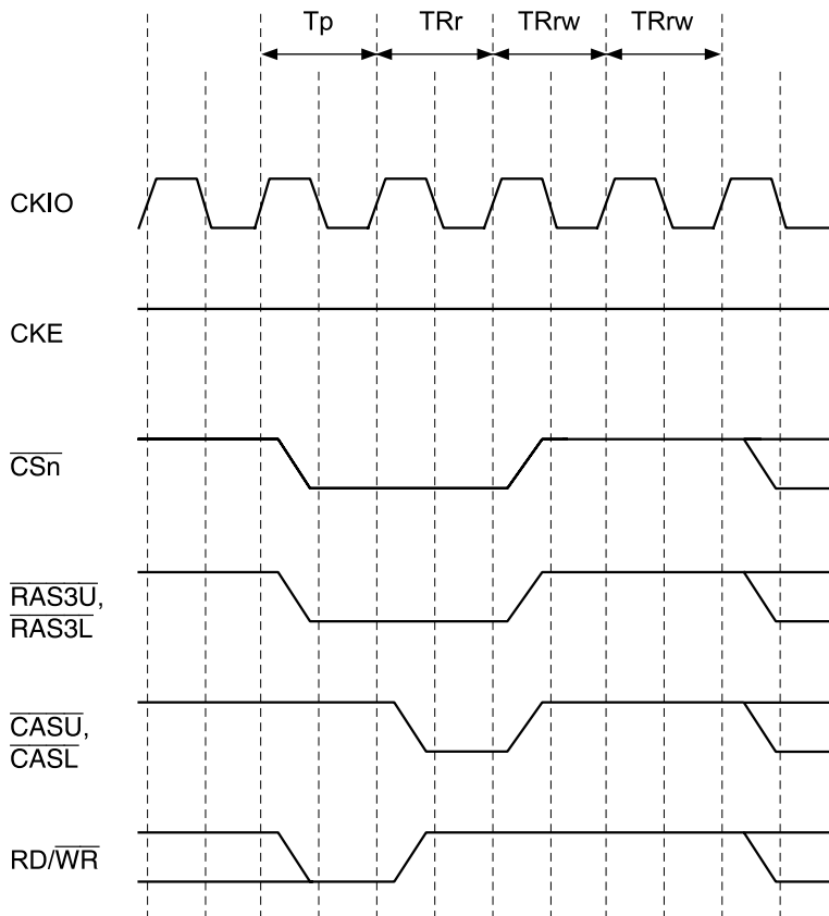
Figure 10.26 Synchronous DRAM Auto-Refresh Timing
