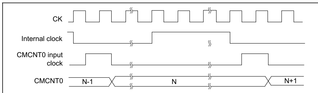
Figure 11.26 Count Timing
