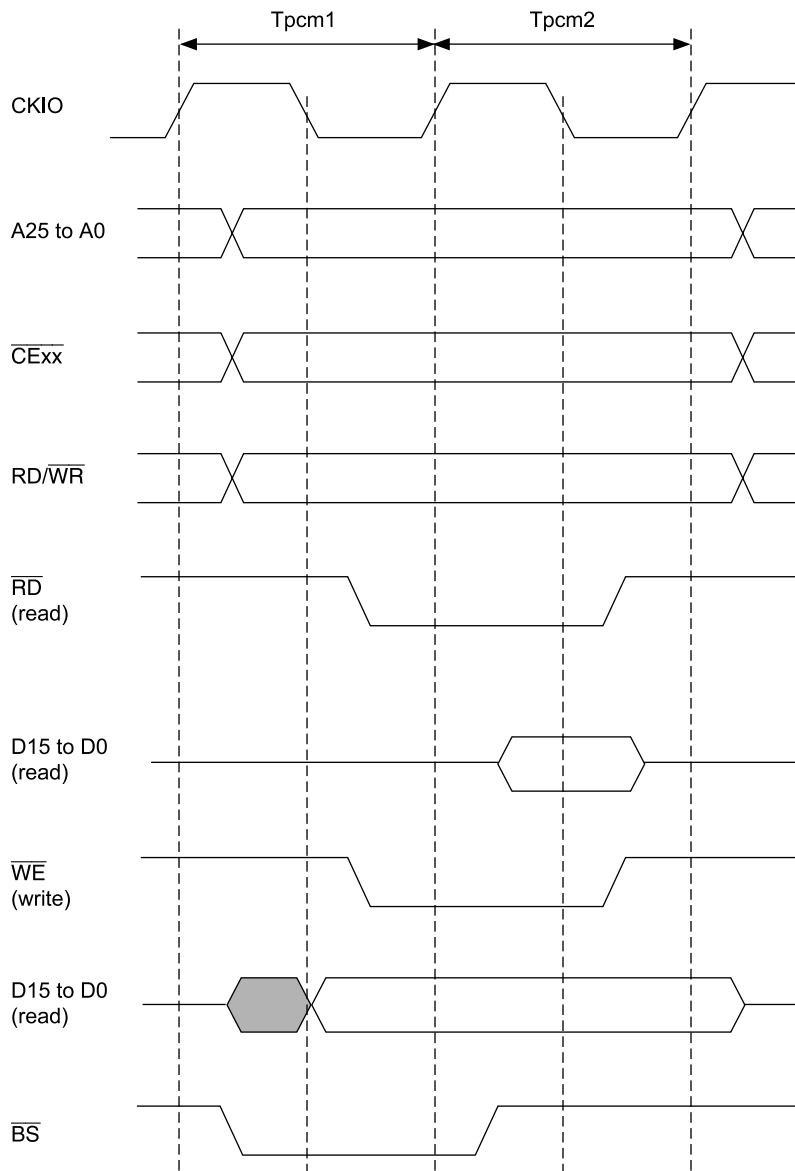
Figure 10.32 Basic Timing for PCMCIA Memory Card Interface
