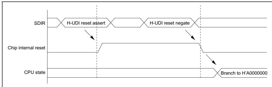
Figure 22.3 H-UDI Reset
