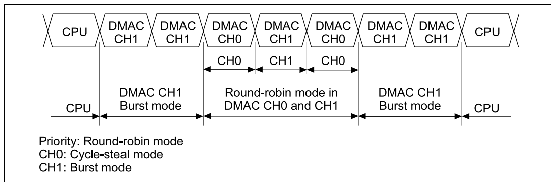
Figure 11.14 Bus State when Multiple Channels Are Operating
