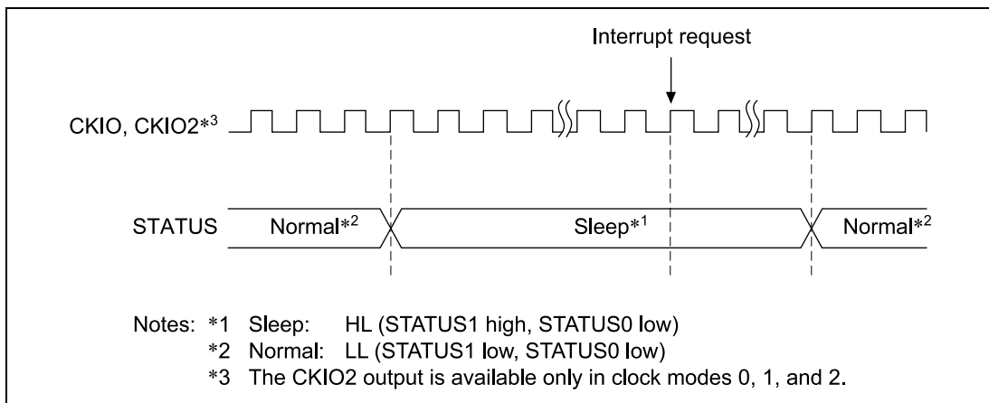
Figure 8.7 Sleep to Interrupt STATUS Output
