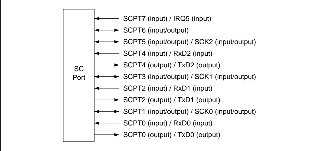
Figure 22.12 SC Port
