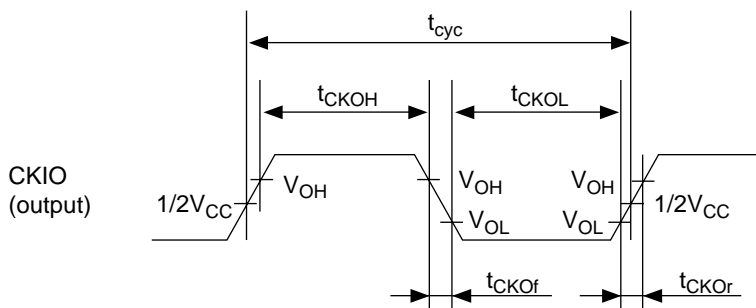
Figure 26.2 (2) CKIO Clock Output Timing
