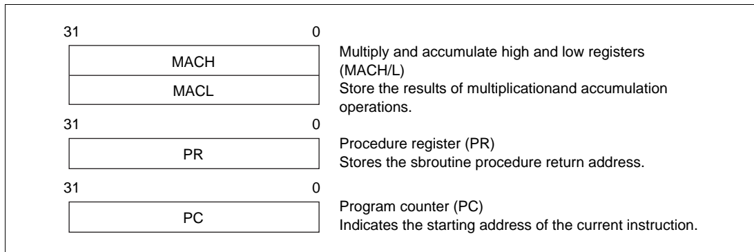
Figure 2.3 System Registers
