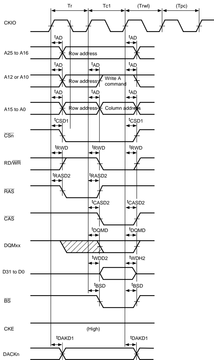
Figure 26.22 Synchronous DRAM Write Bus Cycle ( RCD = 0 , TPC = 0 , TRWL = 0 )
