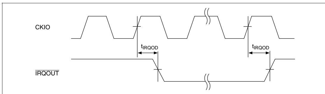
Figure 25.9 \overline{\text{IRQOUT}} Timing
