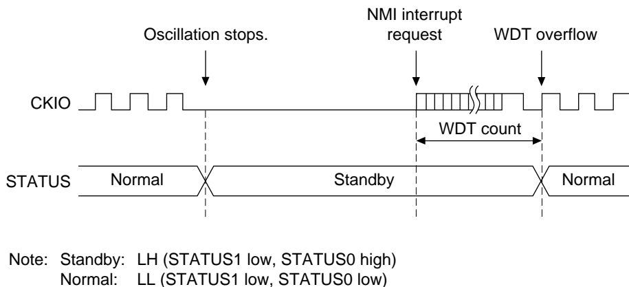
Figure 10.6 Standby to NMI Interrupt STATUS Output
