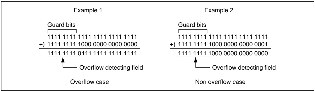
Figure 3.5 DC Bit Generation Examples in Overflow Mode
