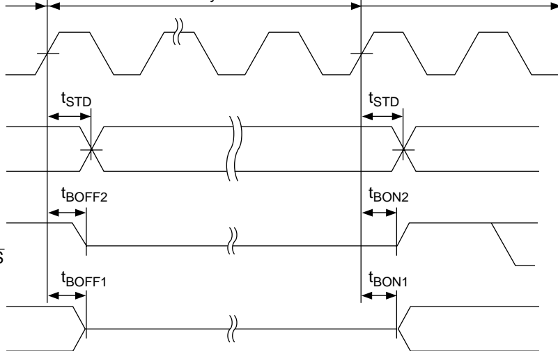
Figure 26.11 Pin Drive Timing at Standby
