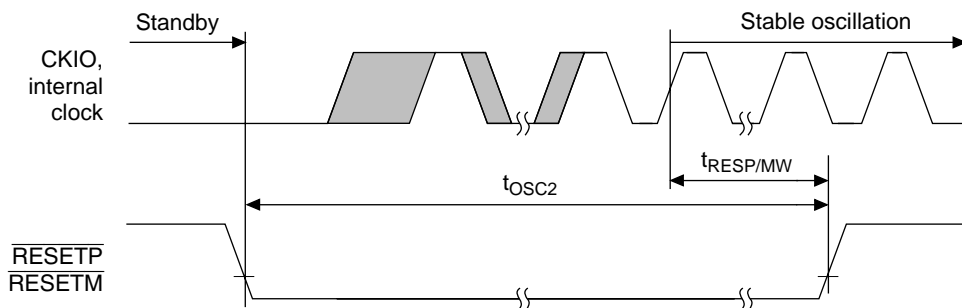
Figure 26.3 Power-on Oscillation Settling Time
