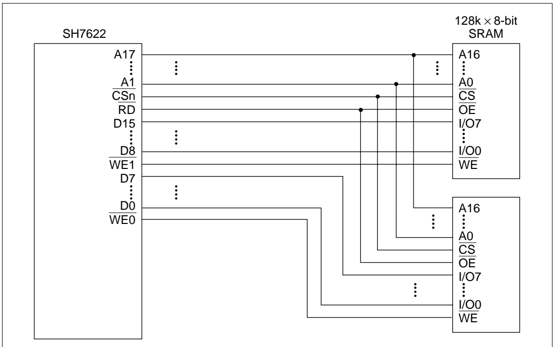
Figure 13.7 Example of 16-Bit Data-Width Static RAM Connection
