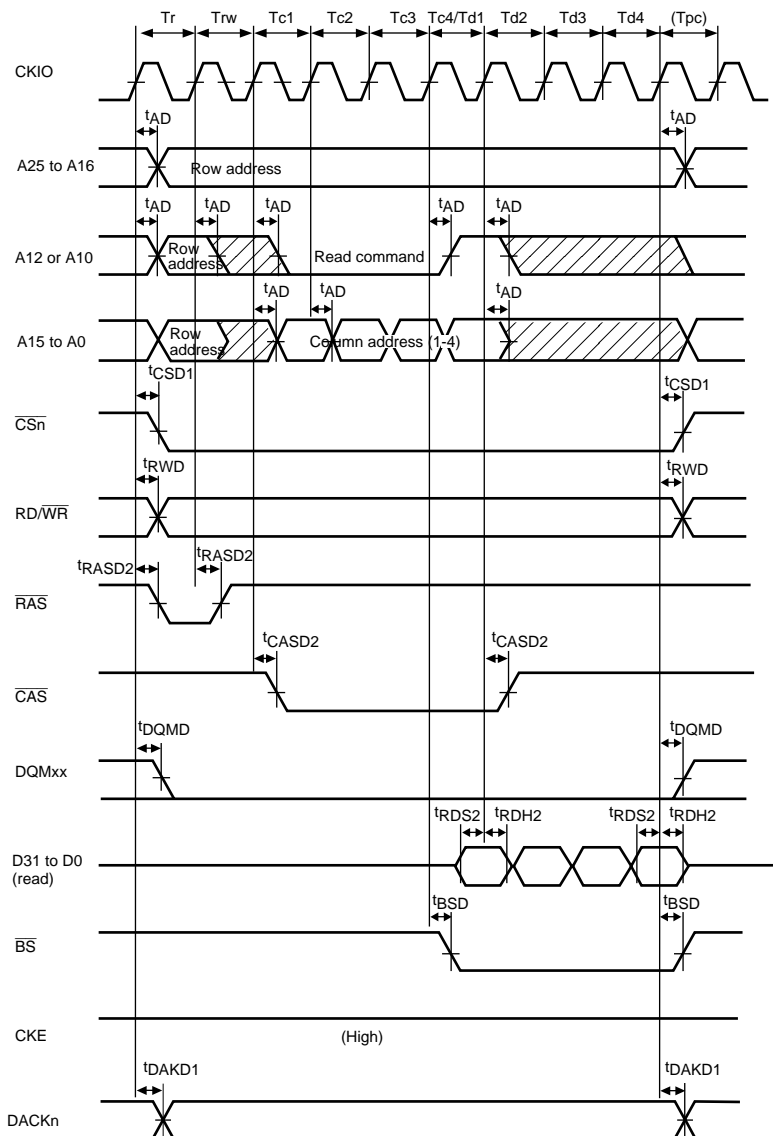
Figure 26.21 Synchronous DRAM Read Bus Cycle (Burst Read (Single Read × 4), RCD = 1, CAS Latency = 3, TPC = 0)
