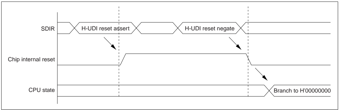
Figure 24.3 H-UDI Reset
