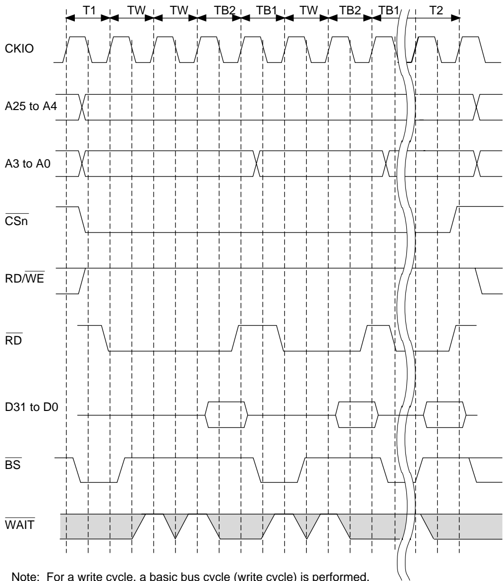
Figure 13.29 Burst ROM Wait Access Timing
