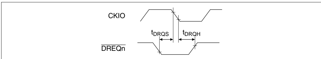
Figure 26.41 \overline{\text{DREQ}} Input Timing
