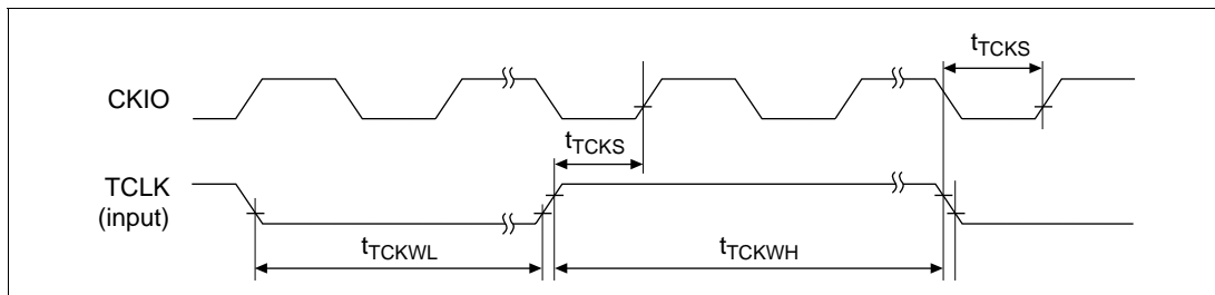
Figure 26.37 TCLK Clock Input Timing
