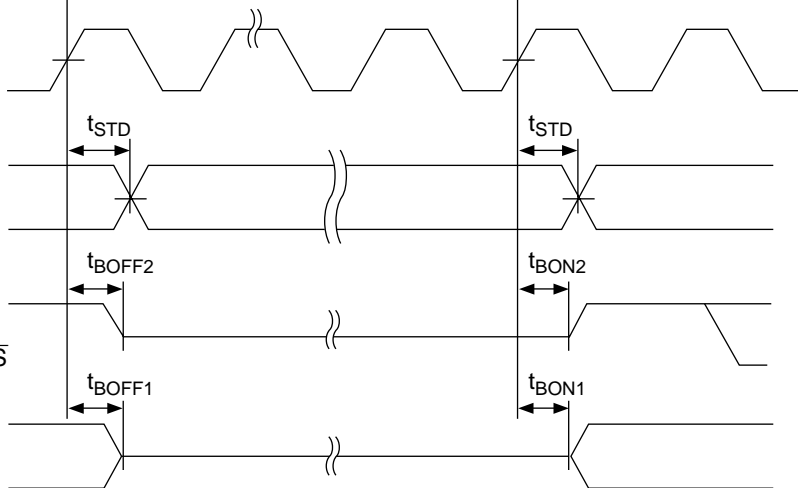
Figure 25.11 Pin Drive Timing at Standby
