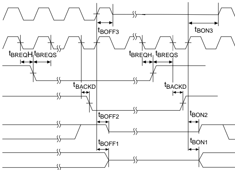
Figure 25.10 Bus Release Timing
