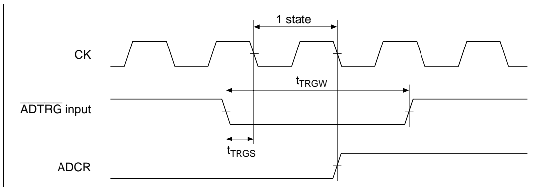
Figure 25.49 External Trigger Input Timing
