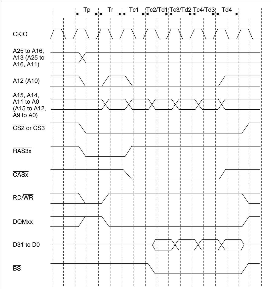
Figure 13.21 Burst Read Timing (Different Row Addresses)
