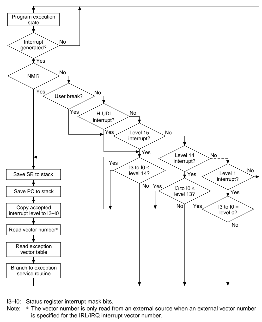
Figure 8.1 Interrupt Sequence Flowchart
