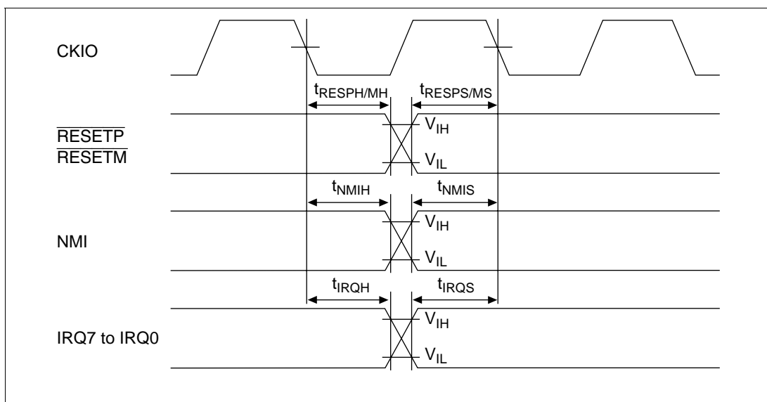
Figure 25.8 Interrupt Signal Input Timing
