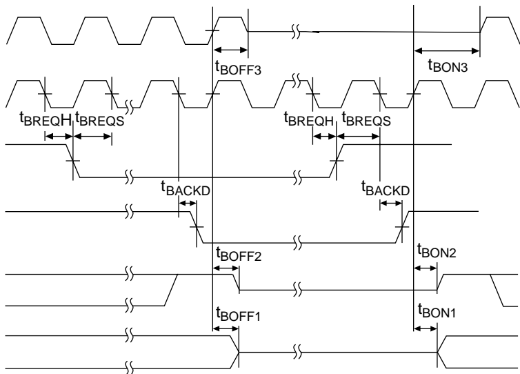
Figure 26.10 Bus Release Timing
