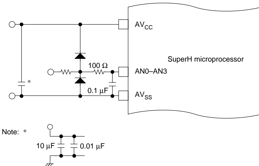
Figure 23.9 Example of Analog Input Protection Circuit
