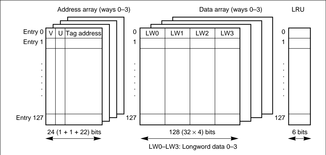
Figure 6.1 Cache Structure
