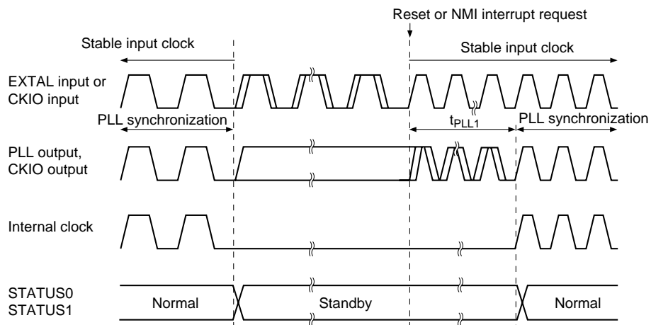
Figure 25.6 PLL Synchronization Settling Time by Reset or NMI
