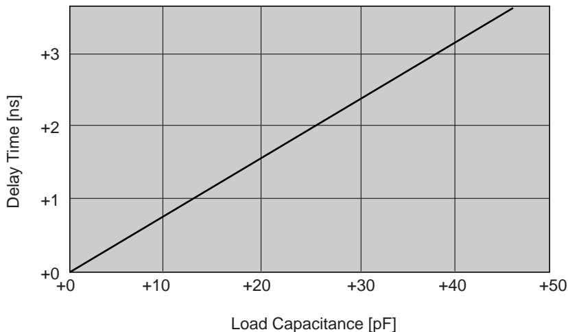
Figure 26.52 Load Capacitance vs. Delay Time
