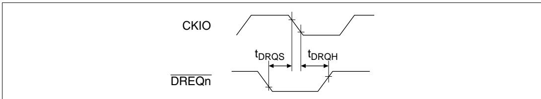
Figure 25.41 \overline{\text{DREQ}} Input Timing
