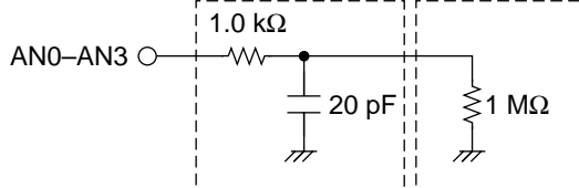
Figure 23.10 Analog Input Pin Equivalent Circuit (Reference Values)
