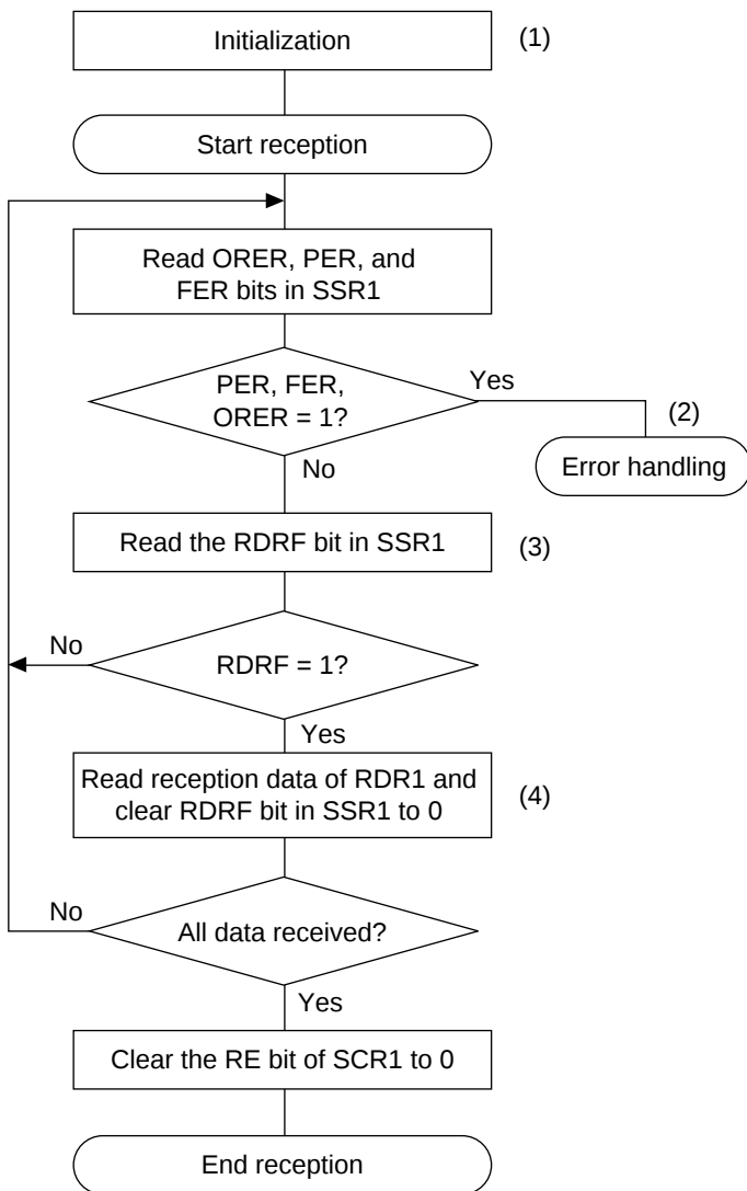
Figure 12.7 Sample Flowchart for Receiving Serial Data
