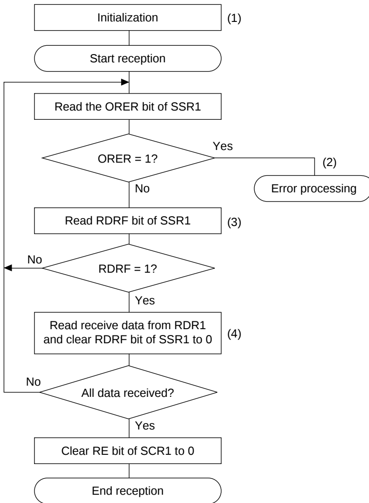
Figure 12.18 Sample Flowchart for Serial Receiving
