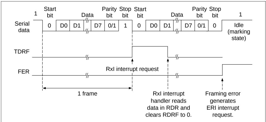
Figure 12.8 SCI1 Receive Operation (8-Bit Data with Parity and One Stop Bit)
