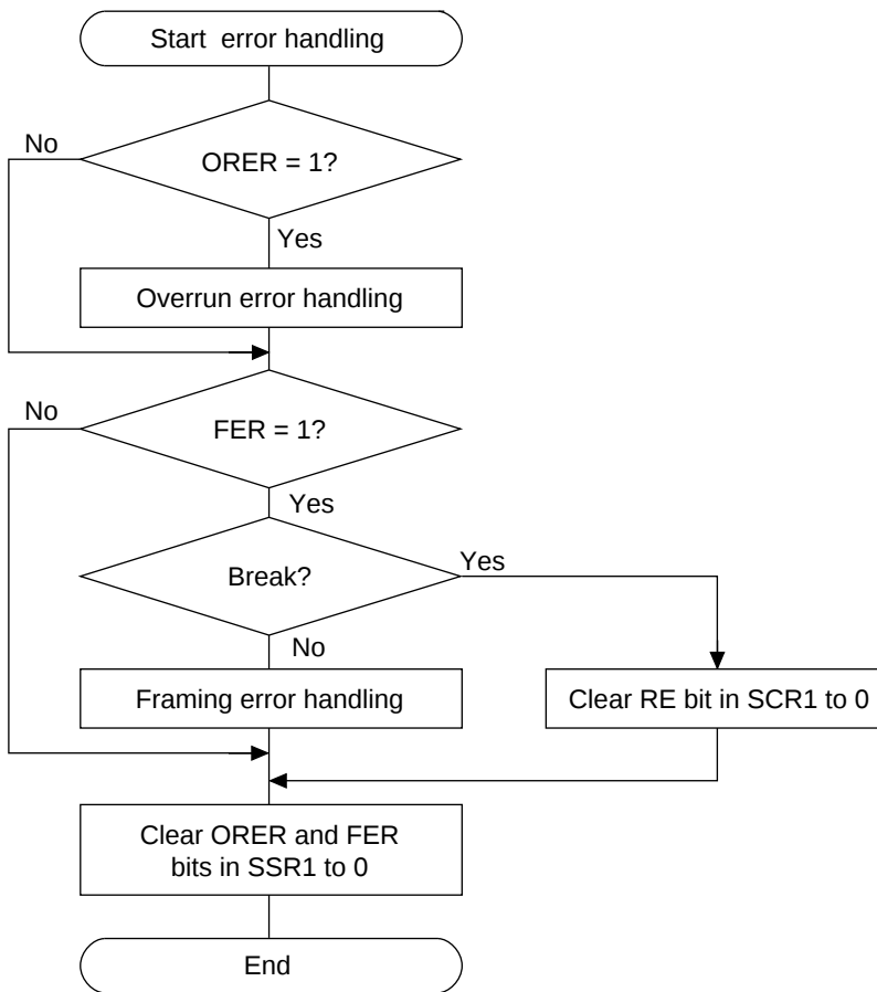
Figure 12.12 Sample Flowchart for Receiving Multiprocessor Serial Data (cont)
