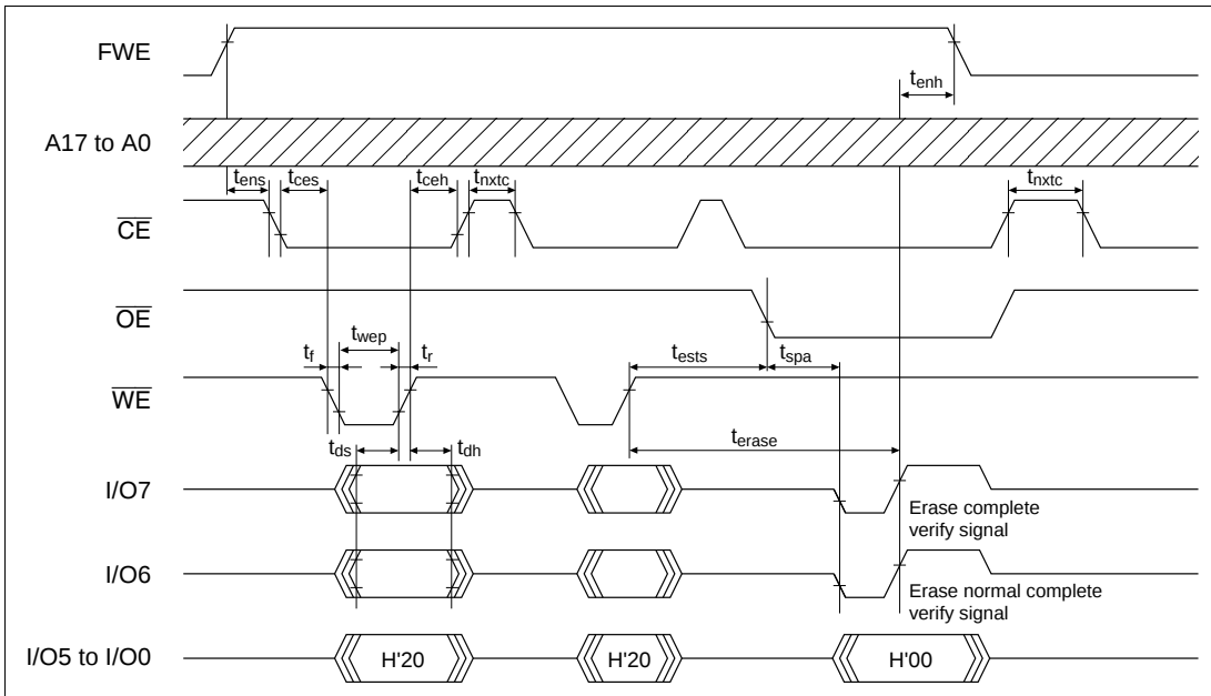
Figure 16.24 Auto-Erase Mode Timing Waveforms
