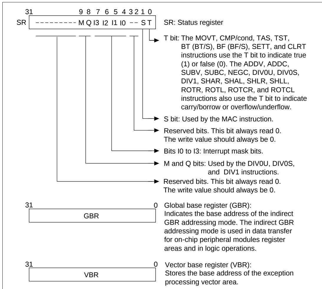
Figure 2.2 Control Registers
