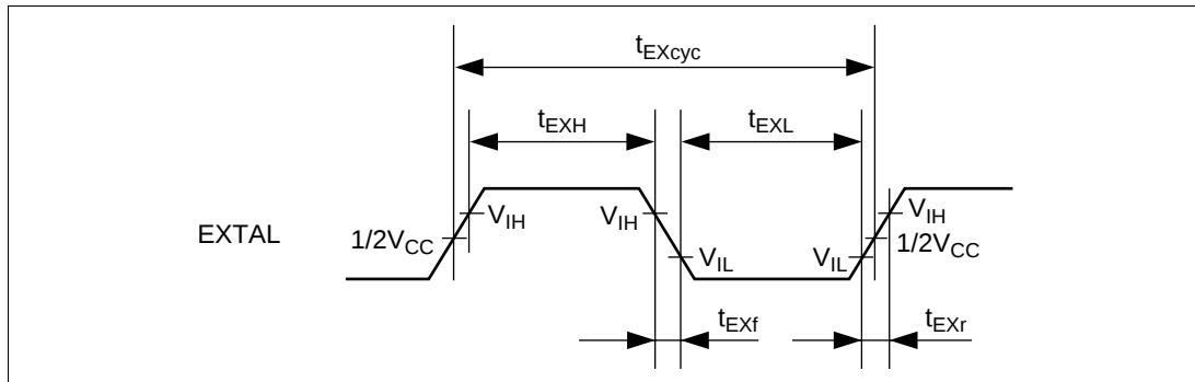
Figure 19.2 EXTAL Clock Input Timing
