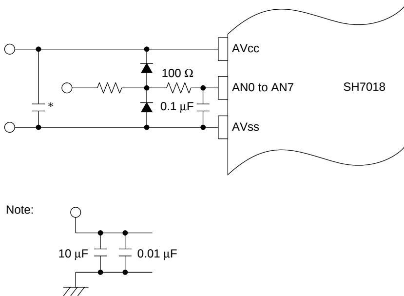
Figure 13.8 Example of Analog Input Pin Protection Circuit
