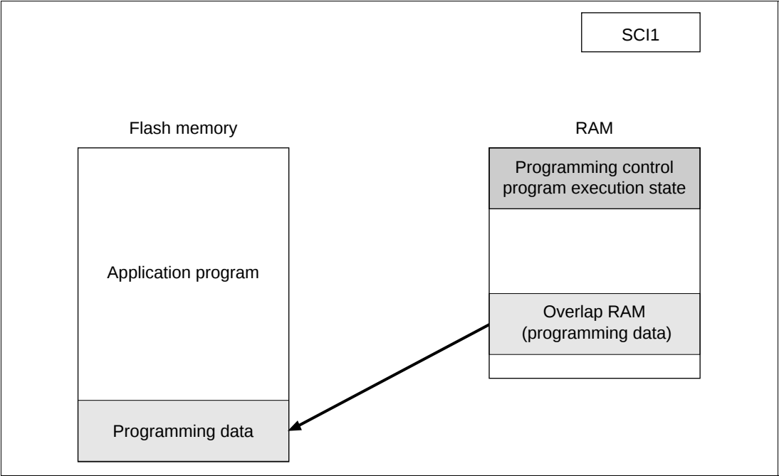
Figure 16.6 RAM Emulation (Flash Memory Overwrite)
