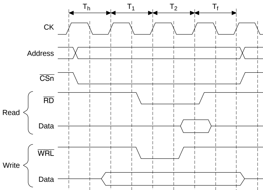
Figure 7.6 \overline{\text{CS}} Assert Period Extension Function
