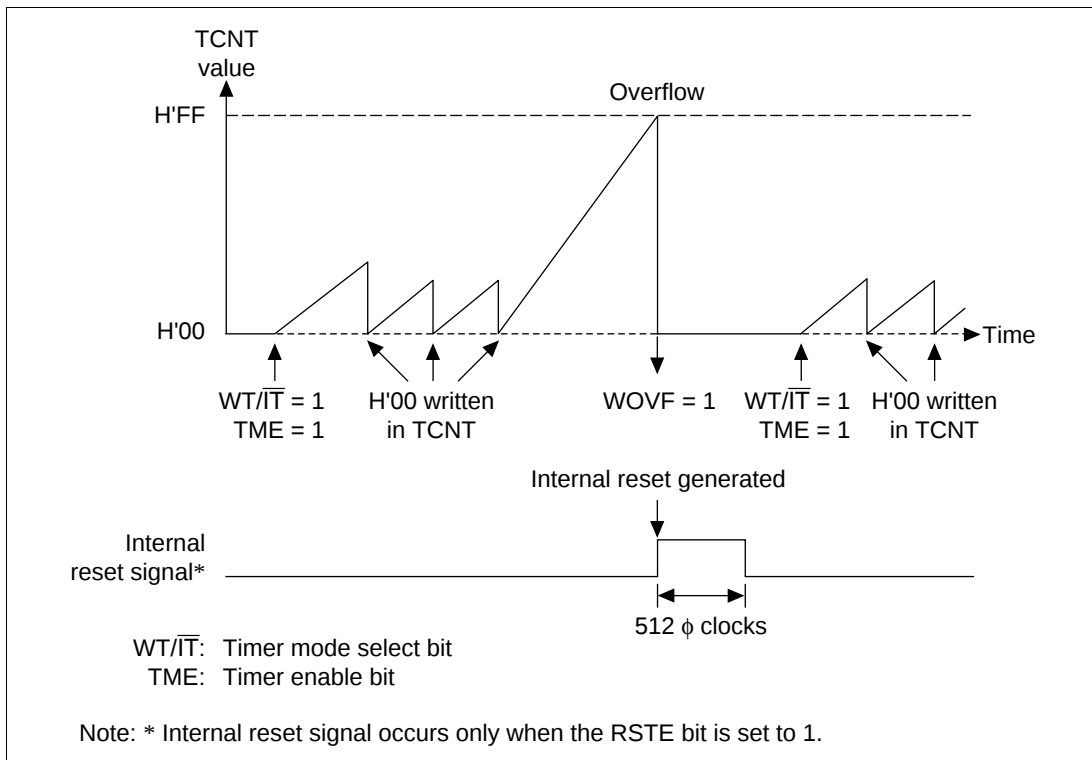
Figure 11.4 Operation in the Watchdog Timer Mode
