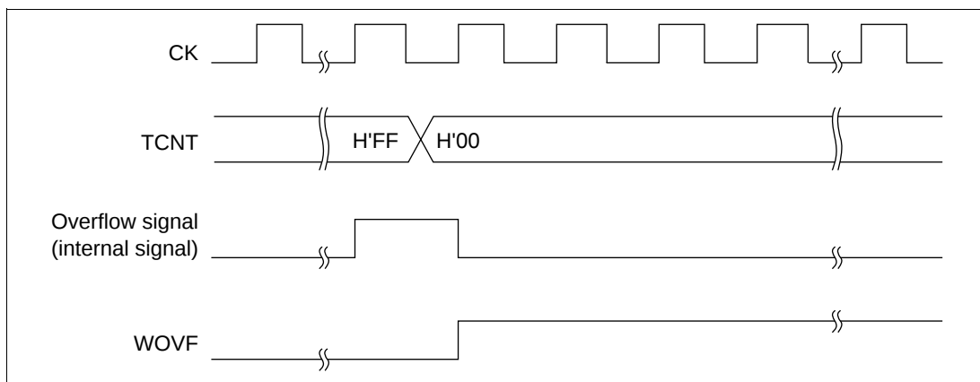
Figure 11.7 Timing of Setting the WOFV Bit
