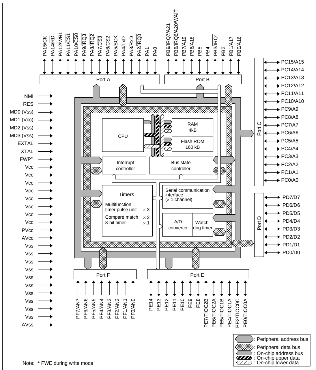
Figure 1.1 Block Diagram of SH7018 (TFP-100B Pins)
