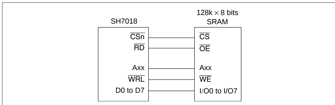
Figure 7.10 8-Bit Data Bus Width SRAM Connection
