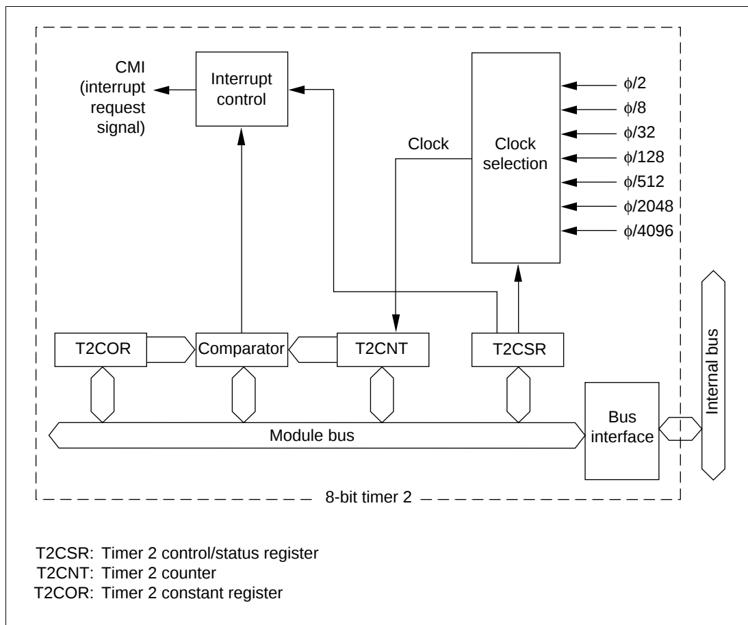
Figure 9.1 Block Diagram of 8-Bit Timer 2
