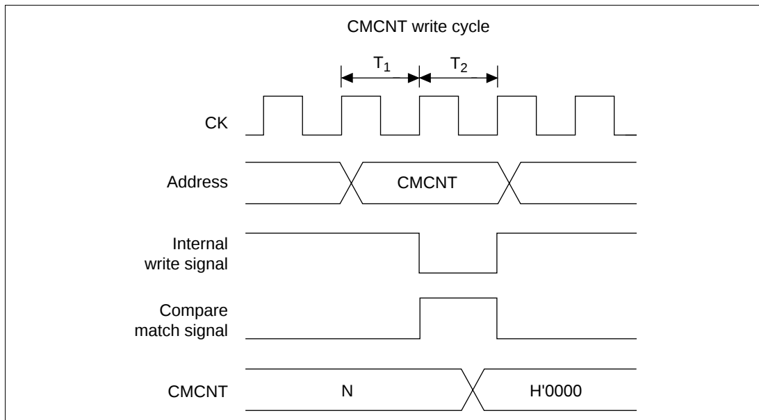
Figure 10.6 CMCNT Write and Compare Match Contention
