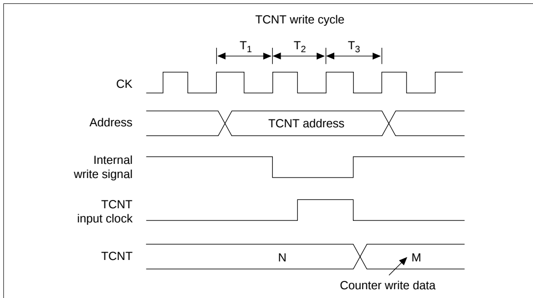
Figure 11.8 Contention between TCNT Write and Increment
