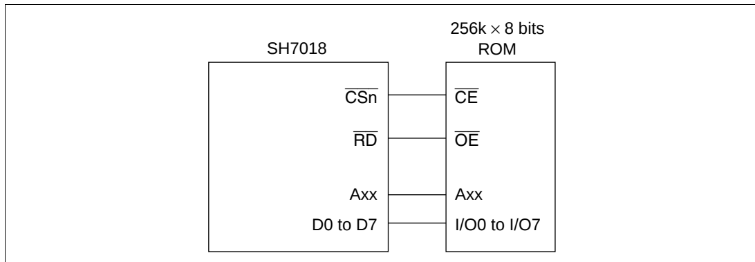
Figure 7.9 8-Bit Data Bus Width ROM Connection
