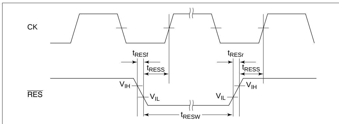
Figure 19.4 Reset Input Timing
