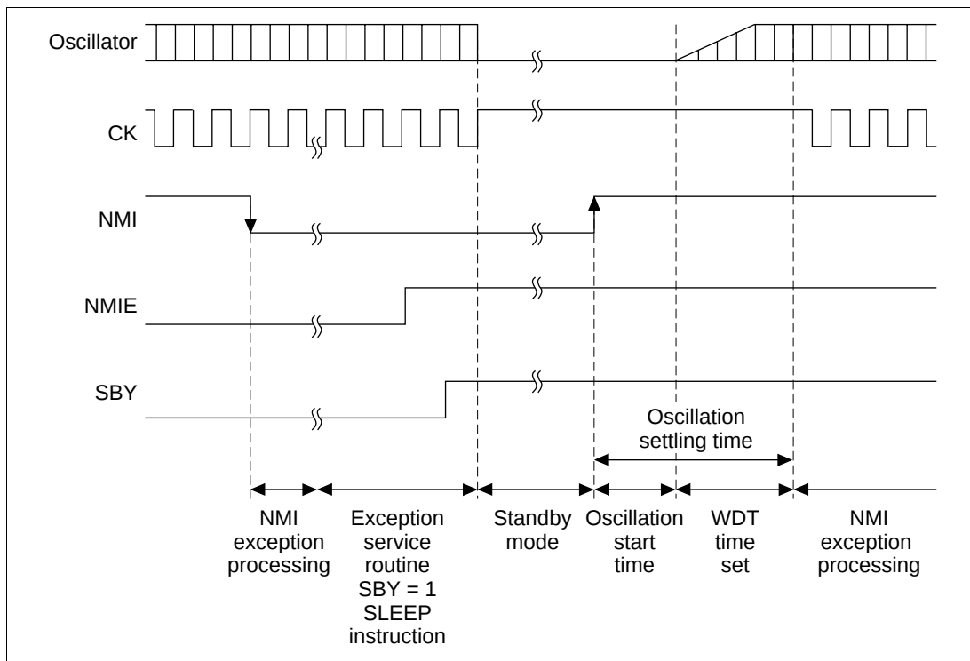
Figure 18.1 Standby Mode NMI Timing (Application Example)
