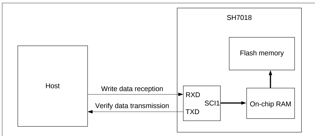
Figure 16.8 System Configuration in Boot Mode
