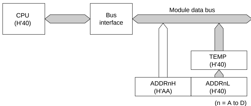
Figure 13.2 ADDR Access Operation (Reading H'AA40)
