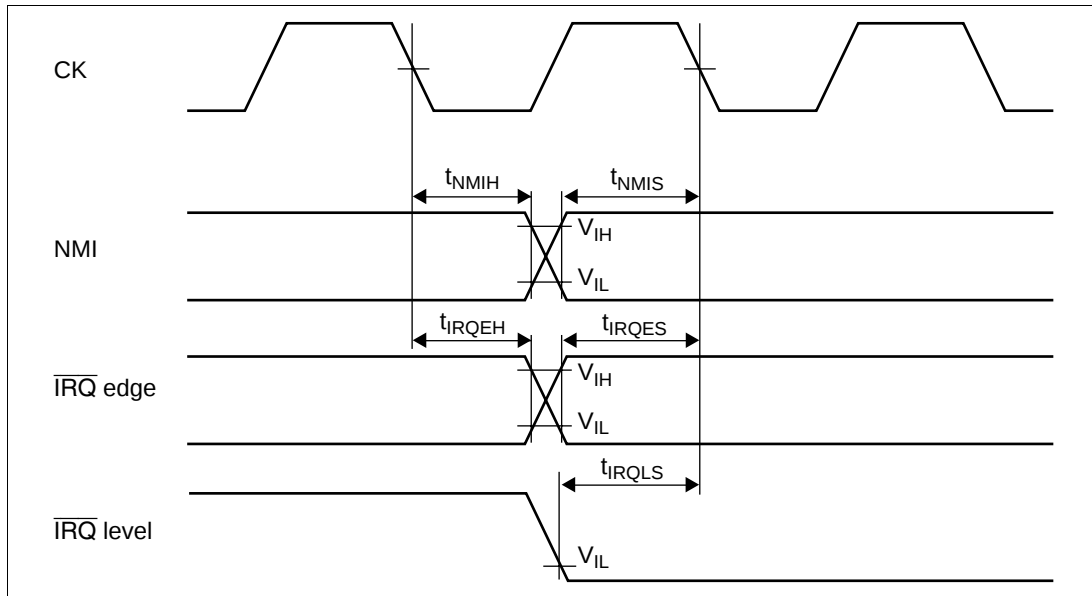
Figure 19.5 Interrupt Signal Input Timing
