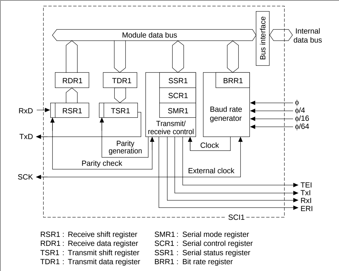
Figure 12.1 SCI1 Block Diagram
