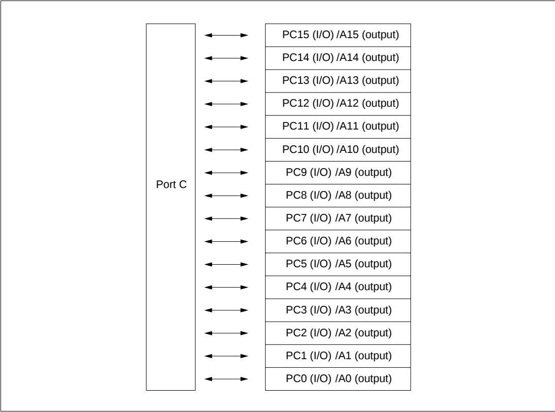
Figure 15.3 Port C
