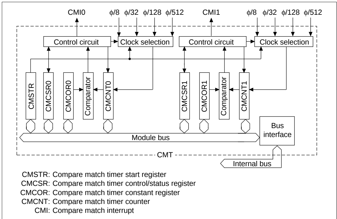
Figure 10.1 CMT Block Diagram
