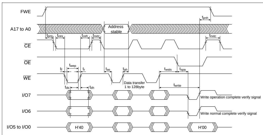
Figure 16.23 Auto-Program Mode Timing Waveforms
