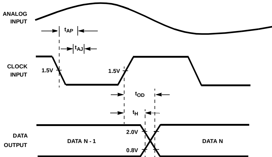
FIGURE 2. INPUT-TO-OUTPUT TIMING
