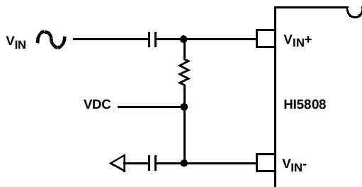
FIGURE 17. AC COUPLED SINGLE ENDED INPUT
