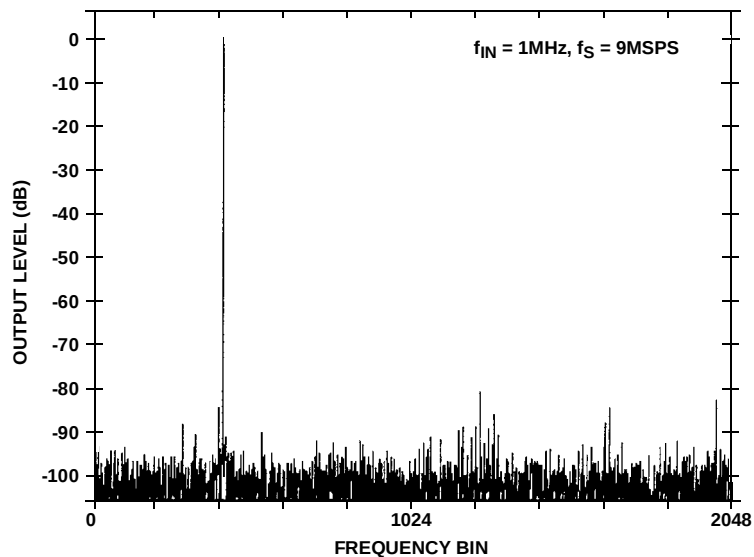
FIGURE 13. 4096 POINT FFT SPECTRAL PLOT
