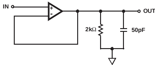
FIGURE 1. SLEW RATE AND TRANSIENT RESPONSE TEST CIRCUIT
