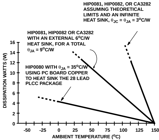
FIGURE 8. DISSIPATION DERATING CURVES SHOWING MAXIMUM DISSIPATION vs AMBIENT TEMPERATURE. THE SLOPE OF EACH CURVE IS THE RECIPROCAL OF THERMAL RESISTANCE FOR THE CONDITIONS NOTED AND THE SAFE OPERATING AREA FOR EACH CURVE IS BELOW THE LINE
