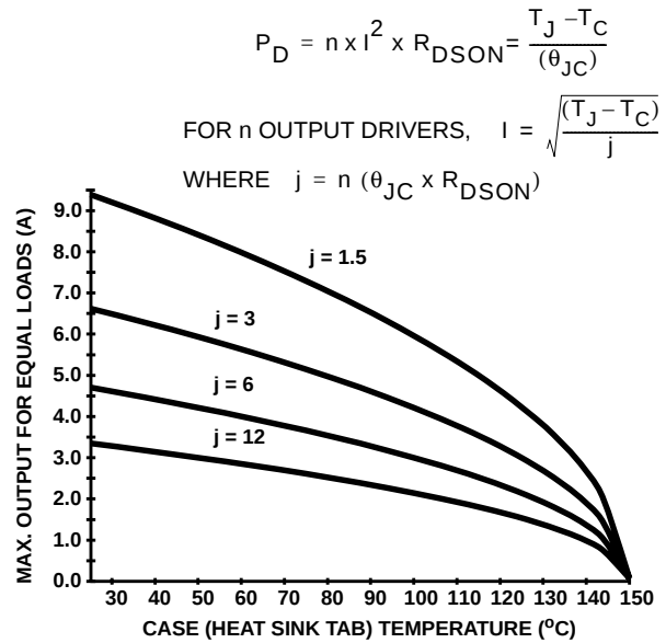
FIGURE 9. GENERAL GRAPH SOLUTION FOR MAXIMUM OUTPUT DRIVER CURRENT, I vs CASE TEMPERATURE, T_C GIVEN EQUAL LOAD CURRENTS AND A MAXIMUM JUNCTION TEMPERATURE, T_J = 150^\circ\text{C}
