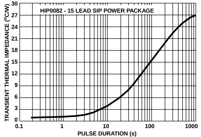
FIGURE 6B. TYPICAL CHARACTERISTIC PLOT OF THE TRANSIENT THERMAL IMPEDANCE FOR A SINGLE PULSE VERSUS PULSE DURATION FOR THE HIP0082 QUAD LOW SIDE POWER DRIVER
