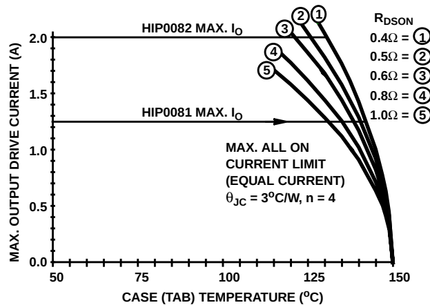
FIGURE 10. HIP0081 AND HIP0082 MAXIMUM CURRENT vs CASE TEMPERATURE. ALL 4 OUTPUTS ON WITH EQUAL CURRENT. Solving for current, I gives: I = \sqrt{\frac{(T_J - T_C)}{n \theta_{JC} R_{DS(ON)}}} \quad (\text{EQ. 15}) The number of output drivers ON and conducting may be from n = 1 to 4 for quad drivers such as the HIP0081 and HIP0082 or n = 1 to 8 for an octal driver such as the CA3282. Maximum temperature, dissipation and current ratings must be observed. For n equal conducting output drivers, we can now plot the maximum rated current, I vs the maximum case temperature, T_C . The denominator term in the radical of Equation 15, n \theta_{JC} R_{DS(ON)} , is used to plot a set of normalized curves, as shown in Figure 9. Using the HIP0081 and HIP0082 as examples, Figure 10 illustrates the boundaries for temperature and current for a range of R_{DS(ON)} with all four outputs ON and equal output HIP0082 OUTPUTS 3, 4 R_{DS(ON)} 0.57\Omega AT 2A (5A OUTPUTS) HIP0082 OUTPUTS 1, 2 R_{DS(ON)} 0.62\Omega AT 2A (2A OUTPUTS) HIP0081 OUTPUTS 1 - 4 R_{DS(ON)} 0.5\Omega AT 1A (EA. OUTPUT) HIP0081 OUTPUTS 1 - 4 R_{DS(ON)} 1.0\Omega AT 1A (LOW V_{CC} OPERATION)
