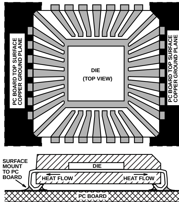
FIGURE 4. THE HIP0080 PLCC PACKAGE ILLUSTRATING THE COPPER LEAD FRAME CONSTRUCTION DESIGNED TO CONDUCT HEAT TO THE GROUND LEADS
