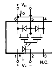
CONNECTION B dc CONNECTION
