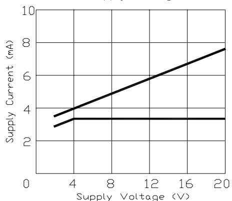
Fig. 1 Supply Current V.S. Supply Voltage
