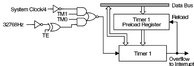
Timer 1
