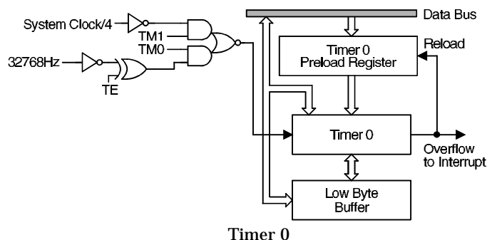
Timer 0
