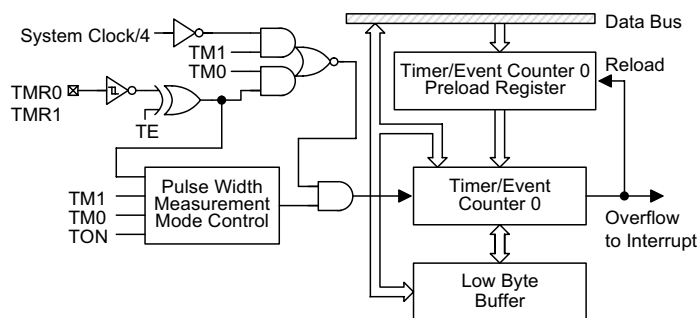
Timer/event counter0/1
