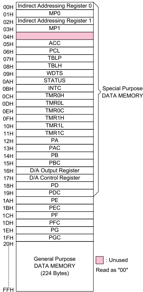
RAM mapping
