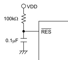
Reset circuit
