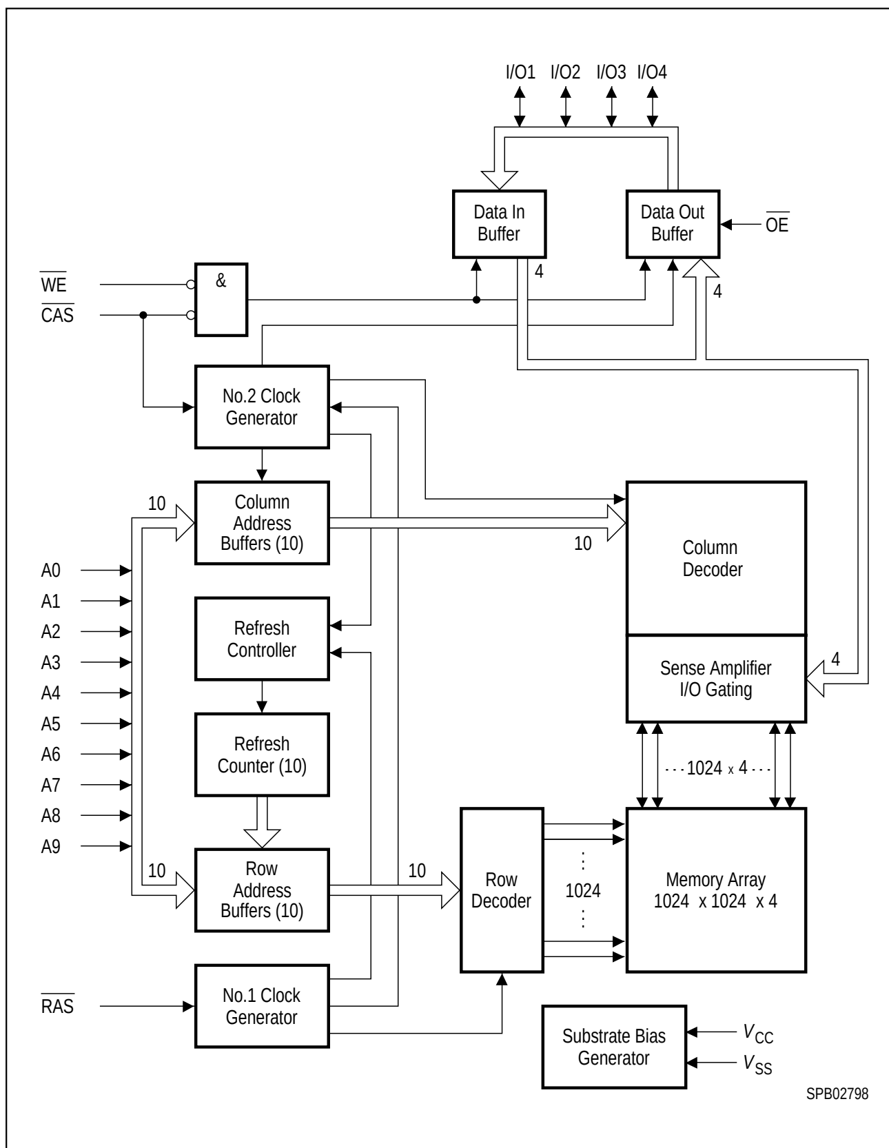
Block Diagram
