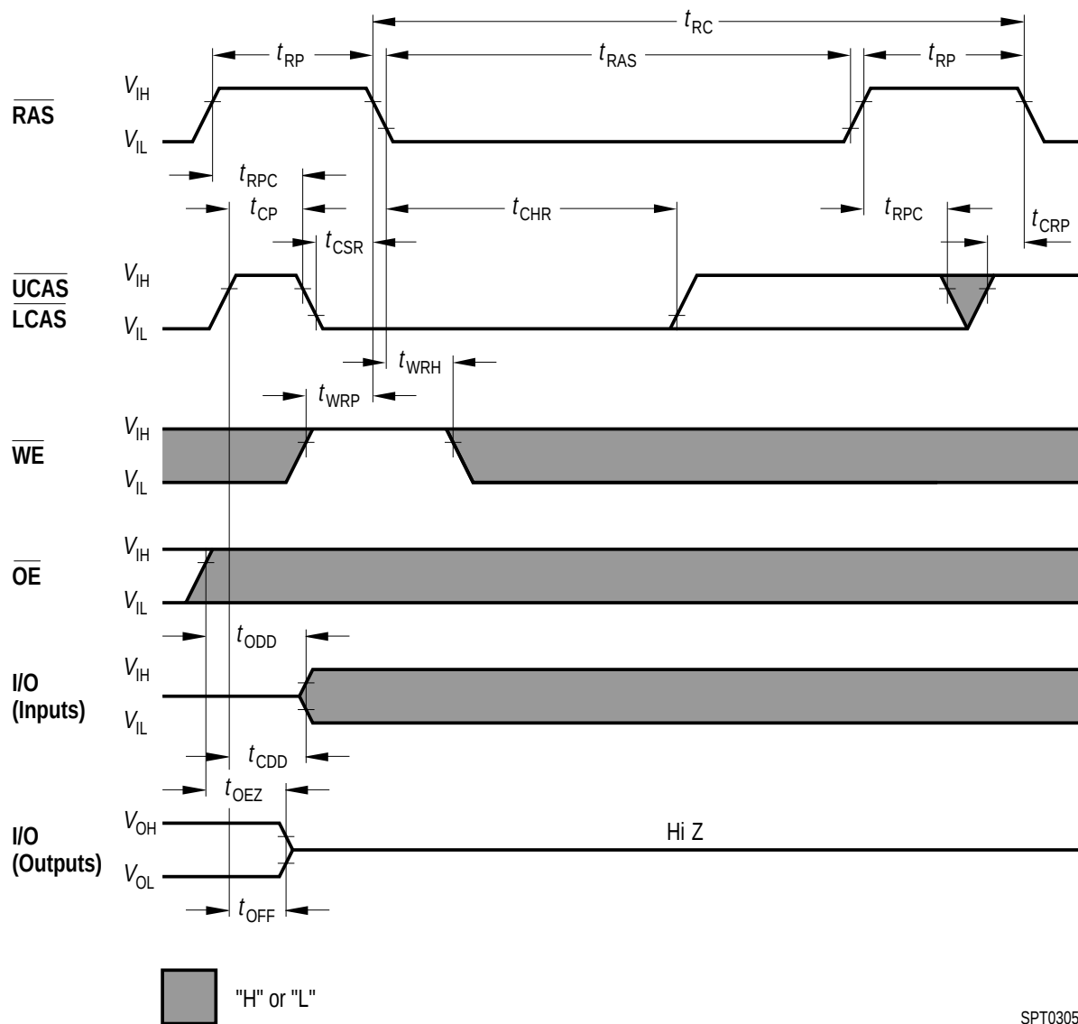
CAS-before-RAS Refresh Cycle
