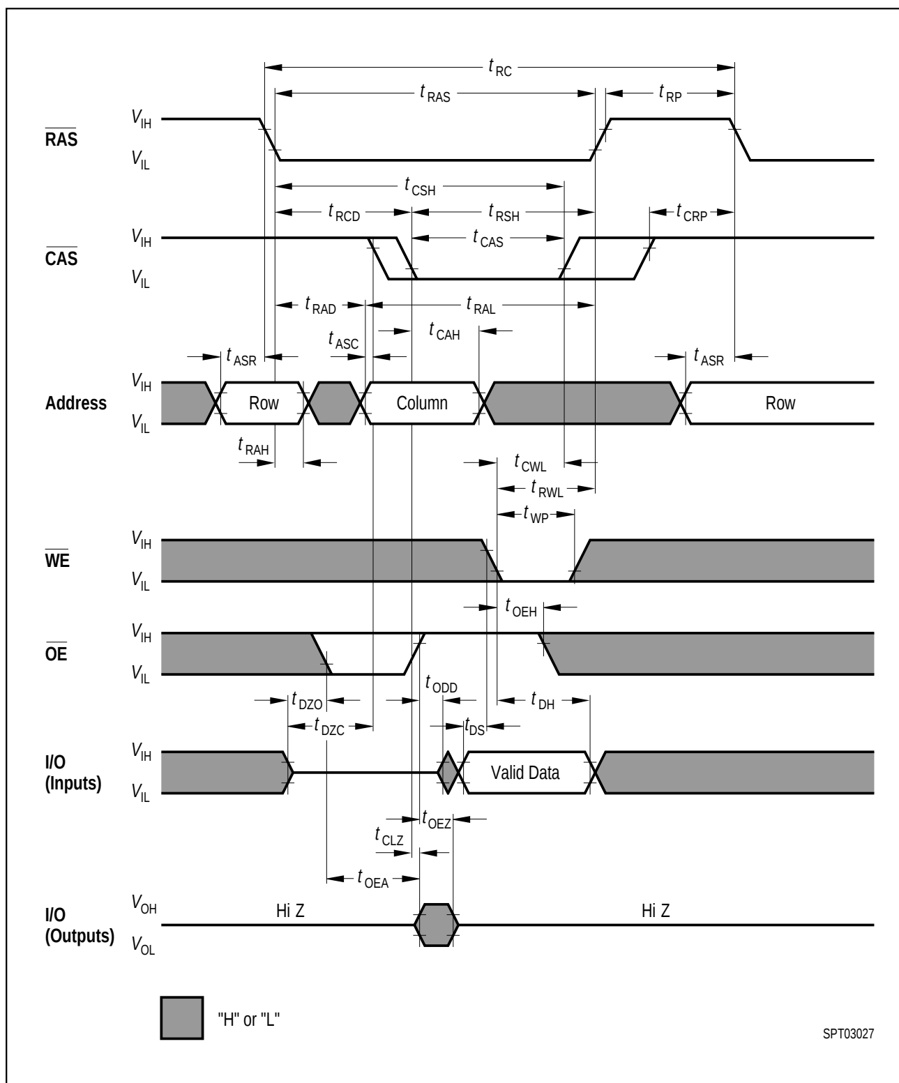
Write Cycle ( \overline{\text{OE}} Controlled Write)
