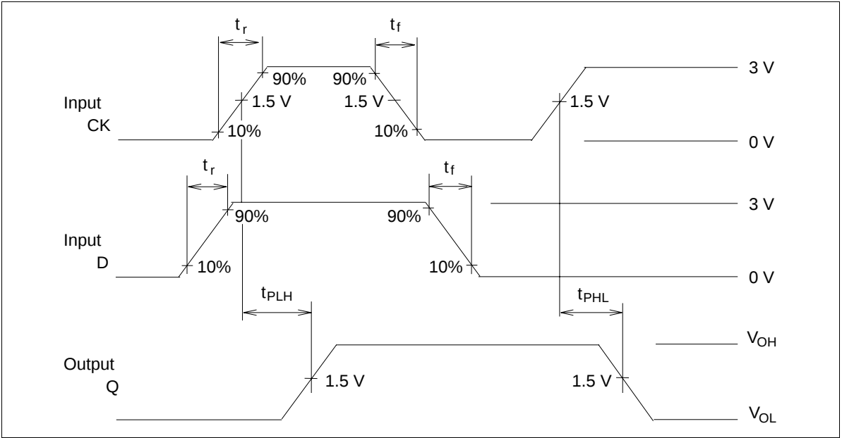
Waveforms-2
