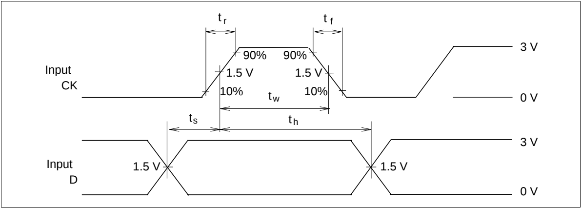
Waveforms-2
