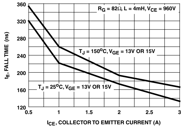
FIGURE 12. TURN-OFF FALL TIME vs COLLECTOR TO EMITTER CURRENT
