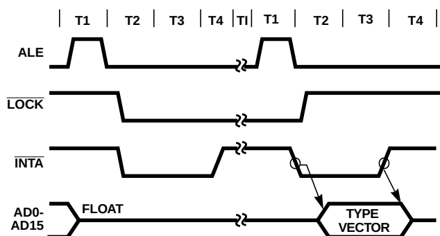
FIGURE 13. INTERRUPT ACKNOWLEDGE SEQUENCE
