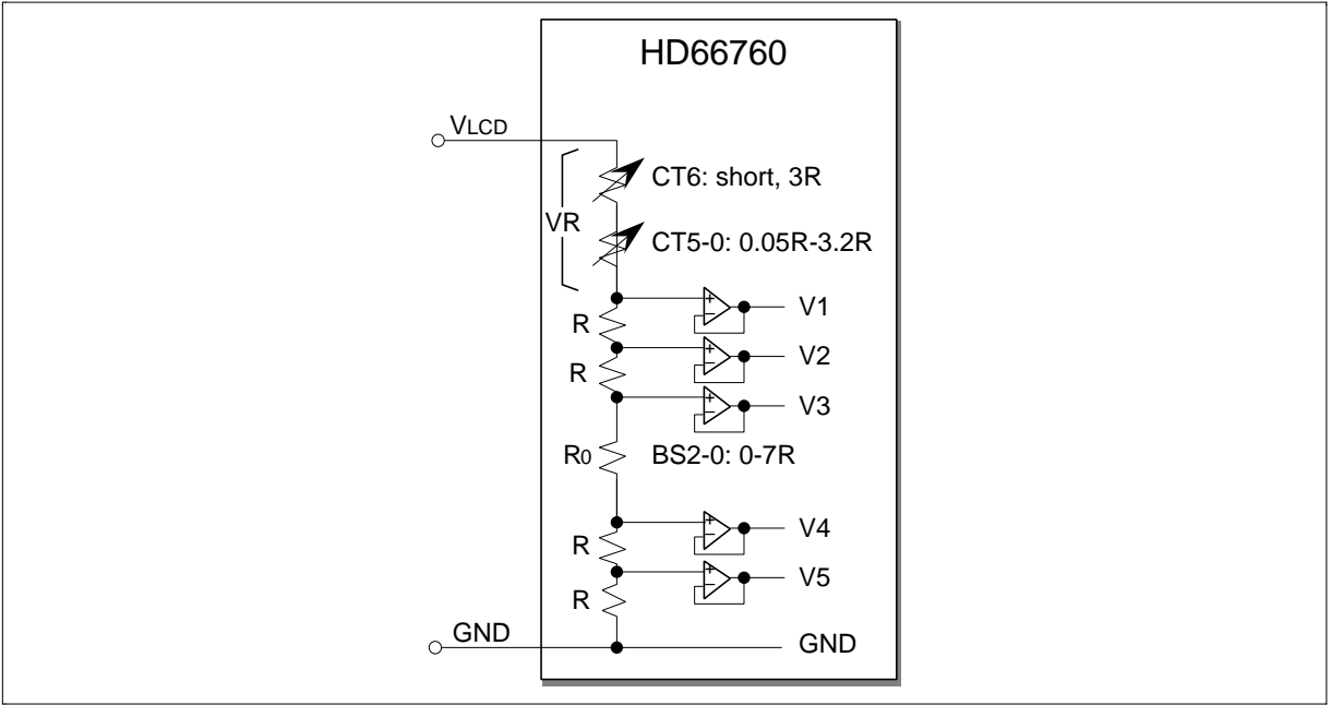
Figure 8 Contrast Adjuster
