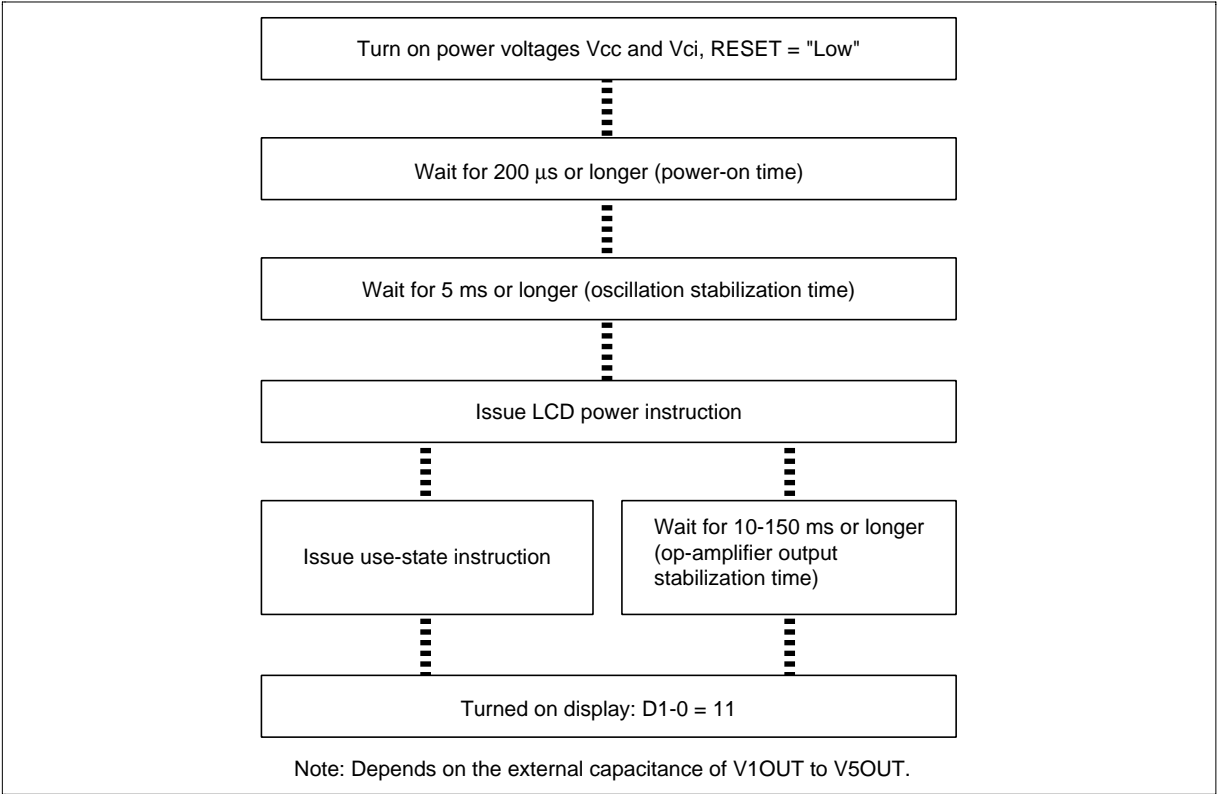
Figure 56 Power-on Sequence
