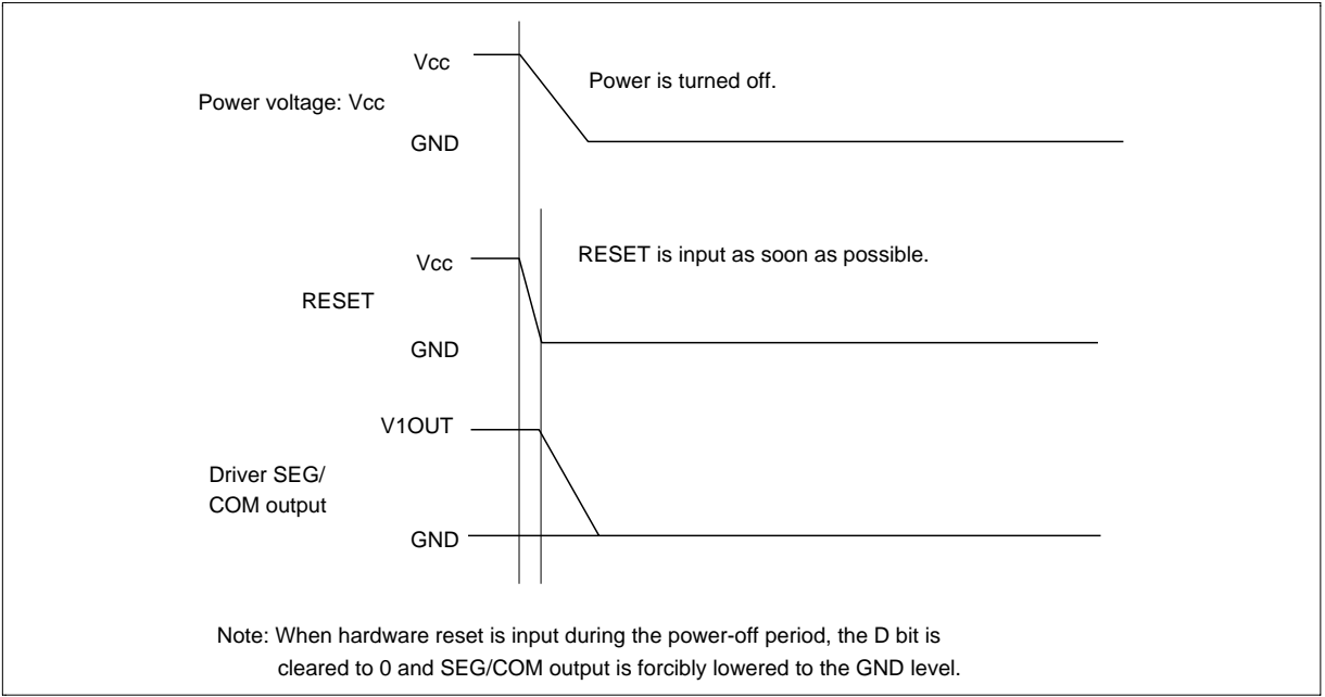
Figure 59 Power-off Timing
