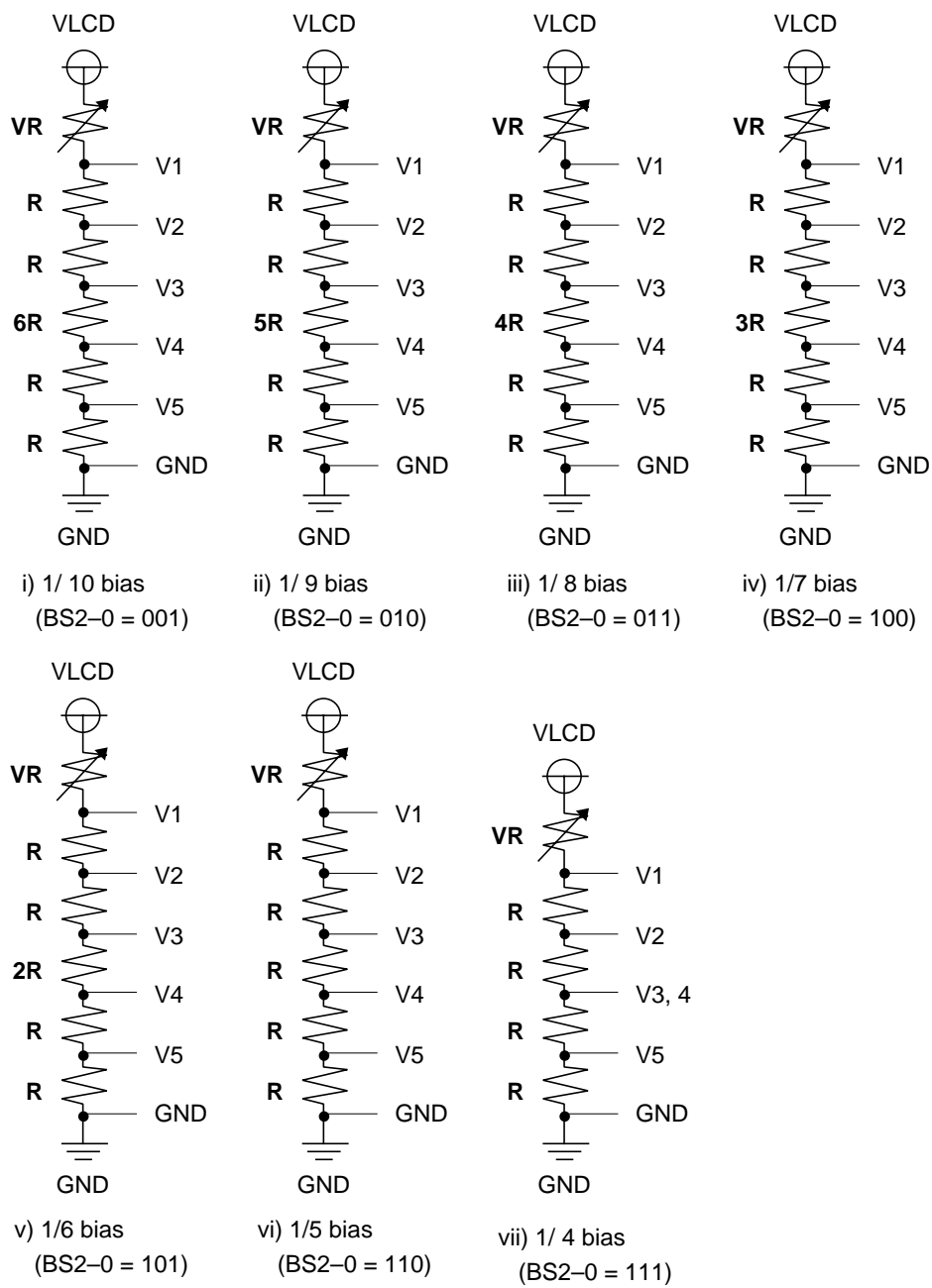
Figure 48 Liquid Crystal Display Drive Bias Circuit
