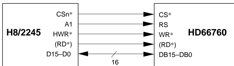
Figure 26 Interface to 16-bit Microcomputer
