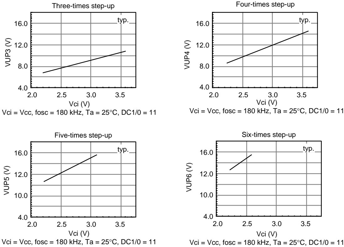
Figure 65 Step-up
