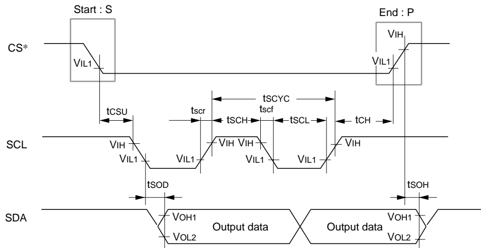
Figure 71 Clock Synchronized Serial Interface Output Timing
