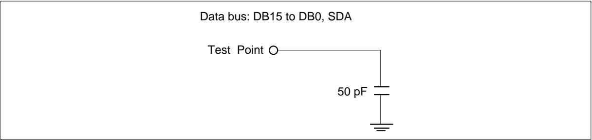
Figure 66 Load Circuit
