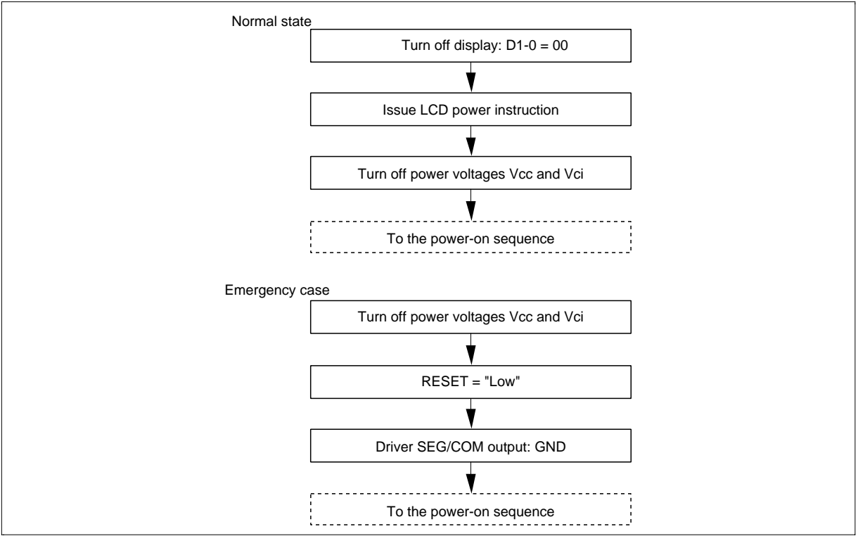
Figure 58 Power-off Sequence
