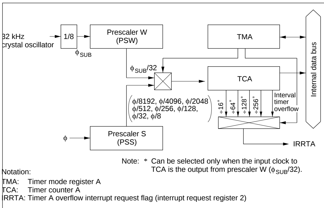
Figure 8-2 Block Diagram
