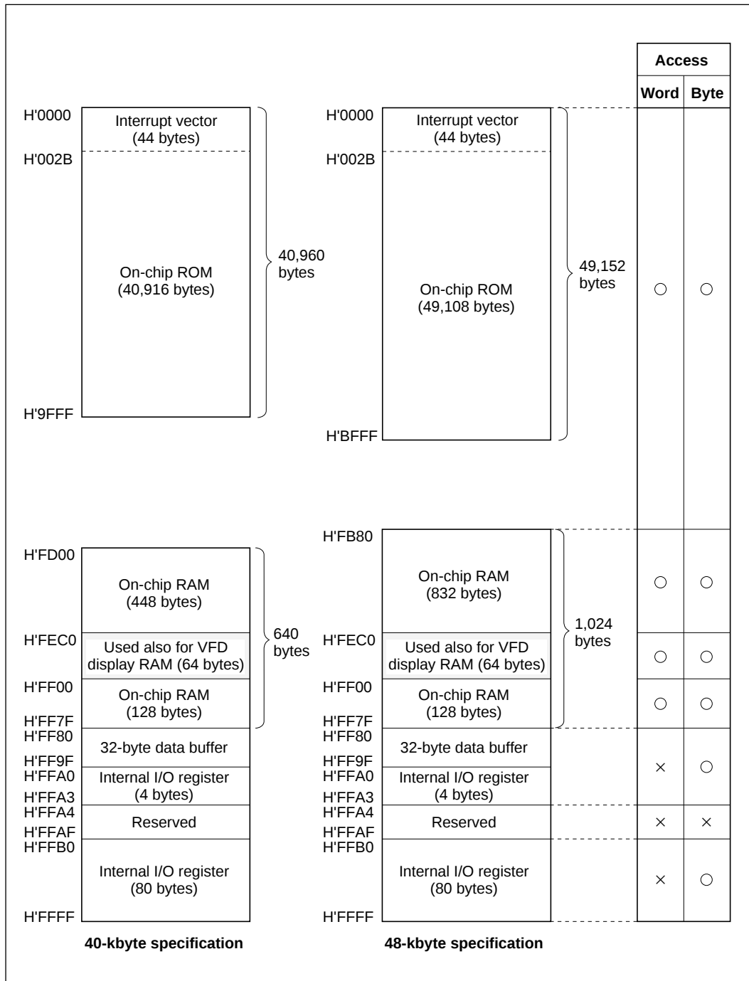
Figure 2-16 Data Size for Access to and from On-Chip Peripheral Modules (2)
