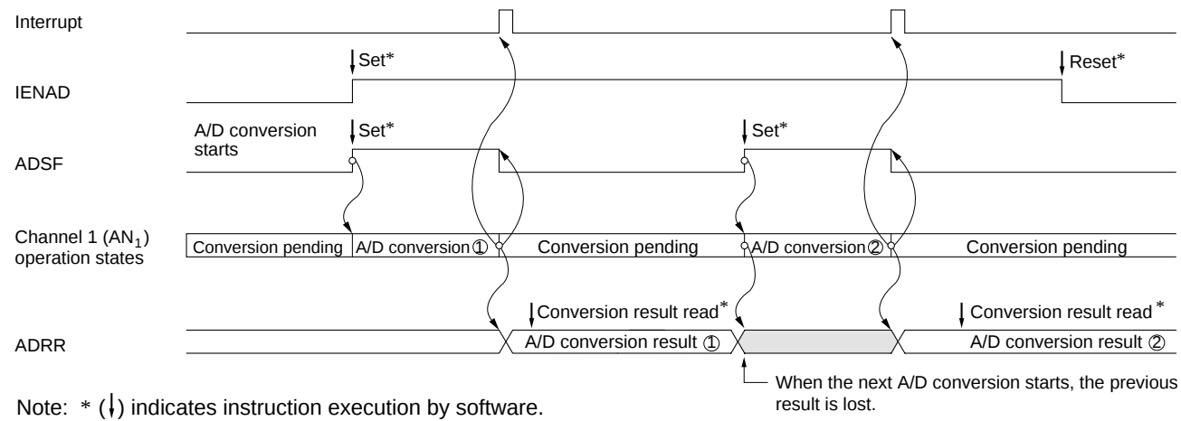
Figure 13-3 Typical A/D Converter Operation Timing
