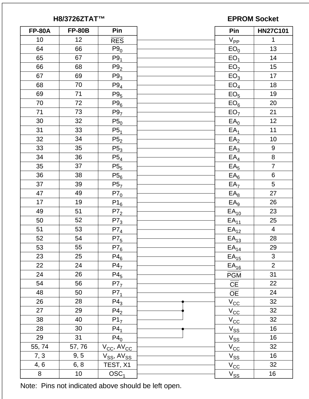
Figure 4-2 Socket Adapter Pin Correspondence (2)
