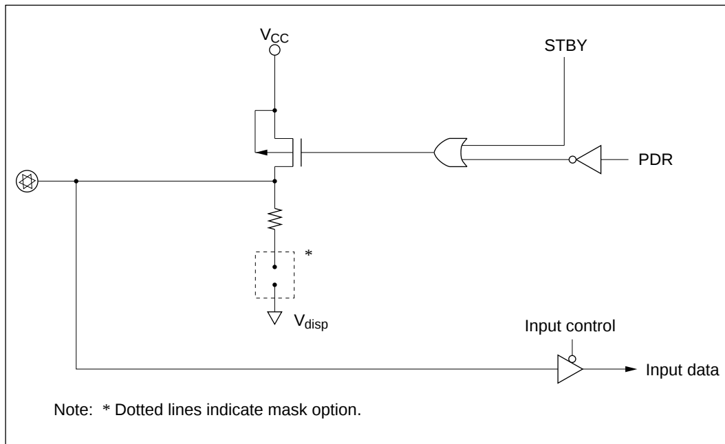
Figure 7-2 Pull-down MOS Circuit Configuration
