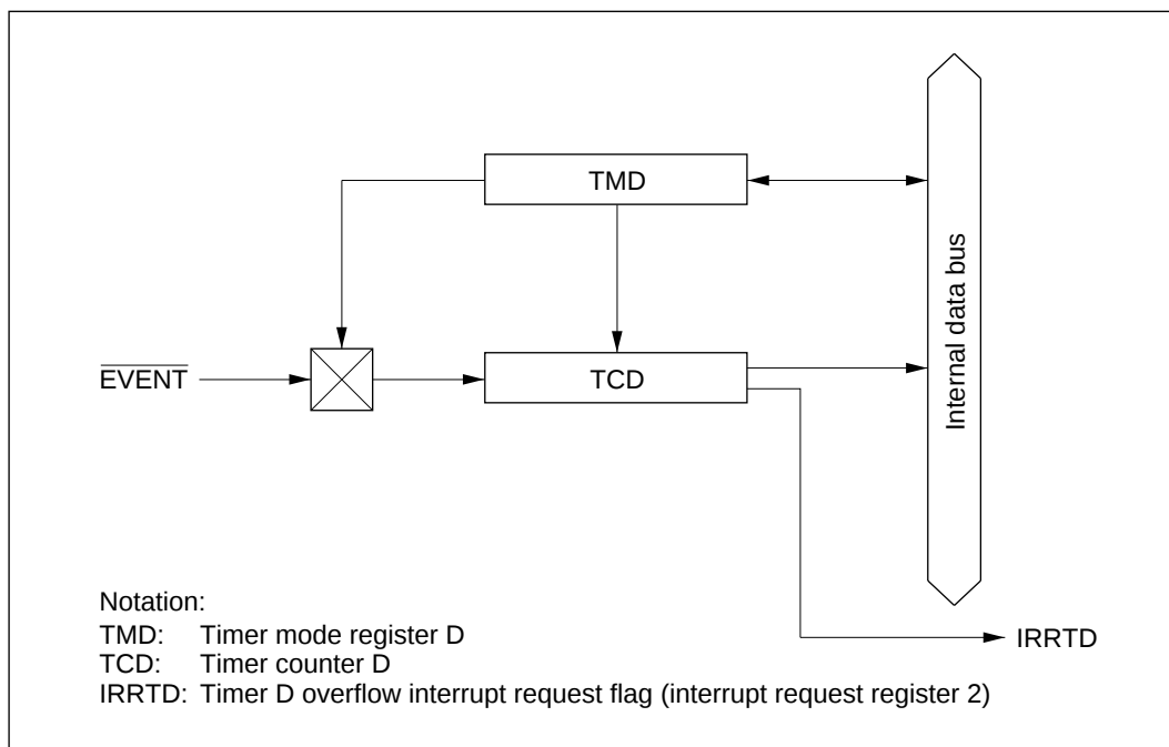
Figure 8-5 Block Diagram
