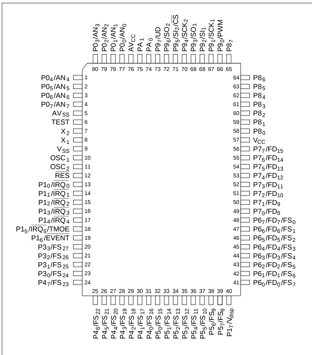
Figure 1-3 Pin Arrangement (FP-80B: Top view)
