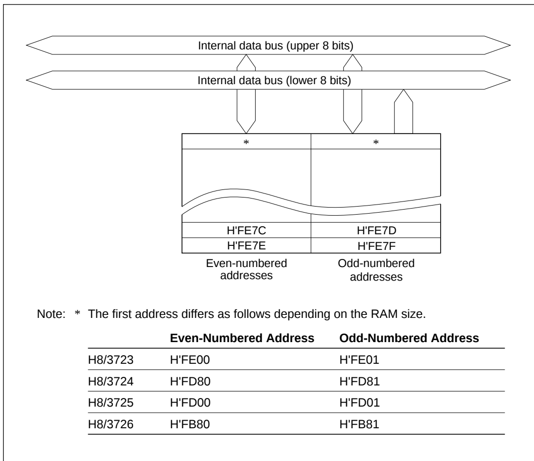
Figure 5-1 RAM Block Diagram
