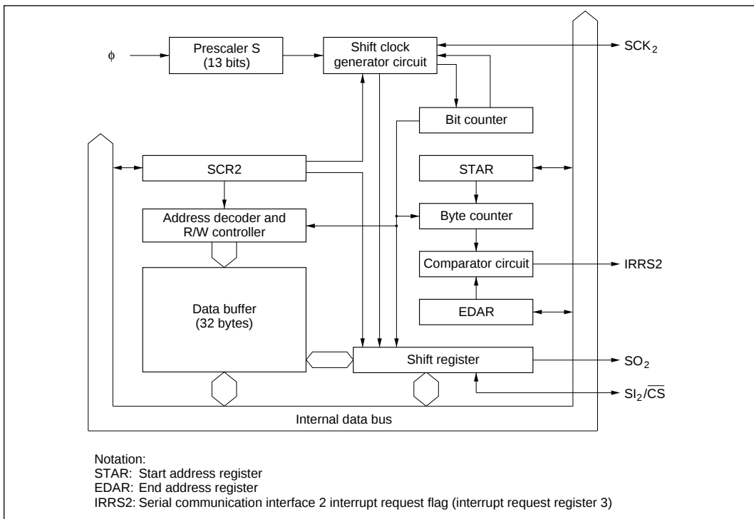
Figure 11-1 Block Diagram
