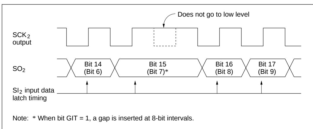
Figure 11-4 Gap Insertion for 1 Clock Cycle (bits GAP2-GAP1 = 01)
