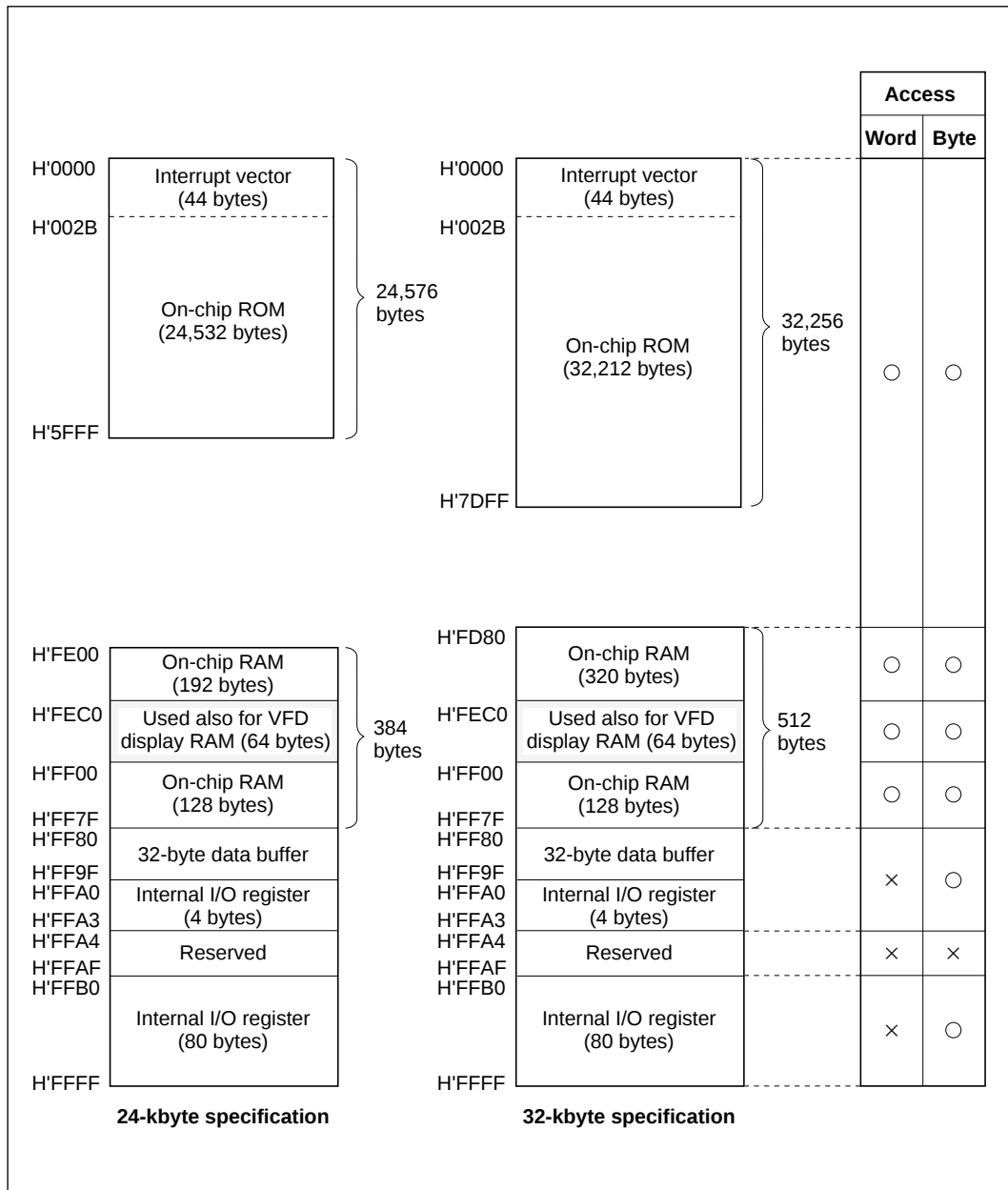
Figure 2-16 Data Size for Access to and from On-Chip Peripheral Modules (1)
