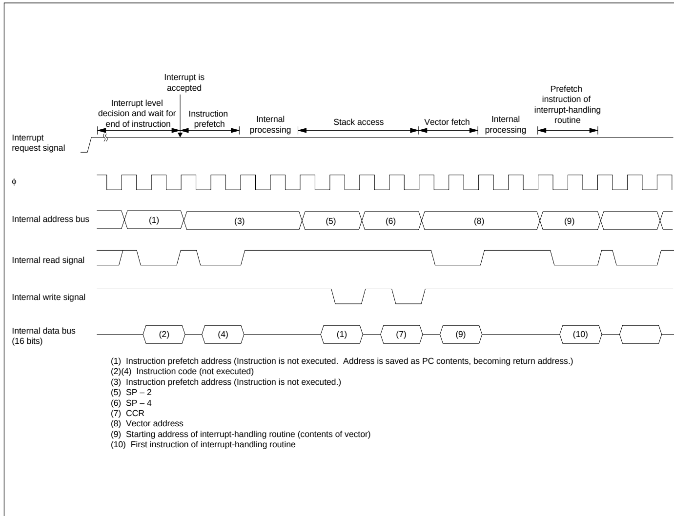
Figure 3-5 Interrupt Sequence
