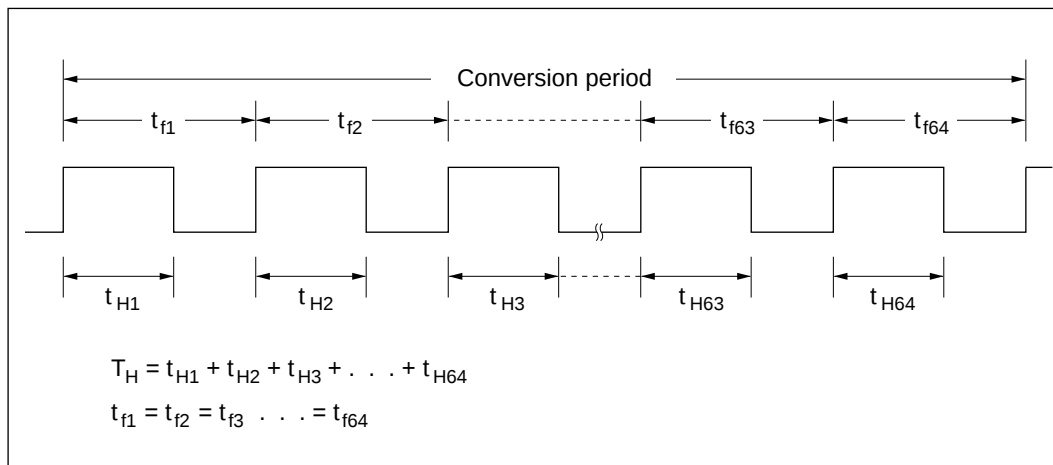
Figure 9-2 PWM Output Waveform
