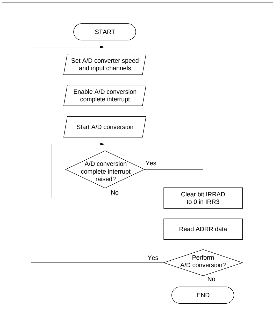
Figure 13-5 Conceptual Flow Chart of A/D Converter Use (2) (interrupts used)
