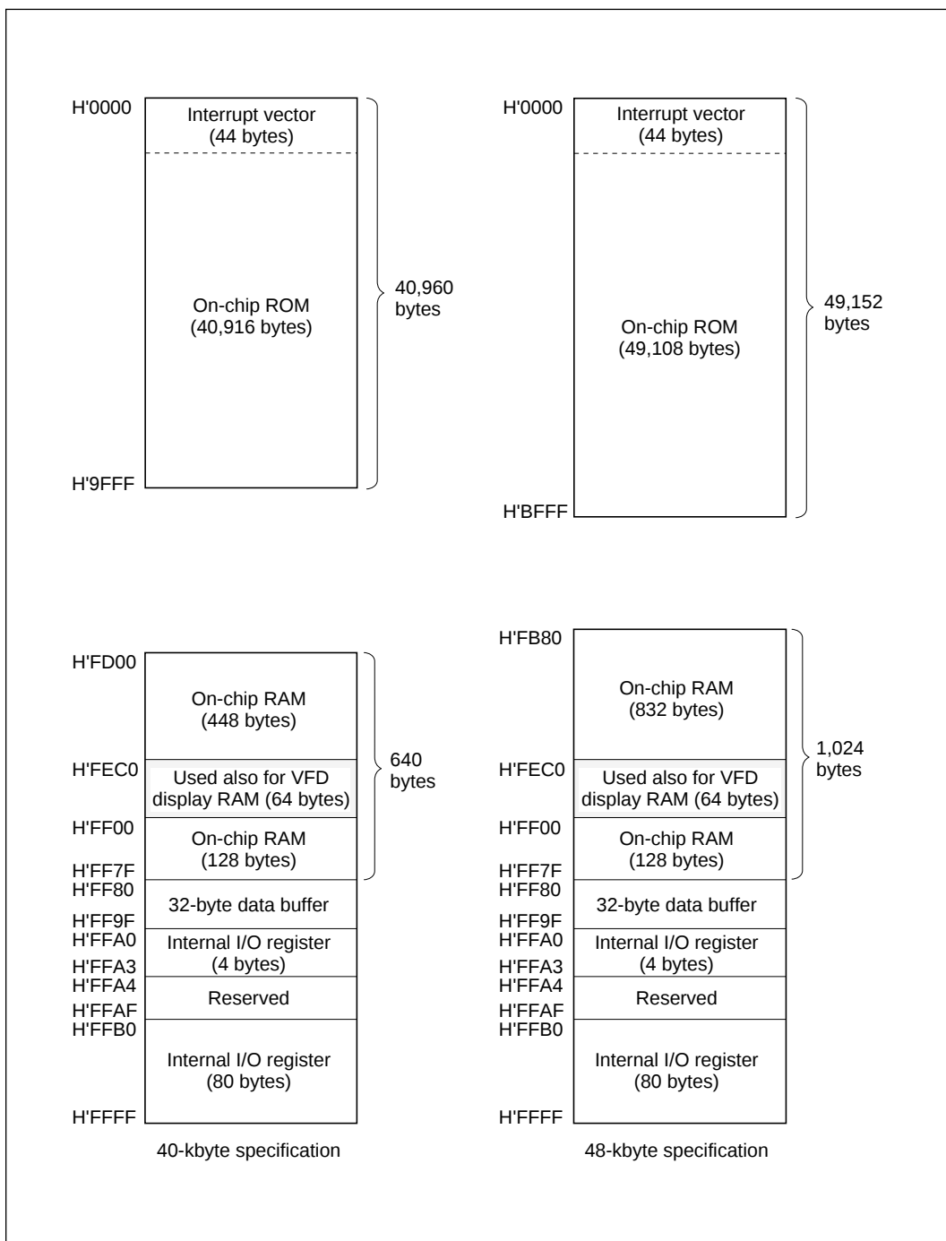
Figure 2-1 Memory Map (2)
