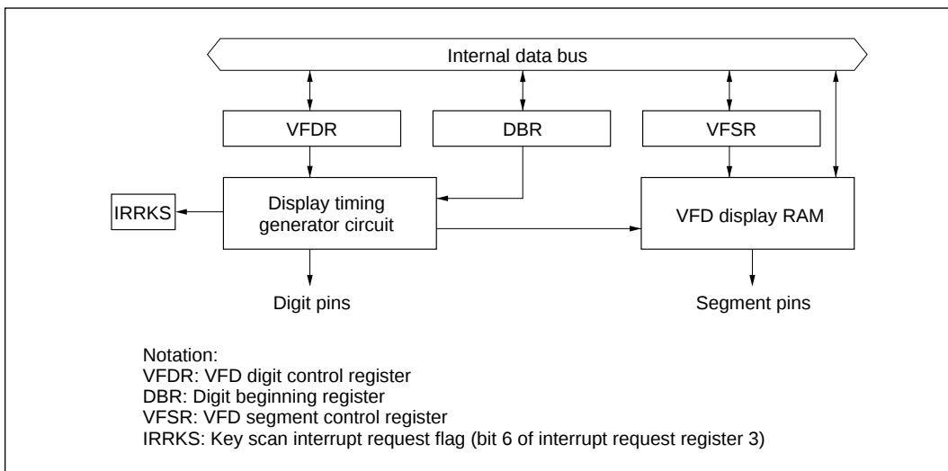
Figure 12-1 Block Diagram
