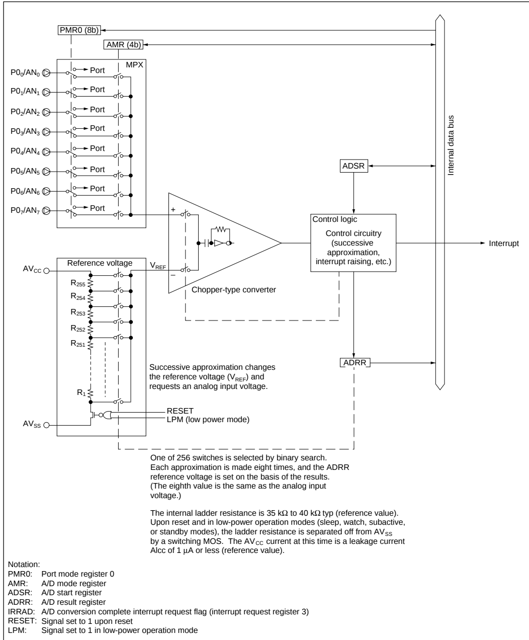
Figure 13-1 Block Diagram
