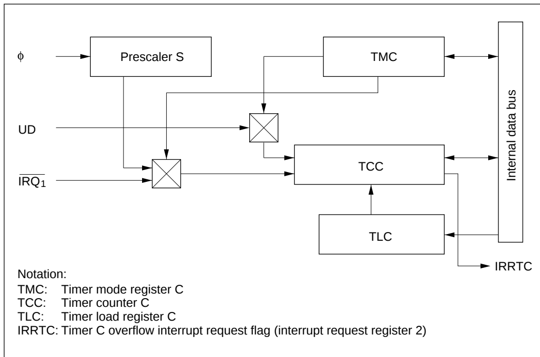
Figure 8-4 Block Diagram
