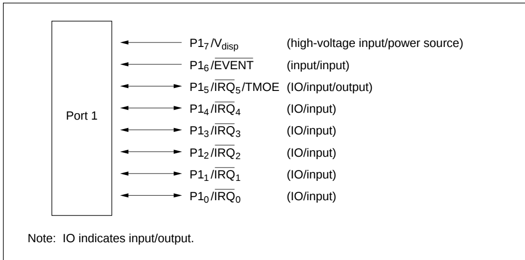
Figure 7-4 Port 1 Pin Configuration
