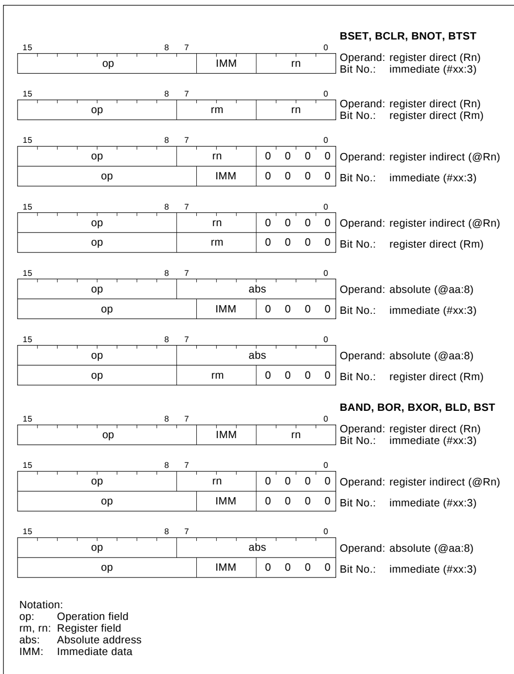
Figure 2-8 Bit Manipulation Instruction Codes
