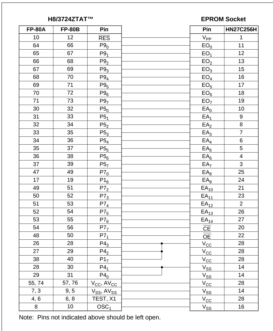
Figure 4-2 Socket Adapter Pin Correspondence (1)
