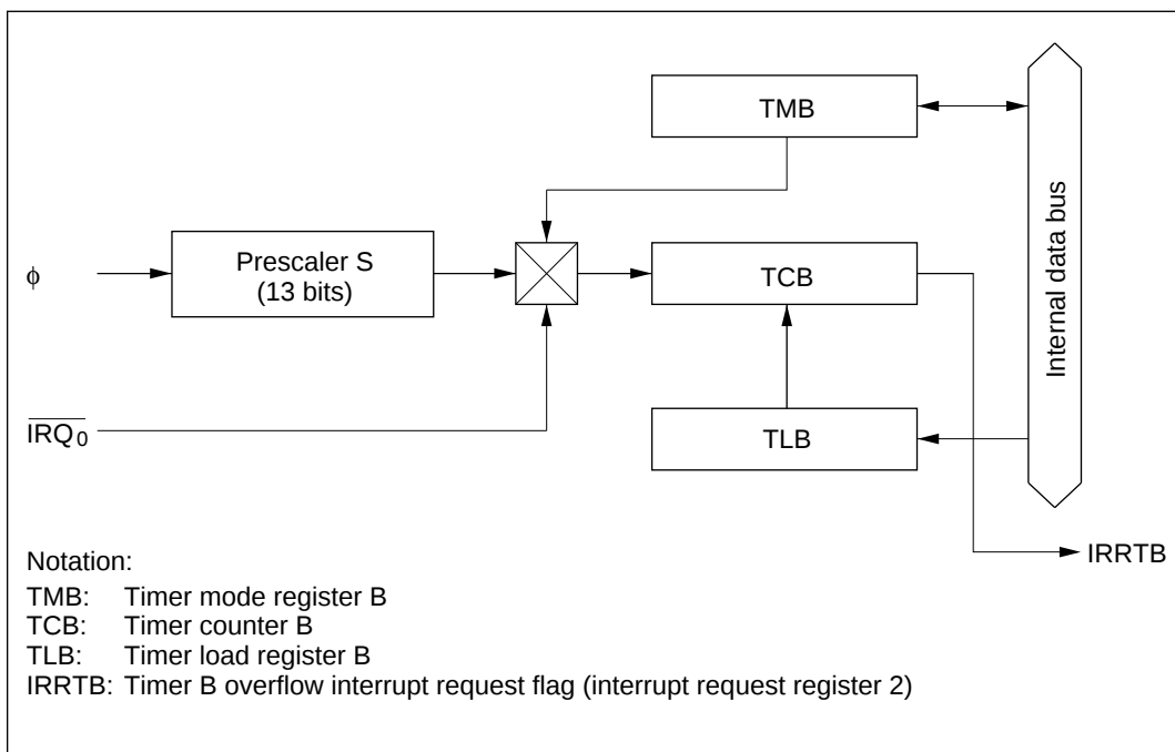
Figure 8-3 Block Diagram
