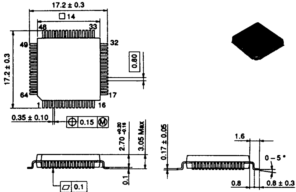
Figure G-1 External Dimensions (FP-64A)
