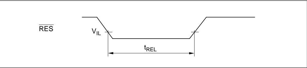
Figure 14-2 RES Pin Pulse Width (Low)
