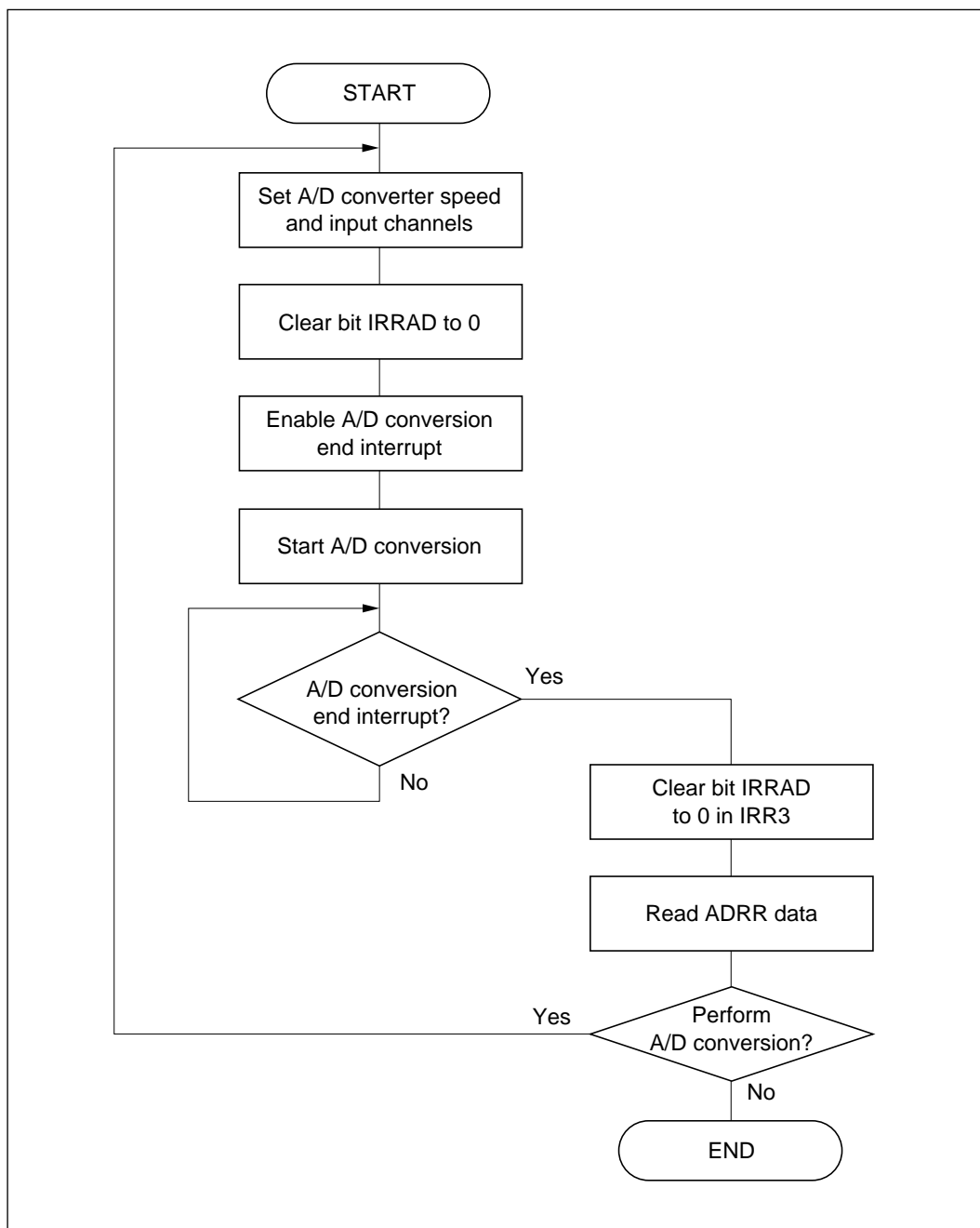
Figure 13-5 Flow Chart of Procedure for Using A/D Converter (2) (Interrupts Used)
