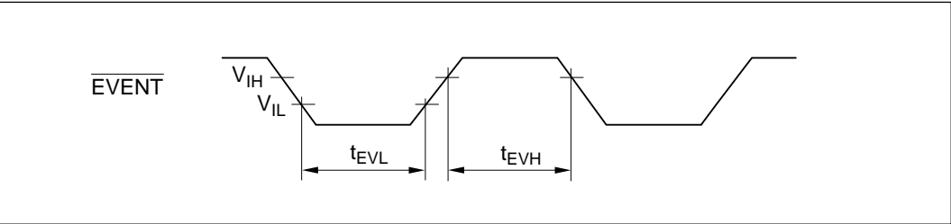
Figure 14-4 EVENT Pin Minimum Pulse Widths
