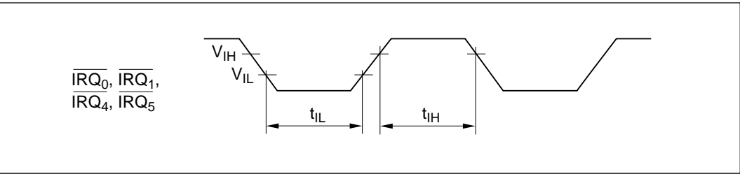
Figure 14-3 IRQ Pin Input Timing
