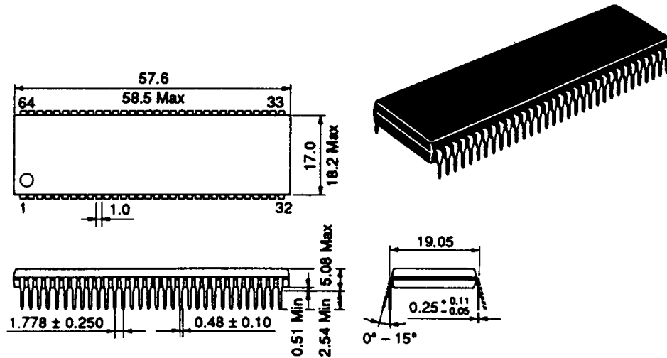
Figure G-2 External Dimensions (DP-64S)
