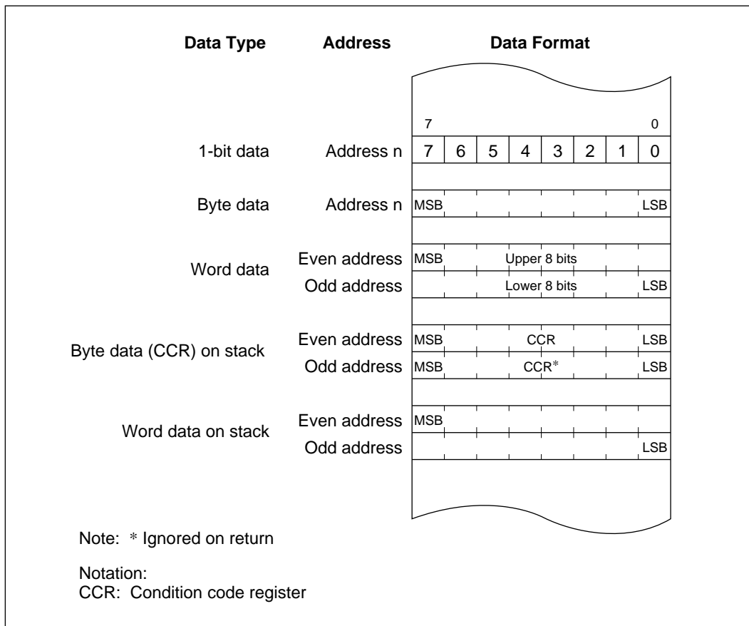
Figure 2-5 Memory Data Formats
