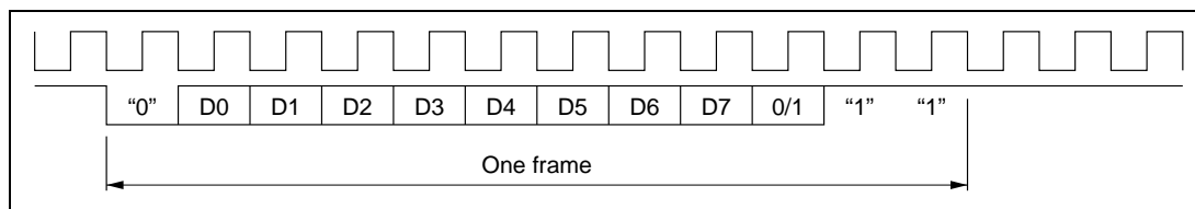
Figure 9-3. Phase Relationship between Clock Output and Transmit Data (Asynchronous Mode)
