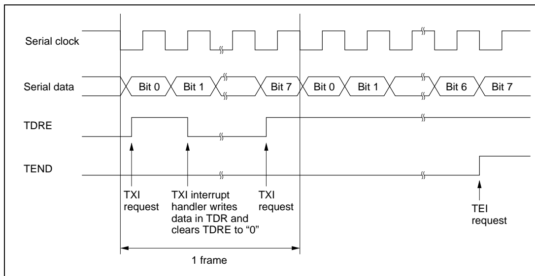
Figure 9-14. Example of SCI Transmit Operation
