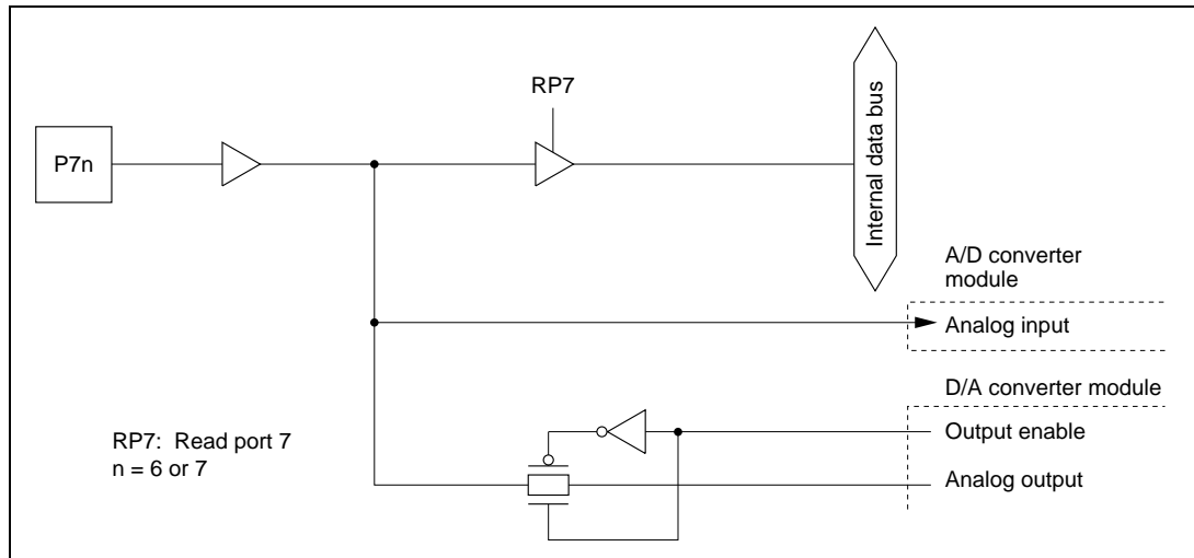
Figure 5-14. Port 7 Schematic Diagram (Pins P7 6 and P7 7 )
