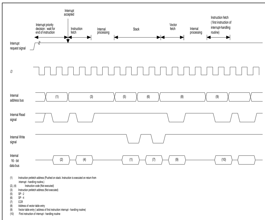
Figure 4-6. Timing of Interrupt Sequence
