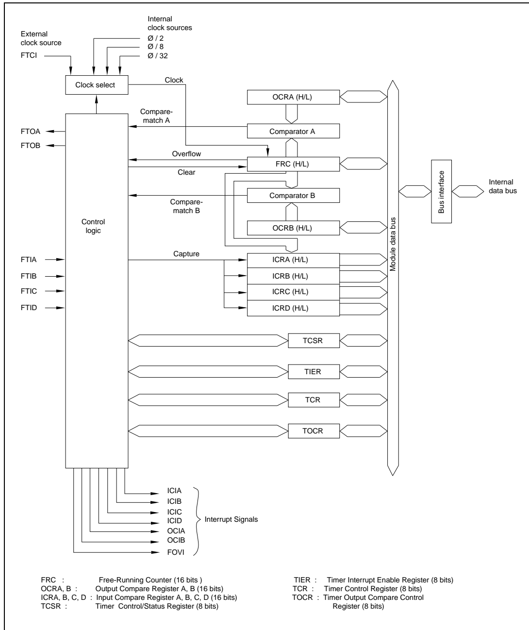
Figure 6-1. Block Diagram of 16-Bit Free-Running Timer
