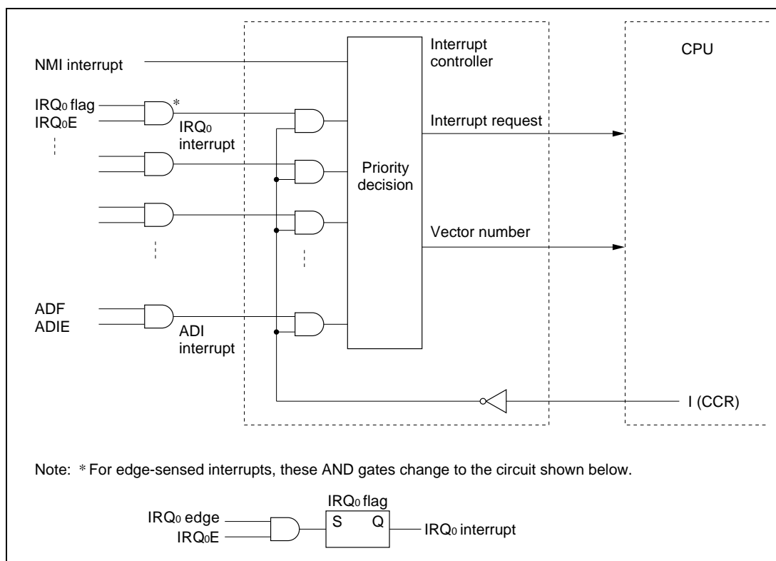
Figure 4-3. Block Diagram of Interrupt Controller
