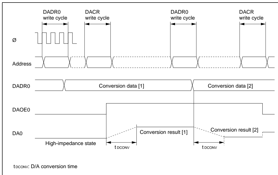
Figure 11-2. D/A Conversion (Example)
