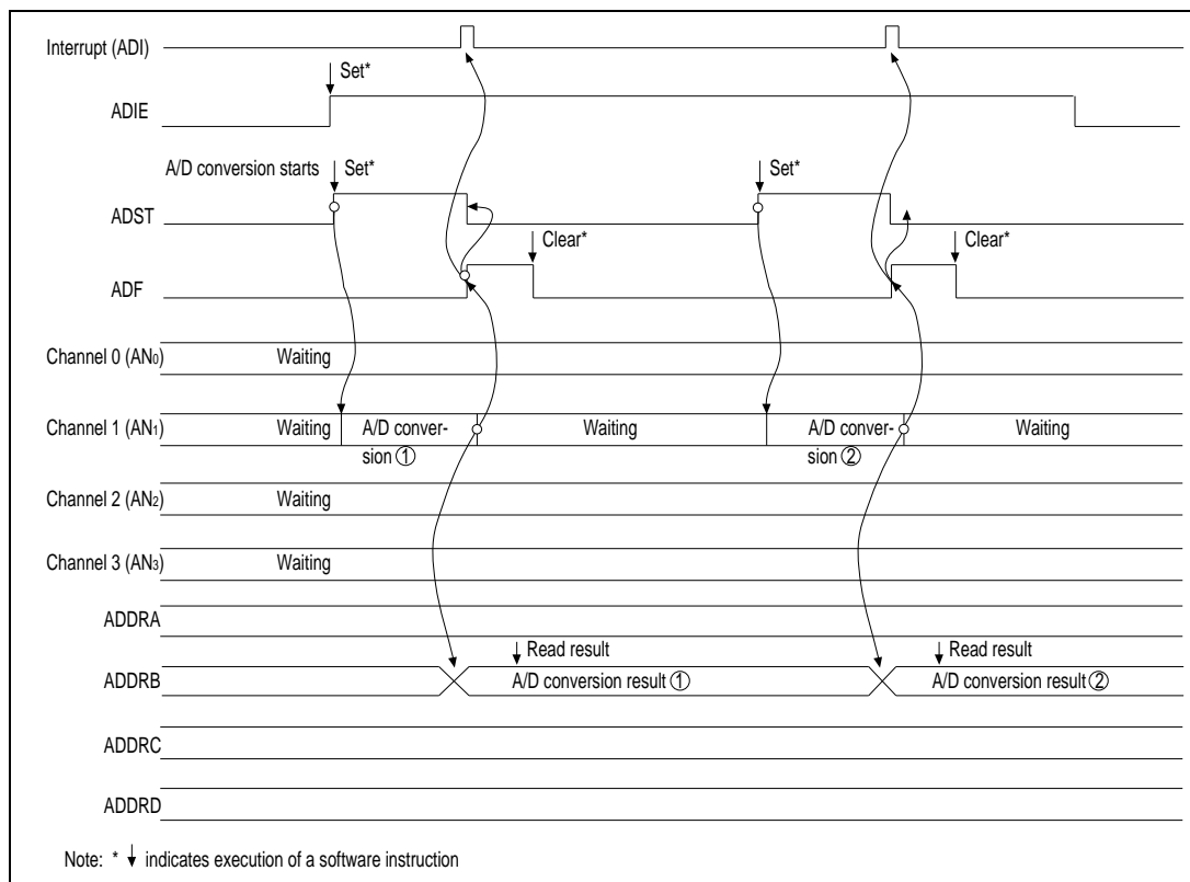
Figure 10-2 A/D Operation in Single Mode (when Channel 1 is Selected)
