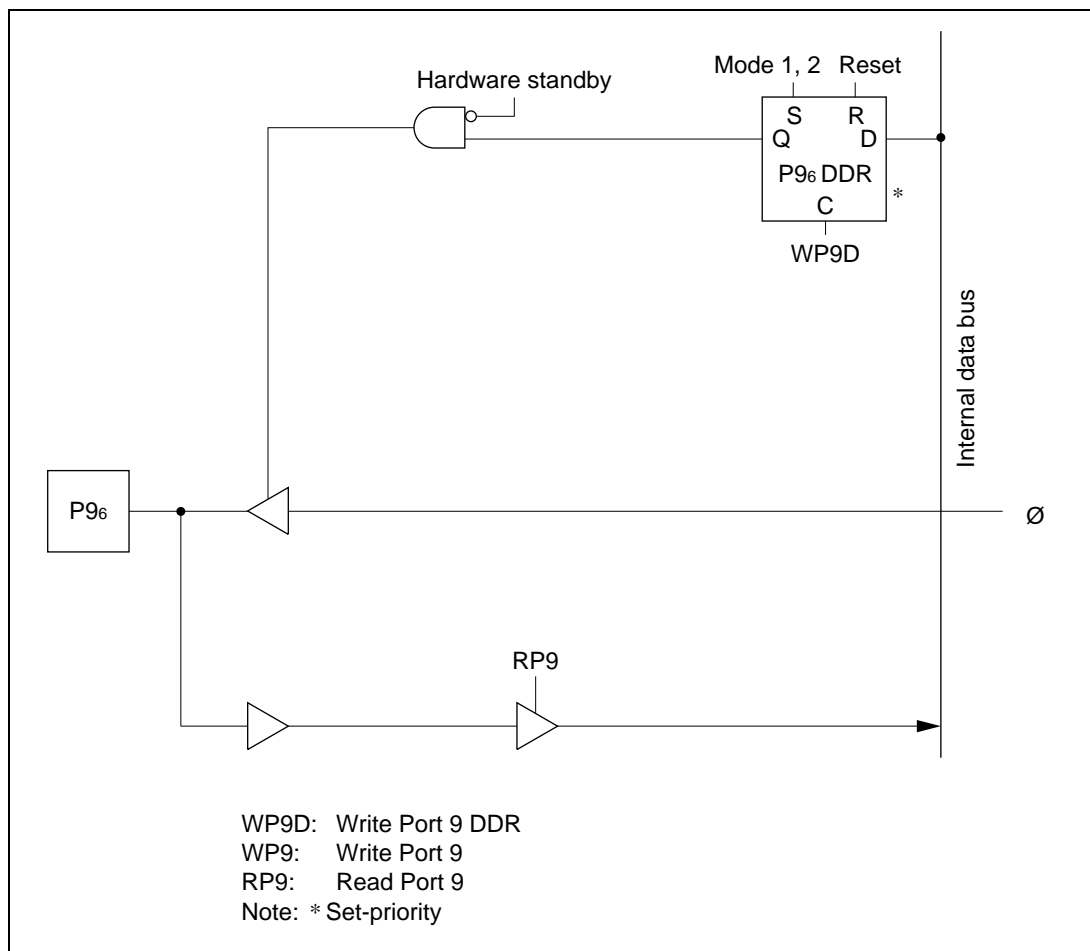
Figure 5-22. Port 9 Schematic Diagram (Pin P9 6 )
