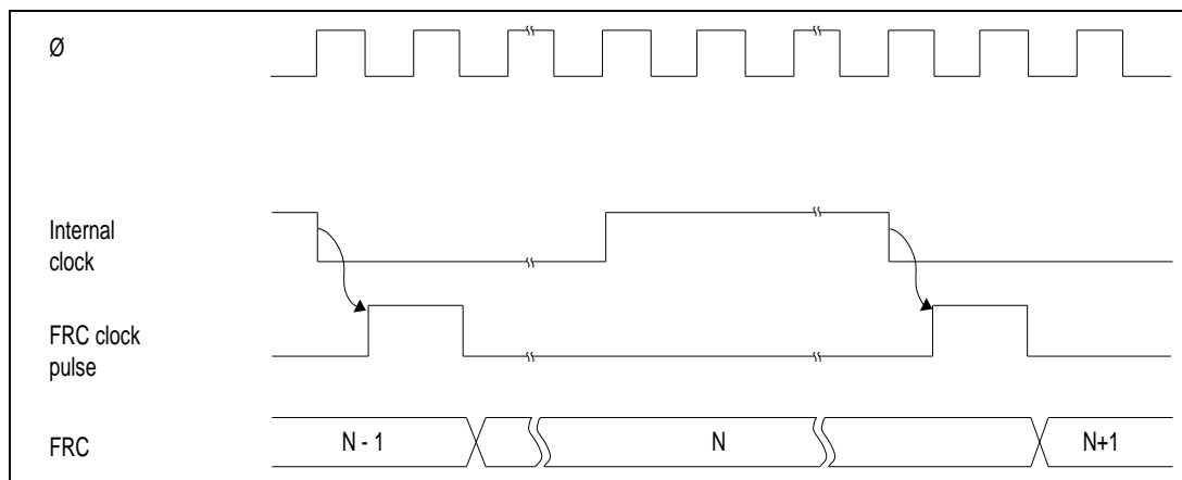
Figure 6-5. Increment Timing for Internal Clock Source
