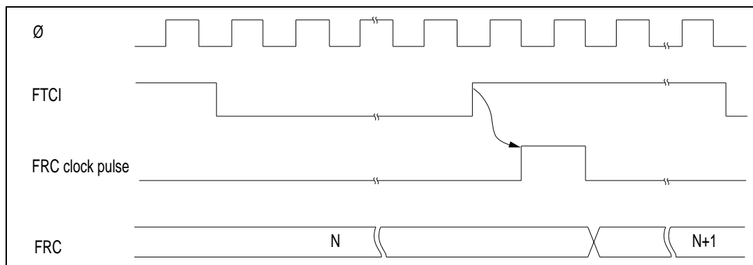
Figure 6-6. Increment Timing for External Clock Source
