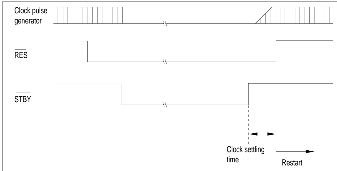
Figure 14-2. Hardware Standby Mode Timing
