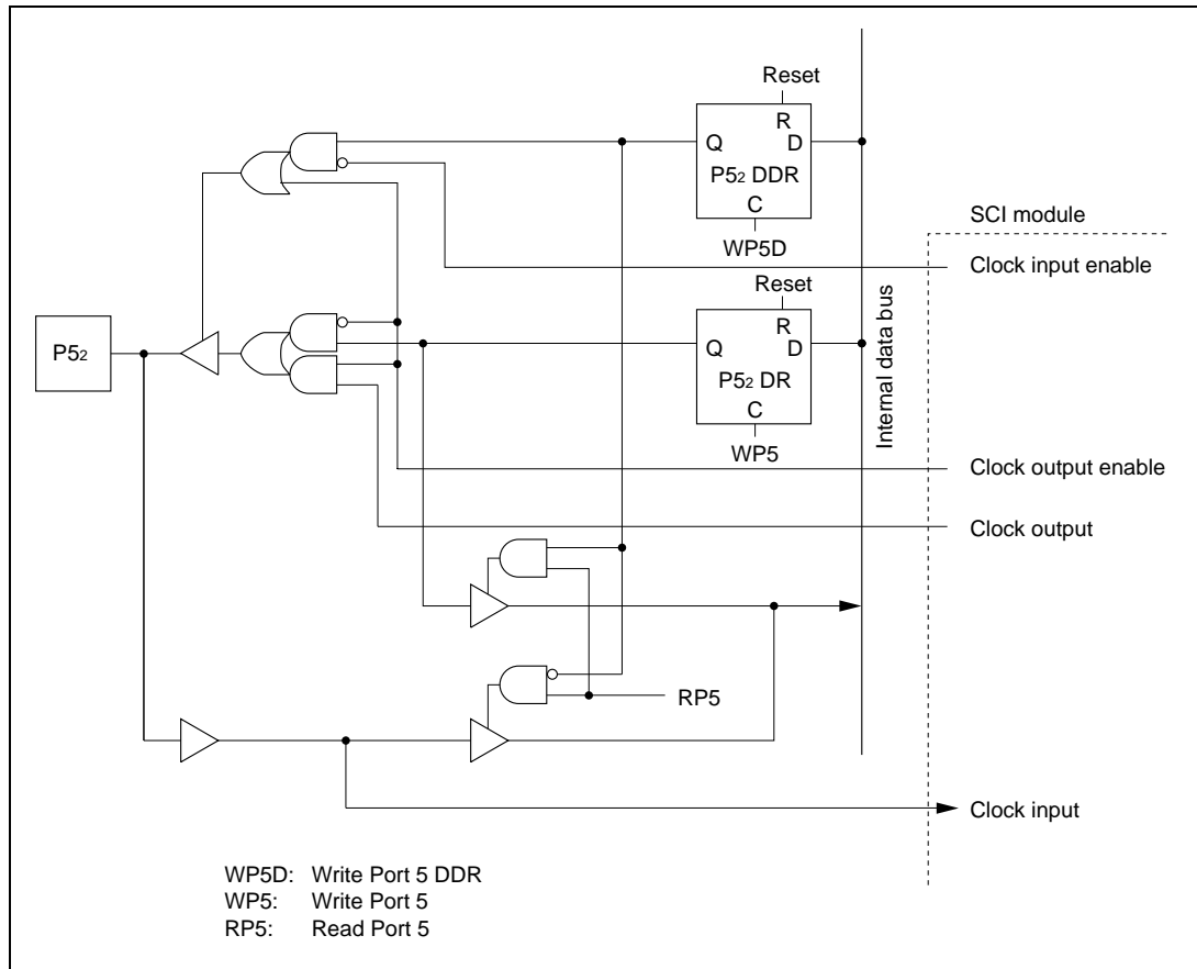
Figure 5-8. Port 5 Schematic Diagram (Pin P5 2 )
