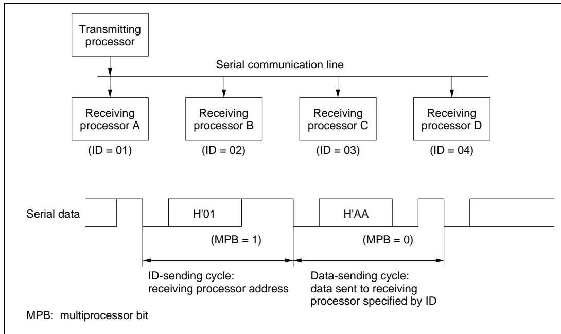
Figure 9-9. Example of Communication among Processors using Multiprocessor Format (Sending Data H'AA to Receiving Processor A)
