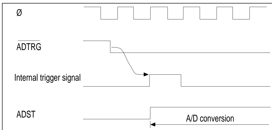
Figure 10-5. External Trigger Input Timing
