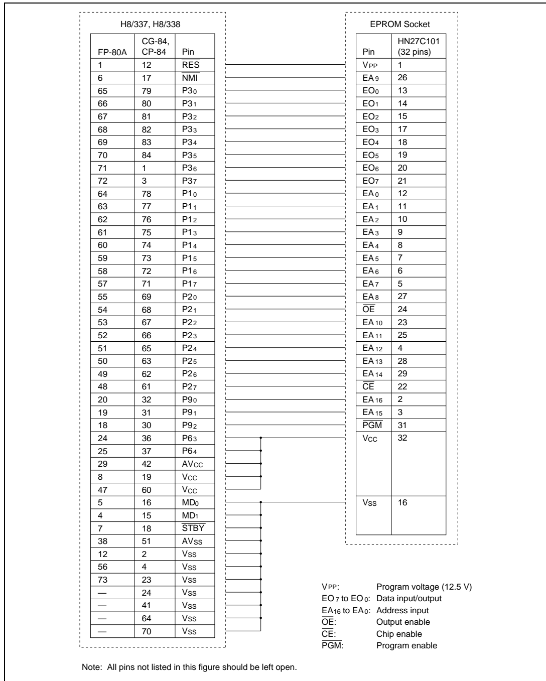
Figure 13-2. Socket Adapter Pin Assignments
