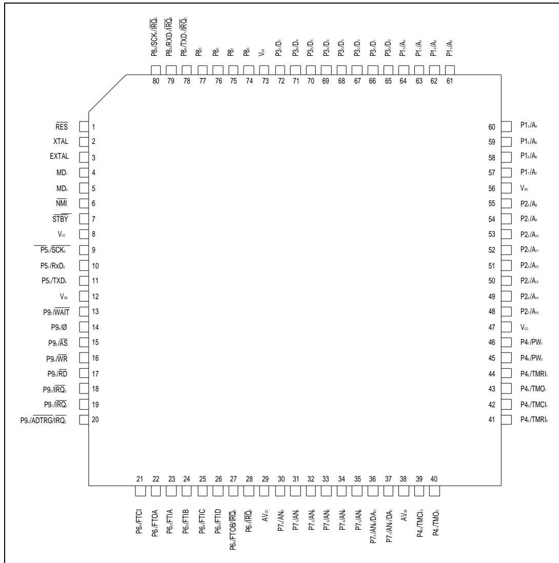
Figure 1-4. Pin Arrangements (FP-80A, Top View)
