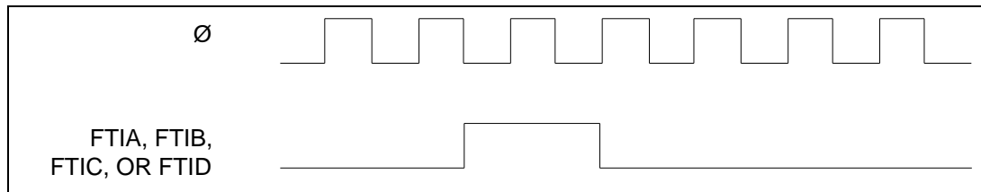
Figure 6-3. Minimum Input Capture Pulse Width
