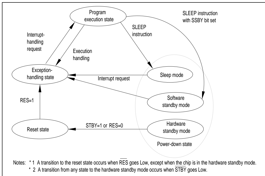
Figure 3-12. State Transitions
