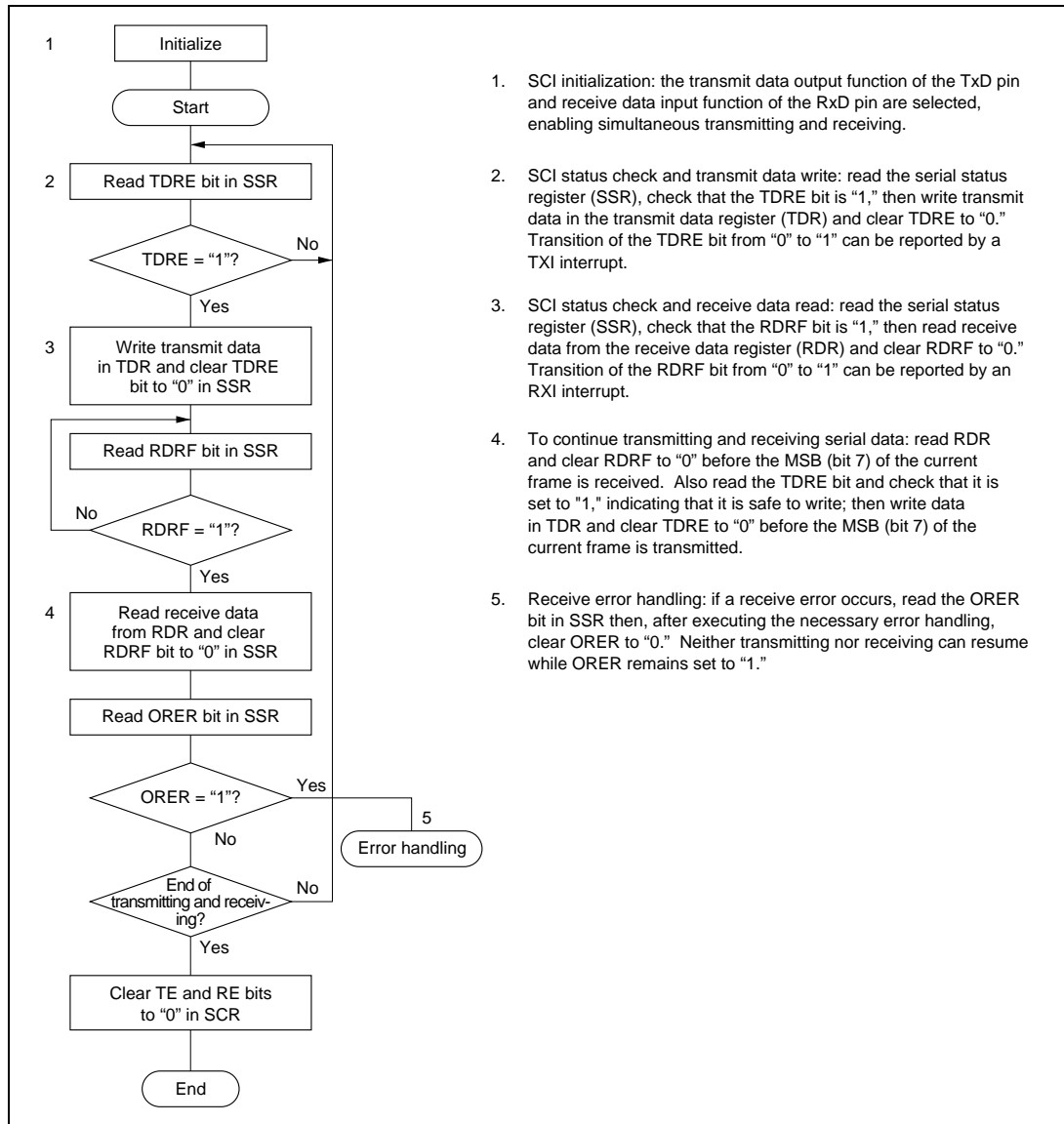
Figure 9-17. Sample Flowchart for Serial Transmitting and Receiving
