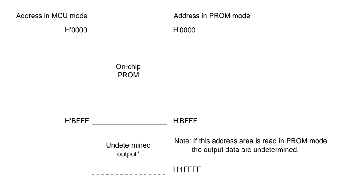
Figure 13-3. H8/338 Memory Map in PROM Mode
