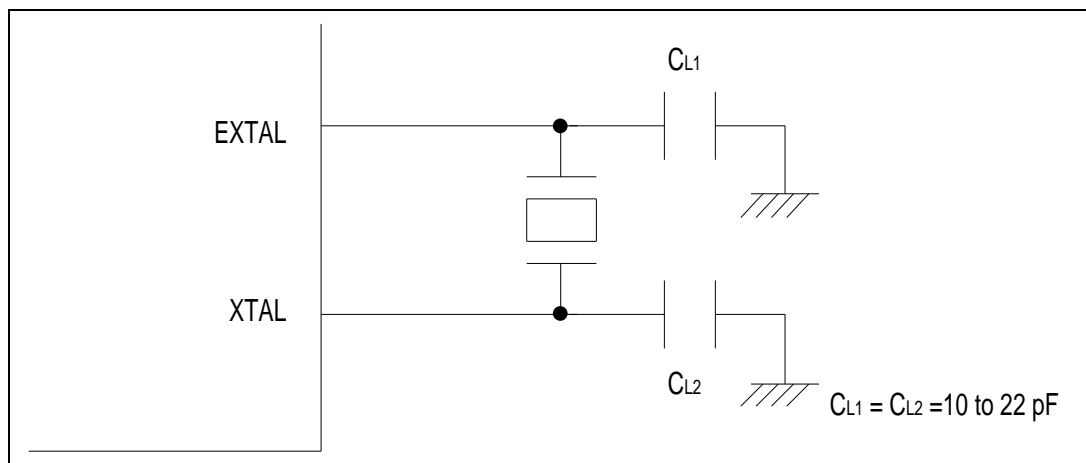
Figure 15-2. Connection of Crystal Oscillator (Example)
