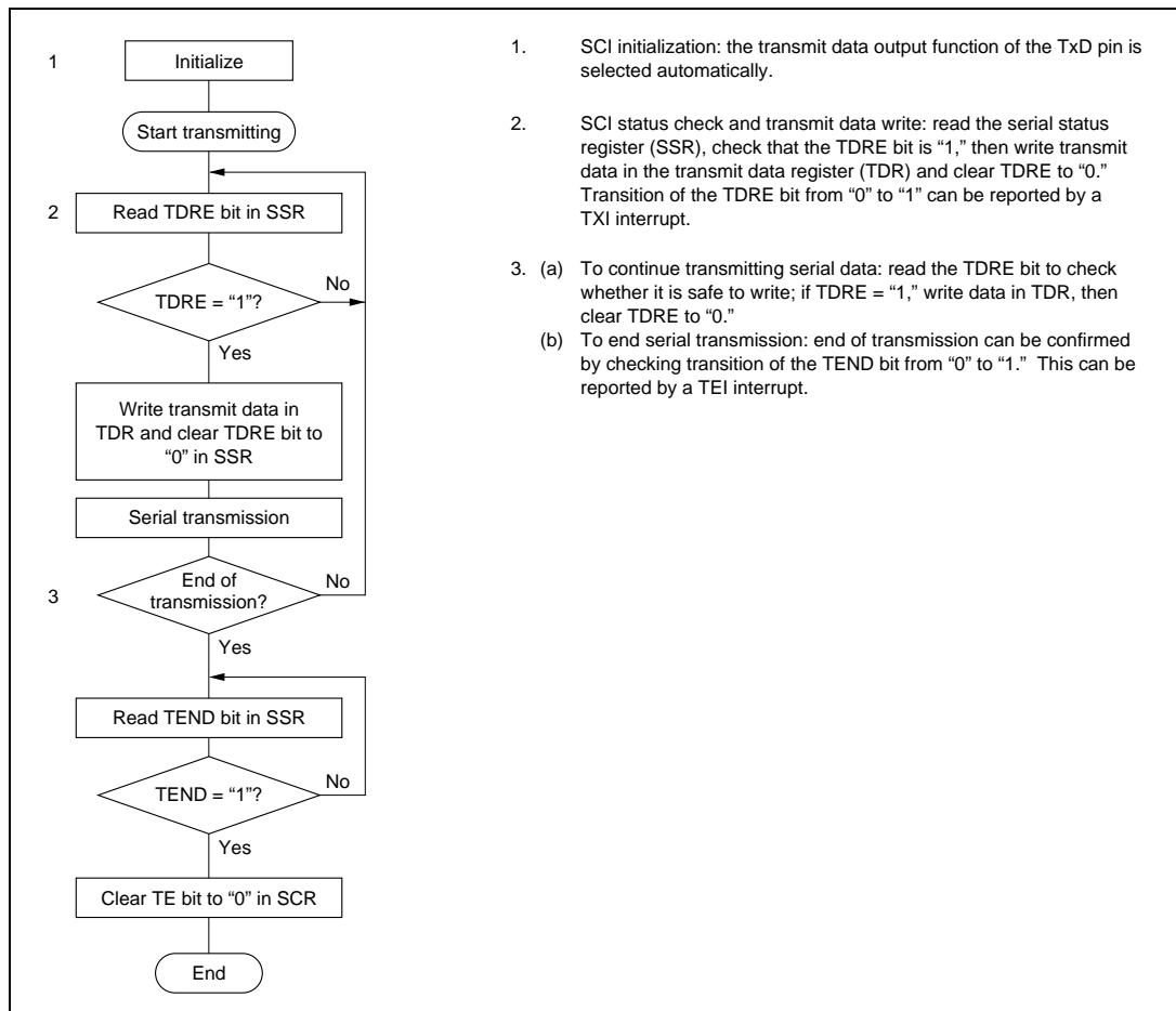
Figure 9-13. Sample Flowchart for Serial Transmitting
