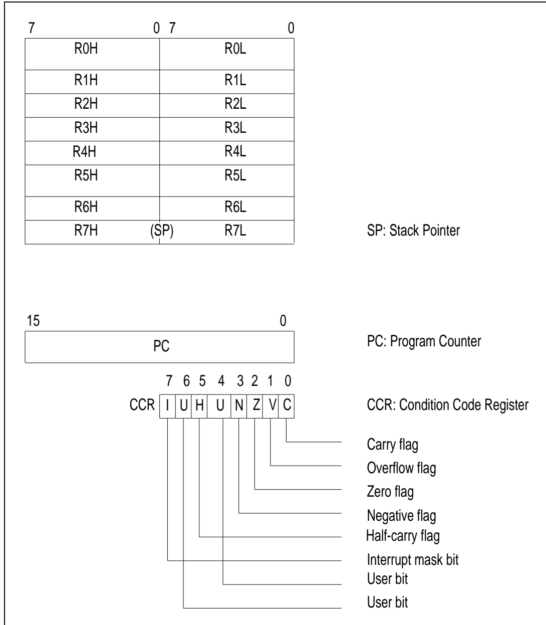
Figure 3-1. CPU Registers
