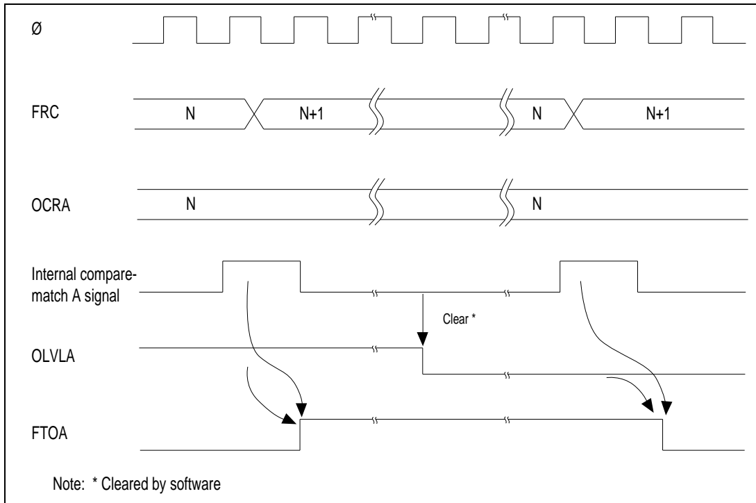
Figure 6-9. Timing of Output Compare A
