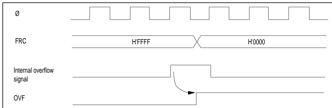
Figure 6-16. Setting of Overflow Flag (OVF)
