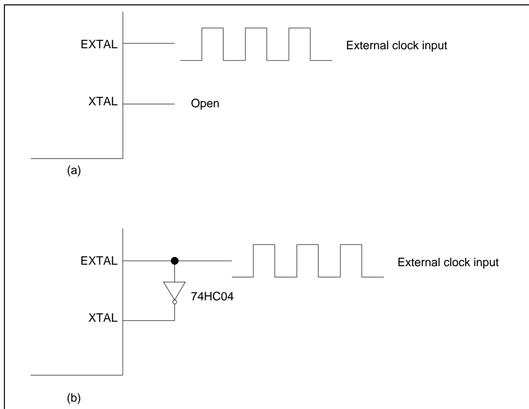
Figure 15-5. External Clock Input (Example)
