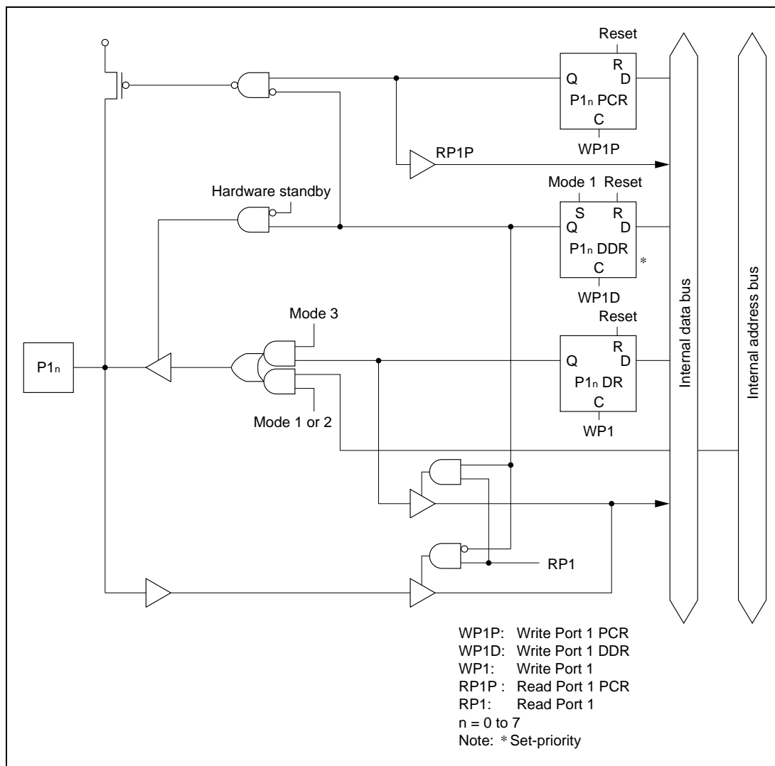
Figure 5-1. Port 1 Schematic Diagram
