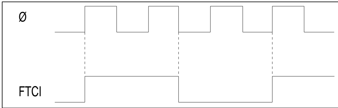
Figure 6-7. Minimum External Clock Pulse Width
