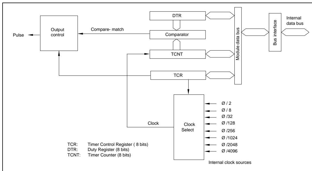
Figure 8-1. Block Diagram of PWM Timer
