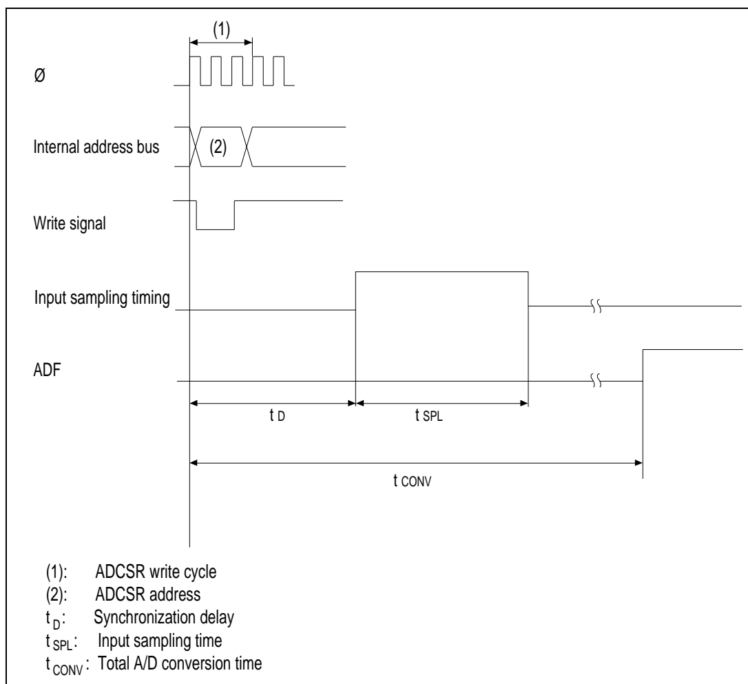
Figure 10-4. A/D Conversion Timing
