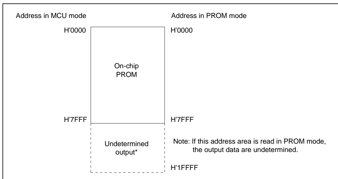
Figure 13-4. H8/337 Memory Map in PROM Mode
