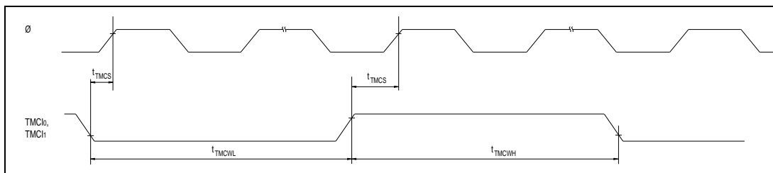
Figure 16-13. 8-Bit Timer Clock Input Timing
