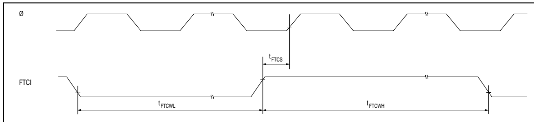
Figure 16-11. External Clock Input Timing for Free-Running Timer
