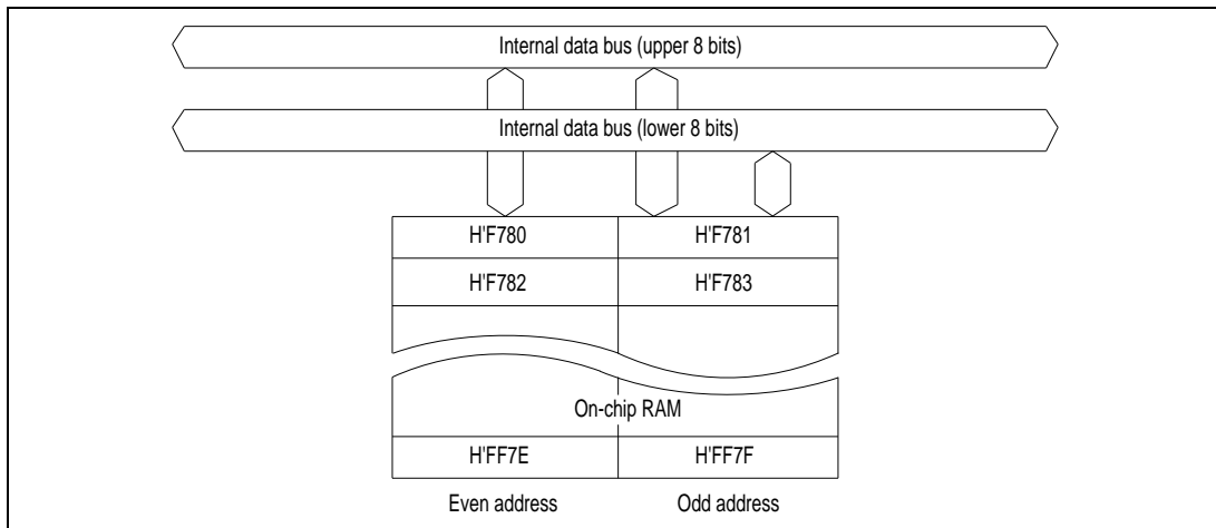
Figure 12-1. Block Diagram of On-Chip RAM (H8/338)
