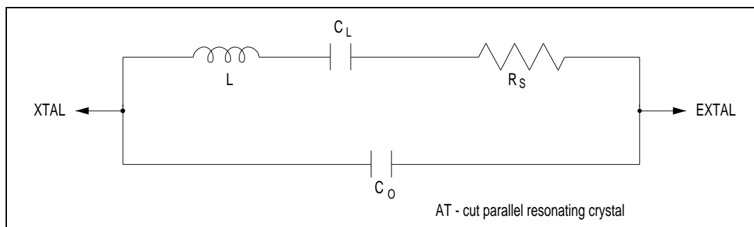
Figure 15-3. Equivalent Circuit of External Crystal
