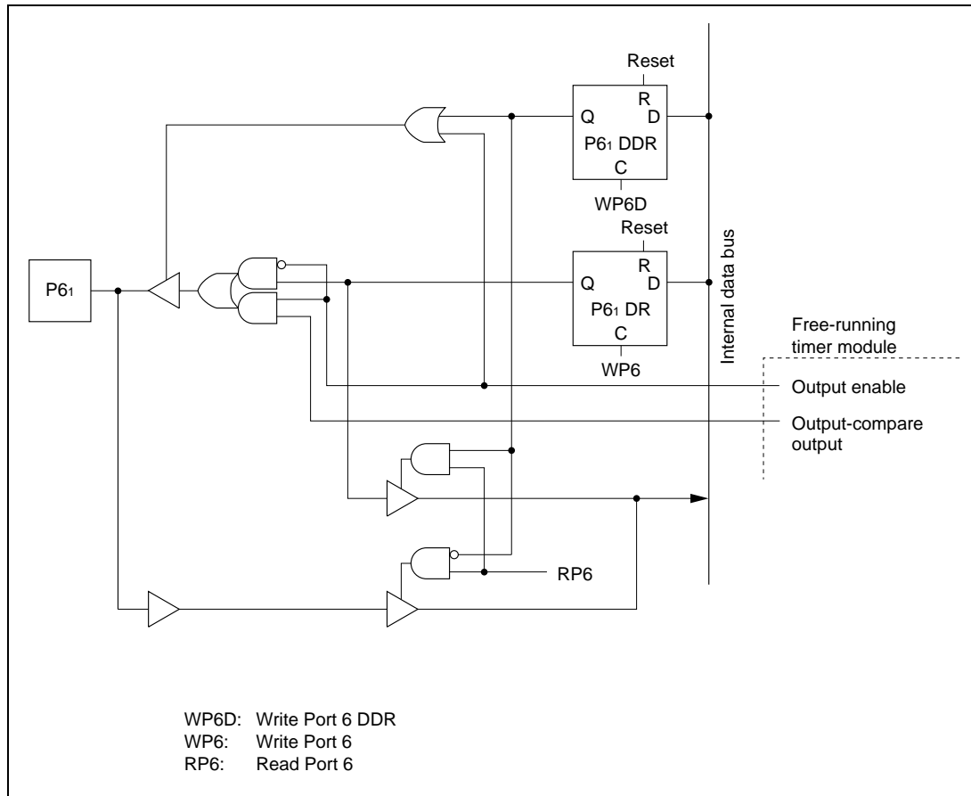
Figure 5-10. Port 6 Schematic Diagram (Pin P6 i )
