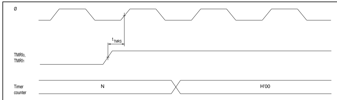
Figure 16-14. 8-Bit Timer Reset Input Timing
