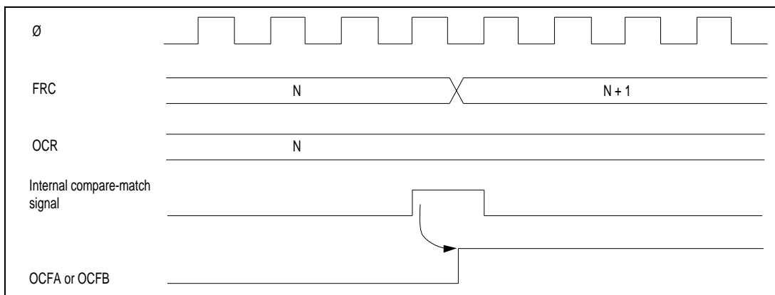
Figure 6-8. Setting of Output Compare Flags
