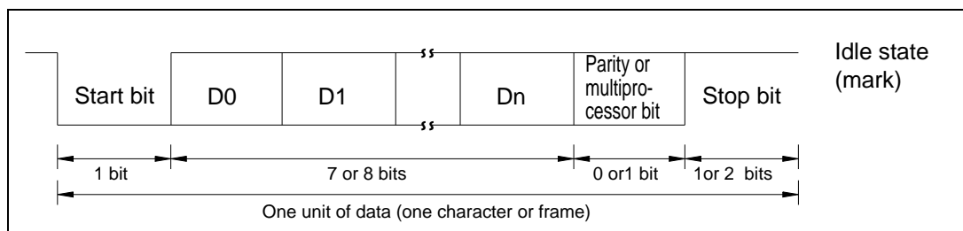
Figure 9-2. Data Format in Asynchronous Mode
