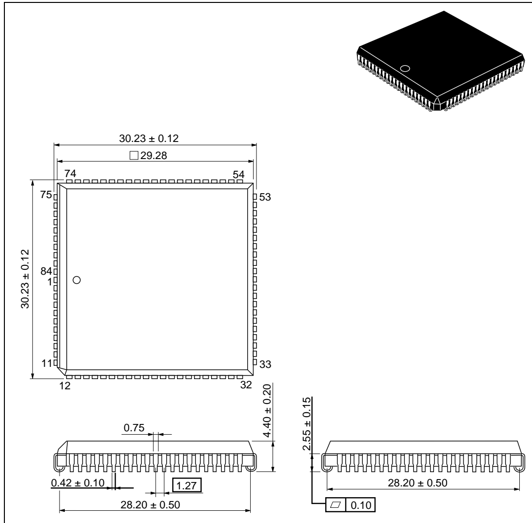
Figure E-2. Package Dimensions (CP-84)
