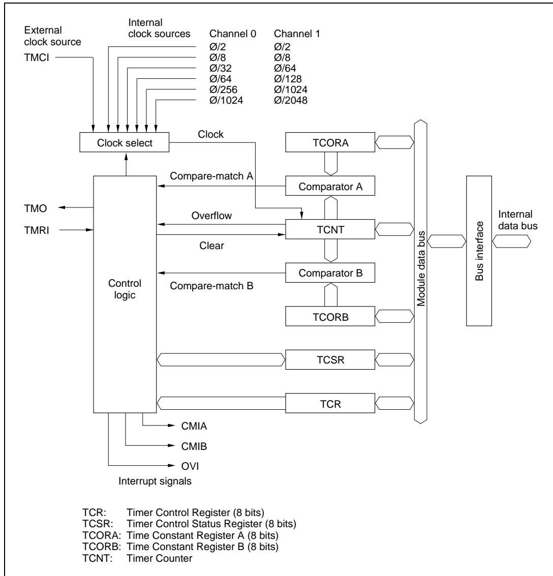
Figure 7-1. Block Diagram of 8-Bit Timer
