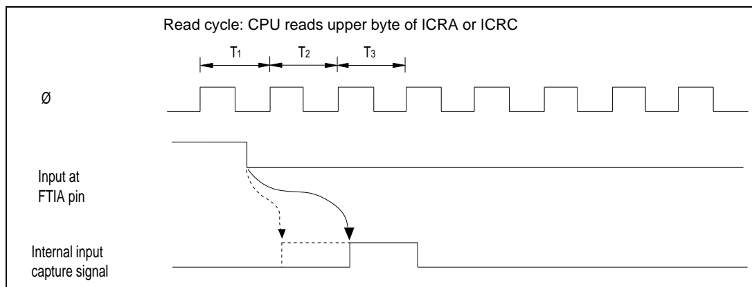
Figure 6-13. Input Capture Timing (1-State Delay, Buffer Mode)
