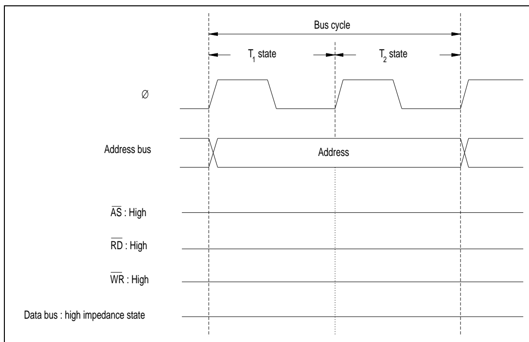
Figure 3-14. Pin States during On-Chip Memory Access Cycle
