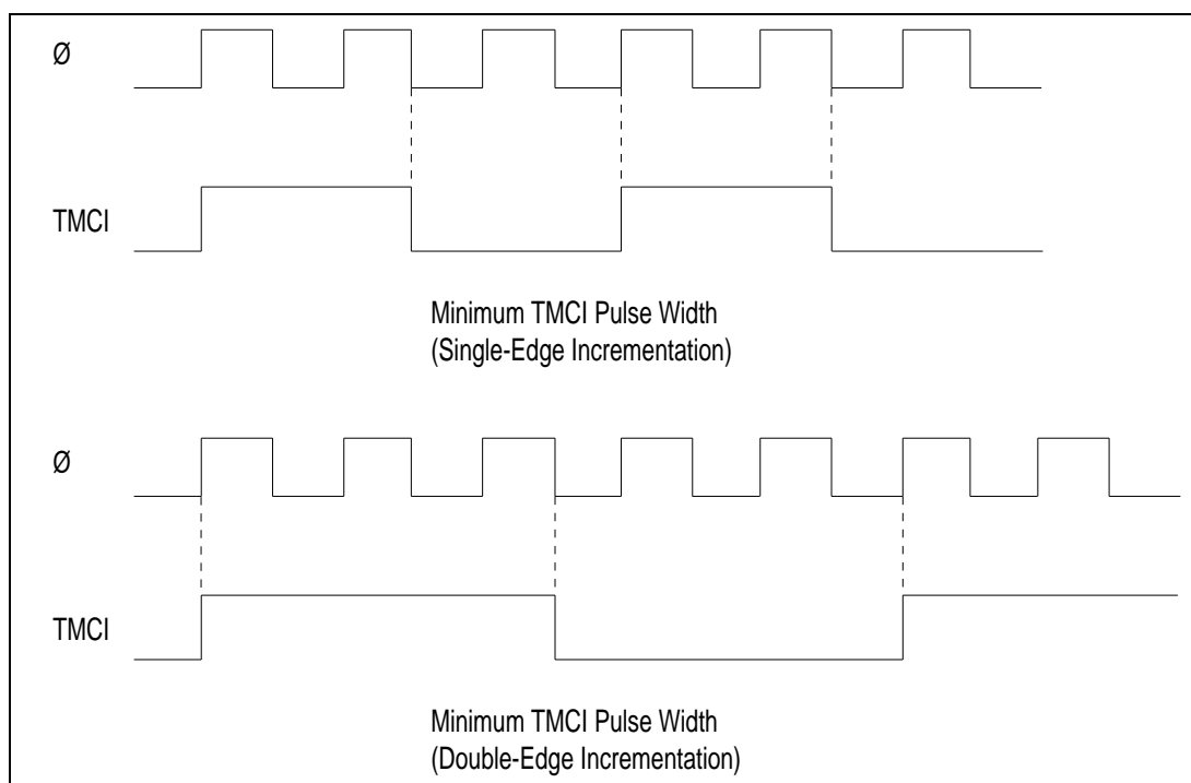
Figure 7-4. Minimum External Clock Pulse Widths (Example)
