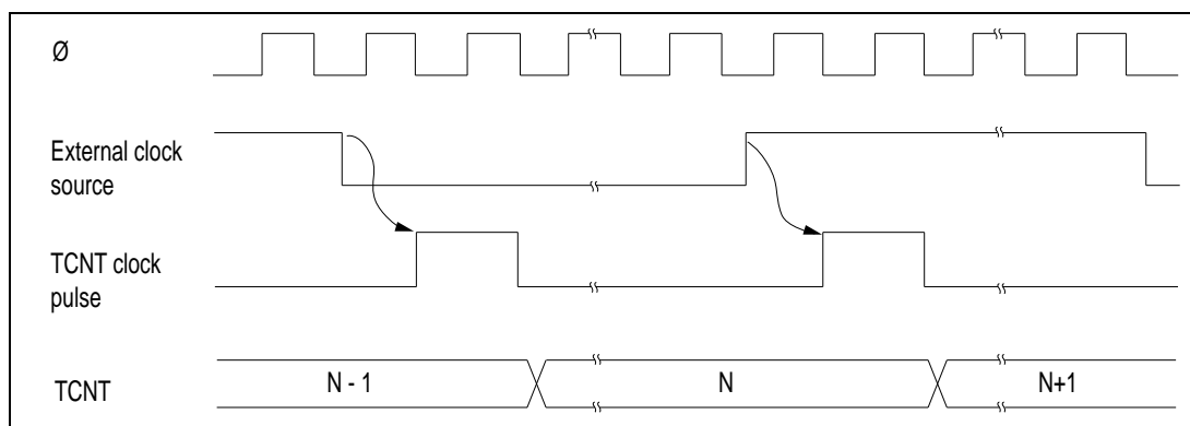
Figure 7-3. Count Timing for External Clock Input
