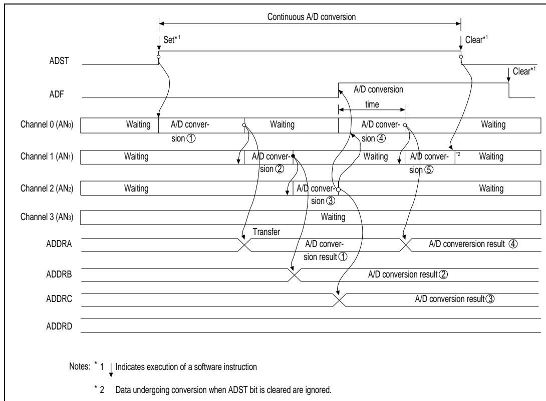
Figure 10-3 A/D Operation in Scan Mode (when Channel 0 to 2 are Selected)
