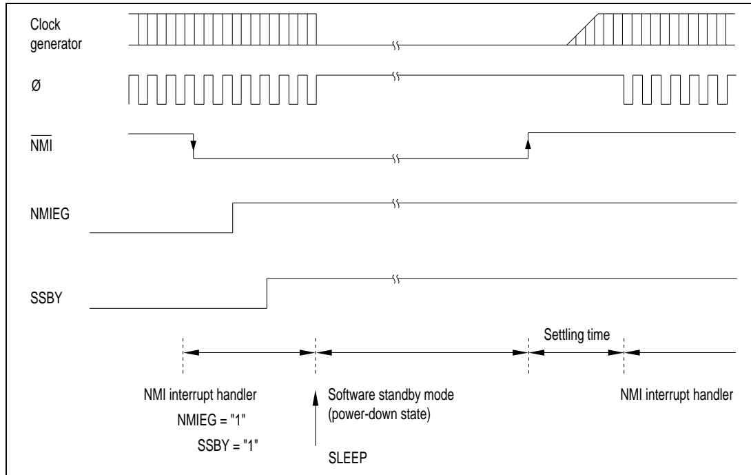
Figure 14-1. NMI Timing in Software Standby Mode
