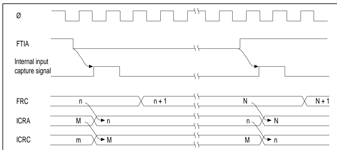
Figure 6-14. Buffered Input Capture with Both Edges Selected
