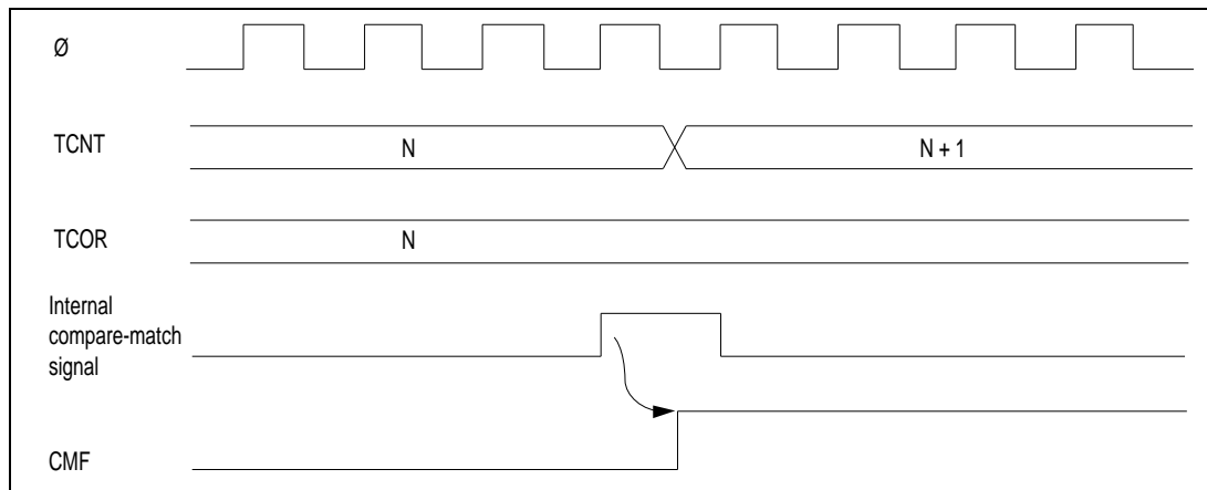
Figure 7-5. Setting of Compare-Match Flags
