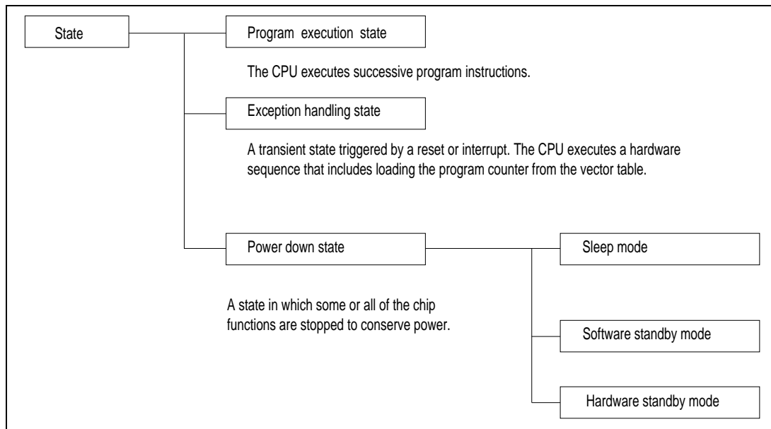
Figure 3-11. Operating States
