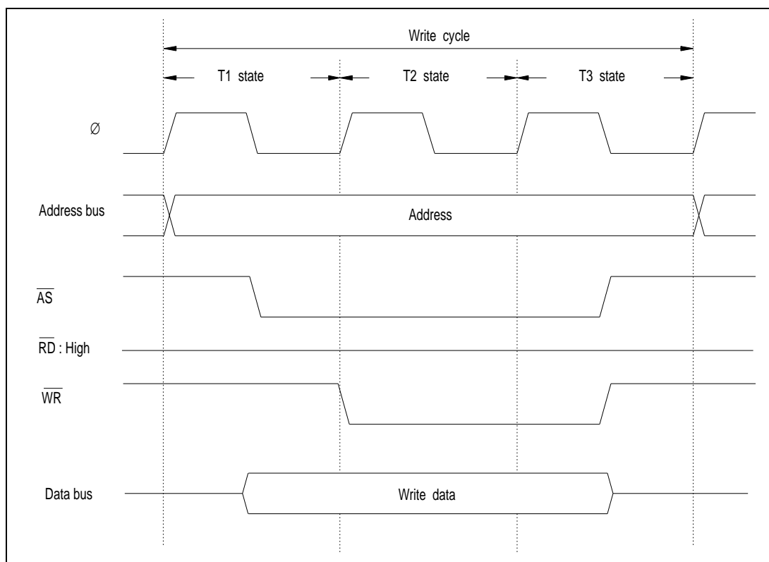
Figure 3-17 (b). External Device Access Timing (Write)
