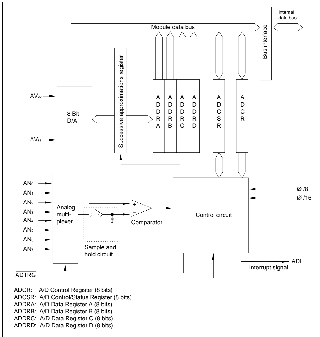
Figure 10-1. Block Diagram of A/D Converter
