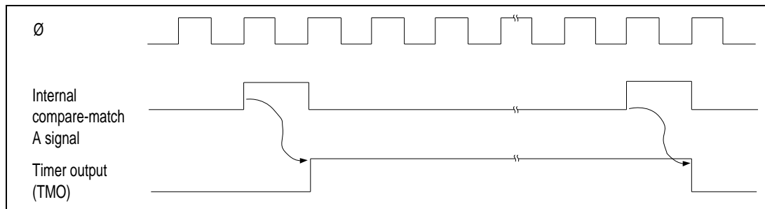
Figure 7-6. Timing of Timer Output
