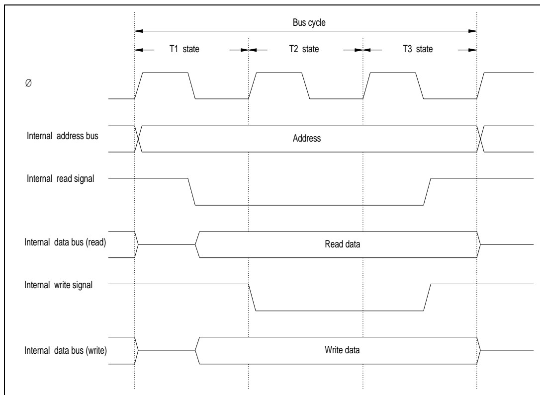
Figure 3-15. On-Chip Register Field Access Cycle
