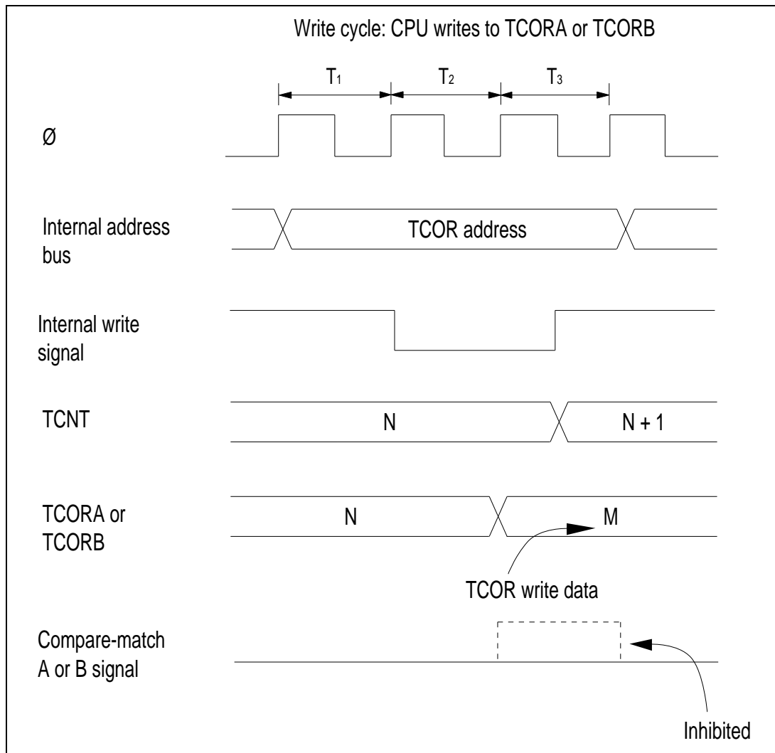
Figure 7-13. Contention between TCOR Write and Compare-Match
