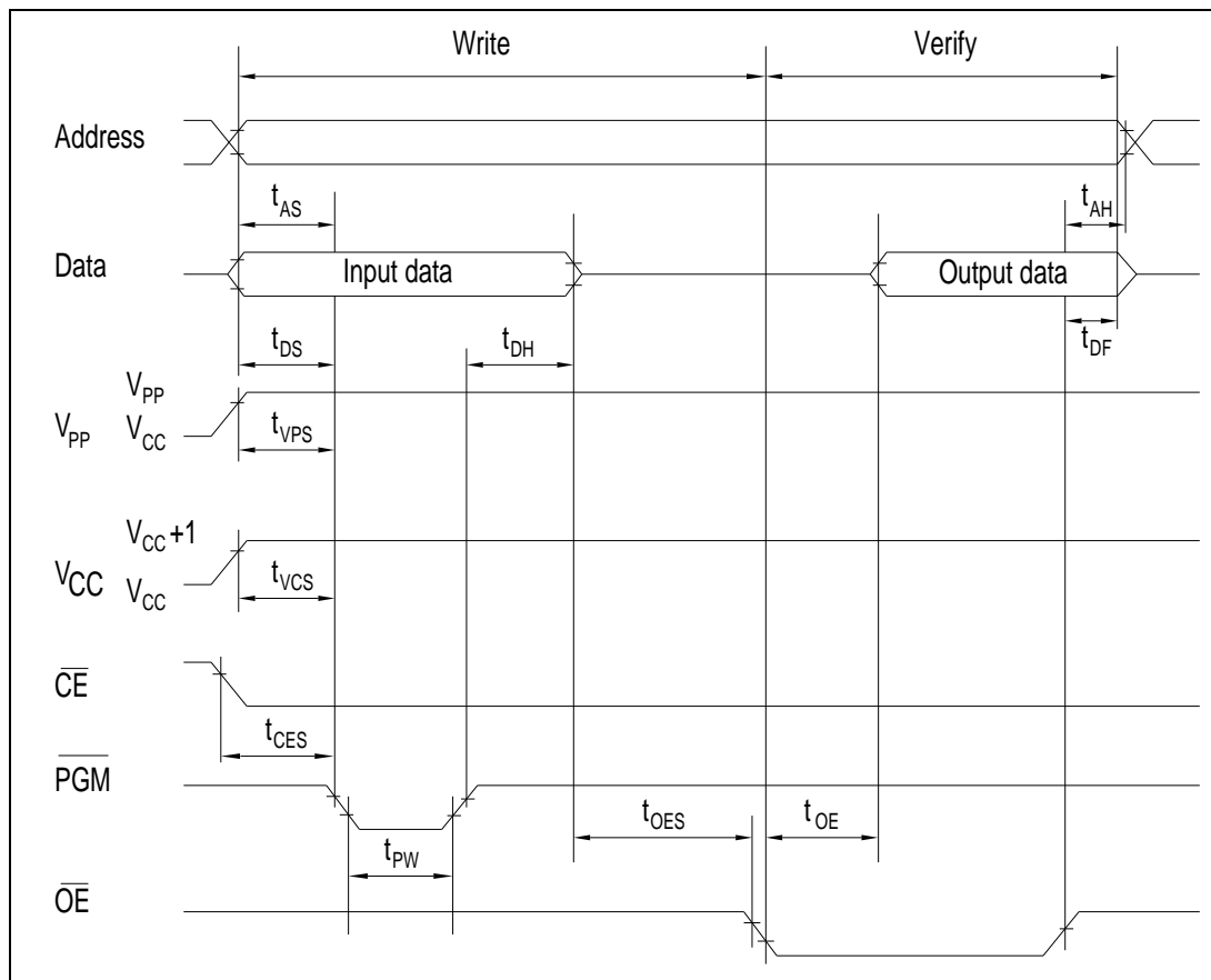
Figure 13-6. PROM Write/Verify Timing
