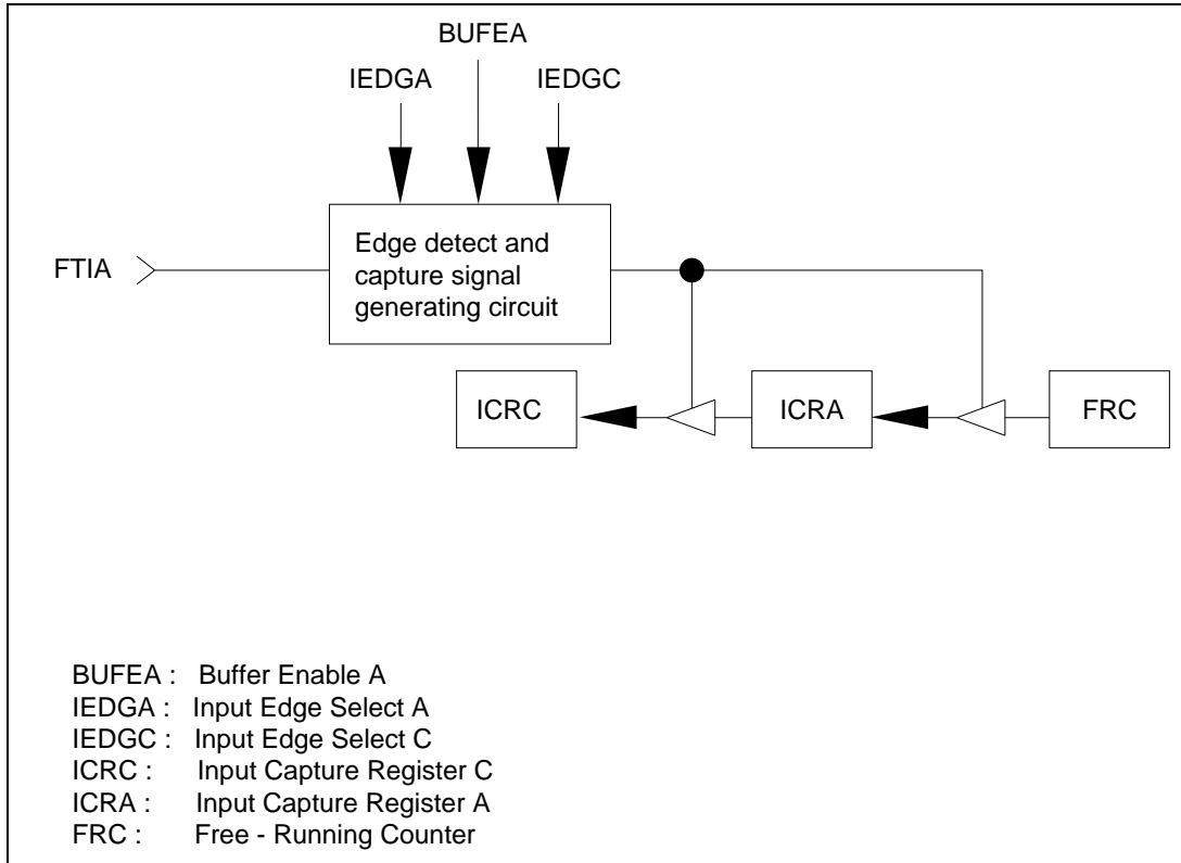
Figure 6-2. Input Capture Buffering
