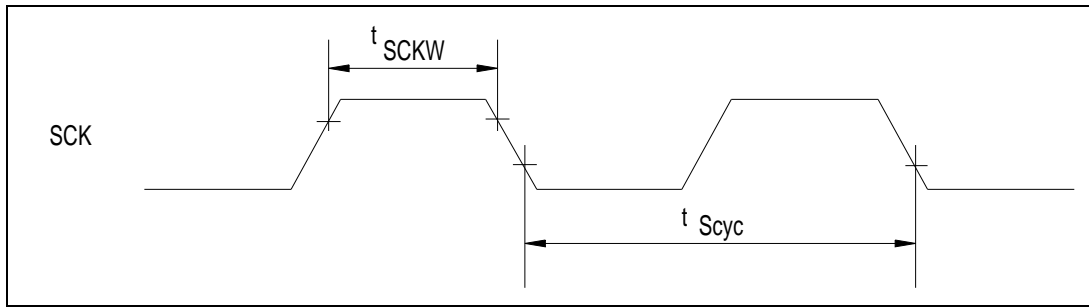
Figure 16-17. SCI Input Clock Timing
