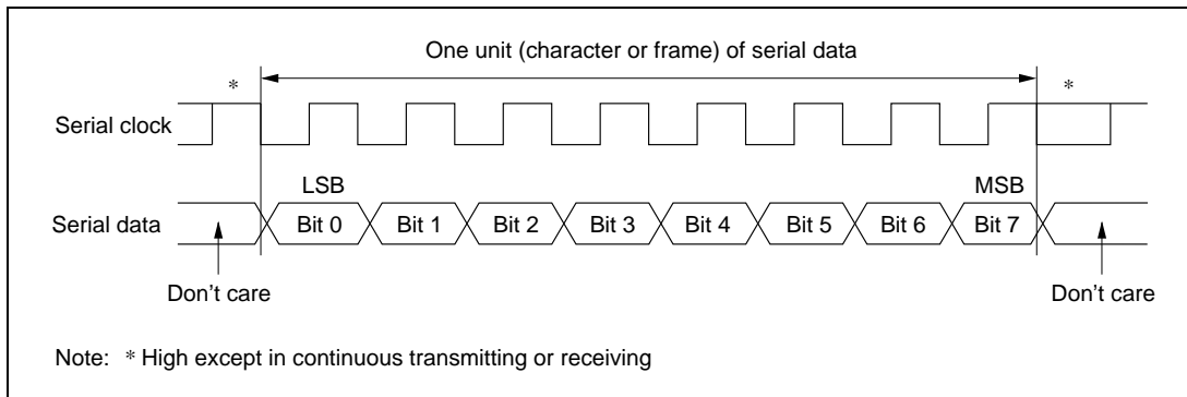
Figure 9-12. Data Format in Clocked Synchronous Communication
