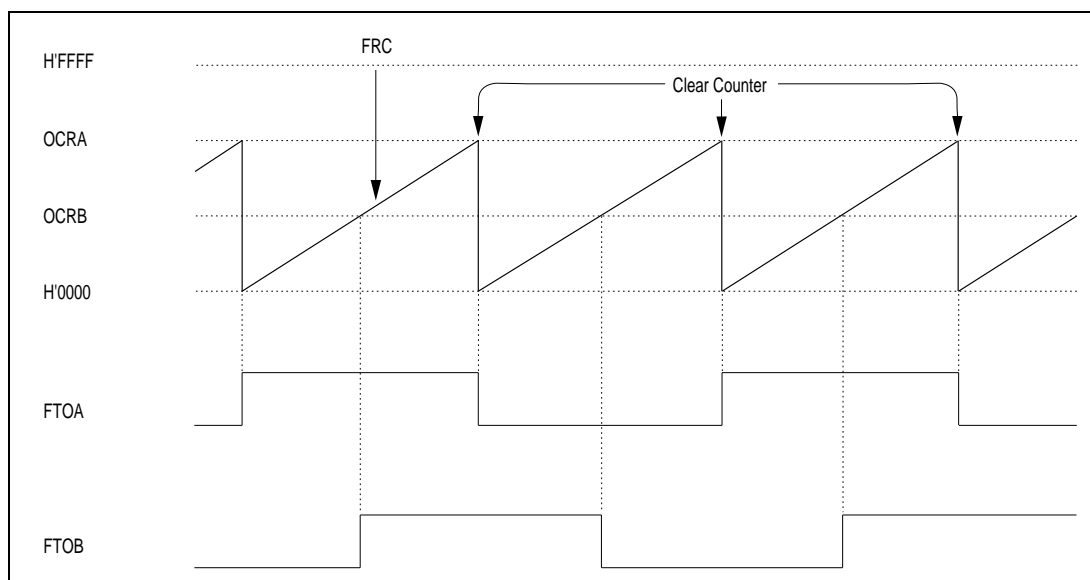
Figure 6-17. Square-Wave Output (Example)
