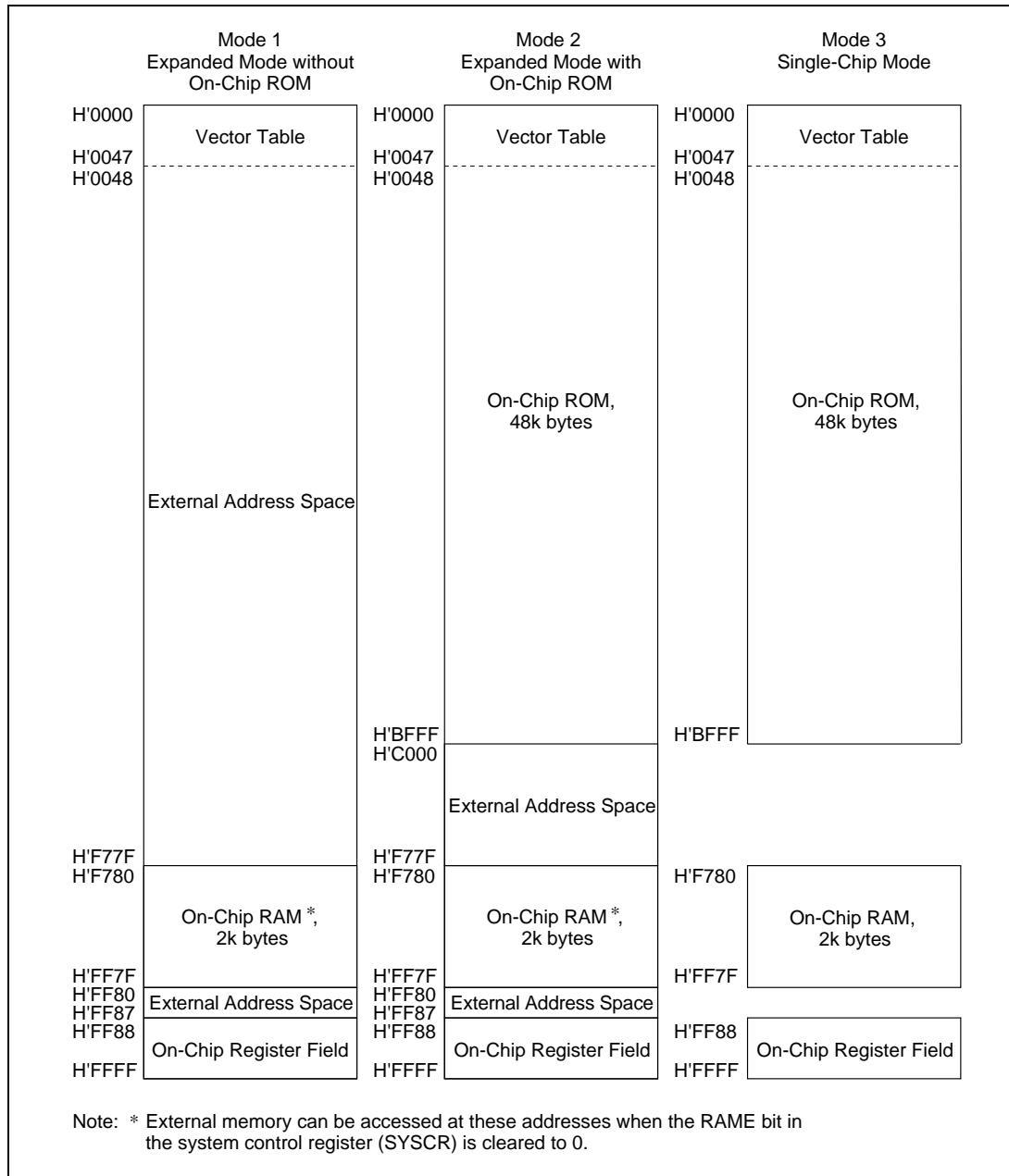
Figure 2-1. H8/338 Address Space Map
