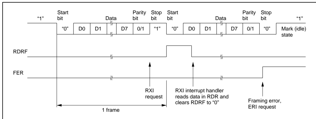
Figure 9-8. Example of SCI Receive Operation (8-Bit Data with Parity and One Stop Bit)
