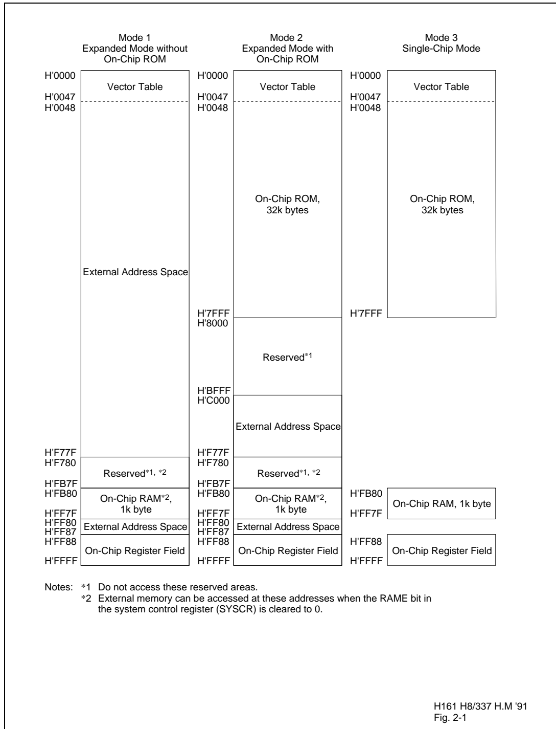
Figure 2-2. H8/337 Address Space Map
