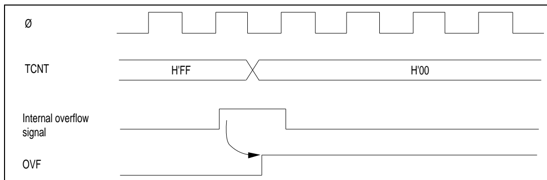
Figure 7-9. Setting of Overflow Flag (OVF)
