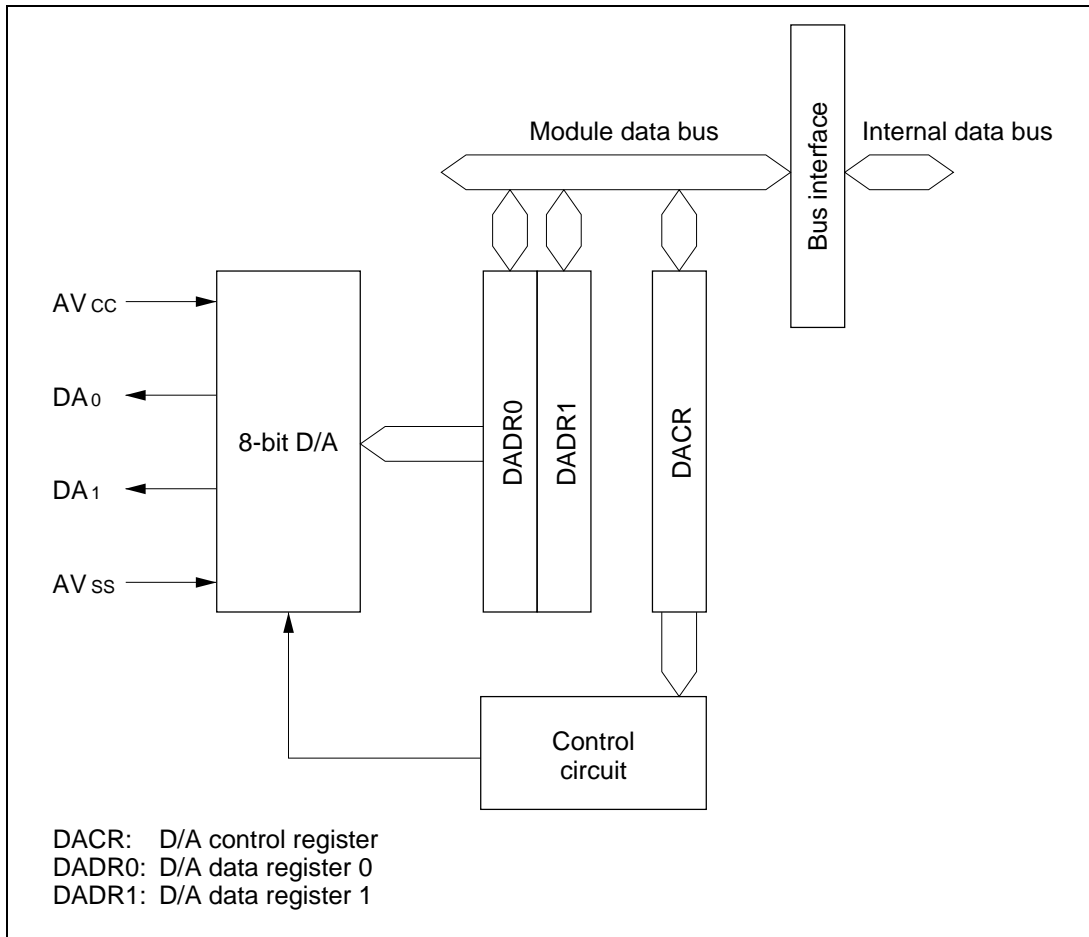
Figure 11-1. D/A Converter Block Diagram
