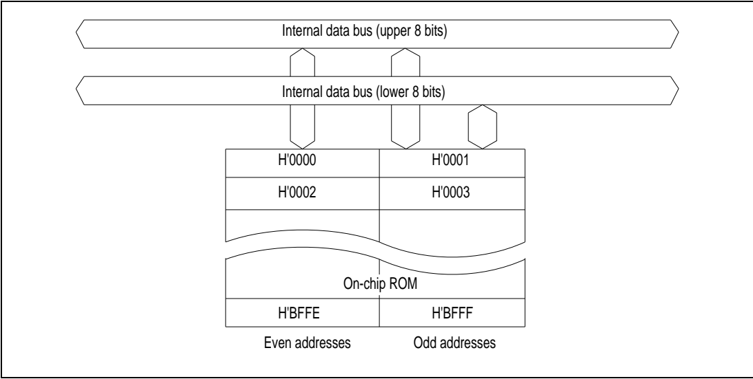
Figure 13-1. Block Diagram of On-Chip ROM (H8/338)
