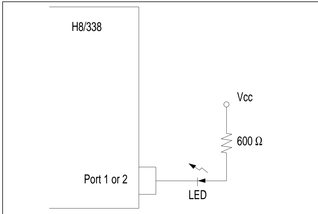
Figure 16-2. Example of Circuit for Driving an LED (5V Version)
