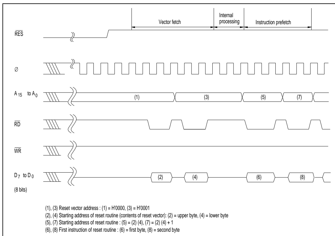
Figure 4-2. Reset Sequence (Model1)
