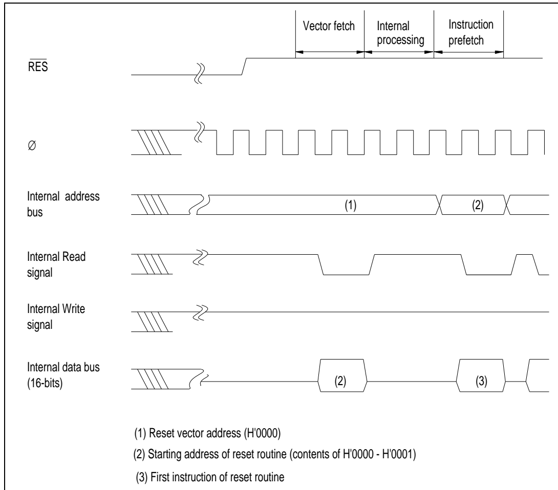
Figure 4-1. Reset Sequence (Mode 2 or 3, Program Stored in On-Chip ROM)
