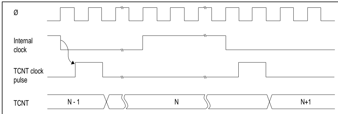
Figure 7-2. Count Timing for Internal Clock Input
