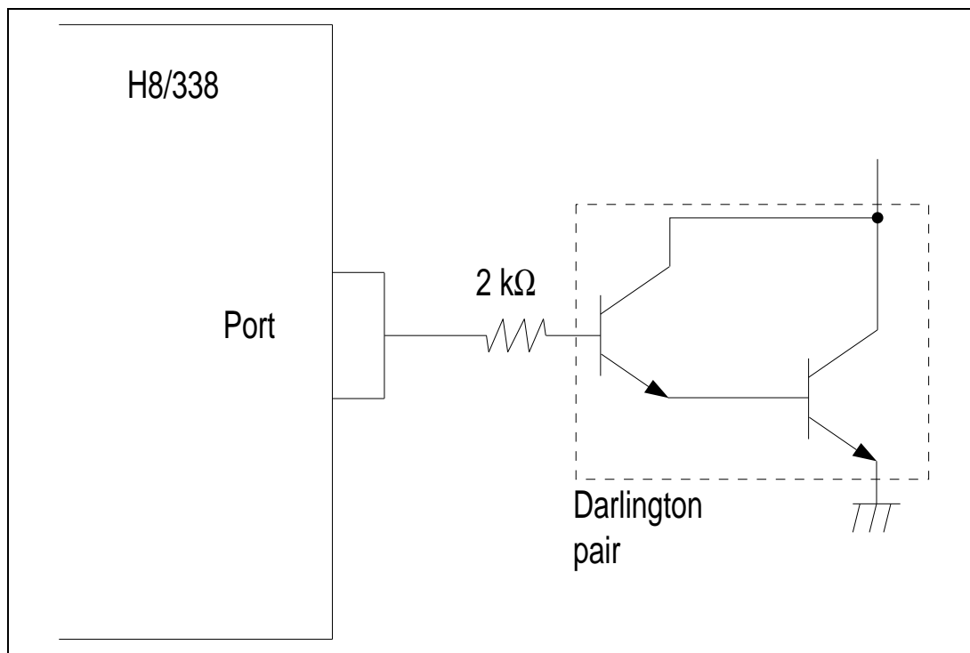
Figure 16-1. Example of Circuit for Driving a Darlington Pair (5V Version)
