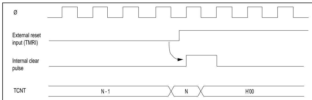
Figure 7-8. Timing of External Reset
