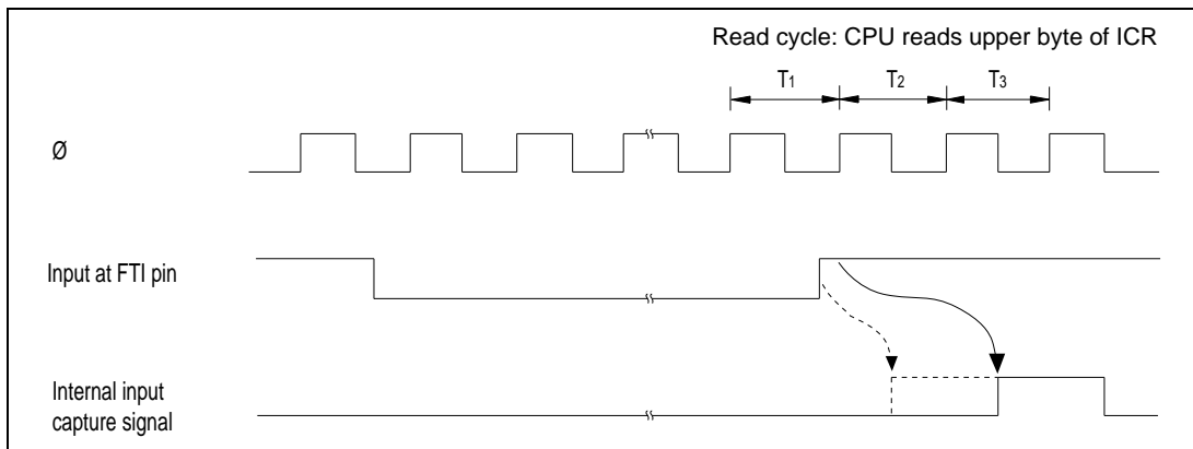
Figure 6-12. Input Capture Timing (1-State Delay)
