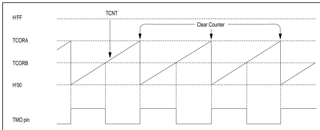
Figure 7-10. Example of Pulse Output
