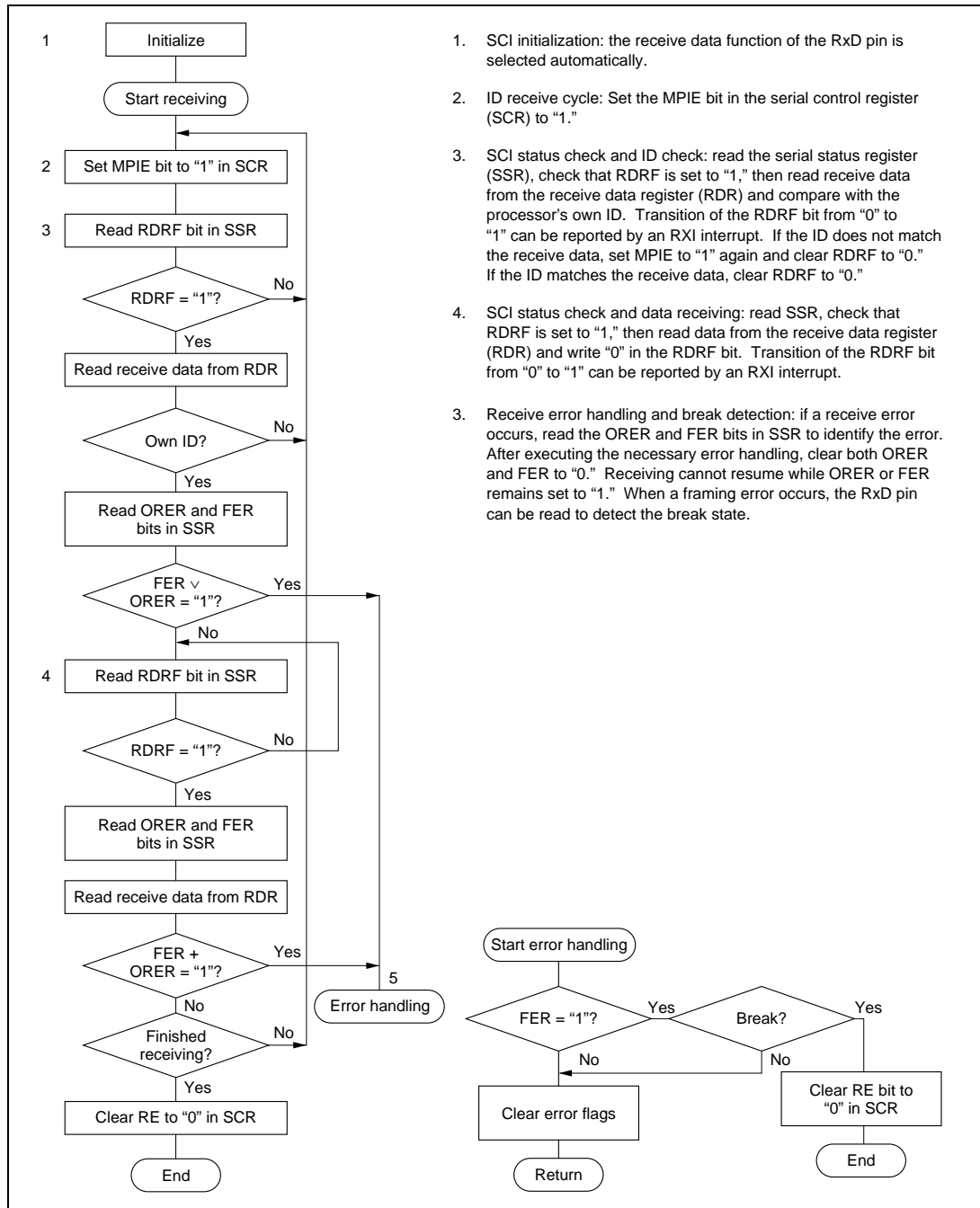
Figure 9-10. Sample Flowchart for Receiving Multiprocessor Serial Data
