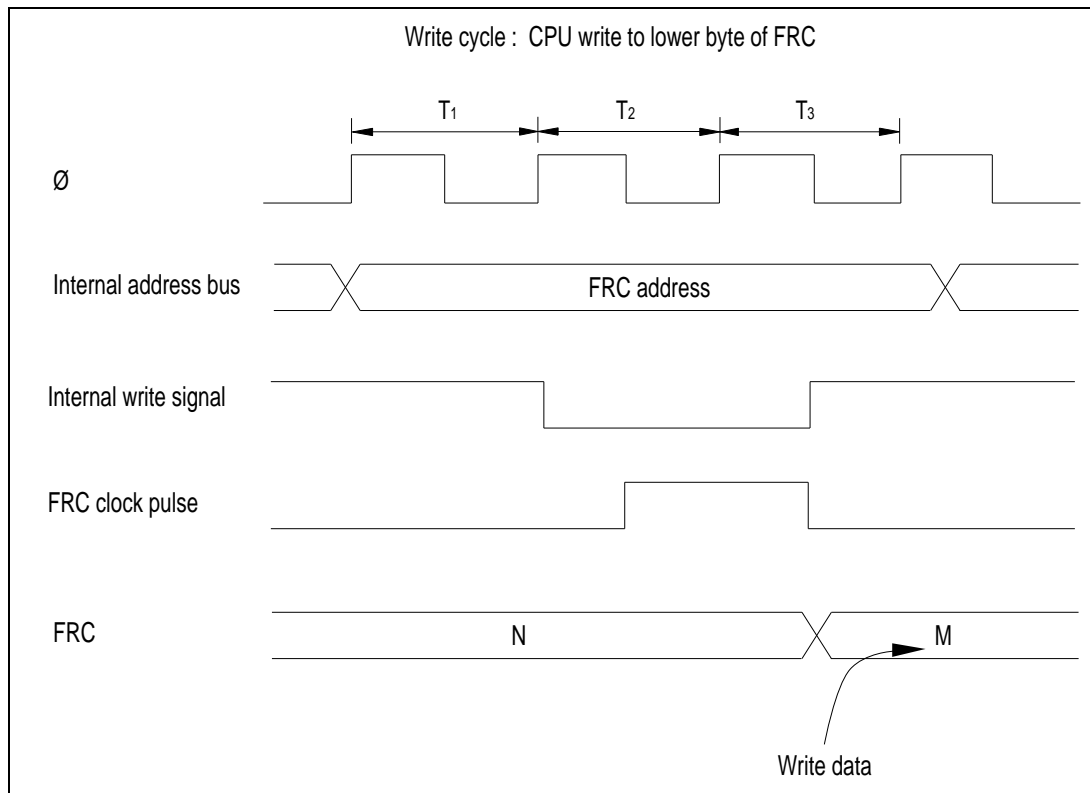
Figure 6-19. FRC Write-Increment Contention
