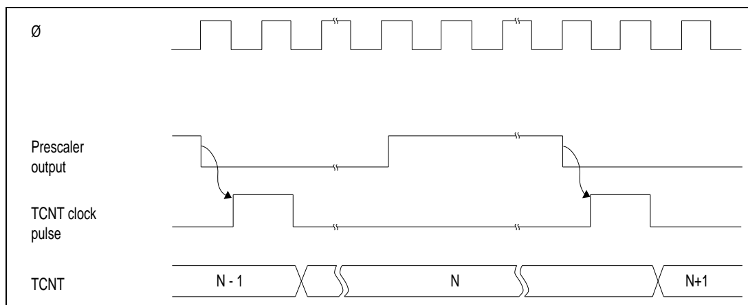
Figure 8-2. TCNT Increment Timing
