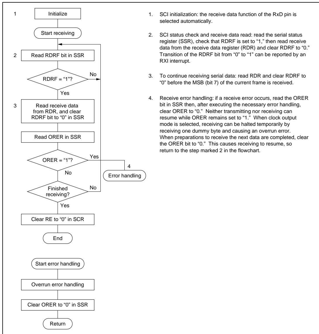
Figure 9-15. Sample Flowchart for Serial Receiving
