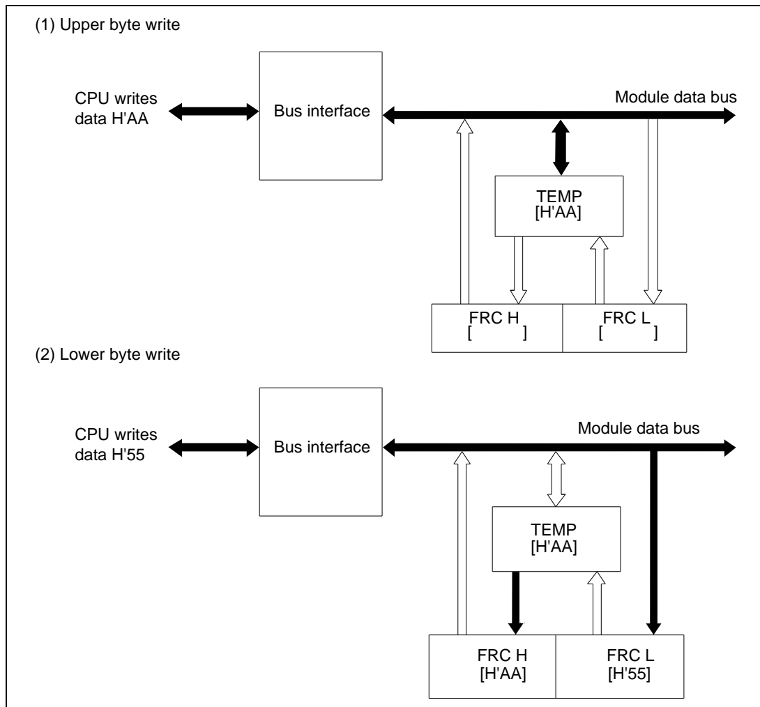
Figure 6-4 (a). Write Access to FRC (when CPU Writes H'AA55)
