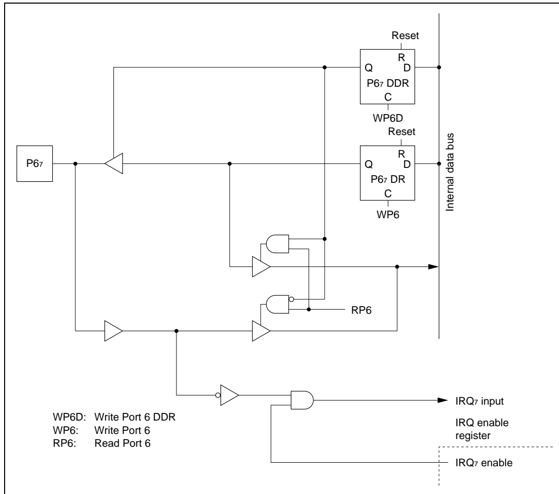
Figure 5-12. Port 6 Schematic Diagram (Pin P6 7 )
