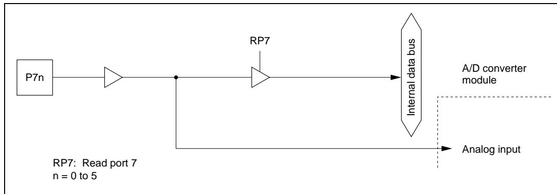
Figure 5-13. Port 7 Schematic Diagram (Pins P7 0 to P7 5 )
