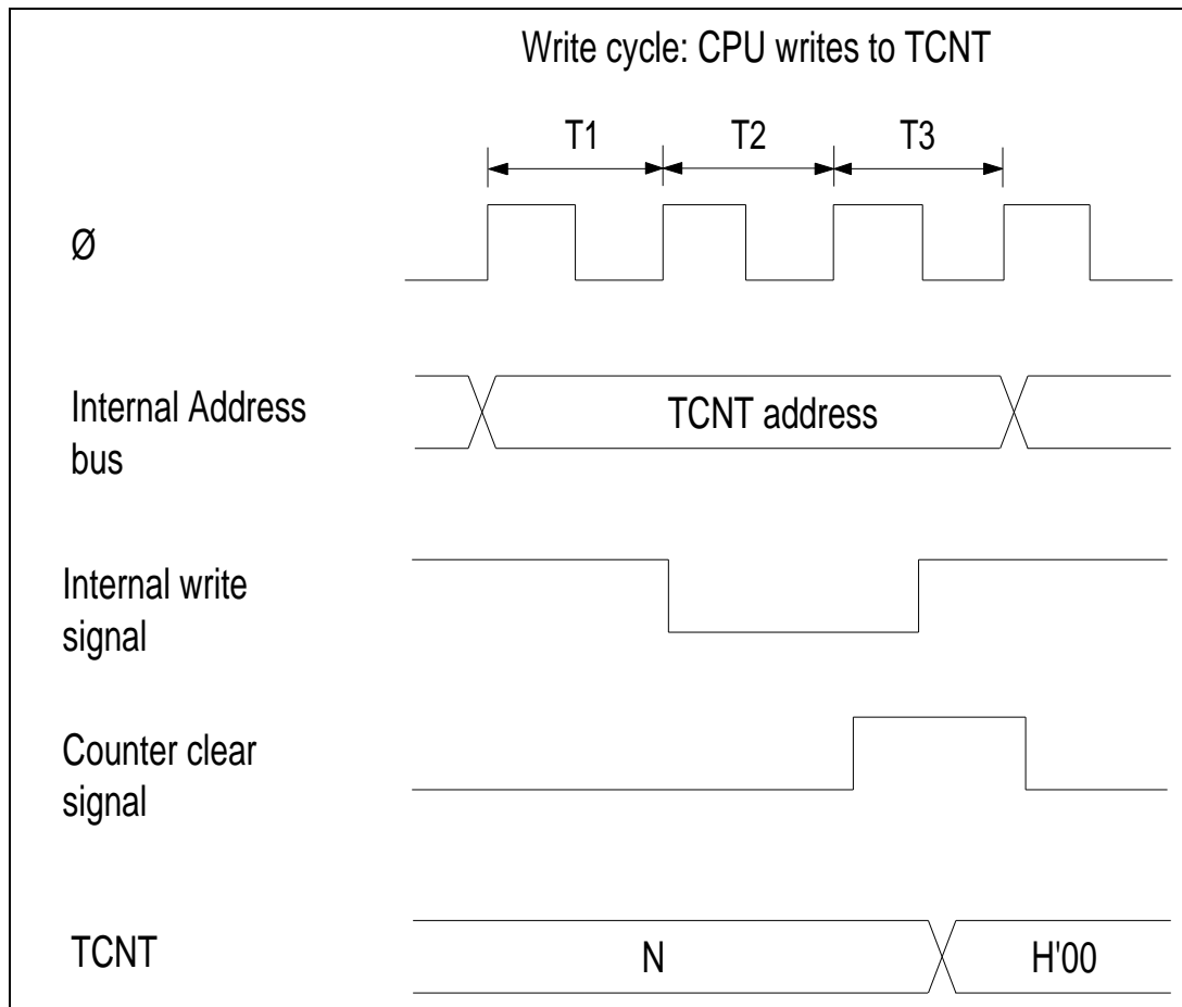
Figure 7-11. TCNT Write-Clear Contention
