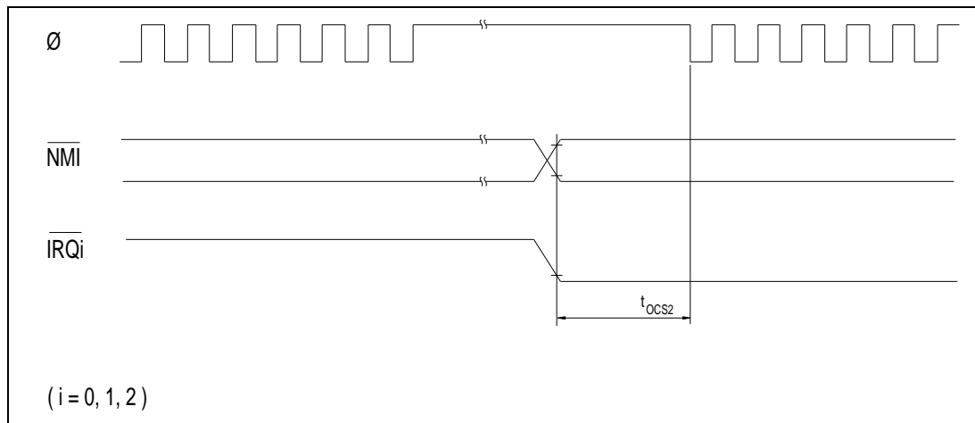
Figure 16-9. Clock Settling Timing for Recovery from Software Standby Mode
