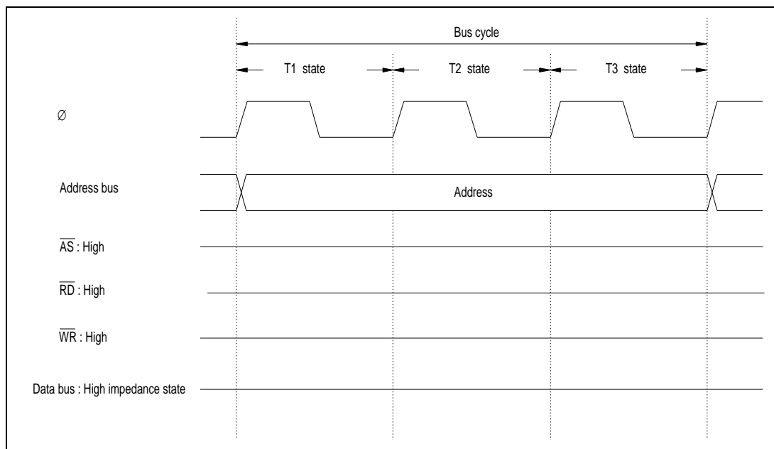
Figure 3-16. Pin States during On-Chip Register Field Access Cycle
