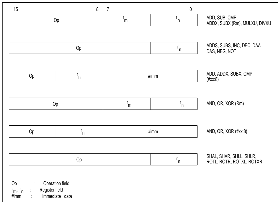
Figure 3-6. Arithmetic, Logic, and Shift Instruction Codes
