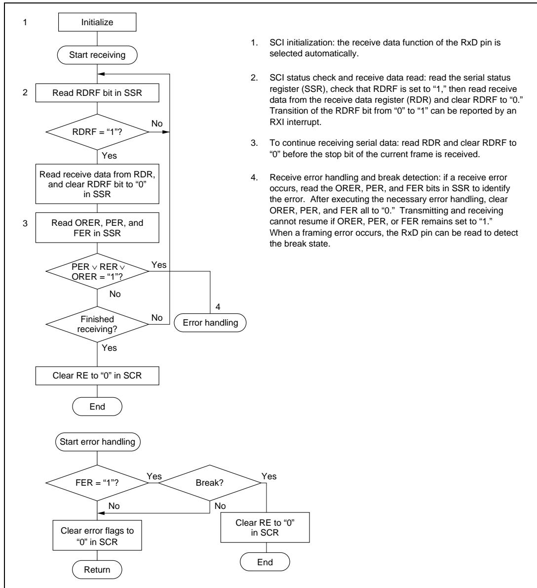
Figure 9-7. Sample Flowchart for Receiving Serial Data
