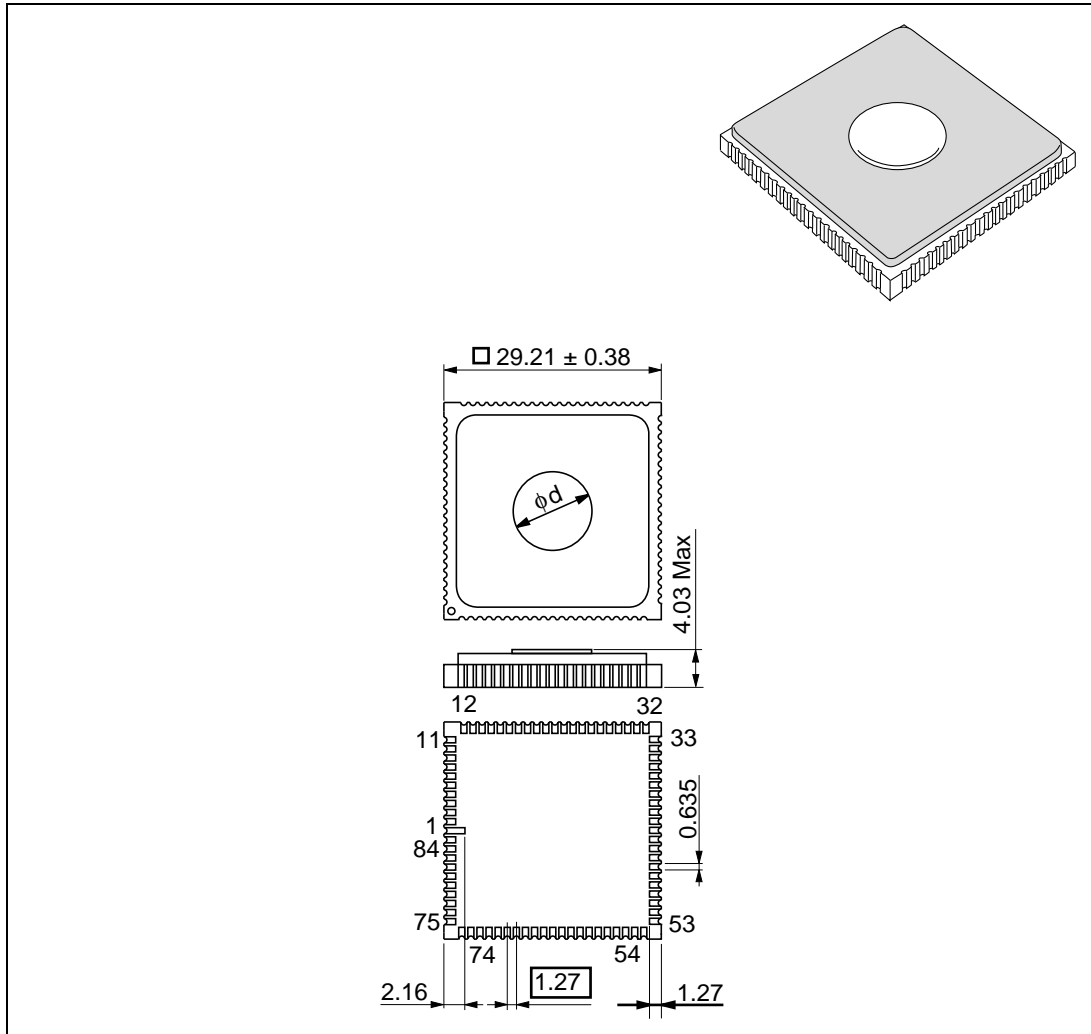
Figure E-1. Package Dimensions (CG-84)
