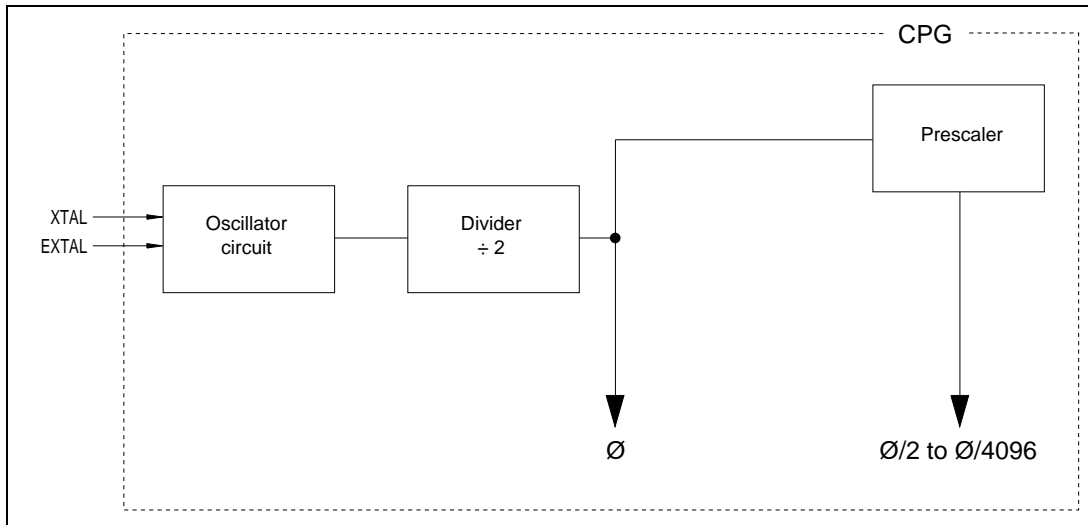
Figure 15-1. Block Diagram of Clock Pulse Generator
