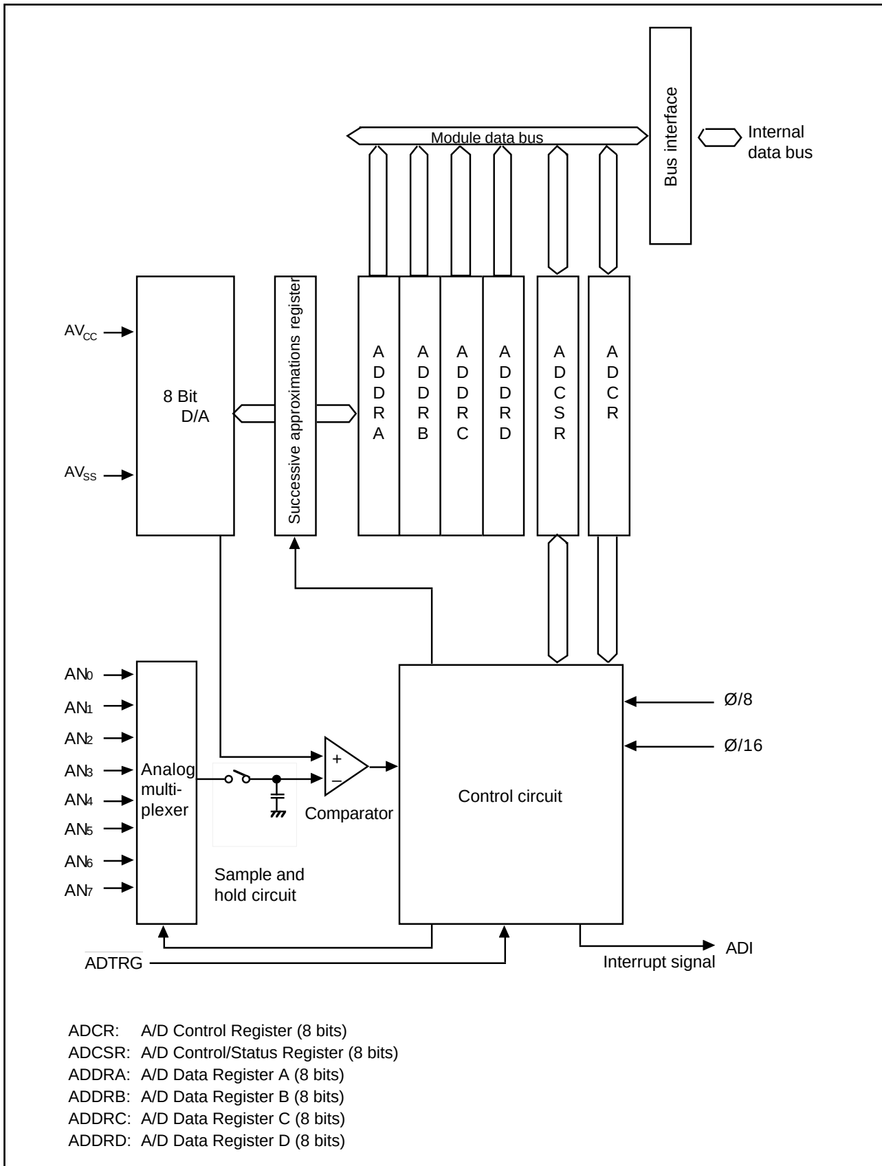
Figure 9-1. Block Diagram of A/D Converter
