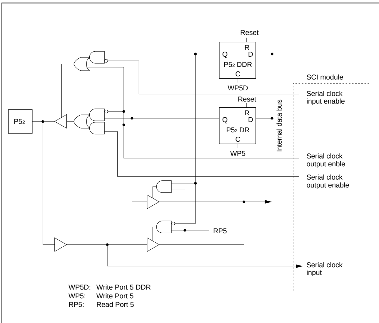
Figure 5-11. Port 5 Schematic Diagram (Pin P52)
