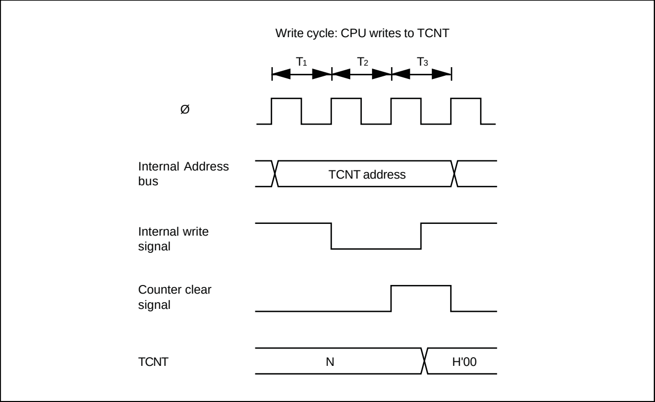
Figure 7-11. TCNT Write-Clear Contention
