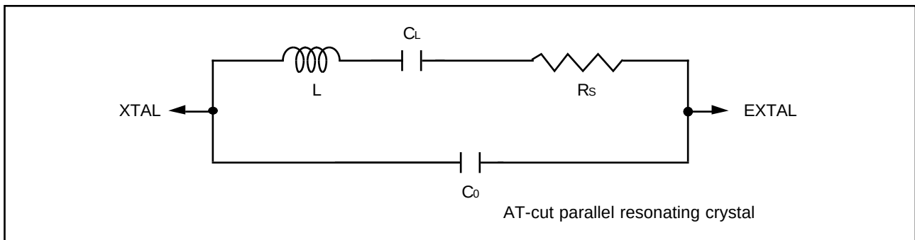
Figure 13-3. Equivalent Circuit of External Crystal
