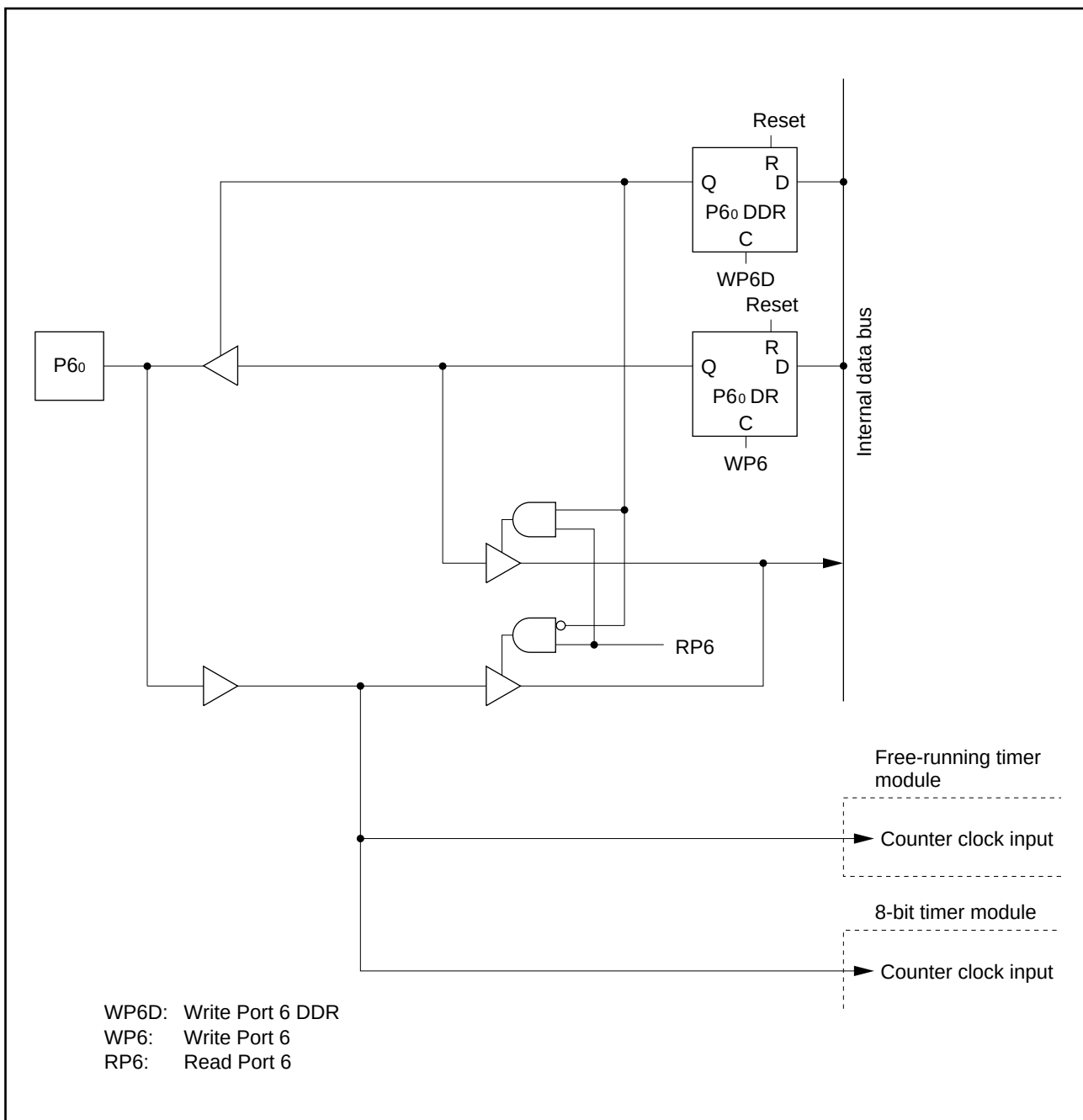
Figure 5-12. Port 6 Schematic Diagram (Pin P60)
