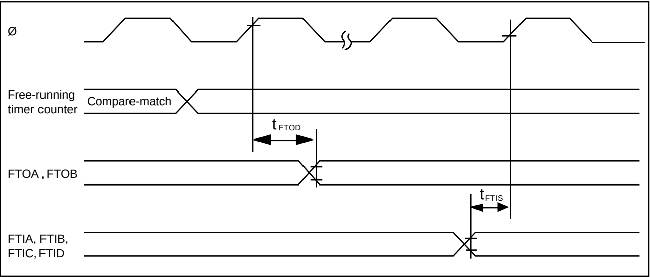
Figure 14-10. Free-Running Timer Input/Output Timing
