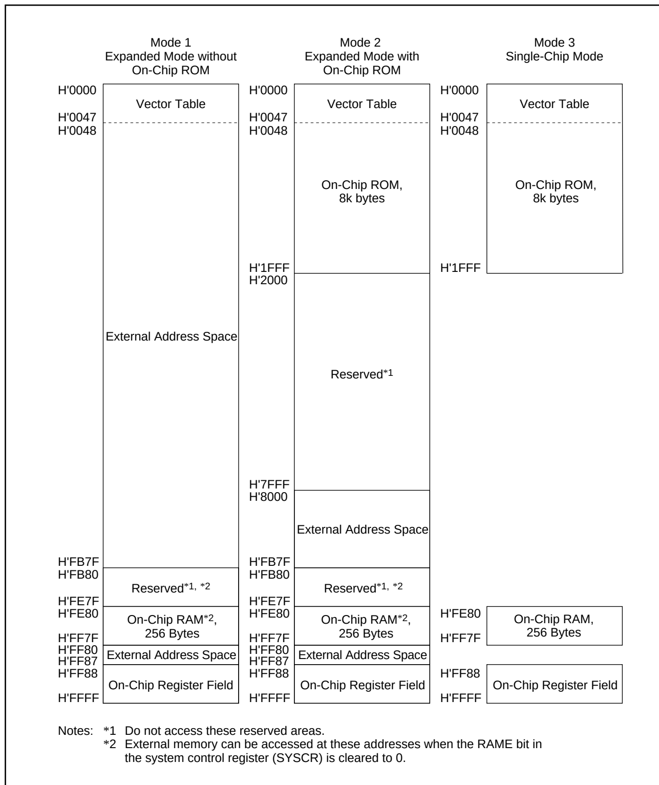
Figure 2-4. H8/326 Address Space Map
