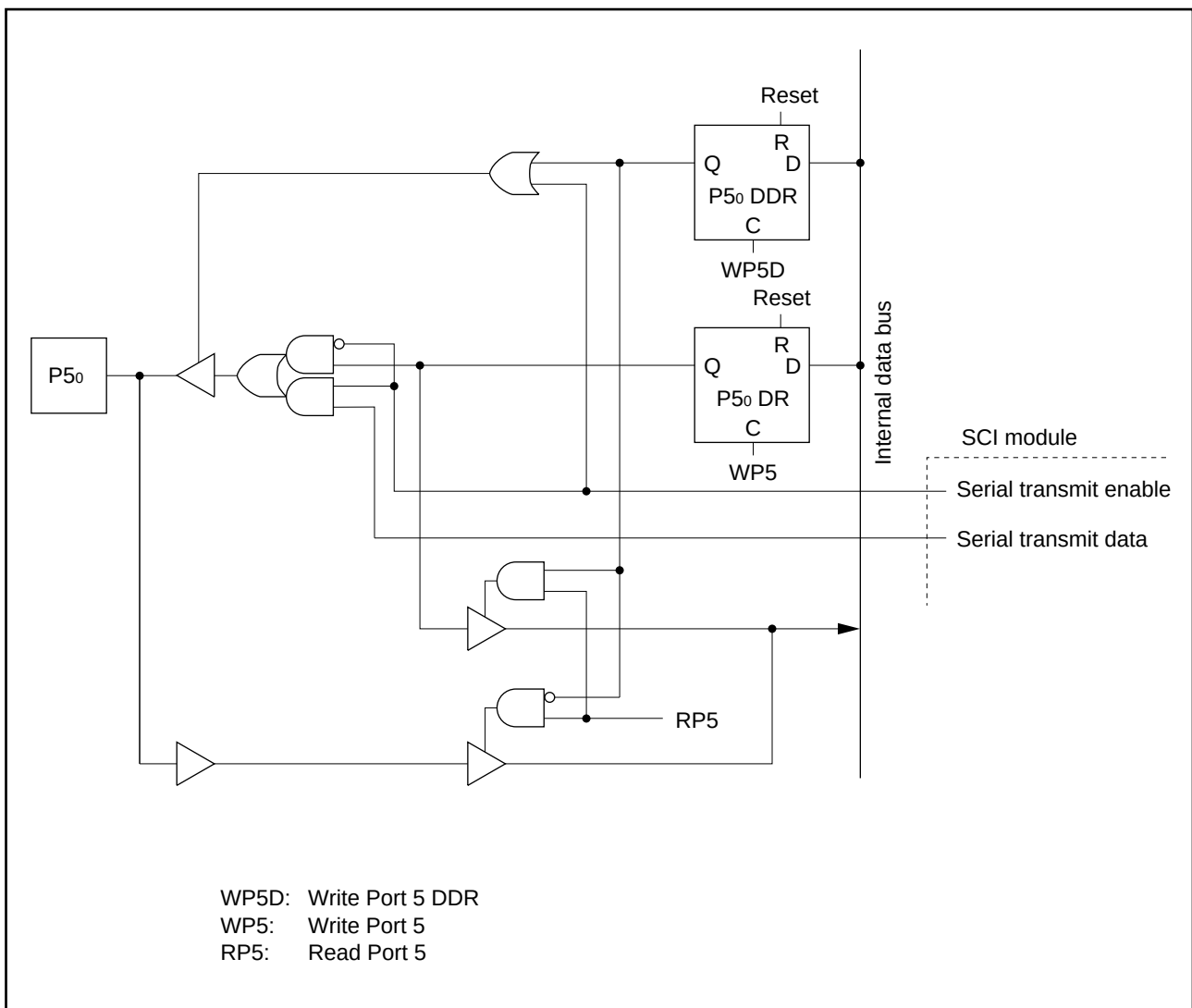
Figure 5-9. Port 5 Schematic Diagram (Pin P50)
