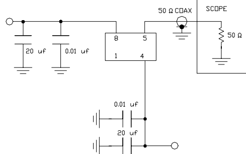
TEST CIRCUIT
