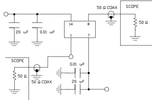
TEST CIRCUIT
