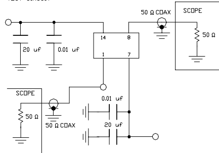
TEST CIRCUIT
