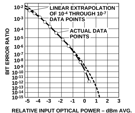
Figure 3. Relative Input Optical Power dBm Average.
